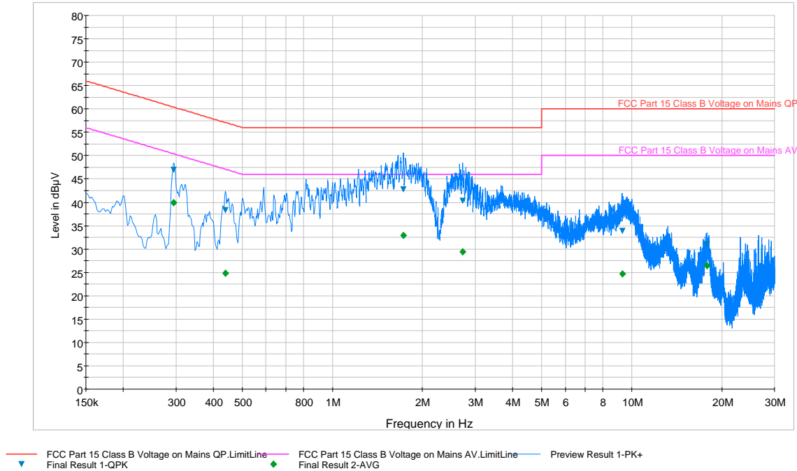
Plot 6-94. Line Conducted Plot with 802.11a UNII Band 3 (L1)
