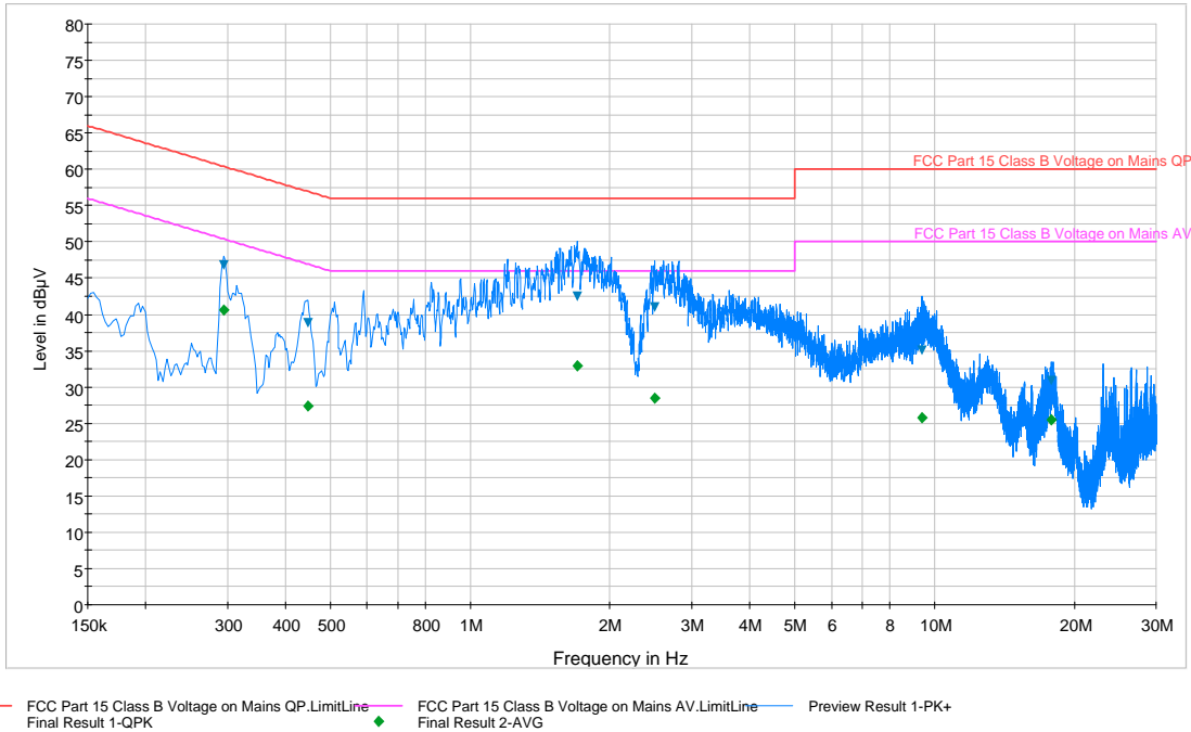
Plot 6-92. Line Conducted Plot with 802.11a UNII Band 2 (L1)
