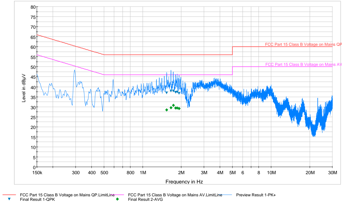
Plot 6-93. Line Conducted Plot with 802.11a UNII Band 2 (N)
