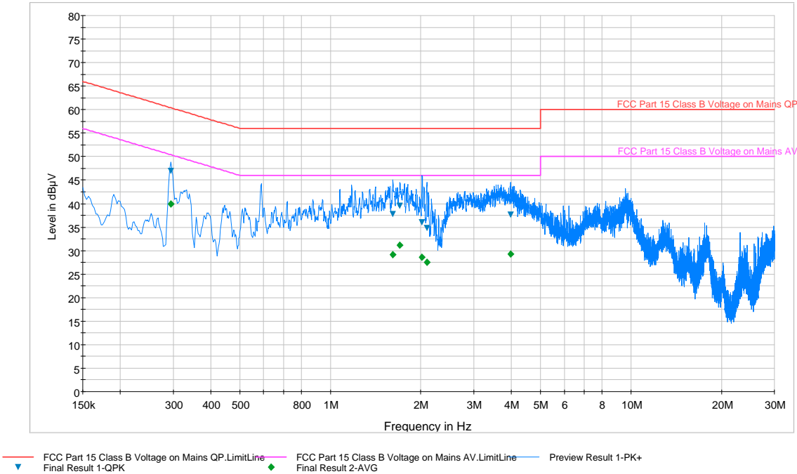
Plot 6-91. Line Conducted Plot with 802.11a UNII Band 1 (N)
