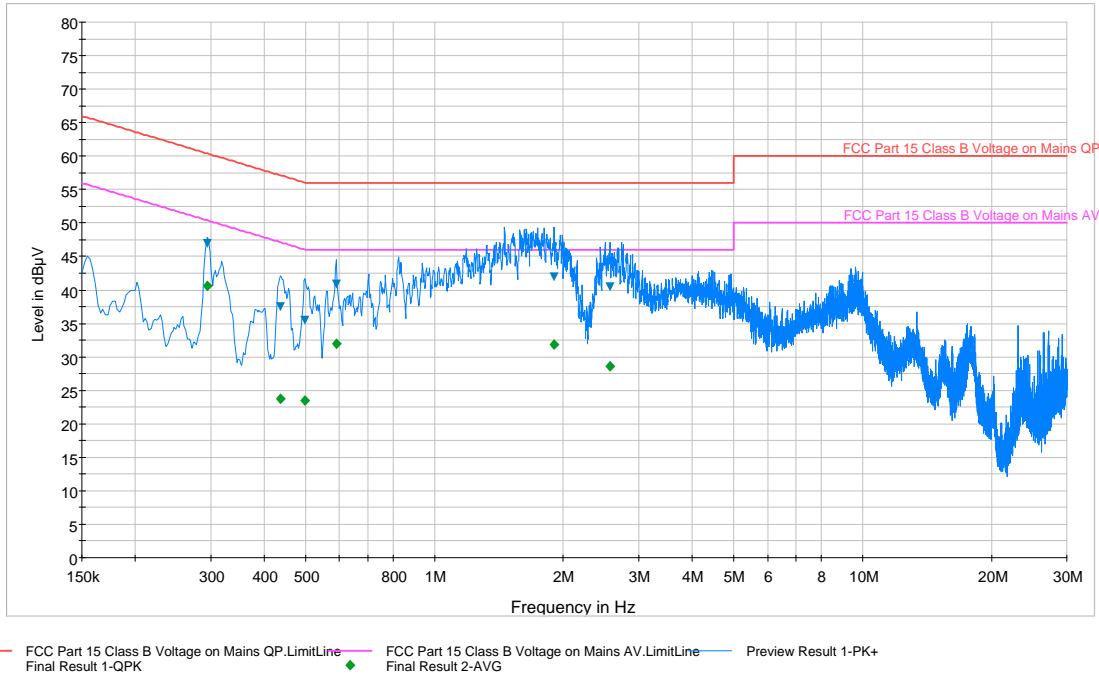
Plot 6-90. Line Conducted Plot with 802.11a UNII Band 1 (L1)
