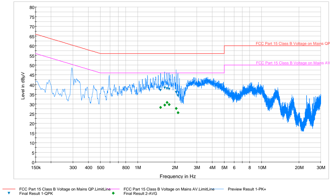
Plot 6-95. Line Conducted Plot with 802.11a UNII Band 3 (N)
