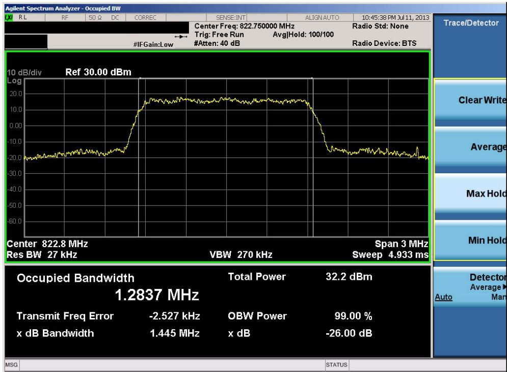
Plot 7-12. Occupied Bandwidth Plot (Ch. 670)
