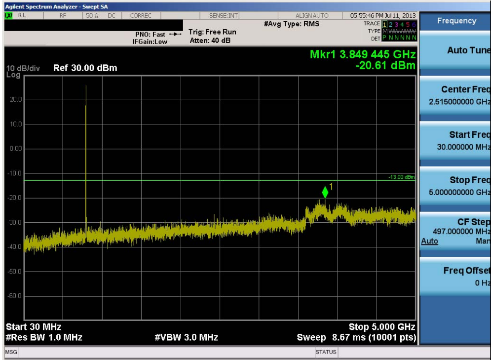
Plot 7-1. Conducted Spurious Plot (Ch. 476)
