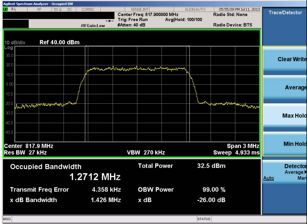
Plot 7-11. Occupied Bandwidth Plot (Ch. 476)
