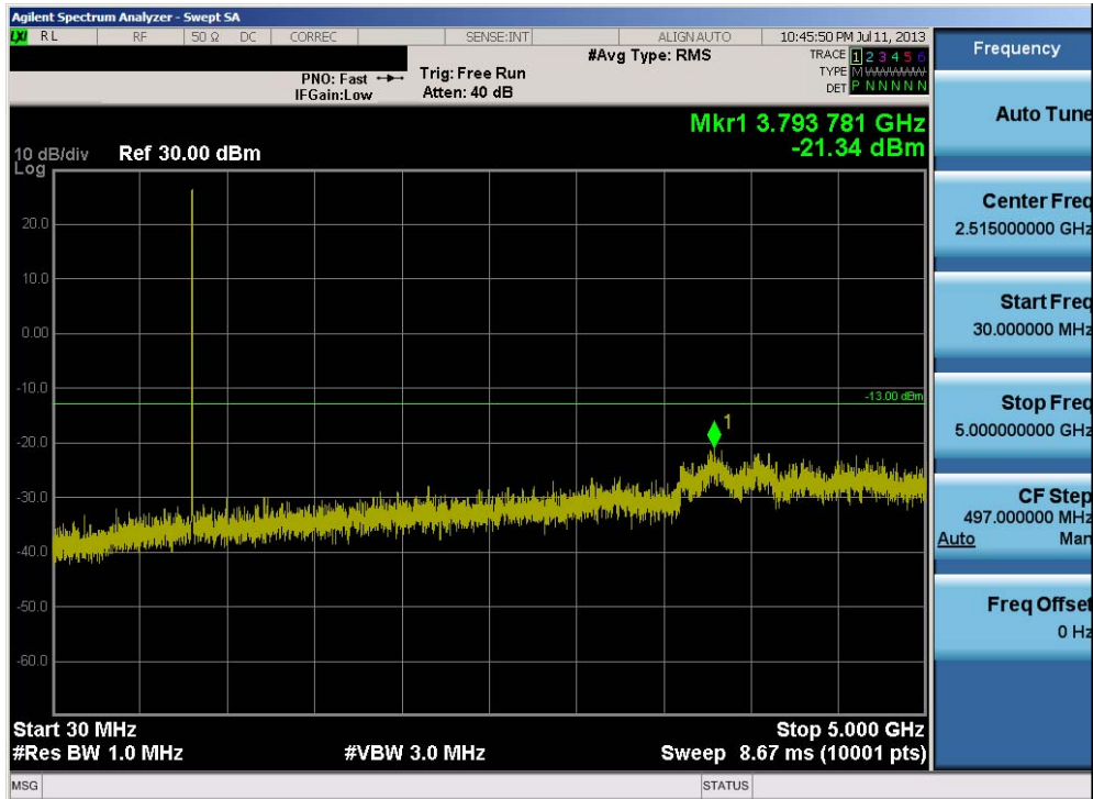
Plot 7-6. Conducted Spurious Plot (Ch. 670)
