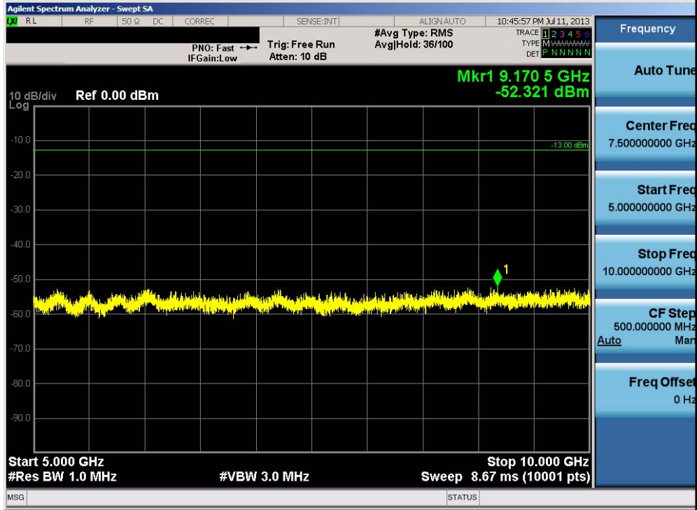
Plot 7-7. Conducted Spurious Plot (Ch. 670)
