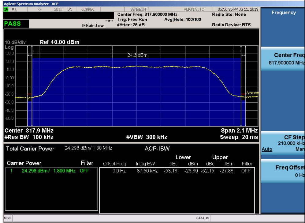
Plot 7-3. Channel Edge Plot (Ch. 476)
