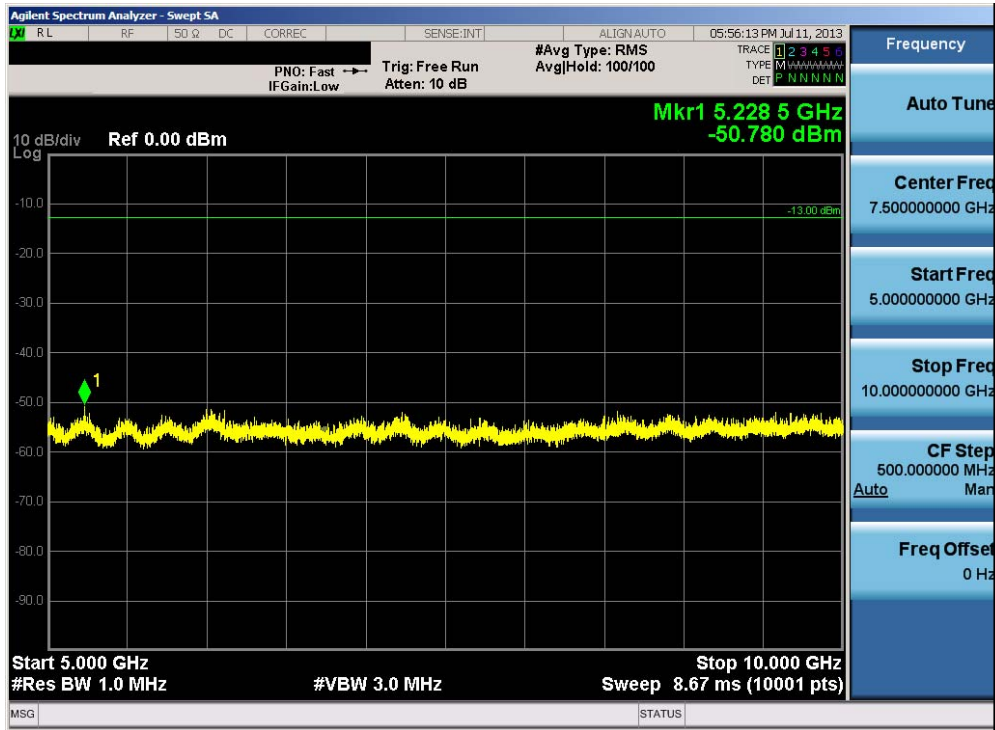
Plot 7-2. Conducted Spurious Plot (Ch. 476)
