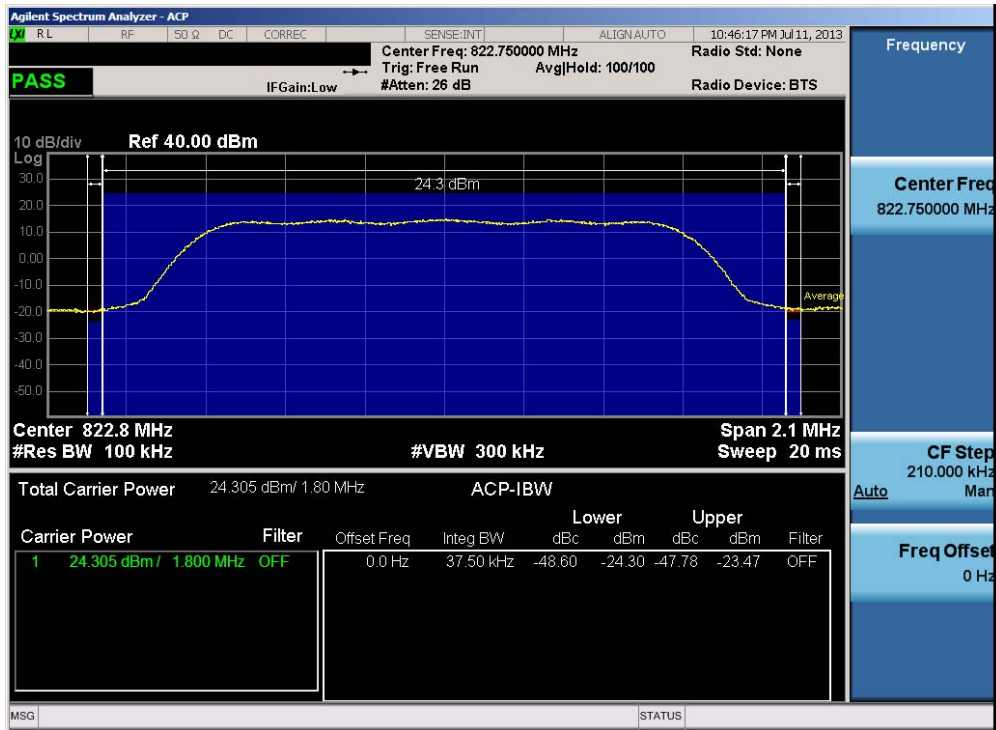
Plot 7-8. Channel Edge Plot (Ch. 670)
