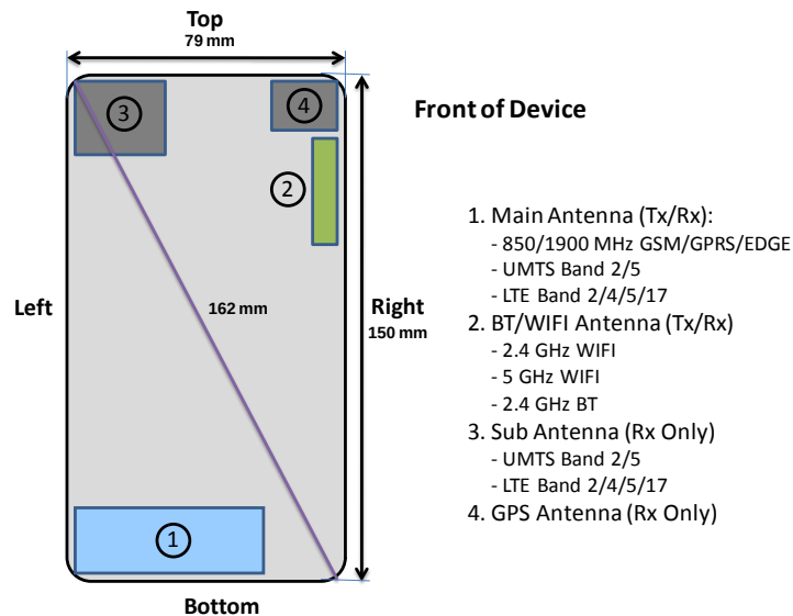
Figure 1-1 DUT Antenna Locations
