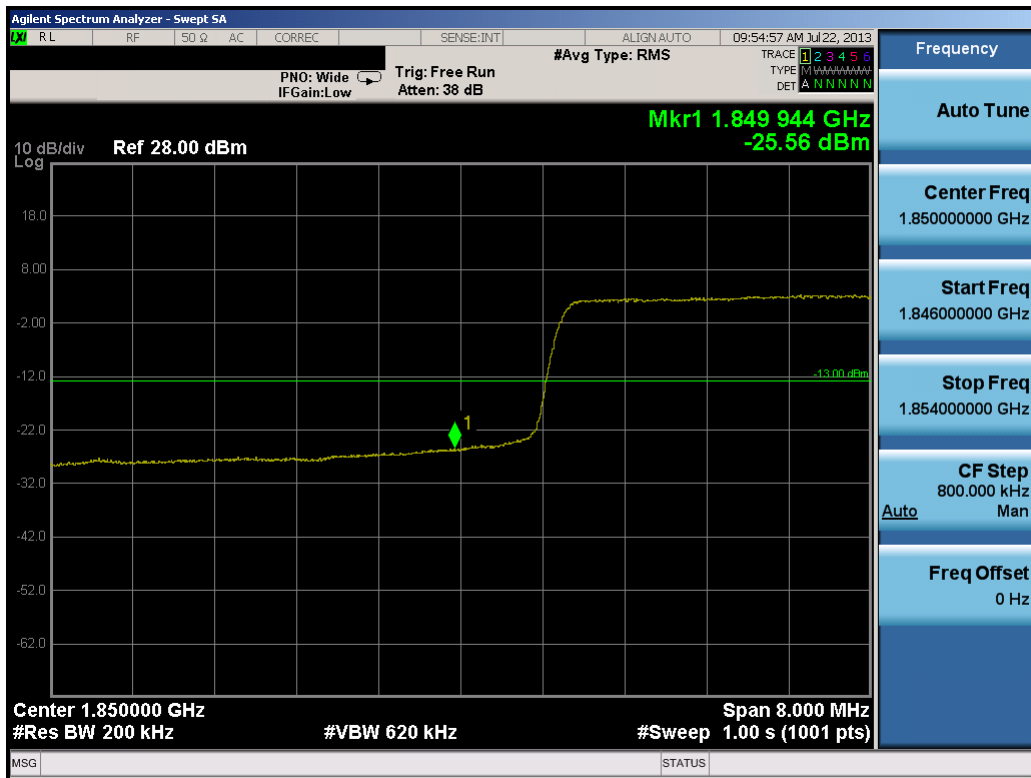
Plot 10-71. Lower Band Edge Plot (20.0MHz QPSK – RB Size 100)
