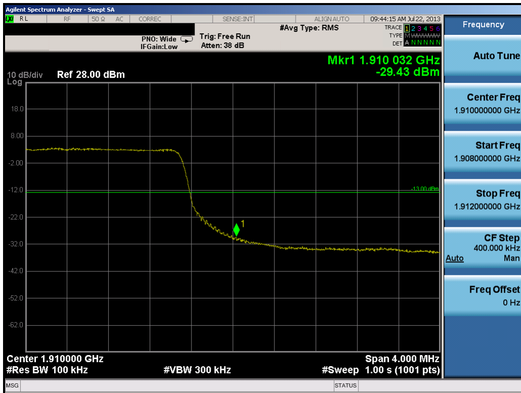
Plot 10-53. Upper Band Edge Plot (10.0MHz QPSK – RB Size 50)
