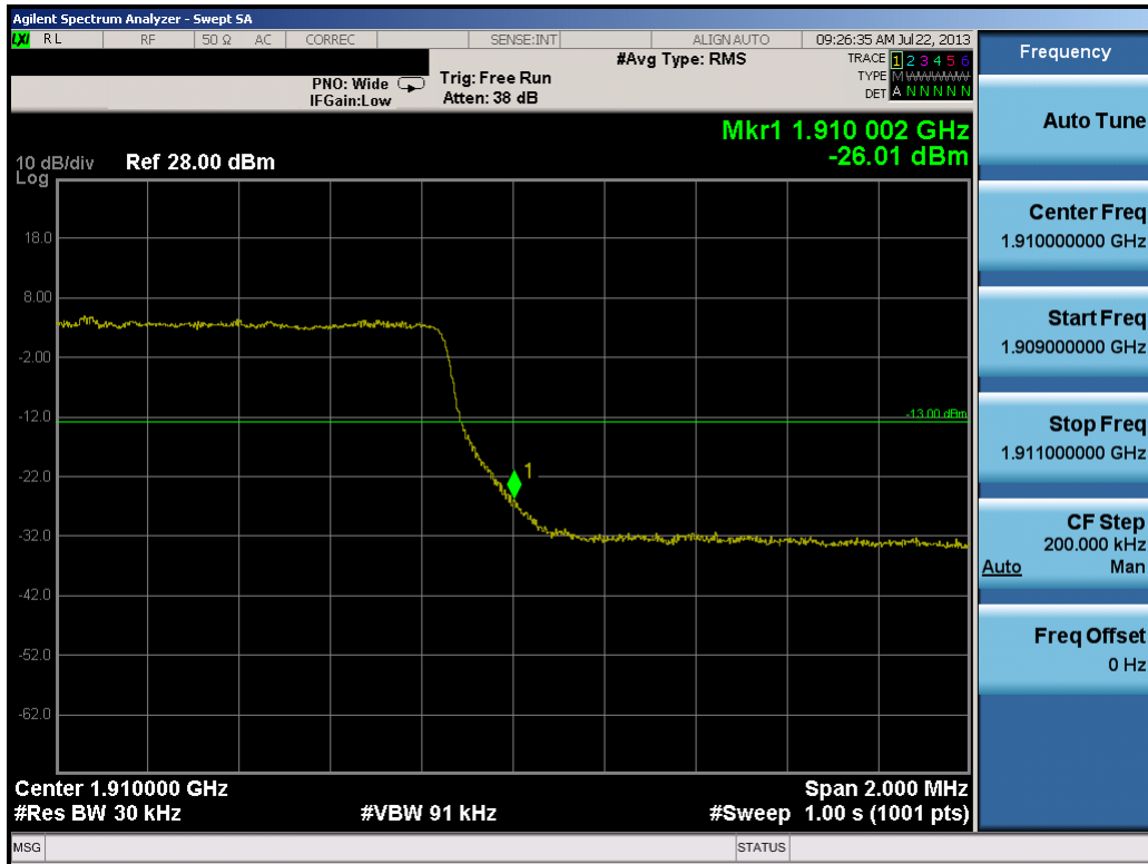
Plot 10-25. Upper Band Edge Plot (3.0MHz QPSK – RB Size 15)
