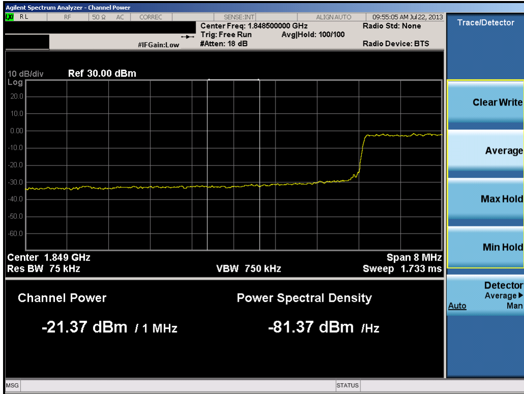
Plot 10-72. Lower Extended Band Edge Plot (20.0MHz QPSK – RB Size 100)
