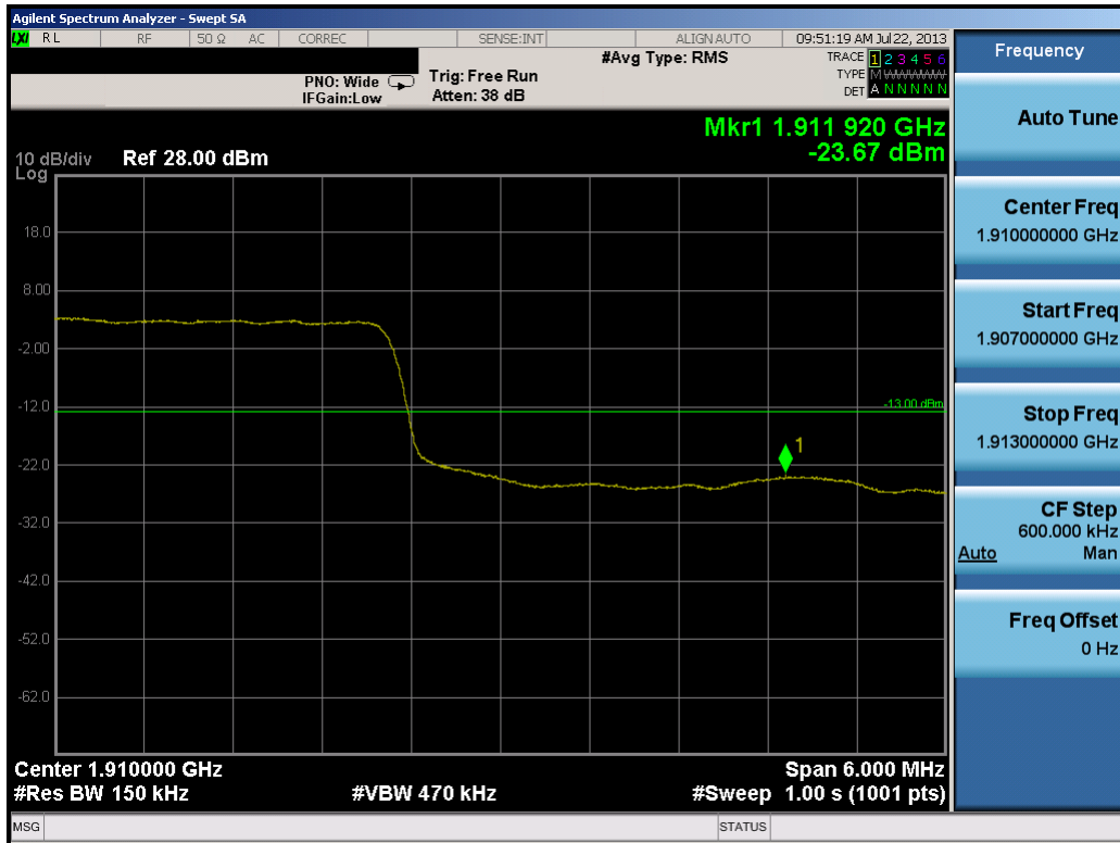
Plot 10-67. Upper Band Edge Plot (15.0MHz QPSK – RB Size 75)
