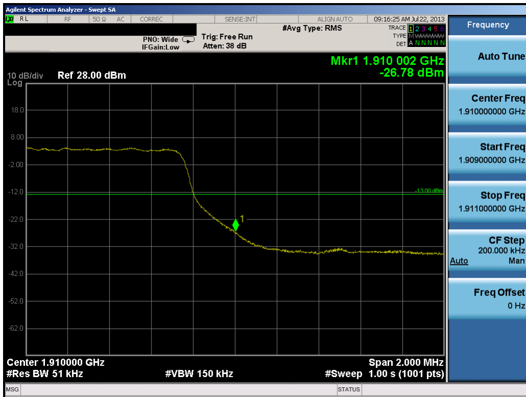
Plot 10-39. Upper Band Edge Plot (5.0MHz QPSK – RB Size 25)
