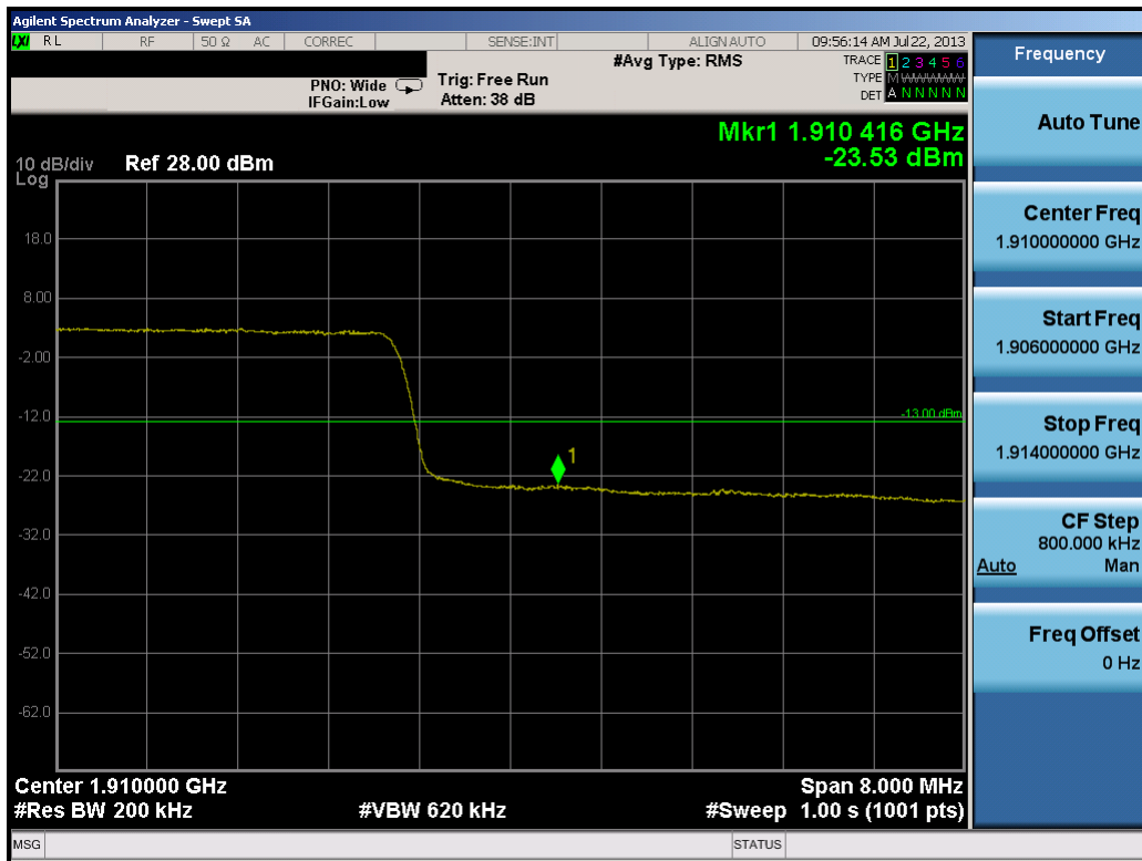
Plot 10-81. Upper Band Edge Plot (20.0MHz QPSK – RB Size 100)
