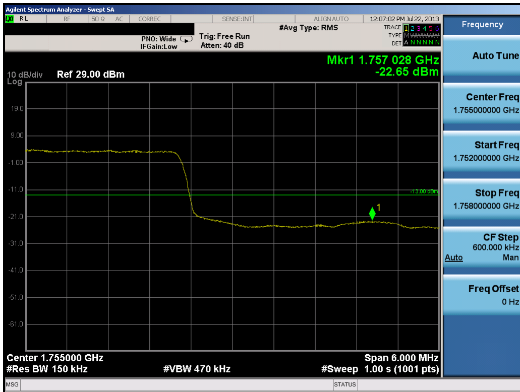
Plot 9-67. Upper Band Edge Plot (15.0MHz QPSK – RB Size 75)
