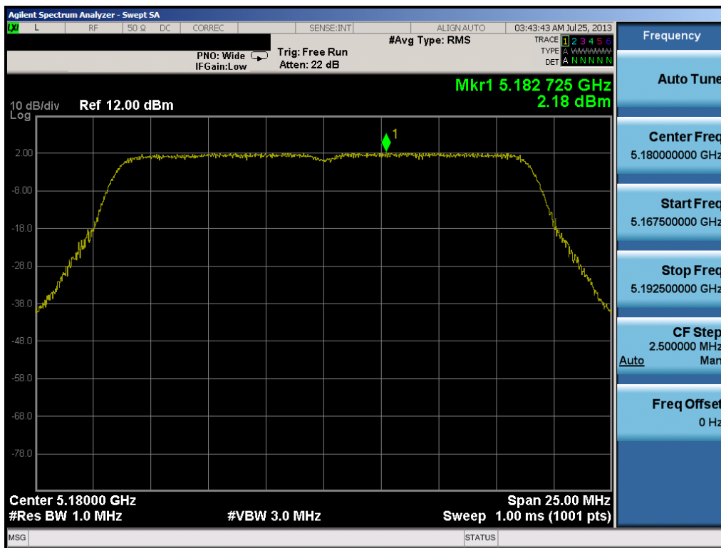
Plot 6-33. Peak Power Spectral Density Plot (20MHz BW 802.11n (UNII Band 1) – Ch. 36)
