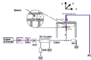
Figure 9-1 System Verification Setup Diagram
