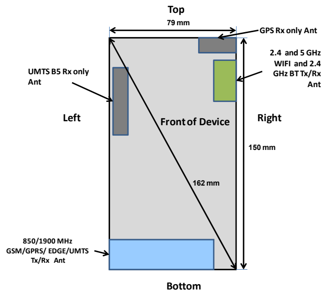
Figure 1-1 DUT Antenna Locations
