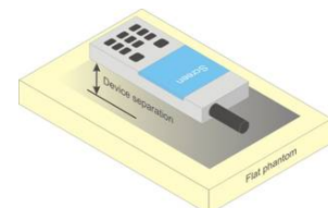
Figure 5-5 Sample Body-Worn Diagram
