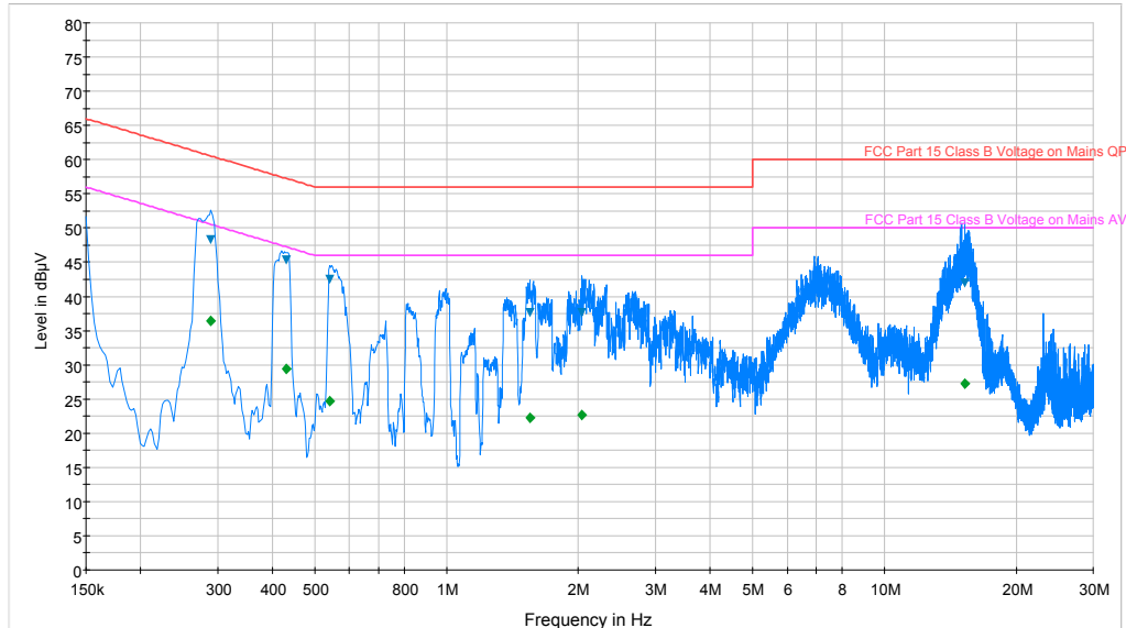
— FCC Part 15 Class B Voltage on Mains QP.LimitLine — FCC Part 15 Class B Voltage on Mains AV.LimitLine — Preview Result 1-QP+ ▼ Final Result 1-QPK ◆ Final Result 2-AVG
