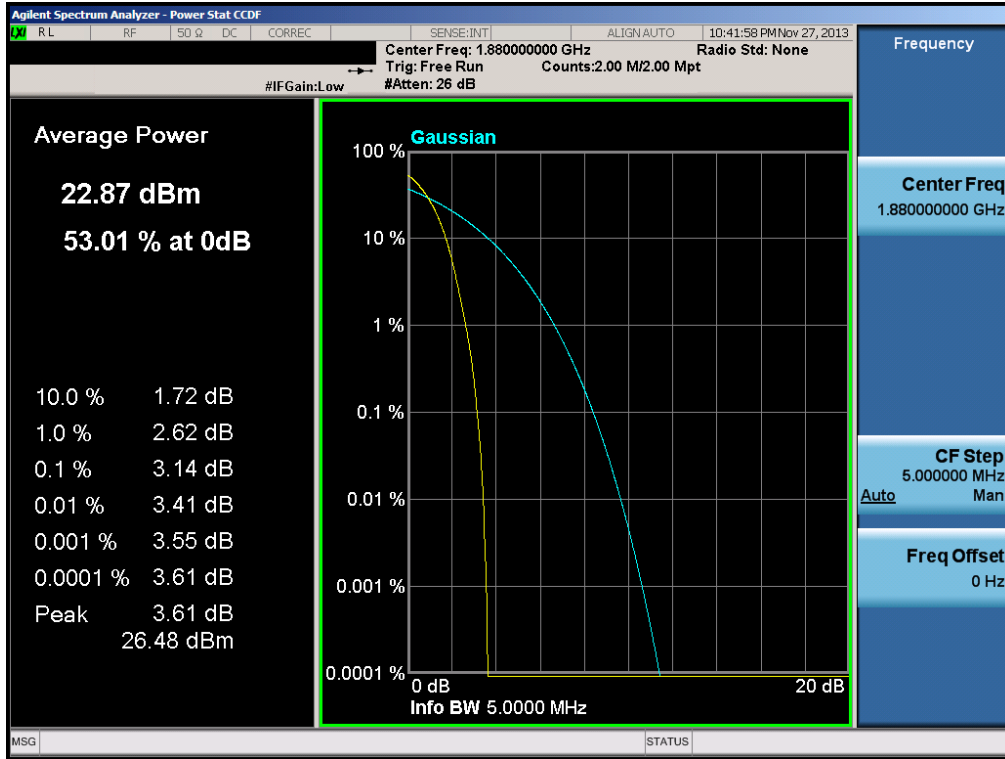
Plot 6-44. Peak-Average Ratio Plot (PCS WCDMA Mode – Ch. 9400)
