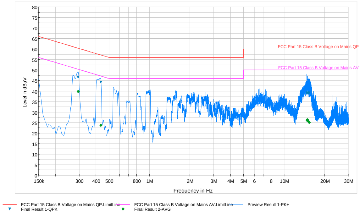
Plot 6-83. Line Conducted Plot with 802.11a UNII Band 1 (N)
