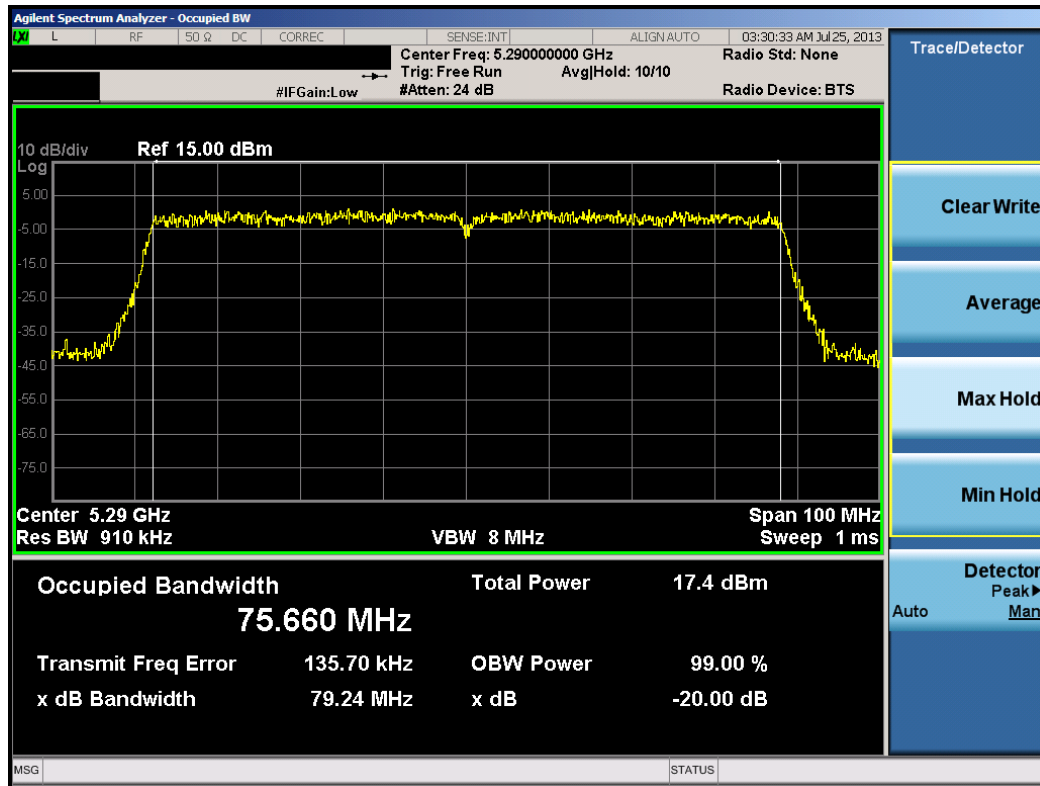
Plot 6-29. 20dB Bandwidth Plot (80MHz BW 802.11ac (UNII Band 2) – Ch. 58)
