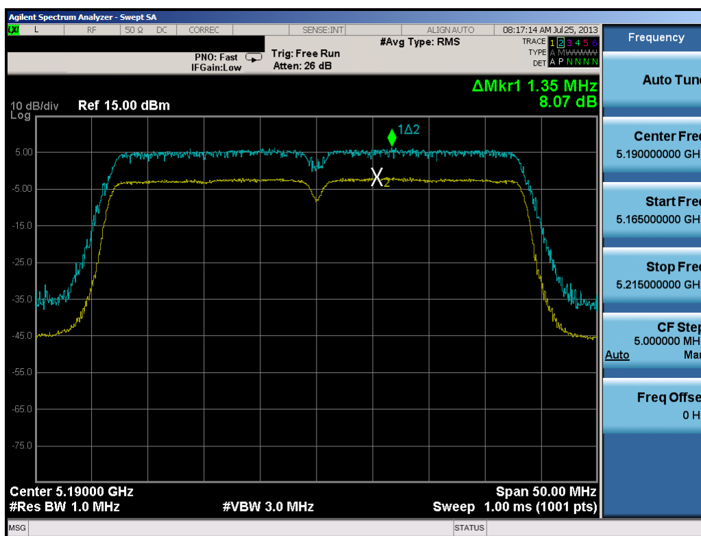
Plot 6-60. Peak Excursion Ratio Plot (40MHz BW 802.11n)
