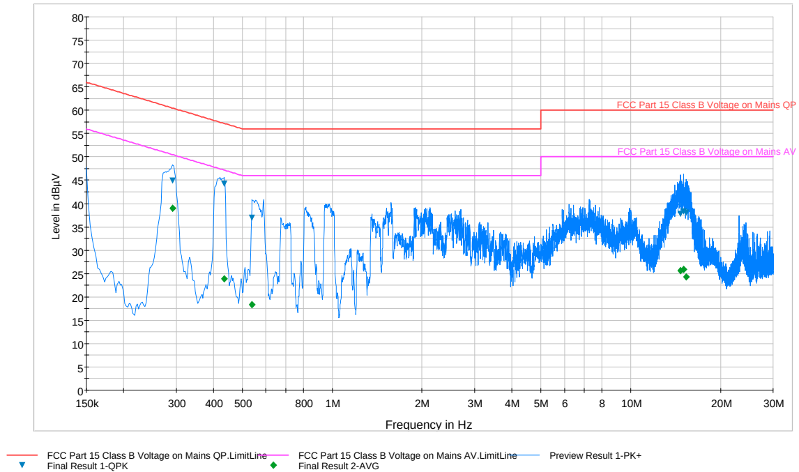
Plot 6-85. Line Conducted Plot with 802.11a UNII Band 2 (N)
