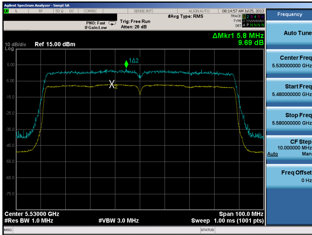
Plot 6-61. Peak Excursion Ratio Plot (80MHz BW 802.11ac)
