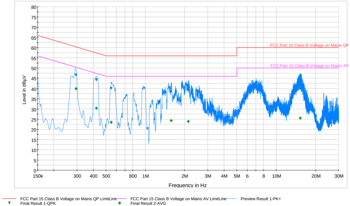
Plot 6-86. Line Conducted Plot with 802.11a UNII Band 3 (L1)
