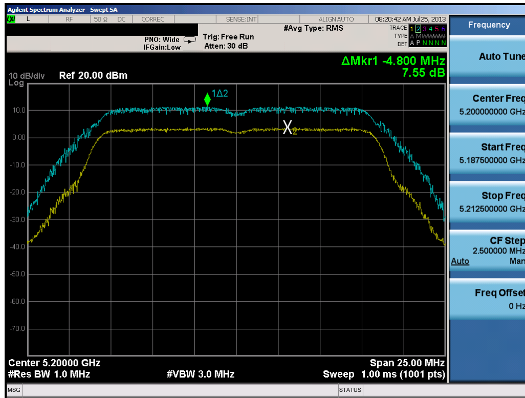
Plot 6-58. Peak Excursion Ratio Plot (802.11a)
