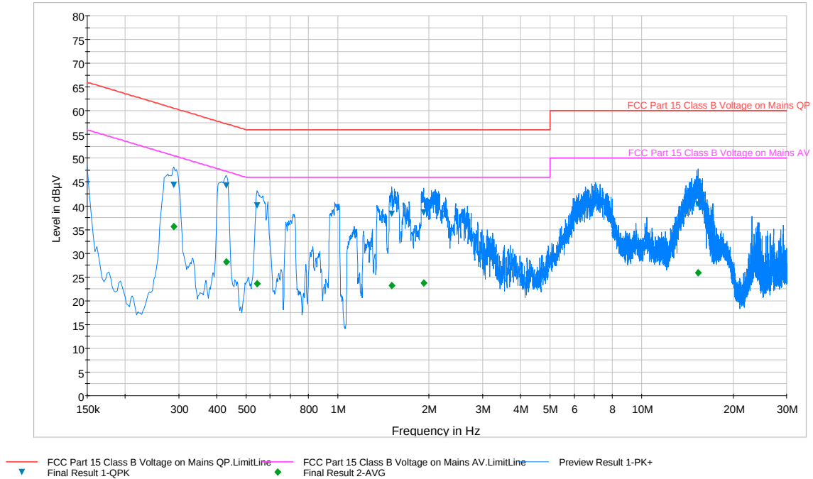
Plot 6-82. Line Conducted Plot with 802.11a UNII Band 1 (L1)
