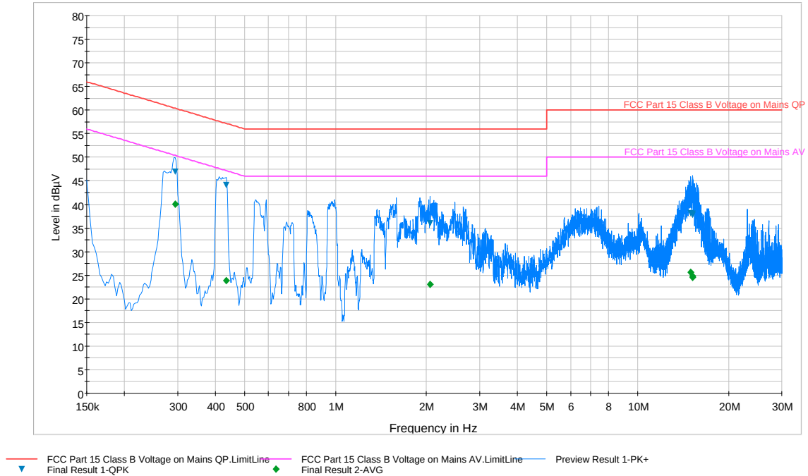
Plot 6-87. Line Conducted Plot with 802.11a UNII Band 3 (N)
