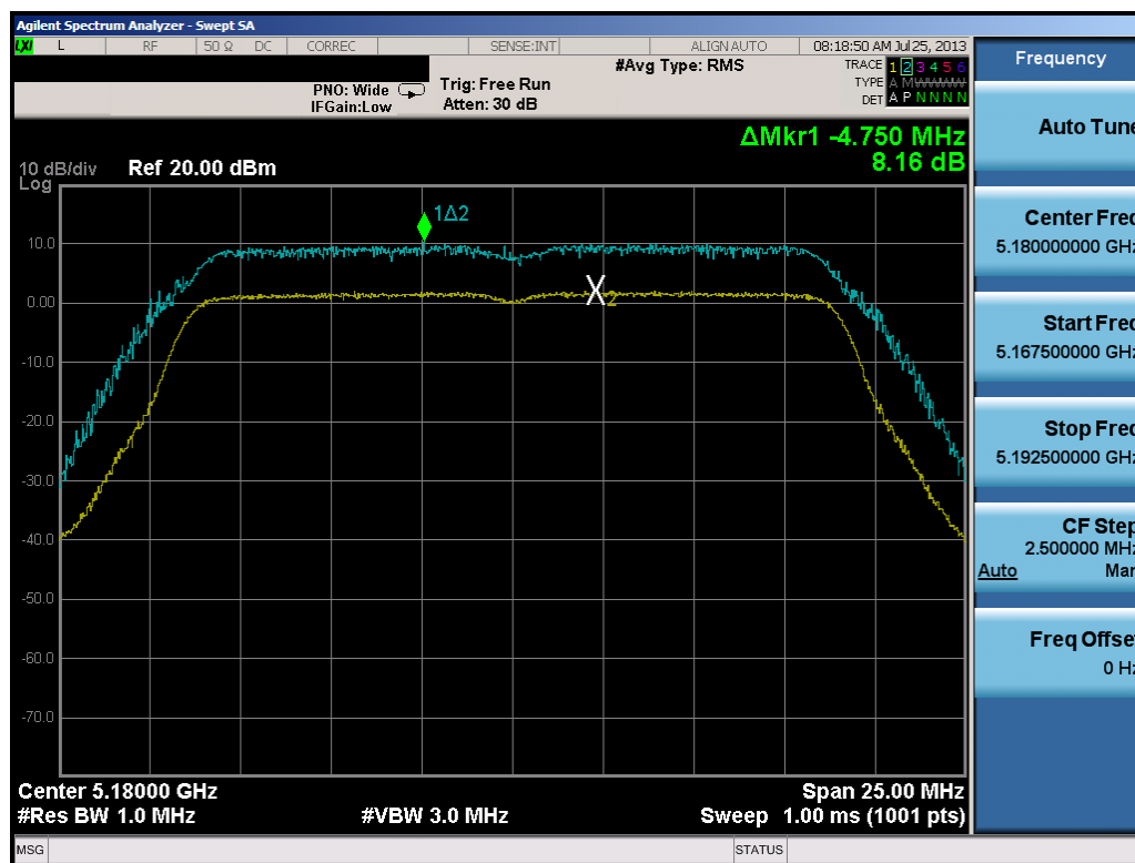
Plot 6-59. Peak Excursion Ratio Plot (20MHz BW 802.11n)
