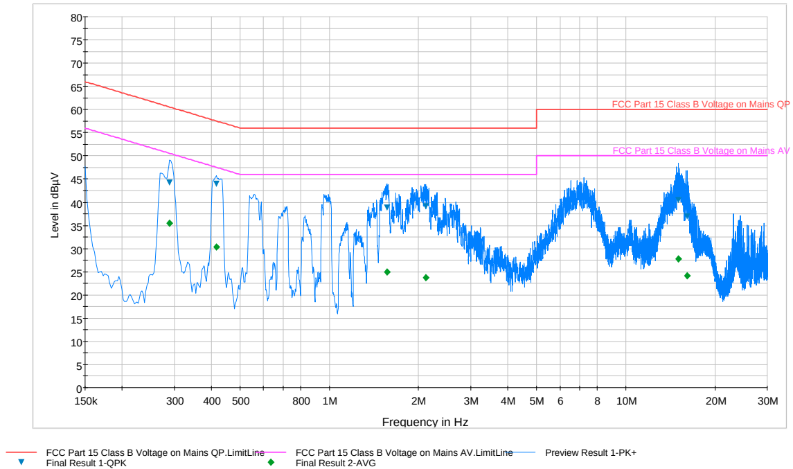
Plot 6-84. Line Conducted Plot with 802.11a UNII Band 2 (L1)
