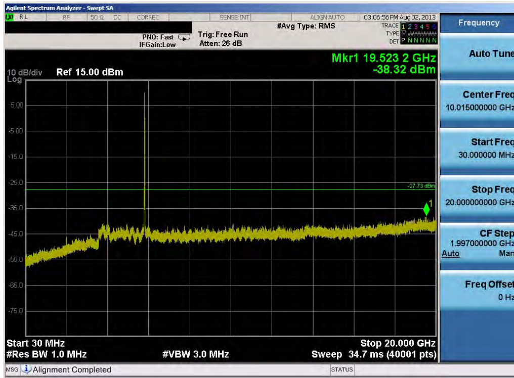
Plot 6-63. Conducted Spurious Plot (802.11a – Ch. 165)
