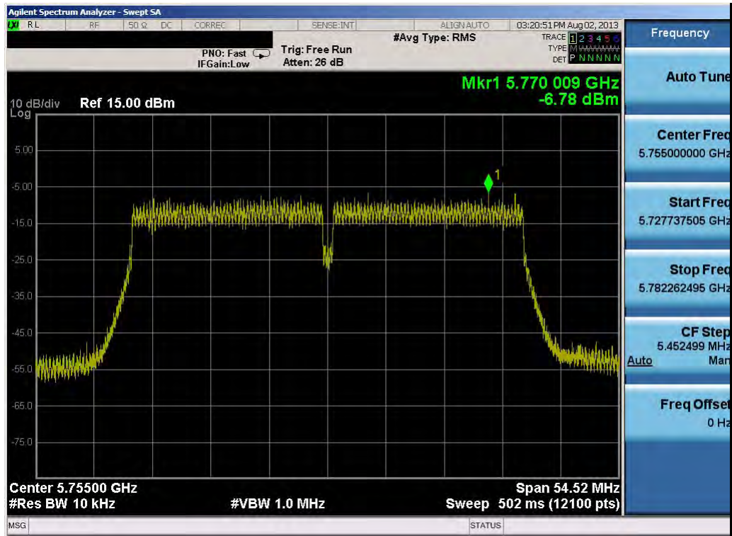
Plot 6-35. Power Spectral Density Plot (40MHz BW 802.11n (5.8GHz) – Ch. 151)
