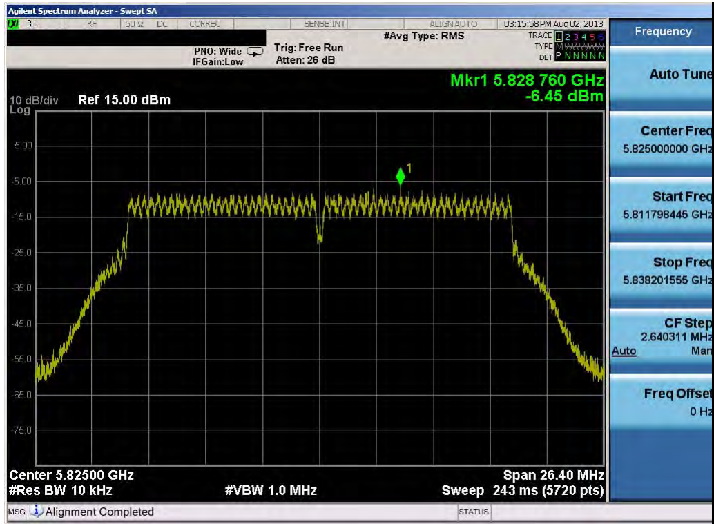
Plot 6-34. Power Spectral Density Plot (20MHz BW 802.11n (5.8GHz) – Ch. 165)
