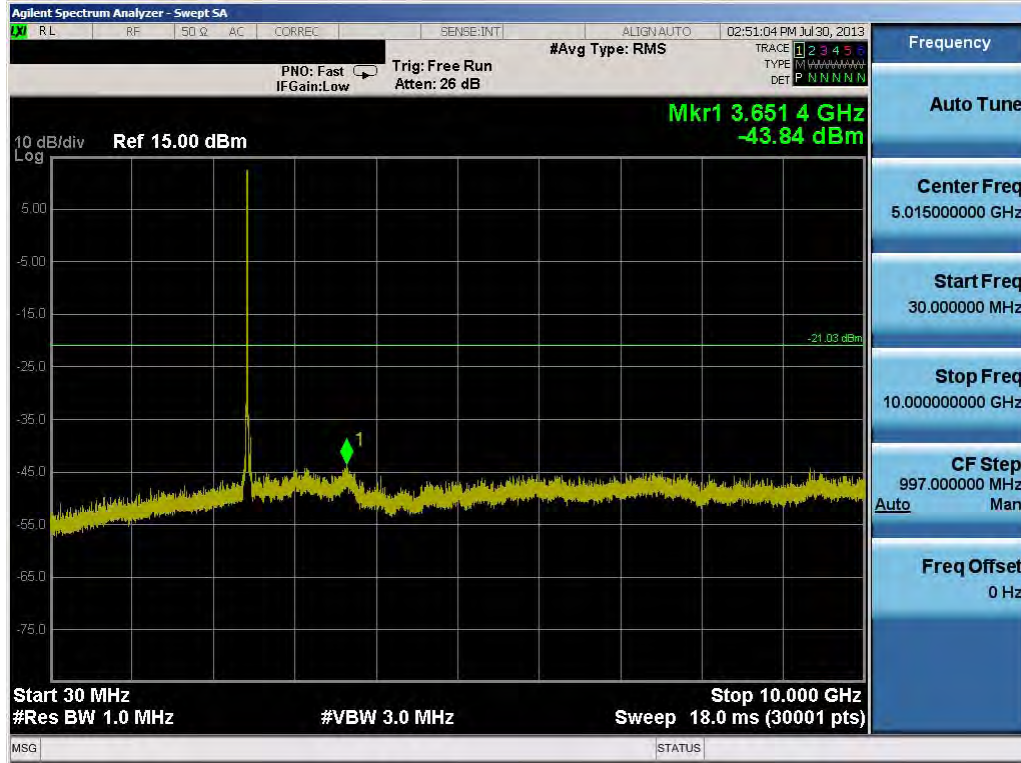
Plot 6-55. Conducted Spurious Plot (802.11b – Ch. 6)
