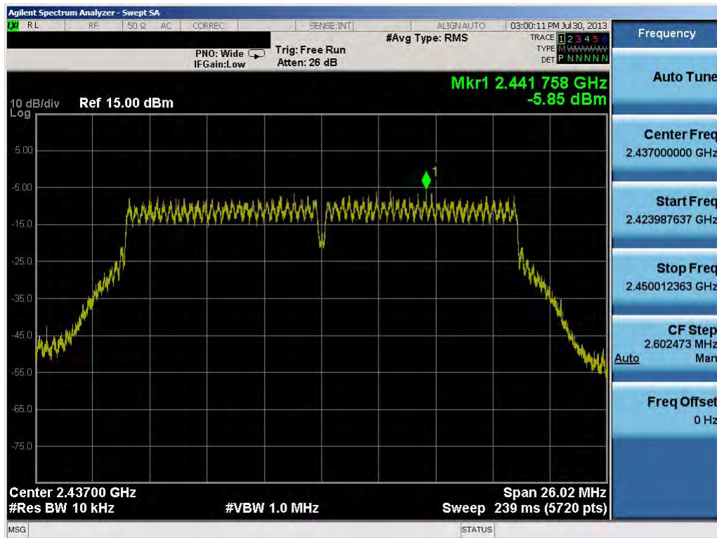
Plot 6-27. Power Spectral Density Plot (802.11n (2.4GHz) – Ch. 6)
