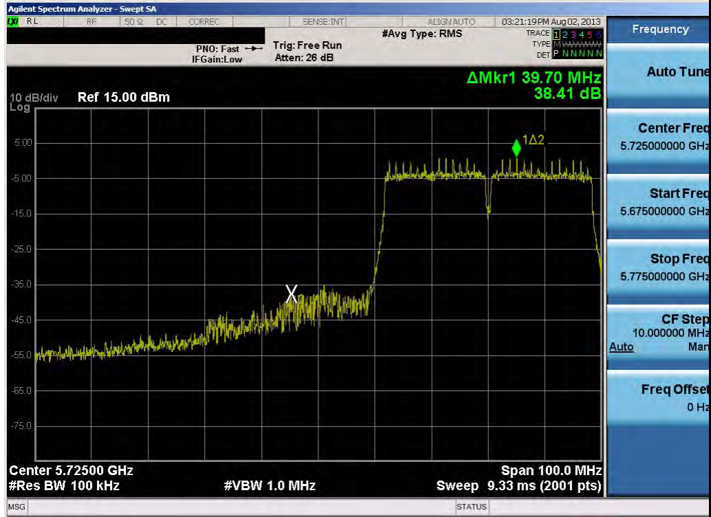
Plot 6-49. Band Edge Plot (40MHz BW 802.11n (5.8GHz) – Ch. 151)
