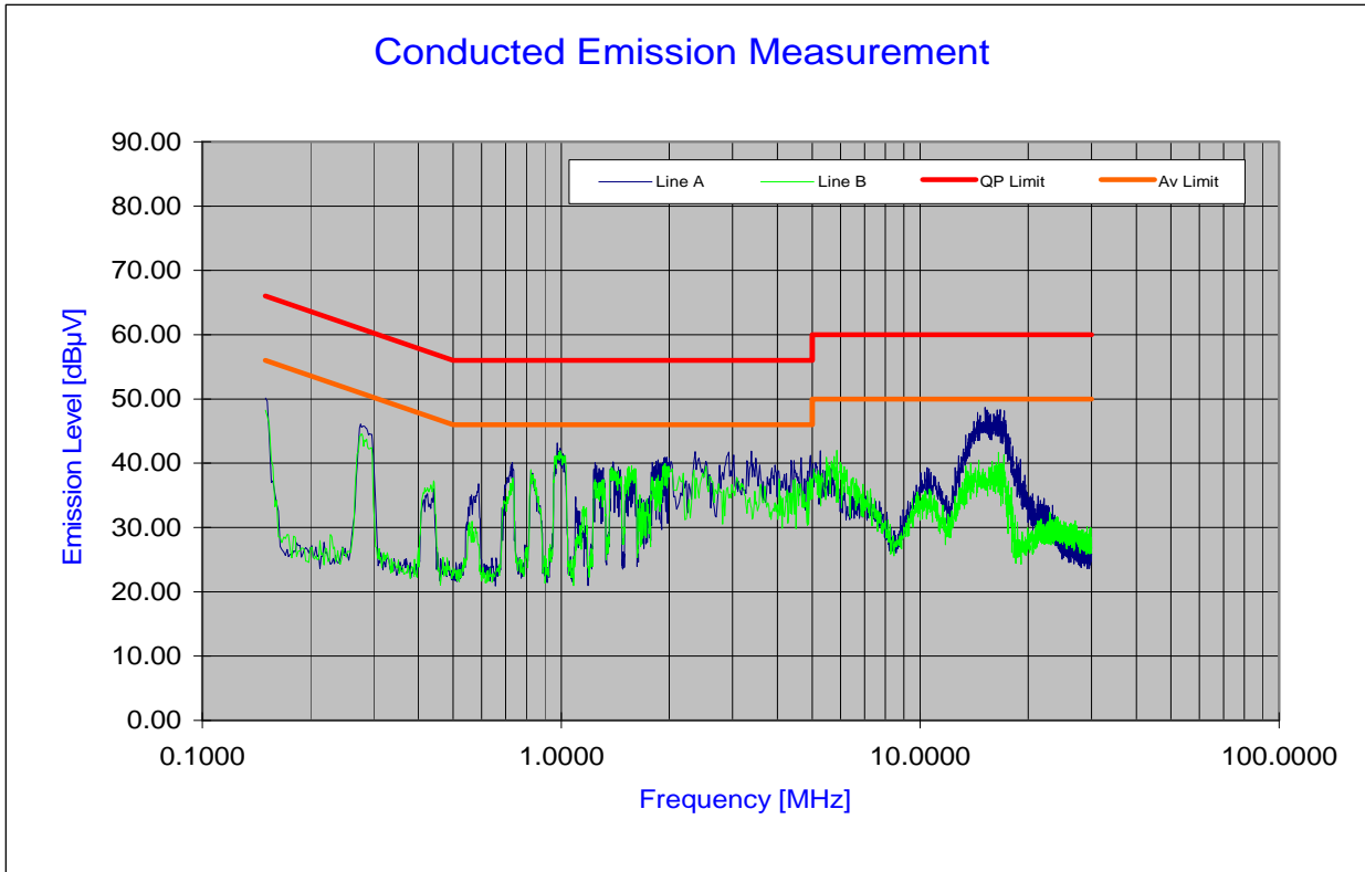
Plot 6-68. Line Conducted Plot with 802.11a
