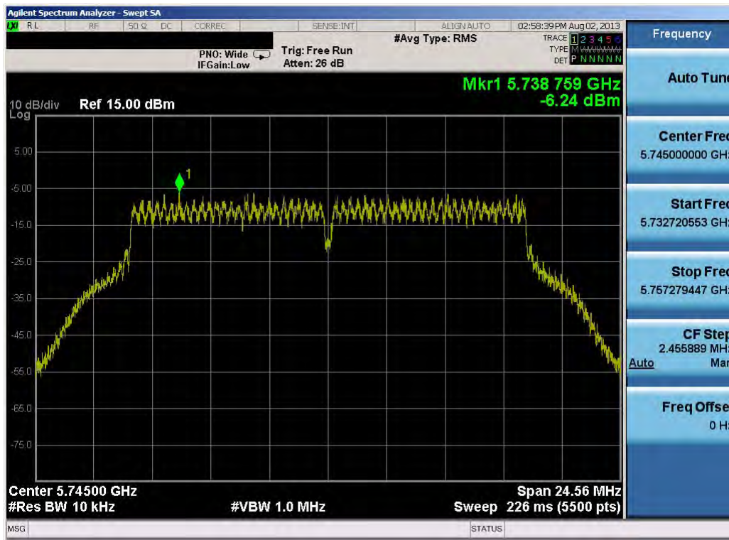
Plot 6-29. Power Spectral Density Plot (802.11a – Ch. 149)
