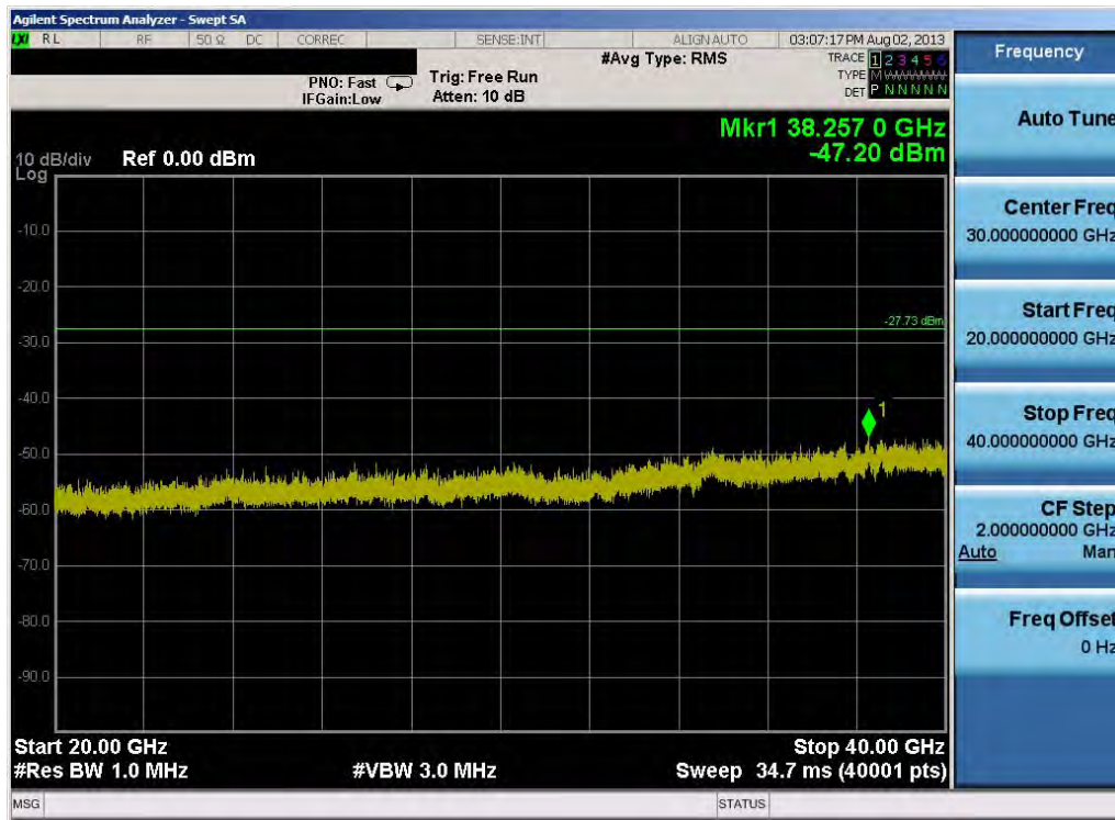
Plot 6-64. Conducted Spurious Plot (802.11a – Ch. 165)
