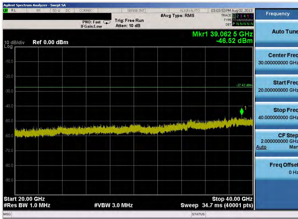
Plot 6-62. Conducted Spurious Plot (802.11a – Ch. 157)
