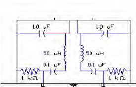
Figure 3-4. LISN Schematic Diagram
