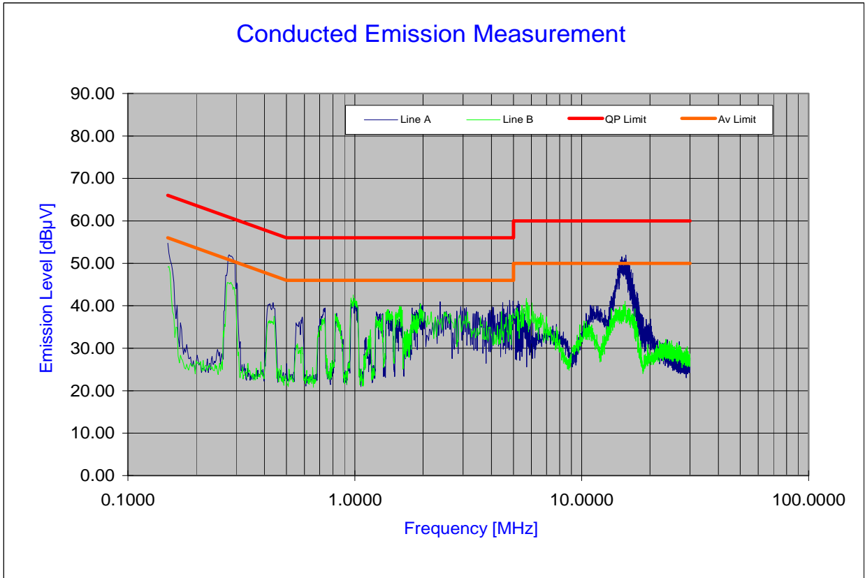
Plot 6-67. Line Conducted Plot with 802.11b
