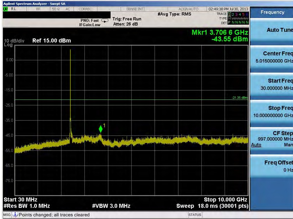
Plot 6-53. Conducted Spurious Plot (802.11b – Ch. 1)
