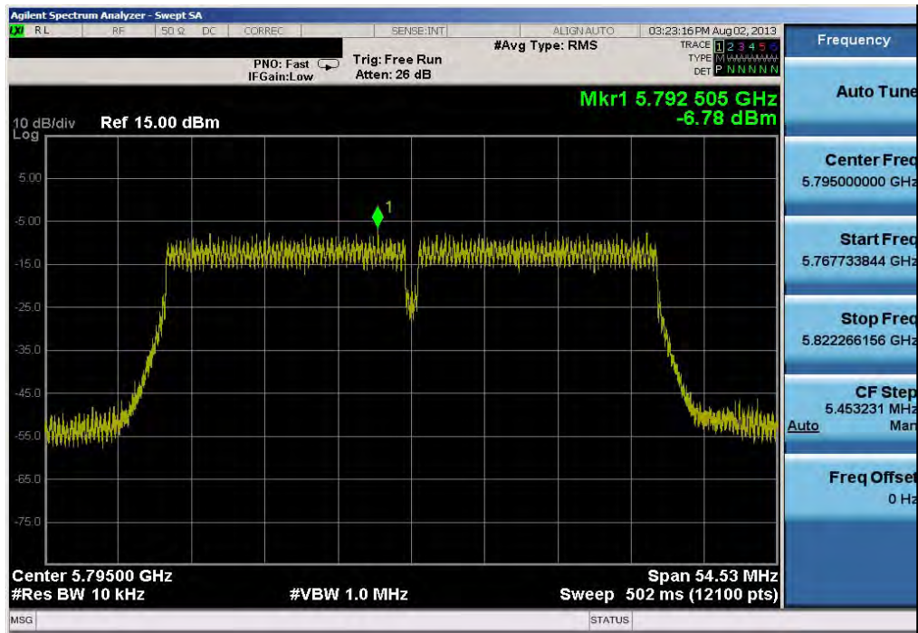
Plot 6-36. Power Spectral Density Plot (40MHz BW 802.11n (5.8GHz) – Ch. 159)
