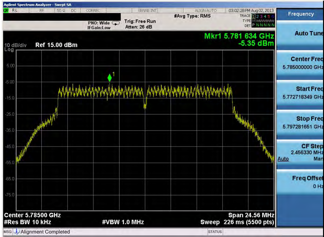
Plot 6-30. Power Spectral Density Plot (802.11a – Ch. 157)
