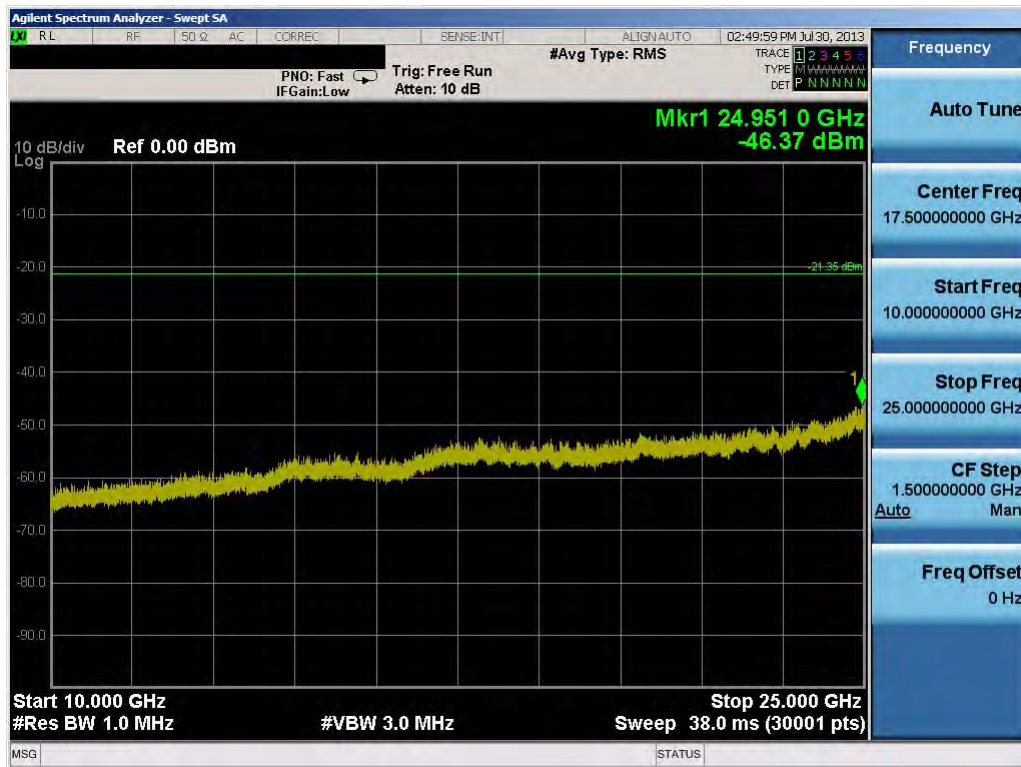
Plot 6-54. Conducted Spurious Plot (802.11b – Ch. 1)
