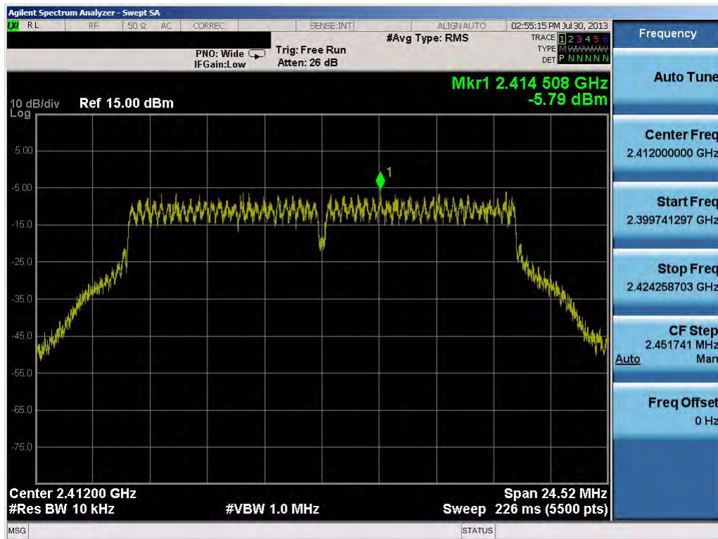
Plot 6-23. Power Spectral Density Plot (802.11g – Ch. 1)
