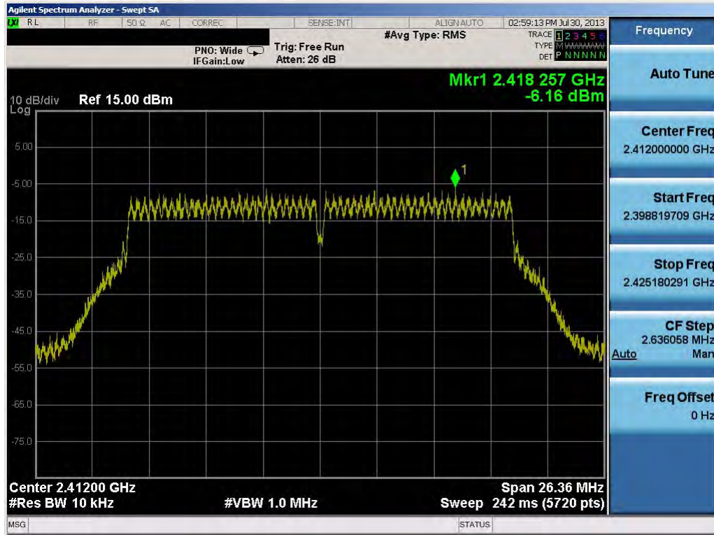
Plot 6-26. Power Spectral Density Plot (802.11n (2.4GHz) – Ch. 1)
