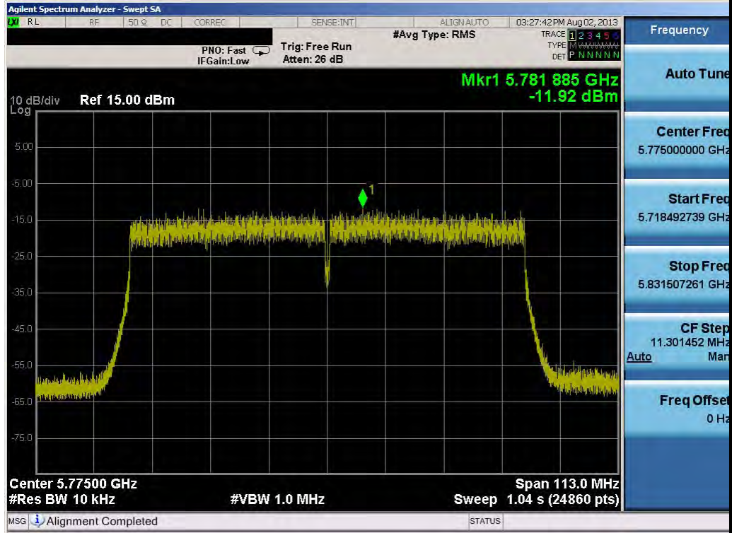
Plot 6-38. Power Spectral Density Plot (80MHz BW 802.11ac (5.8GHz) – Ch. 155)
