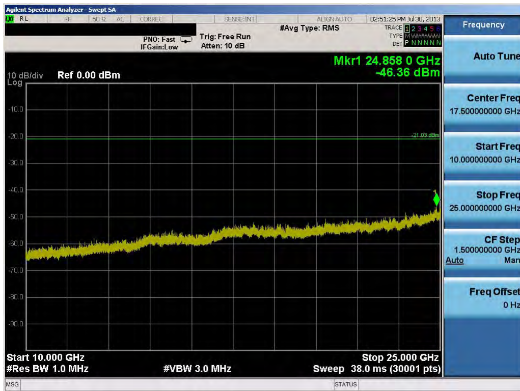
Plot 6-56. Conducted Spurious Plot (802.11b – Ch. 6)
