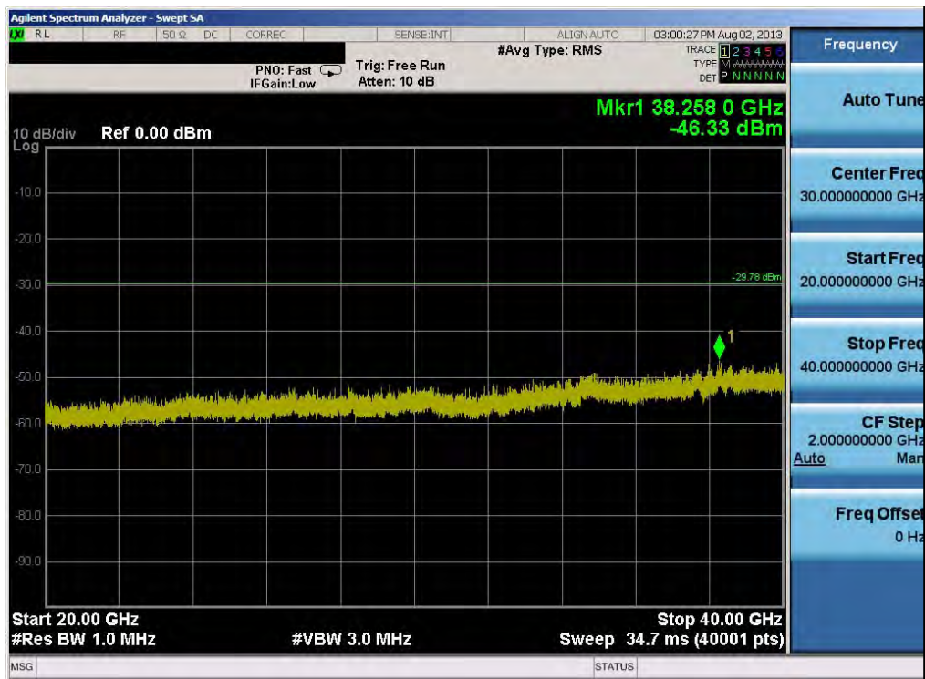
Plot 6-60. Conducted Spurious Plot (802.11a – Ch. 149)
