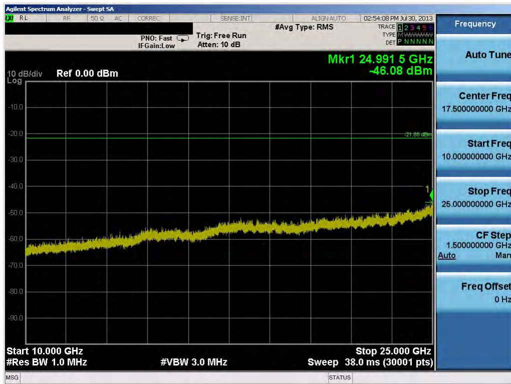
Plot 6-58. Conducted Spurious Plot (802.11b – Ch. 11)
