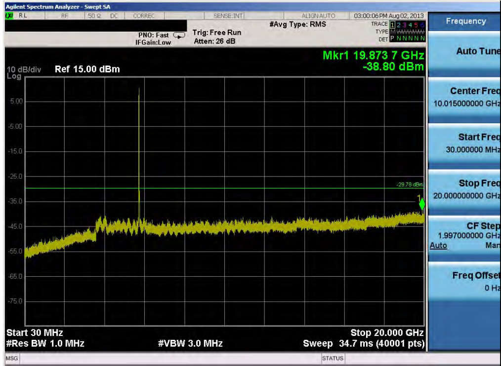
Plot 6-59. Conducted Spurious Plot (802.11a – Ch. 149)
