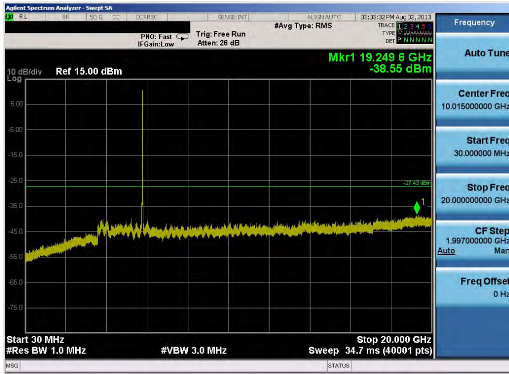
Plot 6-61. Conducted Spurious Plot (802.11a – Ch. 157)
