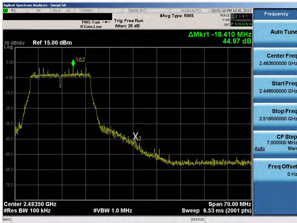
Plot 6-44. Band Edge Plot (802.11n (2.4GHz) – Ch. 11)
