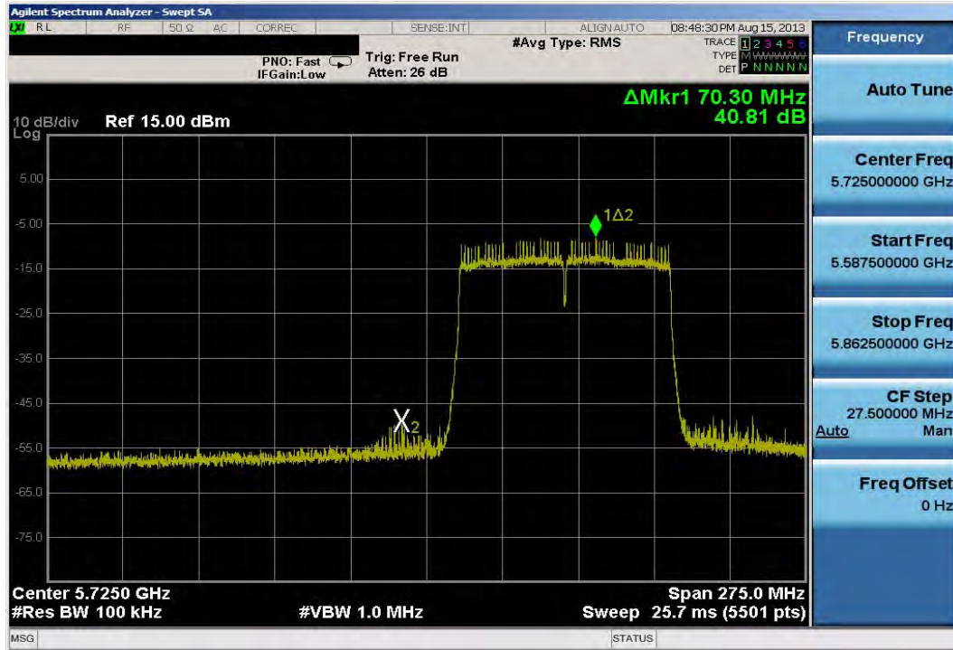
Plot 6-51. Band Edge Plot (80MHz BW 802.11ac (5.8GHz) – Ch. 155)
