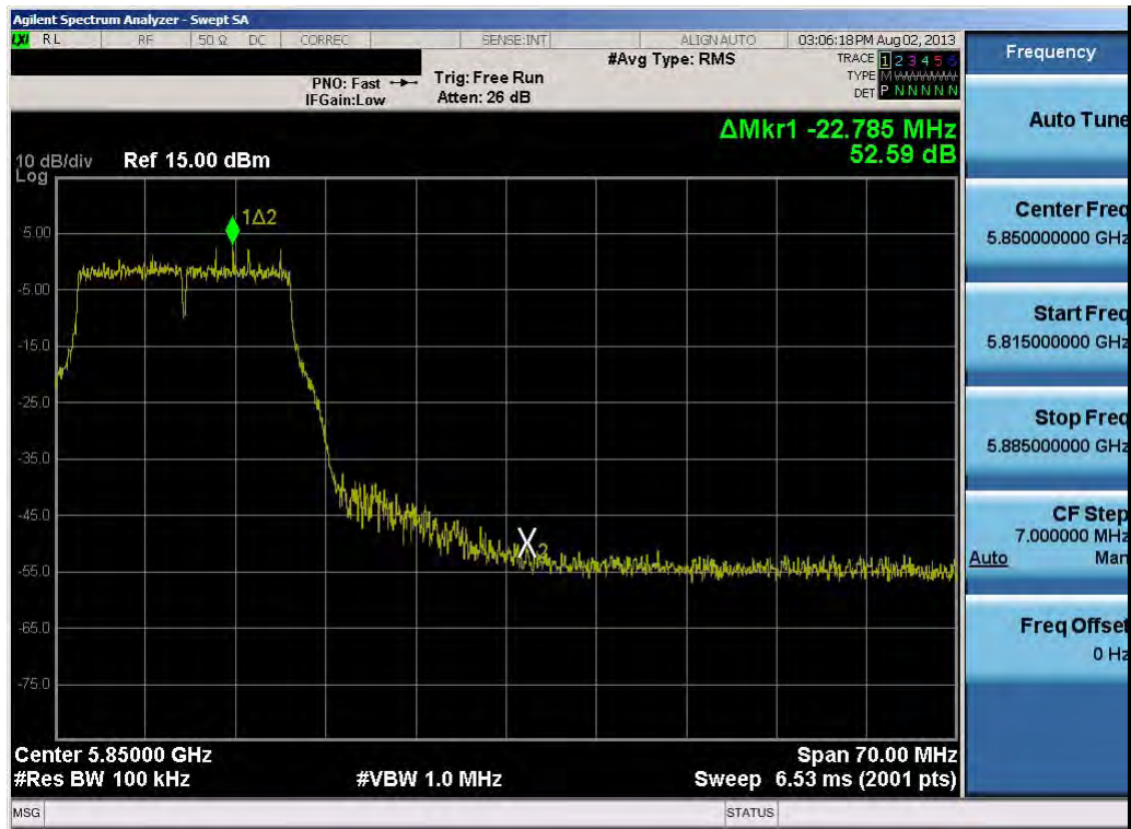
Plot 6-46. Band Edge Plot (802.11a – Ch. 165)
