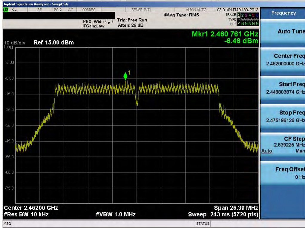
Plot 6-28. Power Spectral Density Plot (802.11n (2.4GHz) – Ch. 11)
