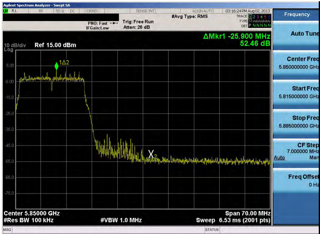
Plot 6-48. Band Edge Plot (20MHz BW 802.11n (5.8GHz) – Ch. 165)
