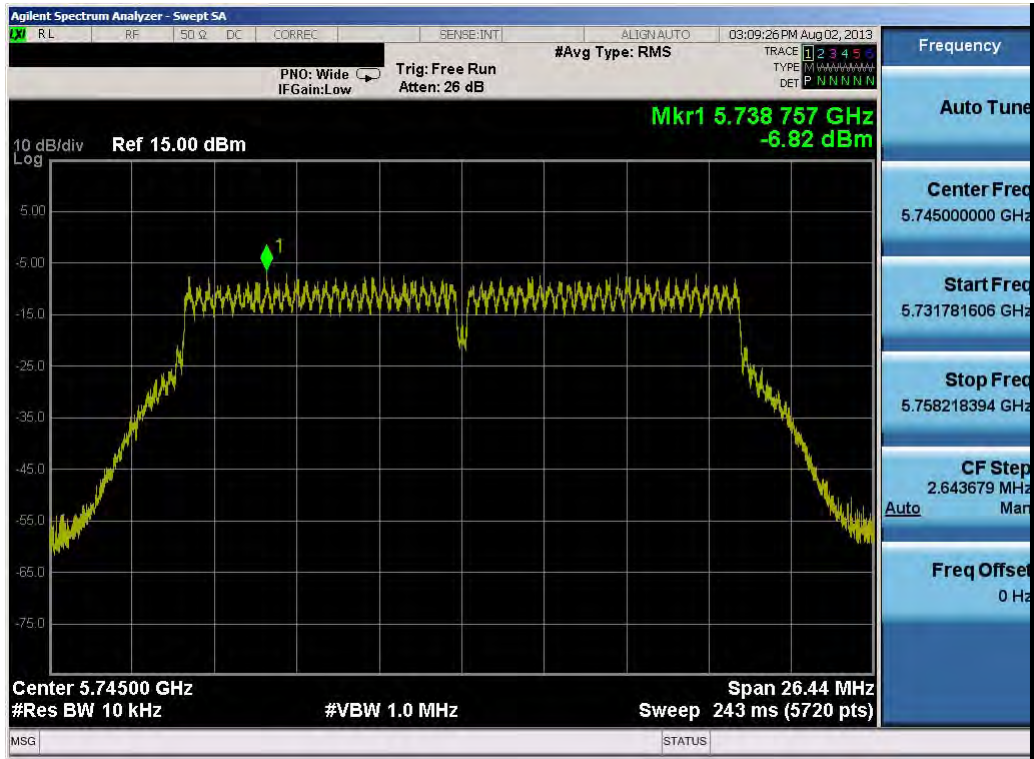
Plot 6-32. Power Spectral Density Plot (20MHz BW 802.11n (5.8GHz) – Ch. 149)
