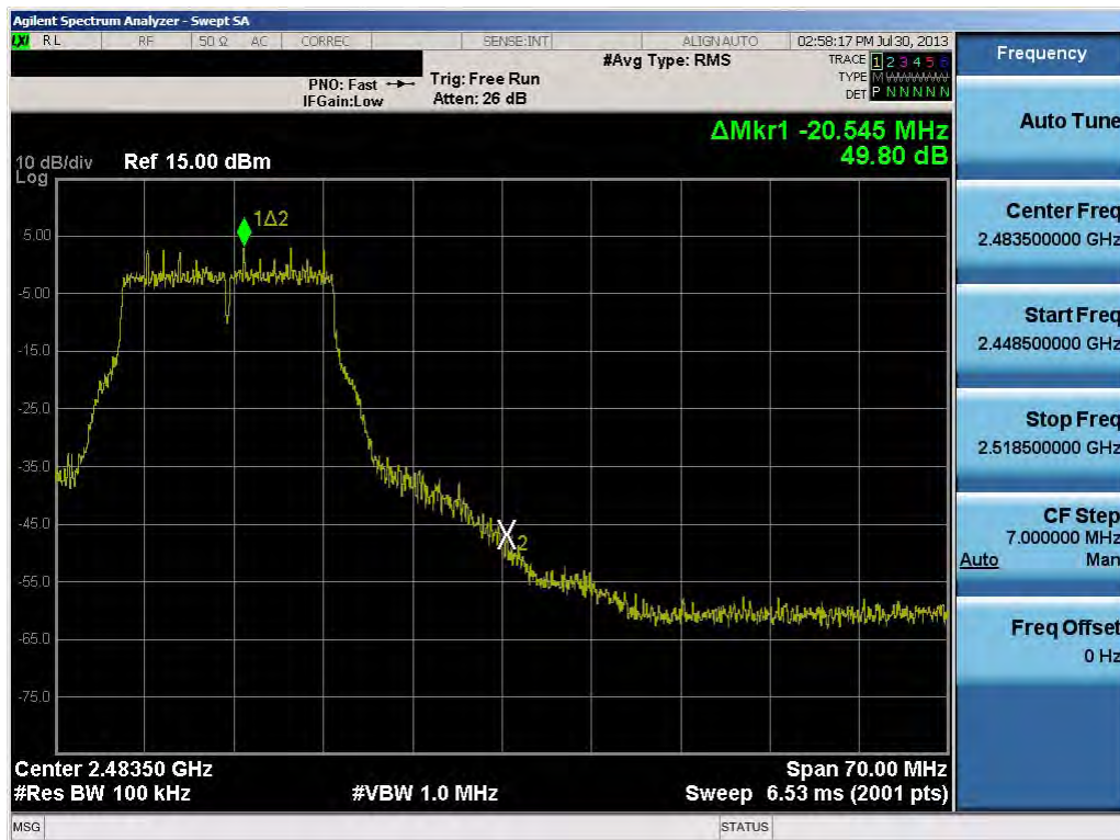
Plot 6-42. Band Edge Plot (802.11g – Ch. 11)
