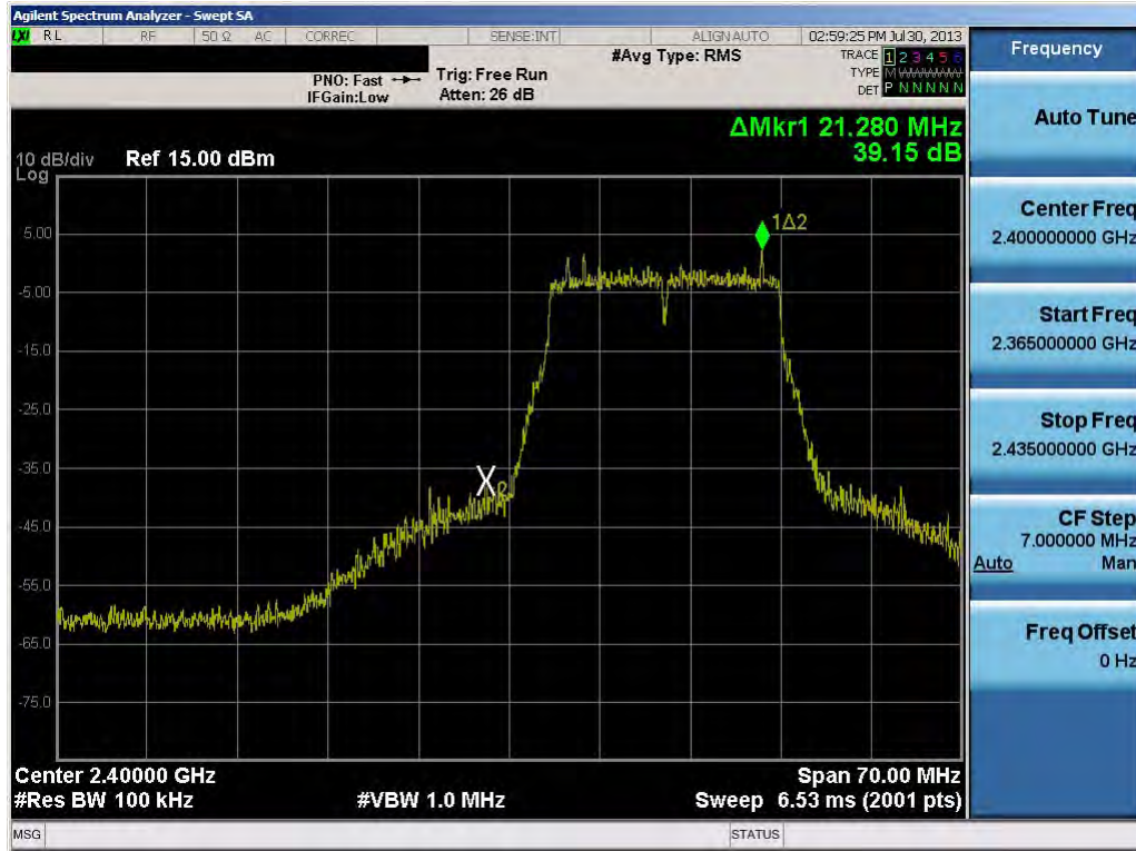
Plot 6-43. Band Edge Plot (802.11n (2.4GHz) – Ch. 1)
