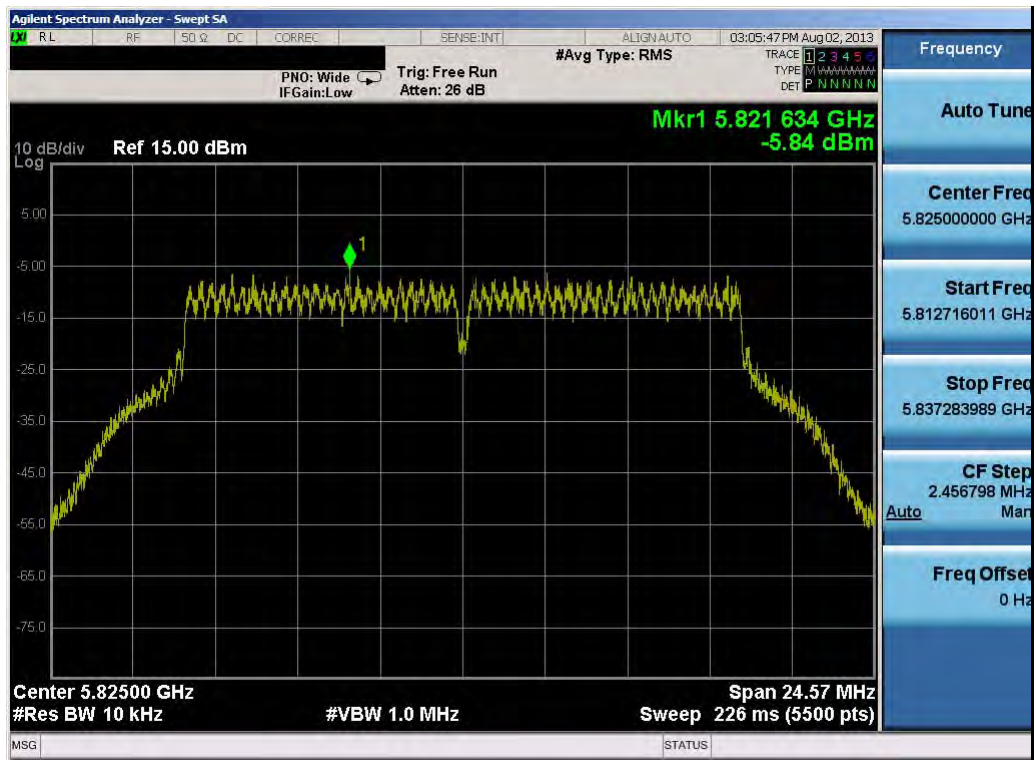
Plot 6-31. Power Spectral Density Plot (802.11a – Ch. 165)
