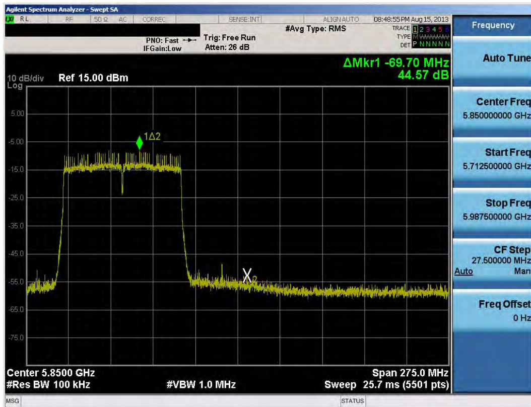
Plot 6-52. Band Edge Plot (80MHz BW 802.11ac (5.8GHz) – Ch. 155)
