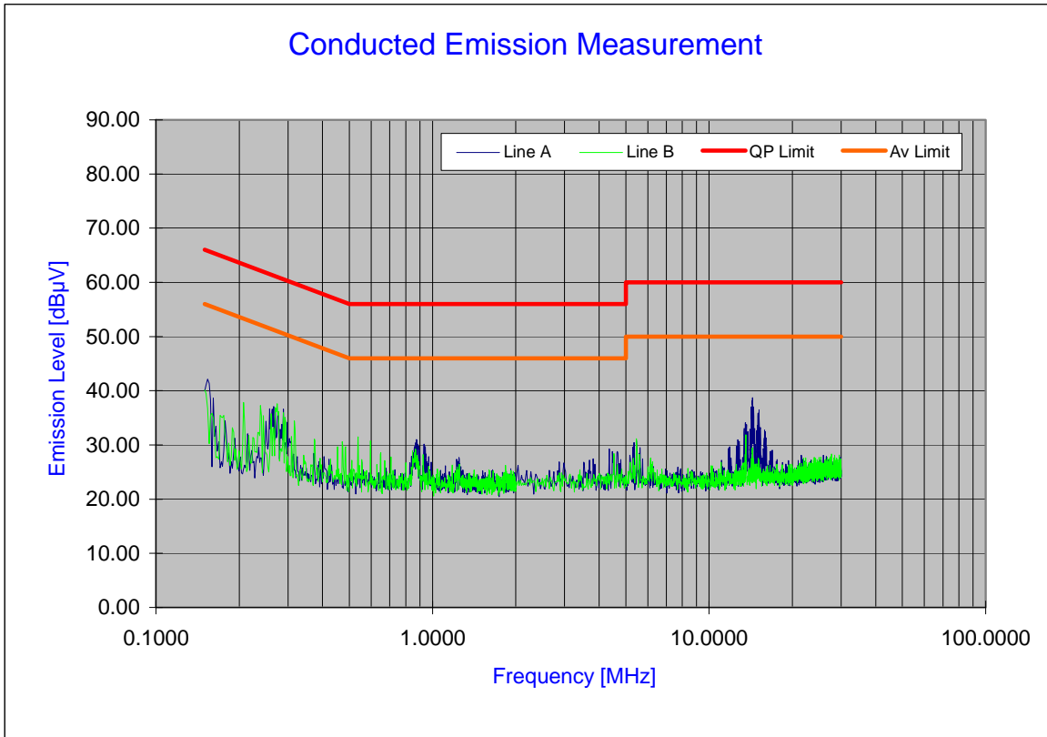
Plot 6-64. Line Conducted Plot with 802.11a UNII Band 2
