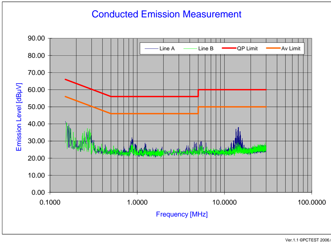
Plot 6-63. Line Conducted Plot with 802.11a UNII Band 1
