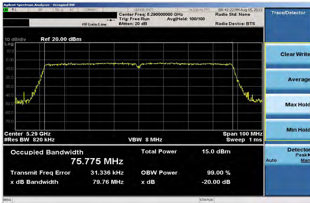
Plot 6-30. 20dB Bandwidth Plot (80MHz BW 802.11ac (UNII Band 2) – Ch. 58)
