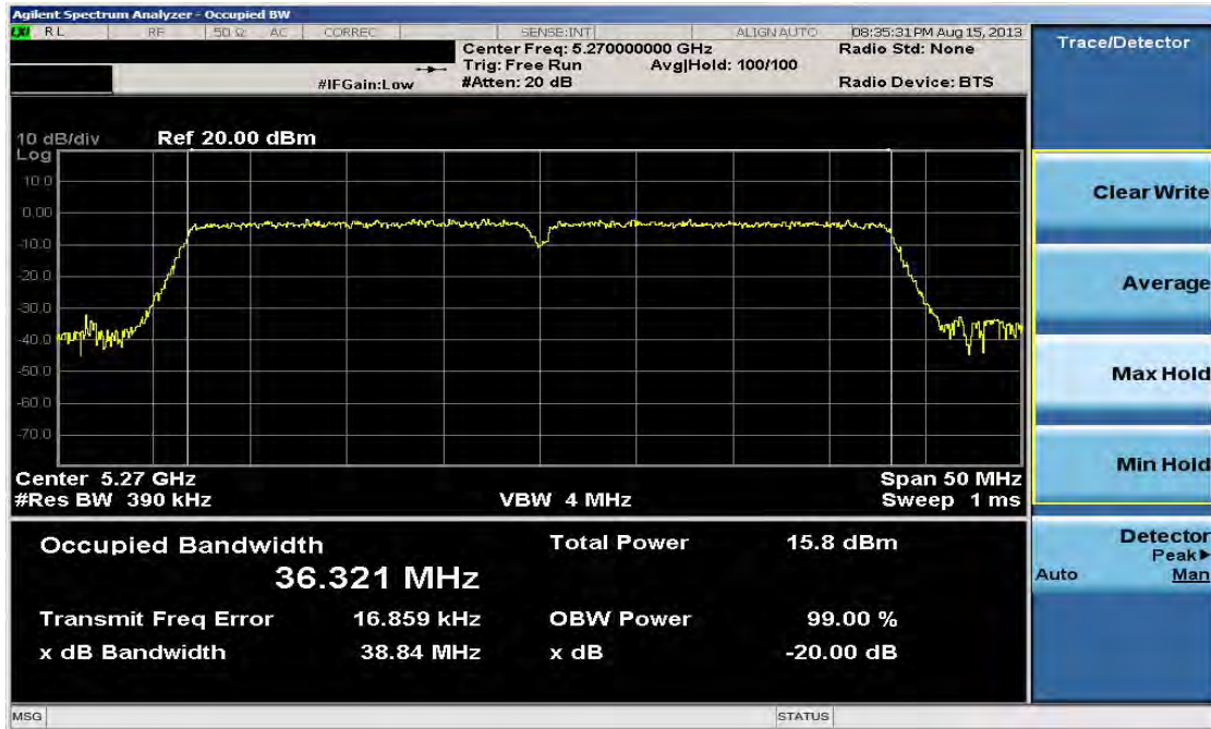
Plot 6-29. 20dB Bandwidth Plot (40MHz BW 802.11n (UNII Band 2) – Ch. 54)
