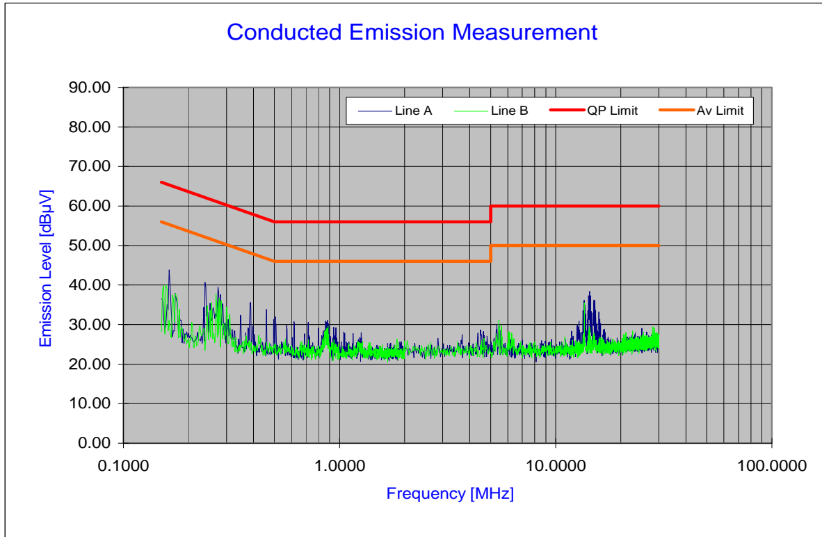
Plot 6-65. Line Conducted Plot with 802.11a UNII Band 3
