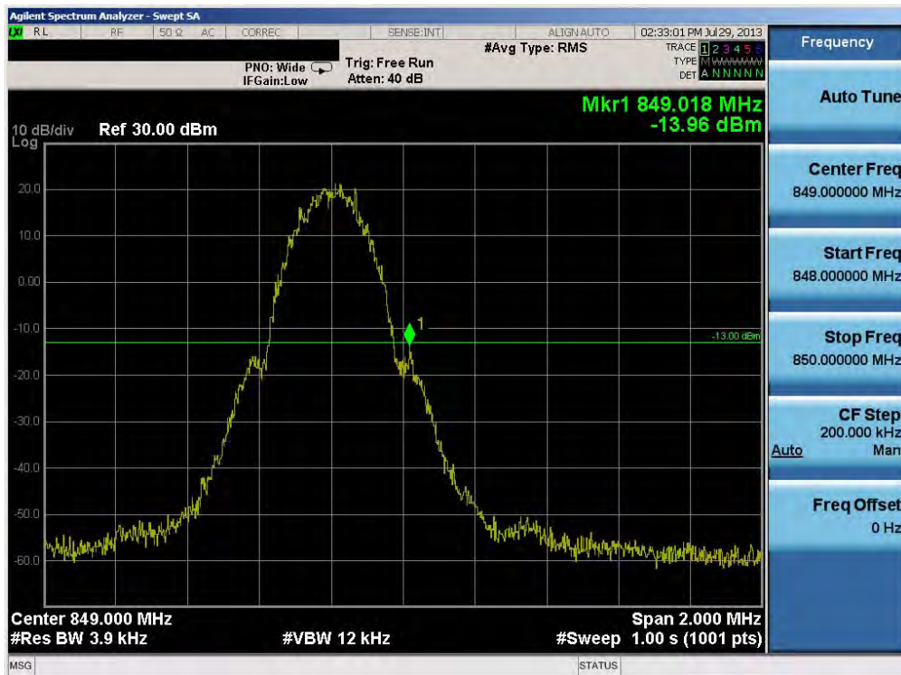
Plot 6-52. Band Edge Plot (Cellular GSM Mode – Ch. 251)
