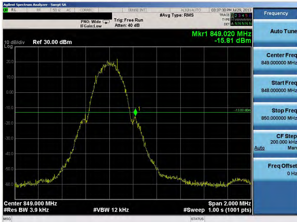
Plot 6-62. Band Edge Plot (Cellular GSM Mode – Ch. 251)
