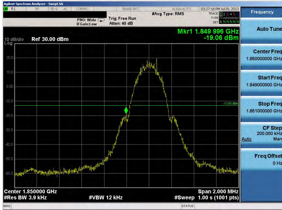
Plot 6-63. Band Edge Plot (PCS GSM Mode – Ch. 512)
