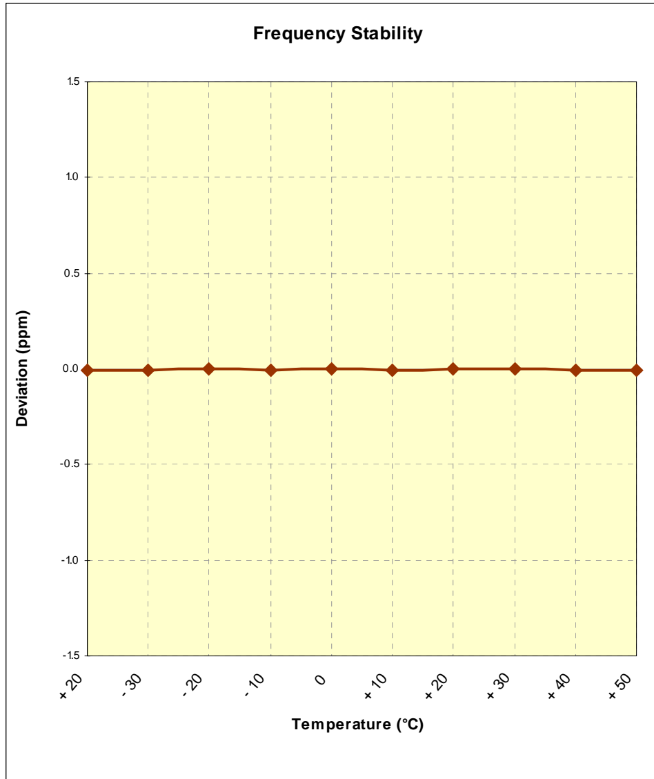
Figure 6-16. Frequency Stability Graph (PCS WCDMA Mode – Ch. 9400)
