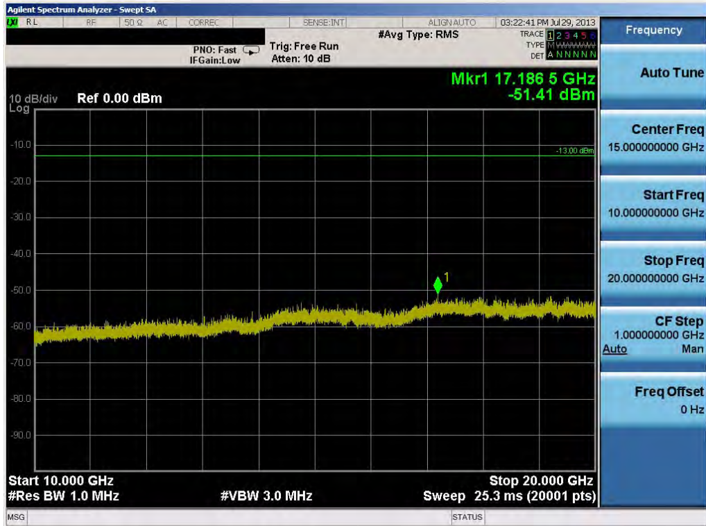
Plot 6-48. Conducted Spurious Plot (PCS GSM Mode – Ch. 661)
