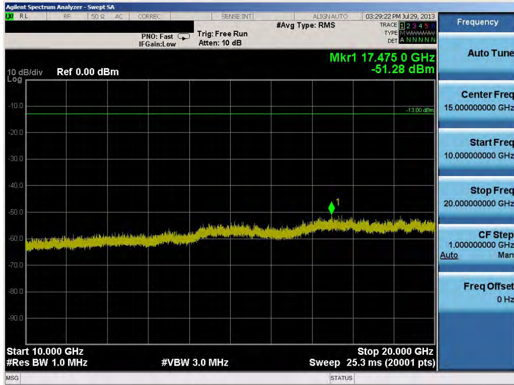
Plot 6-50. Conducted Spurious Plot (PCS GSM Mode – Ch. 810)
