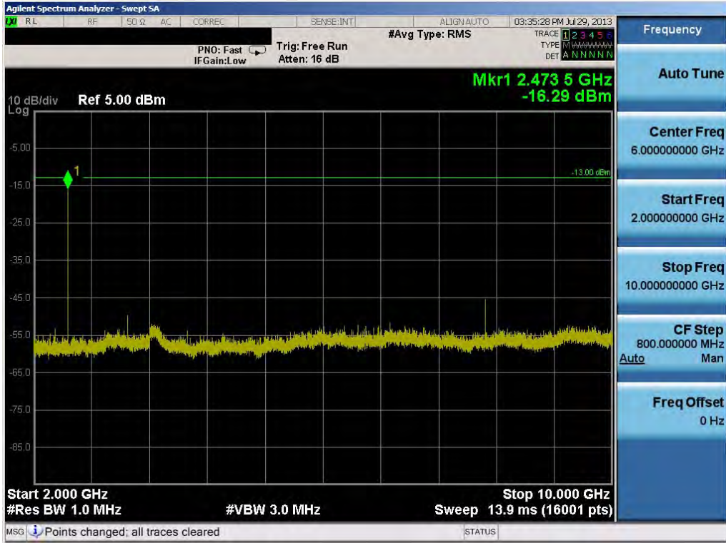
Plot 6-38. Conducted Spurious Plot (Cellular GSM Mode – Ch. 128)
