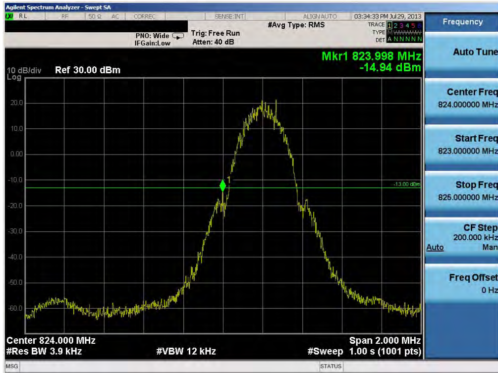
Plot 6-61. Band Edge Plot (Cellular GSM Mode – Ch. 128)
