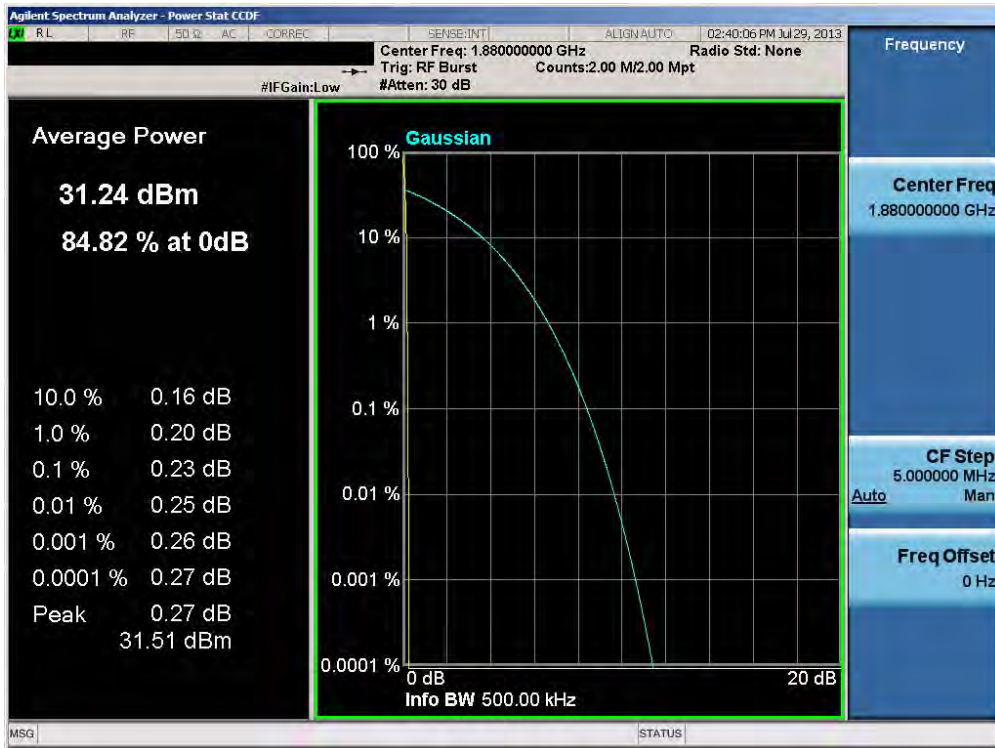
Plot 6-65. Peak-Average Ratio Plot (PCS GSM Mode – Ch. 661)
