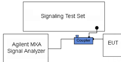
Figure 6-8. Test Instrument & Measurement Setup
