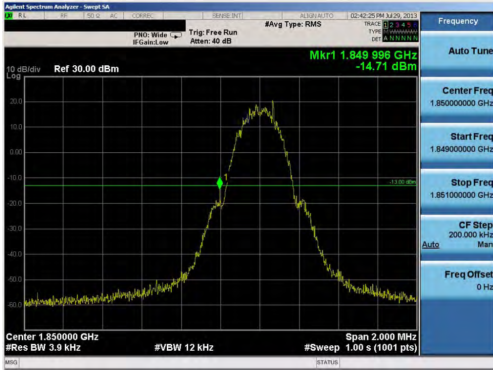
Plot 6-53. Band Edge Plot (PCS GSM Mode – Ch. 512)
