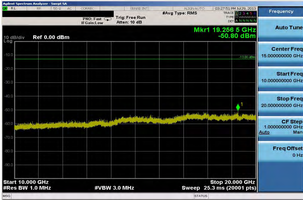
Plot 6-46. Conducted Spurious Plot (PCS GSM Mode – Ch. 512)
