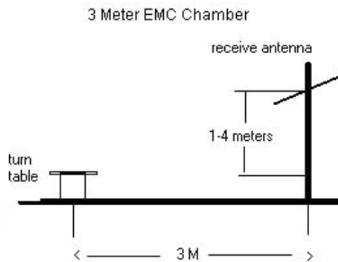
Figure 6-12. Test Instrument & Measurement Setup
