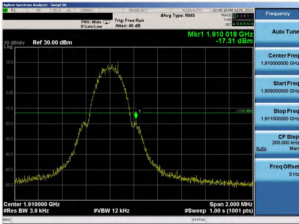
Plot 6-54. Band Edge Plot (PCS GSM Mode – Ch. 810)
