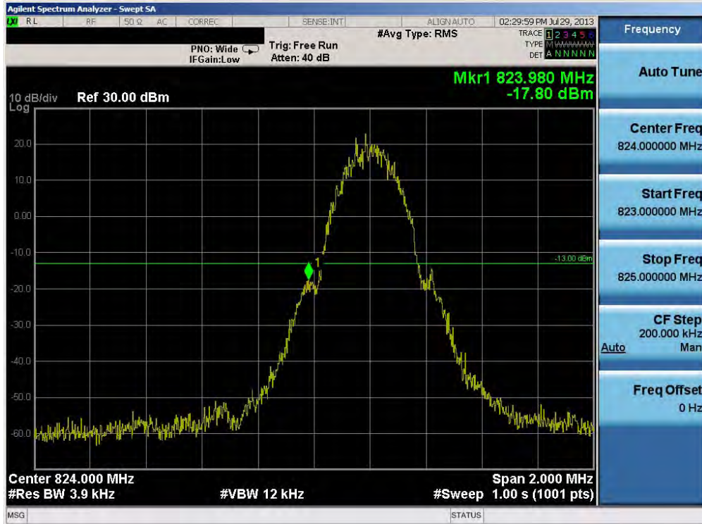
Plot 6-51. Band Edge Plot (Cellular GSM Mode – Ch. 128)
