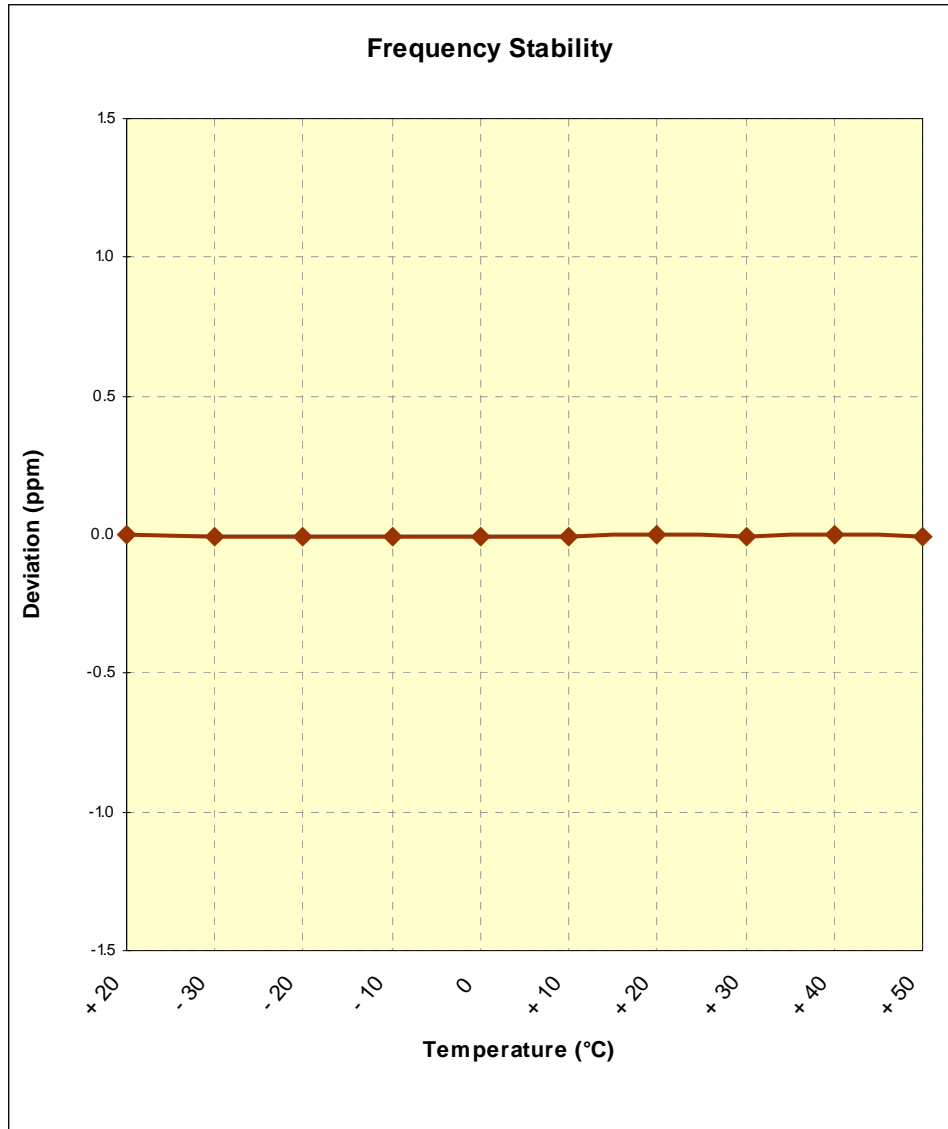
Figure 6-15. Frequency Stability Graph (PCS GSM Mode – Ch. 661)
