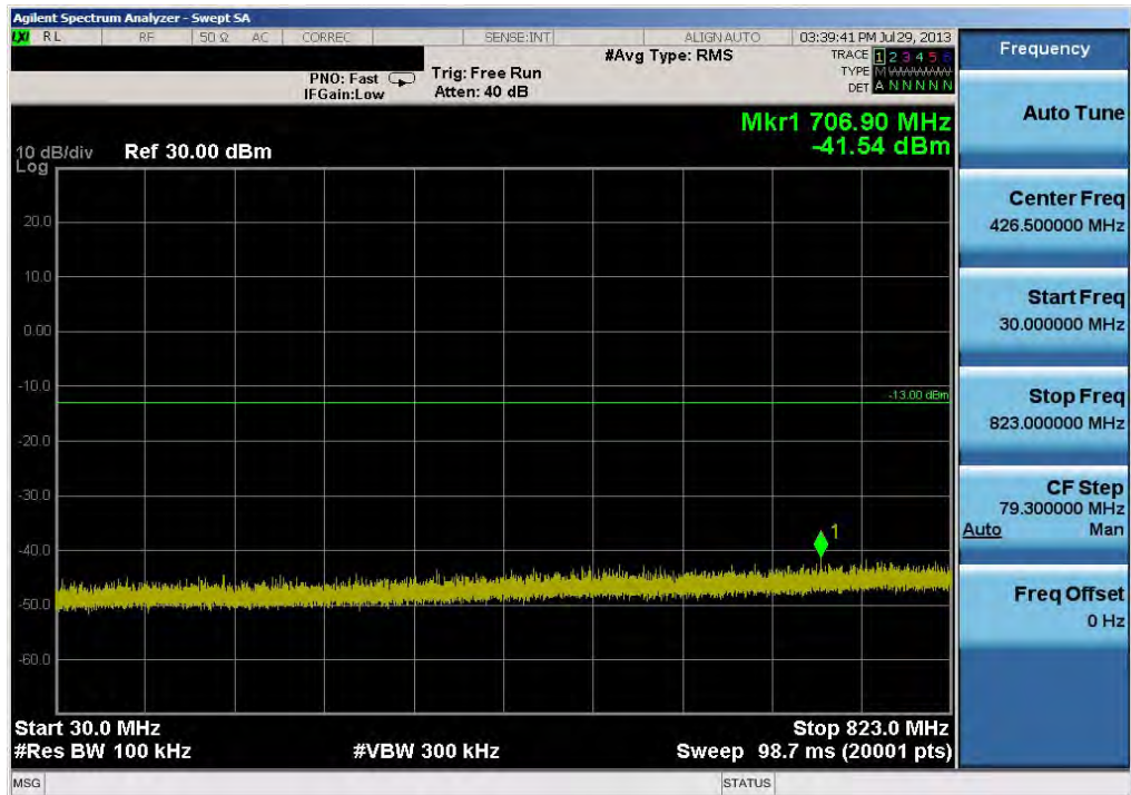
Plot 6-39. Conducted Spurious Plot (Cellular GSM Mode – Ch. 190)
