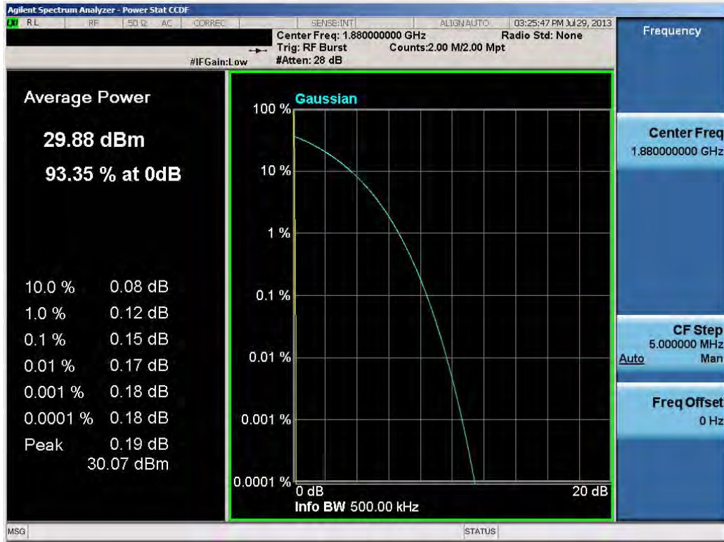
Plot 6-68. Peak-Average Ratio Plot (PCS GSM Mode – Ch. 661)
