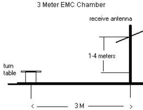
Figure 6-9. Test Instrument & Measurement Setup
