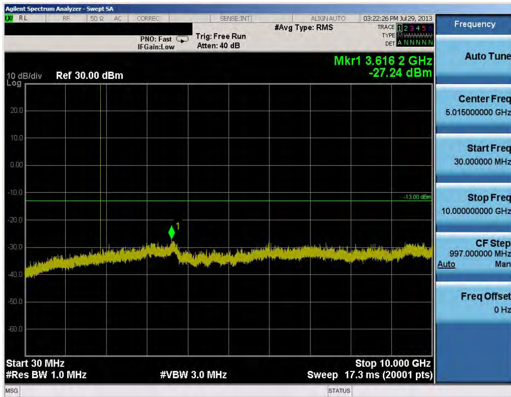
Plot 6-47. Conducted Spurious Plot (PCS GSM Mode – Ch. 661)
