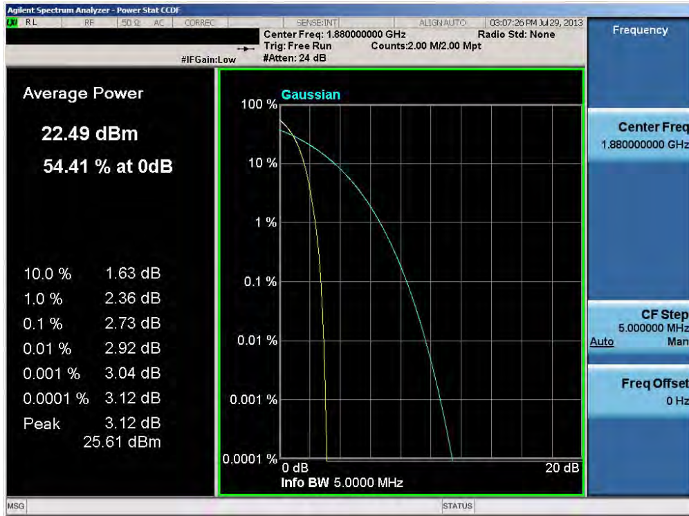
Plot 6-67. Peak-Average Ratio Plot (PCS WCDMA Mode – Ch. 9400)
