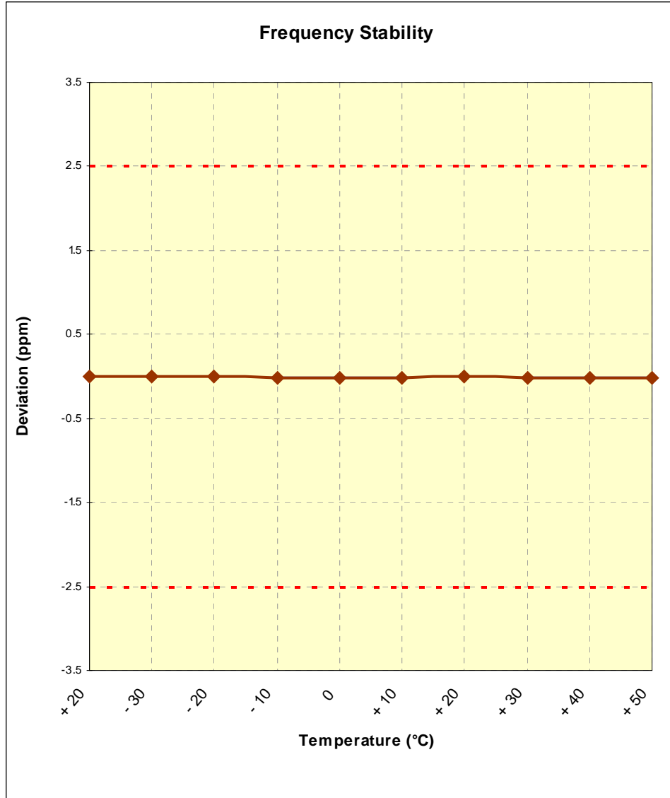
Figure 6-13. Frequency Stability Graph (Cellular GSM Mode – Ch. 190)
