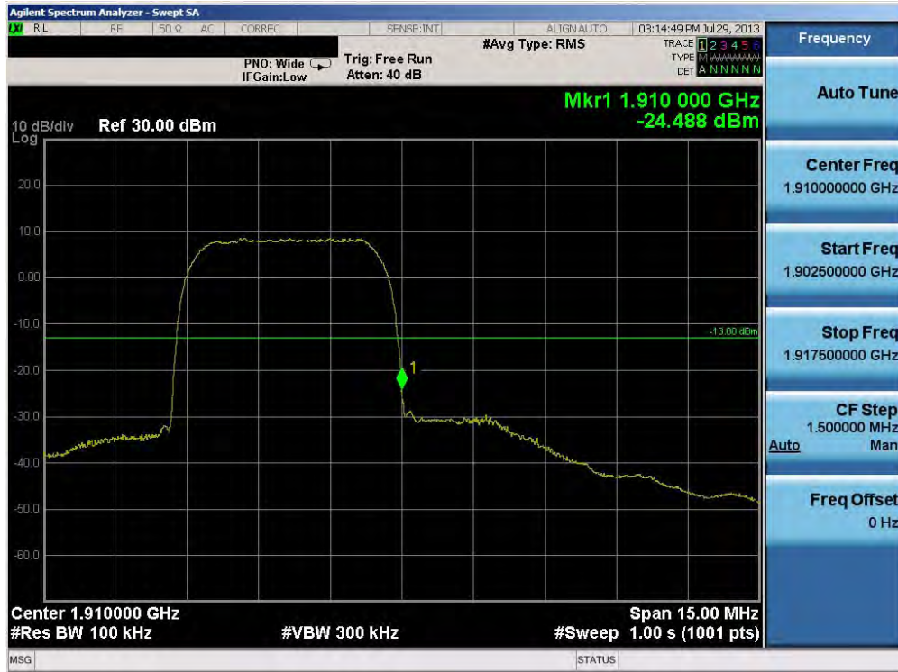
Plot 6-59. Band Edge Plot (PCS WCDMA Mode – Ch. 9538)
