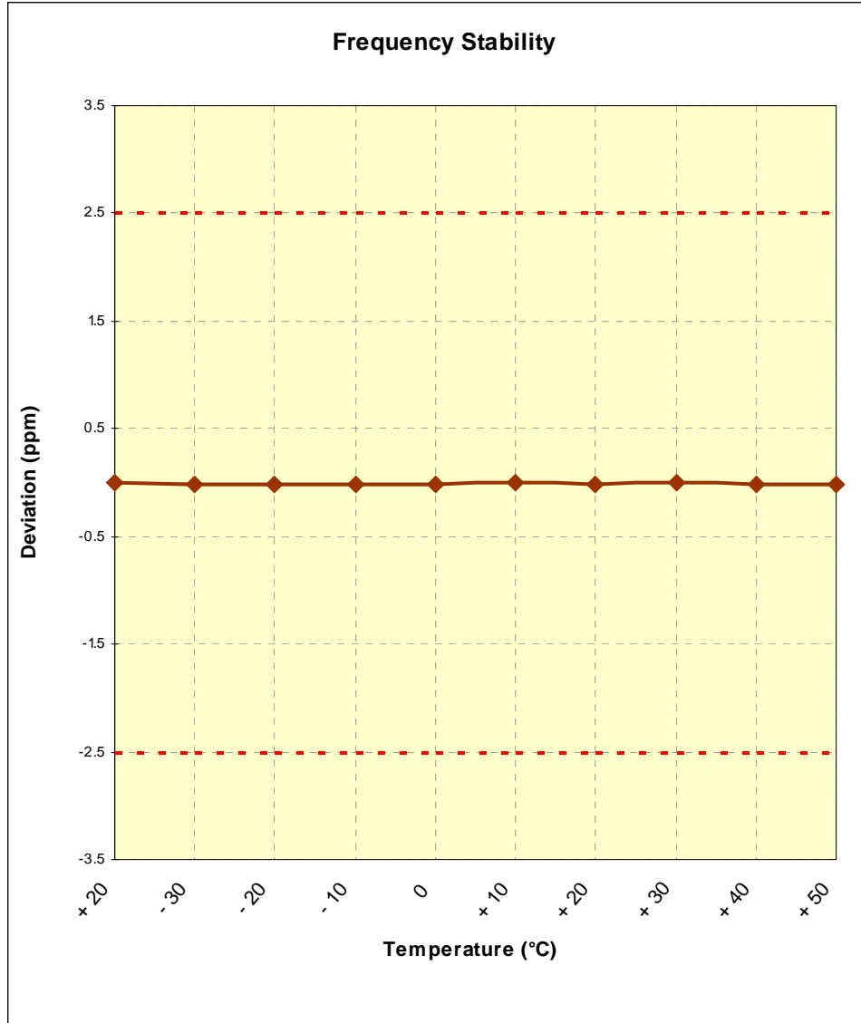
Figure 6-17. Frequency Stability Graph (Cellular GSM Mode – Ch. 190)
