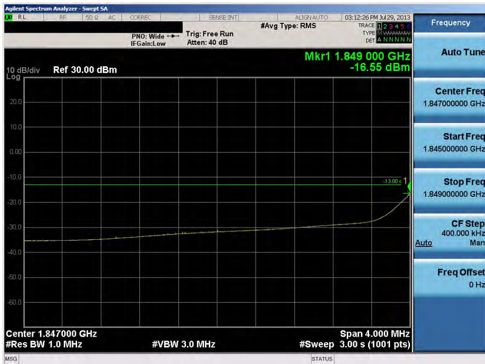
Plot 6-58. 4MHz Span Plot (PCS WCDMA Mode – Ch. 9262)
