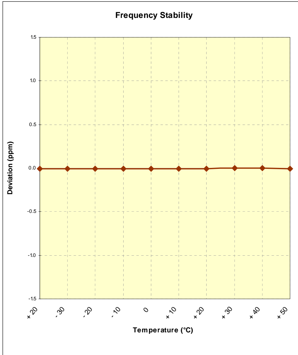
Figure 6-18. Frequency Stability Graph (PCS GSM Mode – Ch. 661)
