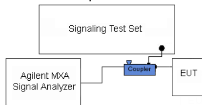
Figure 6-7. Test Instrument & Measurement Setup
