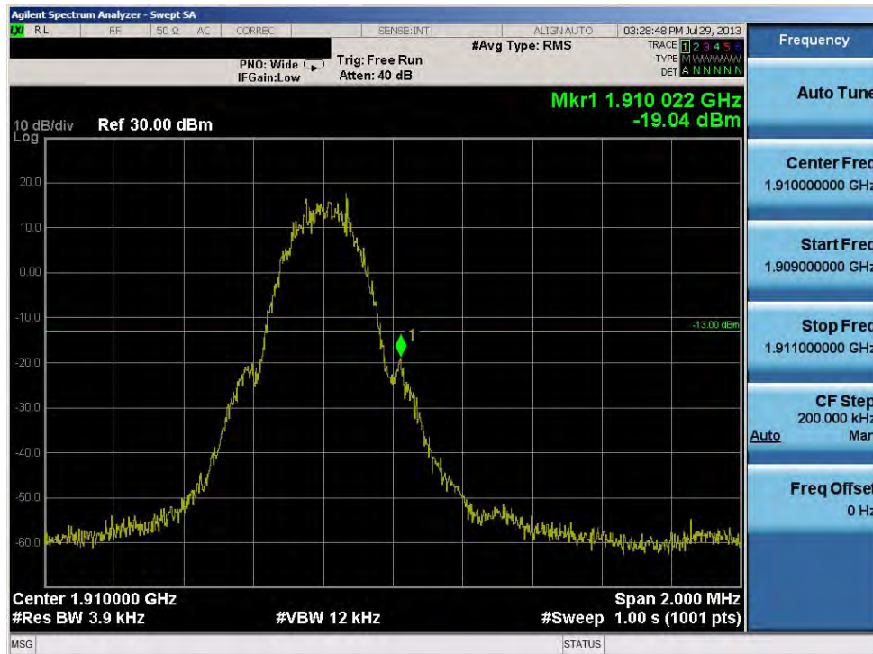
Plot 6-64. Band Edge Plot (PCS GSM Mode – Ch. 810)
