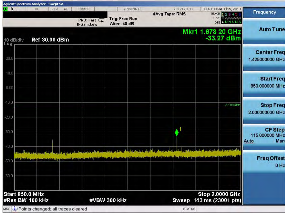
Plot 6-40. Conducted Spurious Plot (Cellular GSM Mode – Ch. 190)
