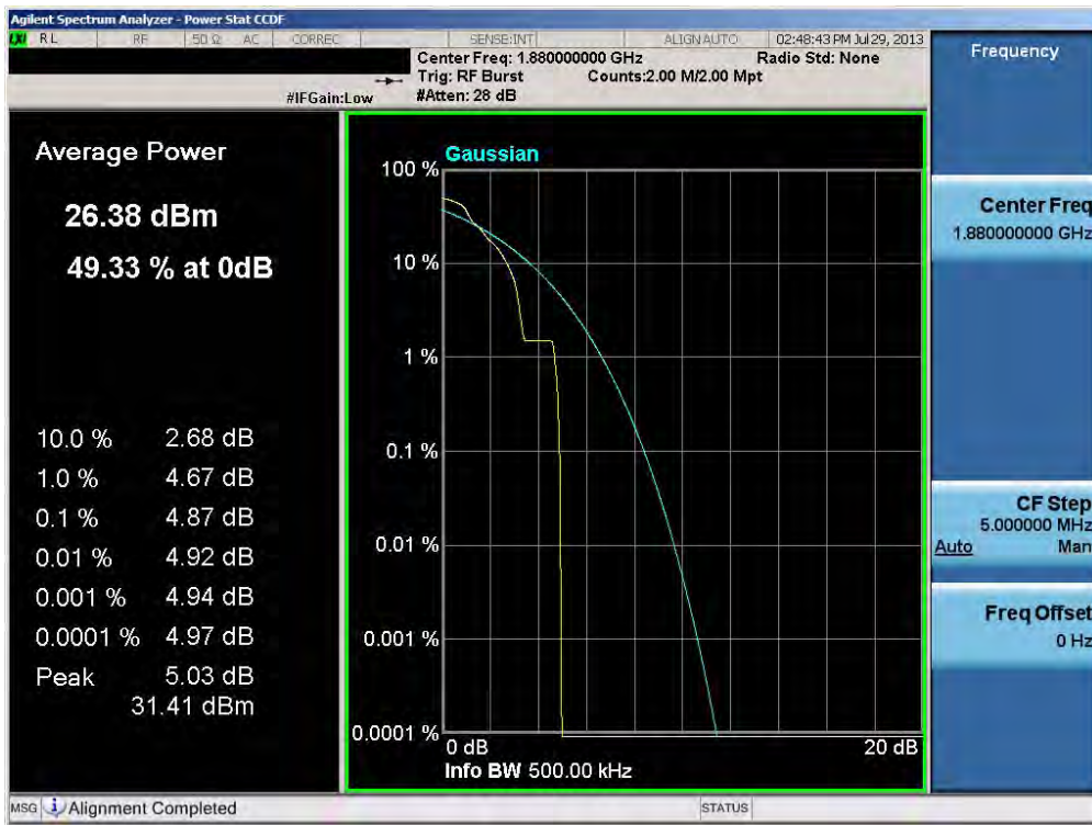
Plot 6-66. Peak-Average Ratio Plot (EDGE1900 Mode – Ch. 661)
