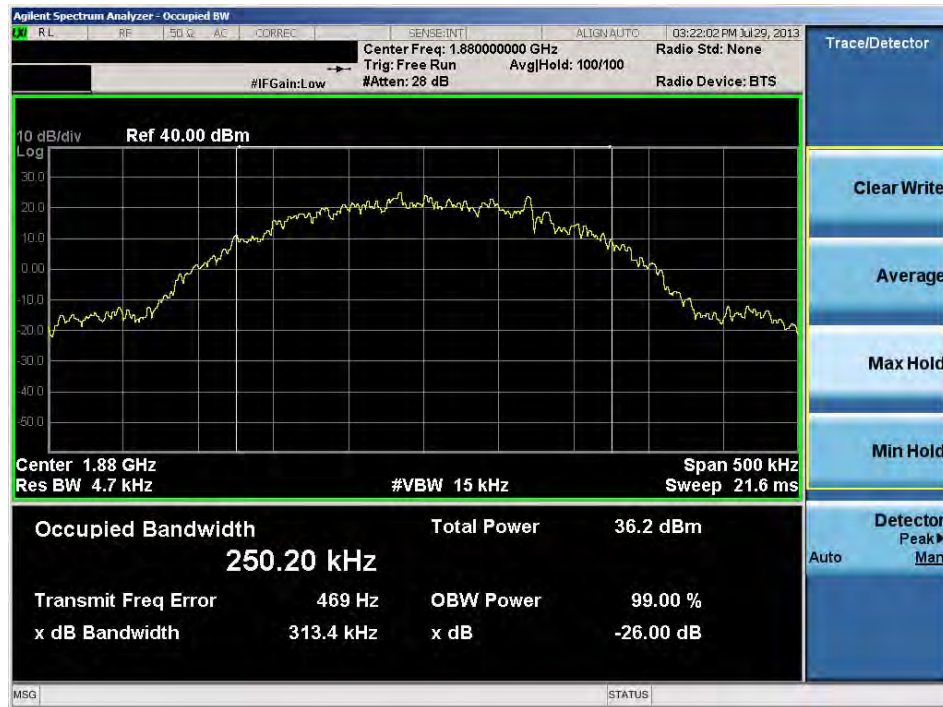
Plot 6-8. Occupied Bandwidth Plot (PCS GSM Mode – Ch. 661)
