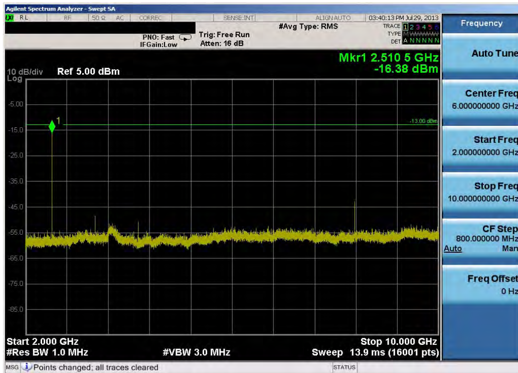
Plot 6-41. Conducted Spurious Plot (Cellular GSM Mode – Ch. 190)
