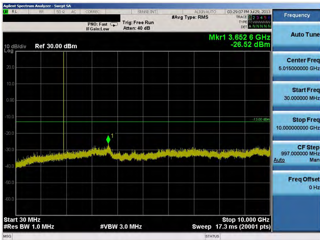
Plot 6-49. Conducted Spurious Plot (PCS GSM Mode – Ch. 810)
