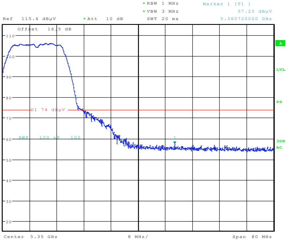
Plot 6-66. Radiated Restricted Upper Band Edge Plot (Peak – UNII Band 2)
