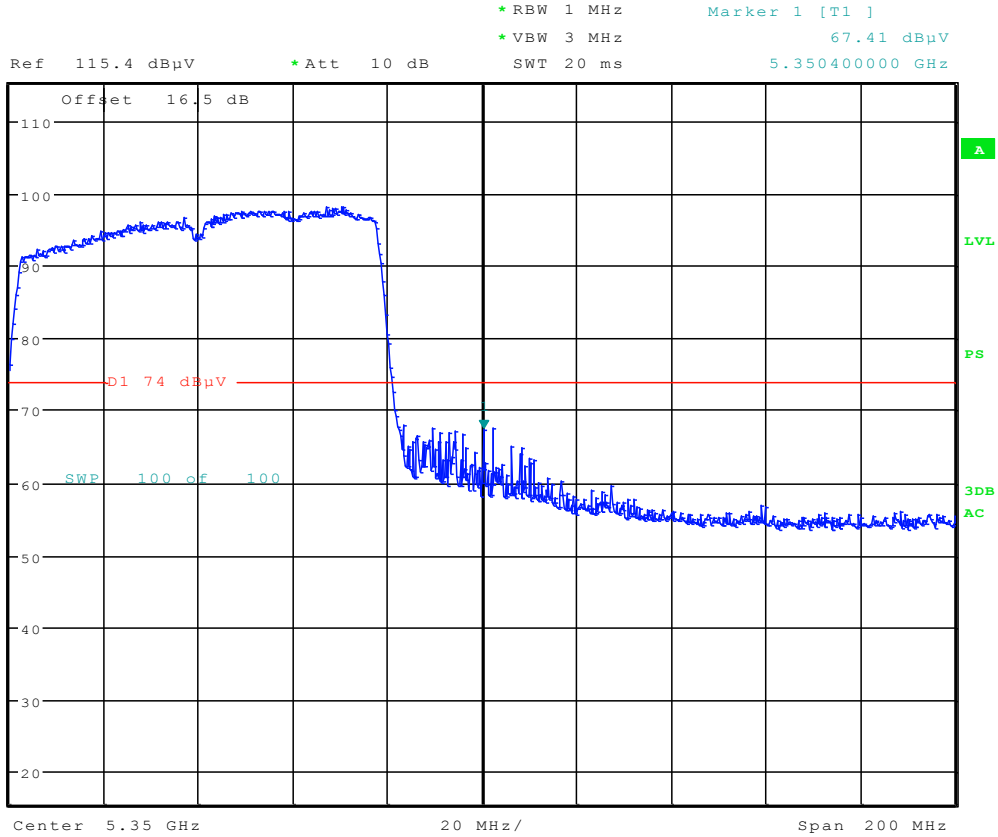
Plot 6-80. Radiated Restricted Upper Band Edge Plot (Peak – UNII Band 2)
