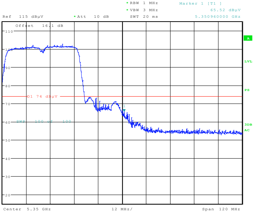
Plot 6-73. Radiated Restricted Upper Band Edge Plot (Peak – UNII Band 2)
