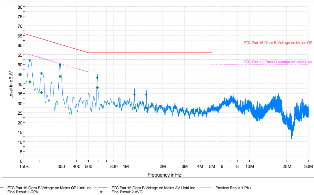
Plot 6-87. Line Conducted Plot with 802.11a UNII Band 3 (L1)
