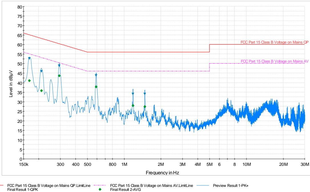
Plot 6-84. Line Conducted Plot with 802.11a UNII Band 1 (N)
