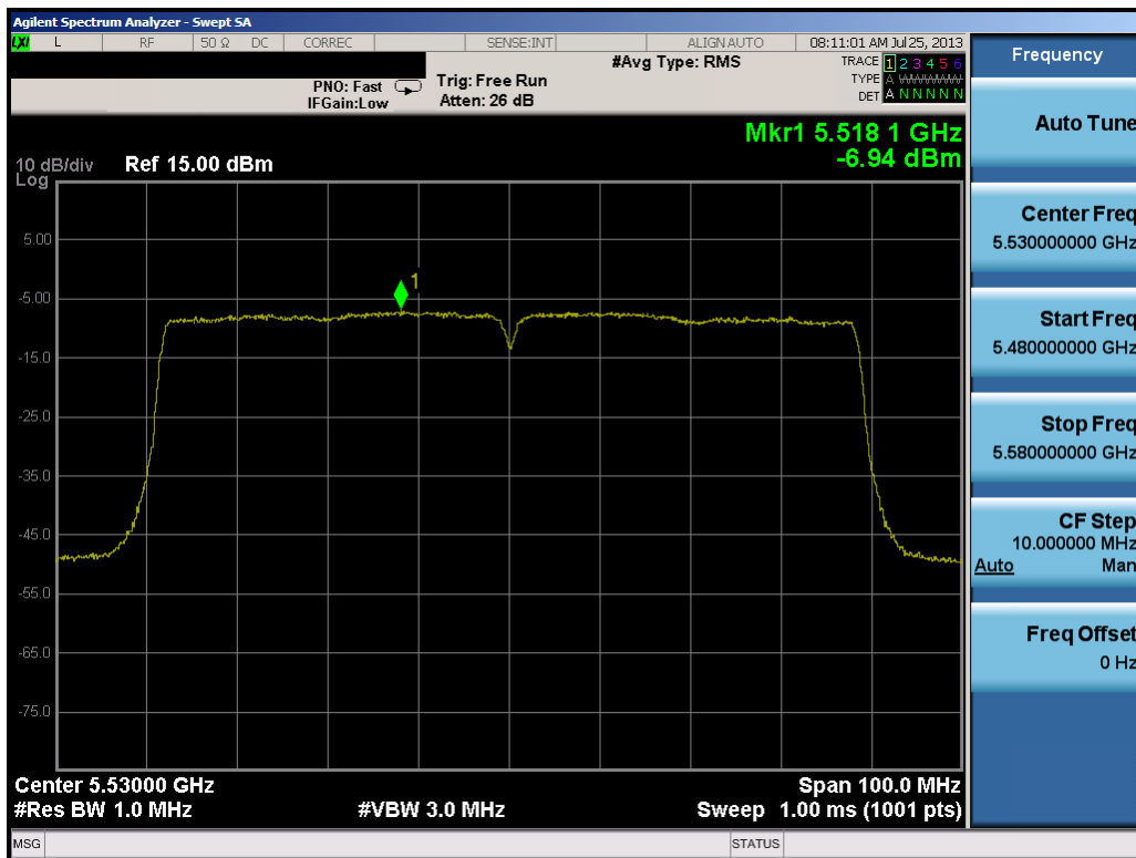
Plot 6-58. Peak Power Spectral Density Plot (80MHz BW 802.11ac (UNII Band 3) – Ch. 106)
