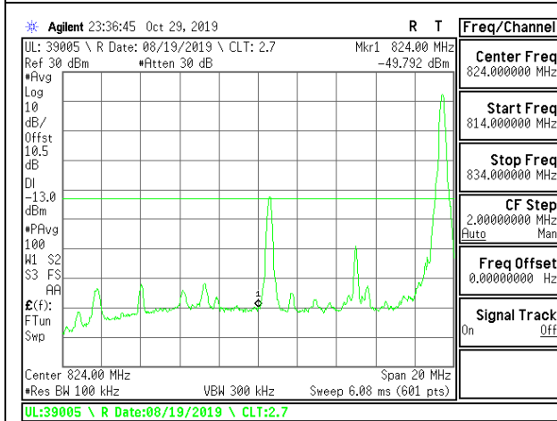
LTE B5 10MHz QPSK Low Channel RB1-49
