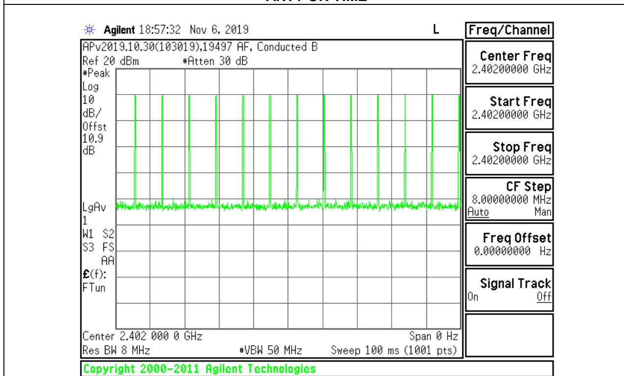
ANT+ 100ms PERIOD
