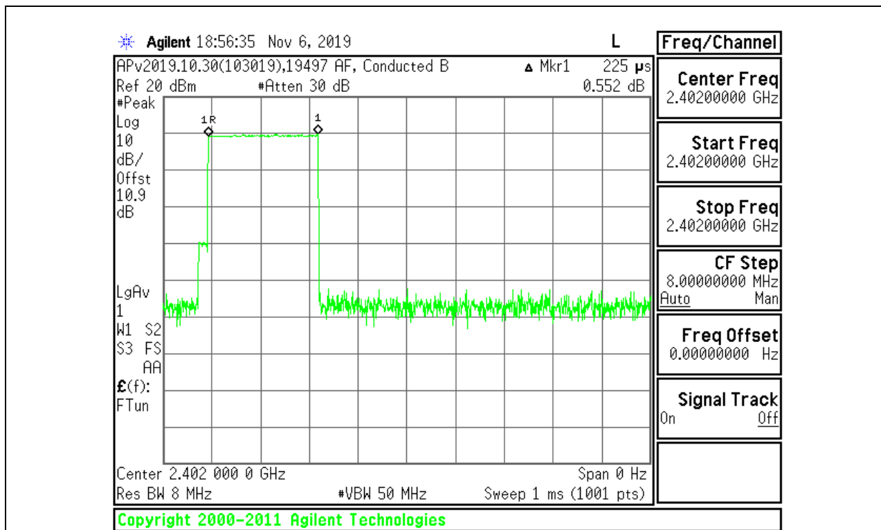
ANT+ ON TIME
