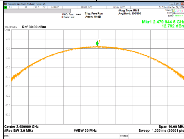
8PSK, 78 CHANNEL
