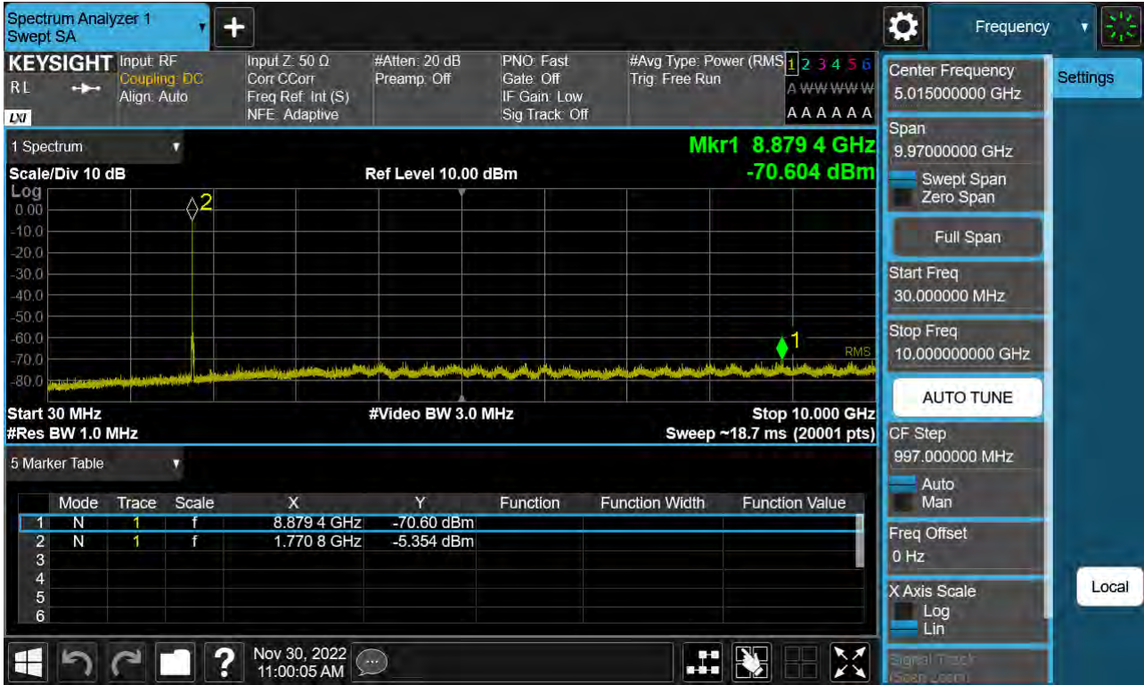
Sub6 n66. Conducted Spurious Plot_1 (355000ch_10 MHz_BPSK_RB 1_1)
