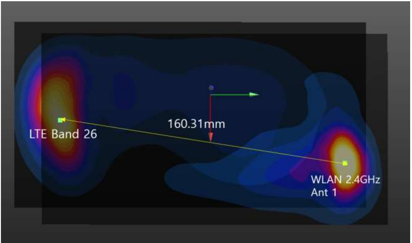
#2 LTE Band 26 + 2.4 GHz WLAN SISO Ant.1
