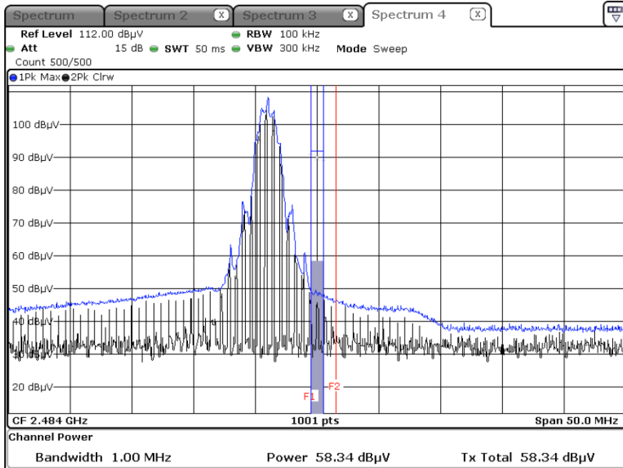
Radiated Restricted Band Edges plot – Peak Result (Ch.39, X-H) 2484 MHz
