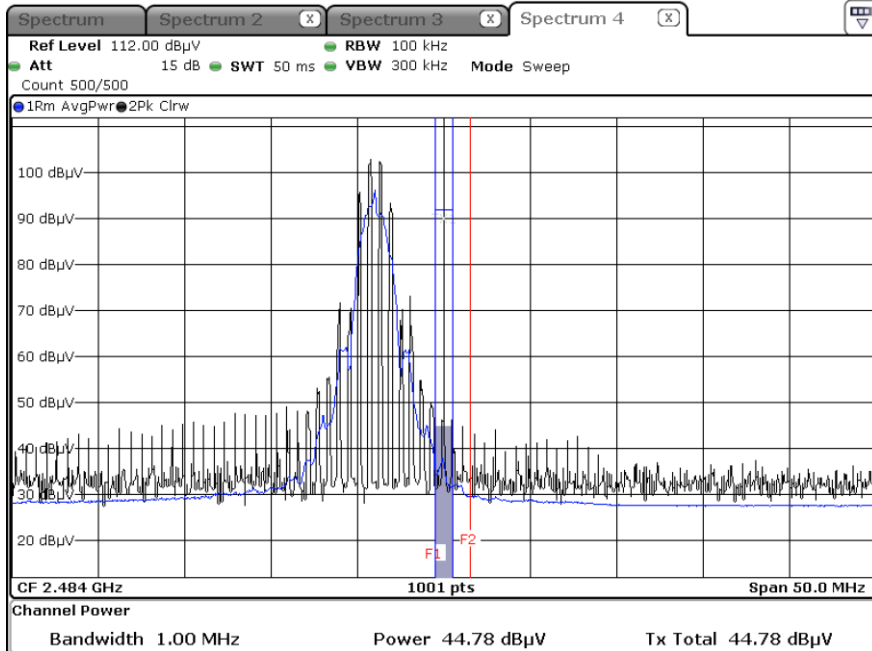
Radiated Restricted Band Edges plot – Average Result (Ch.39, X-H) 2484 MHz
