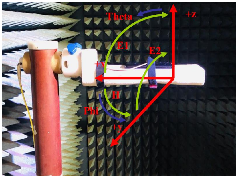
Geometry for SM-M546B for Radiation patterns.
