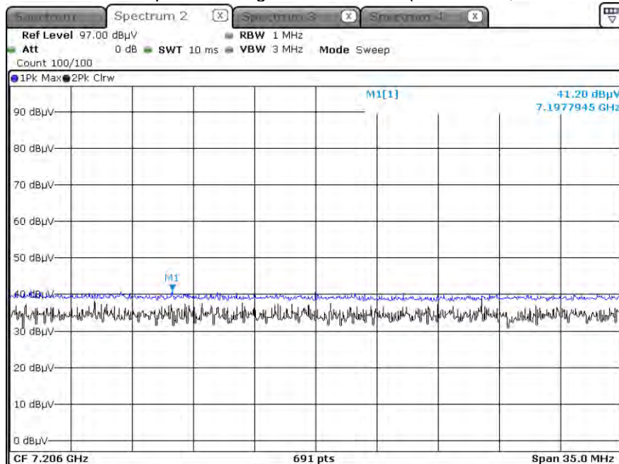
Radiated Spurious Emissions plot – Average & Peak Result ( \pi/4 DQPSK, Ch.0 3rd Harmonic, Y-H)
