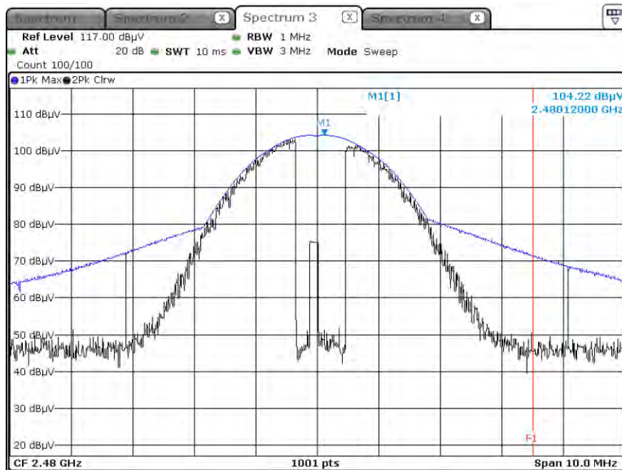
Radiated Restricted Band Edges plot – Fundamental Result ( \pi/4 DQPSK, Ch.78, X-H) 2 483.5 MHz ~ 2 485.5 MHz
