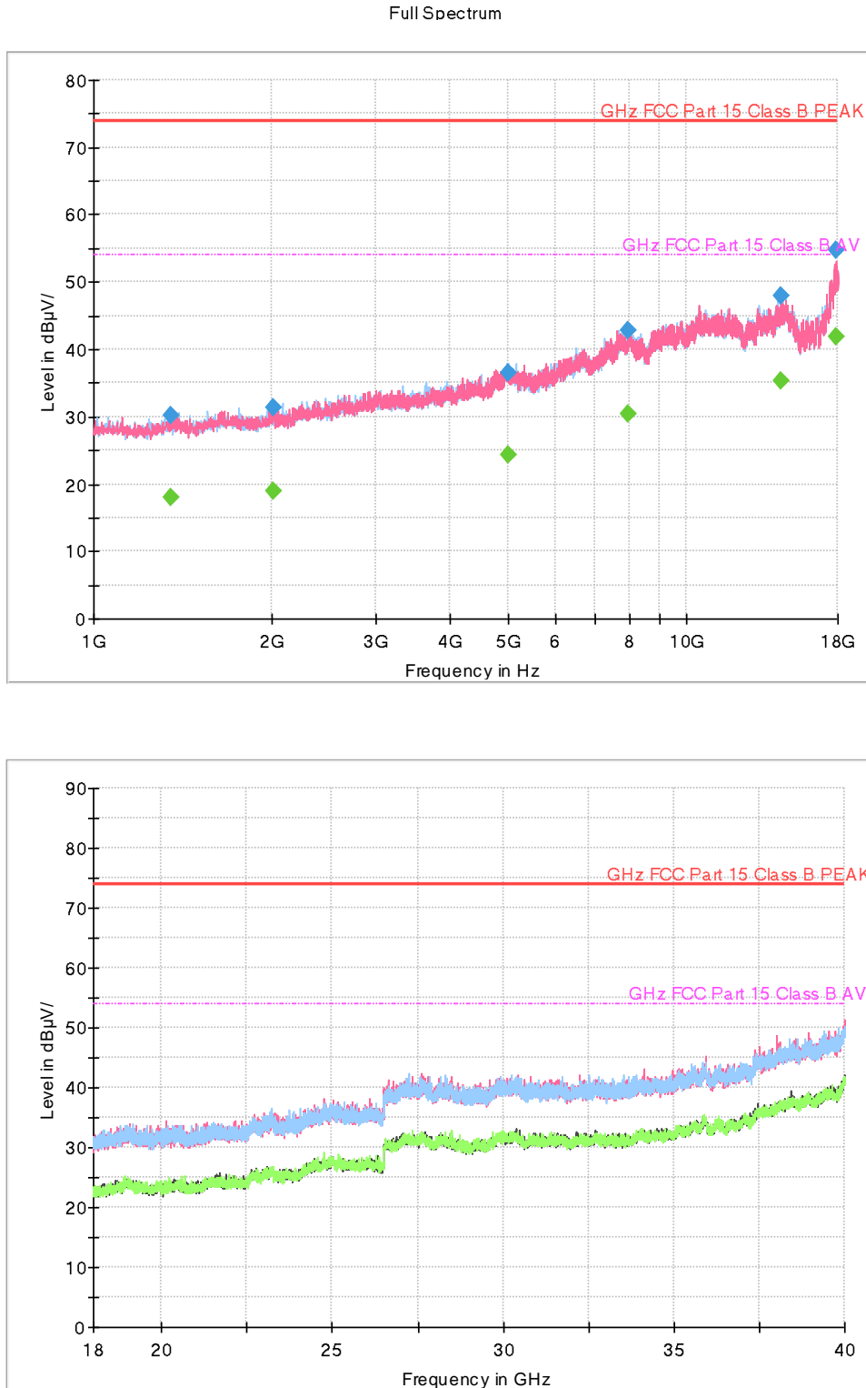
Figure 6: Radiated Emission (1 to 40) GHz, [EUT+Earphone] LTE B12(B17) Middle ch Idle
