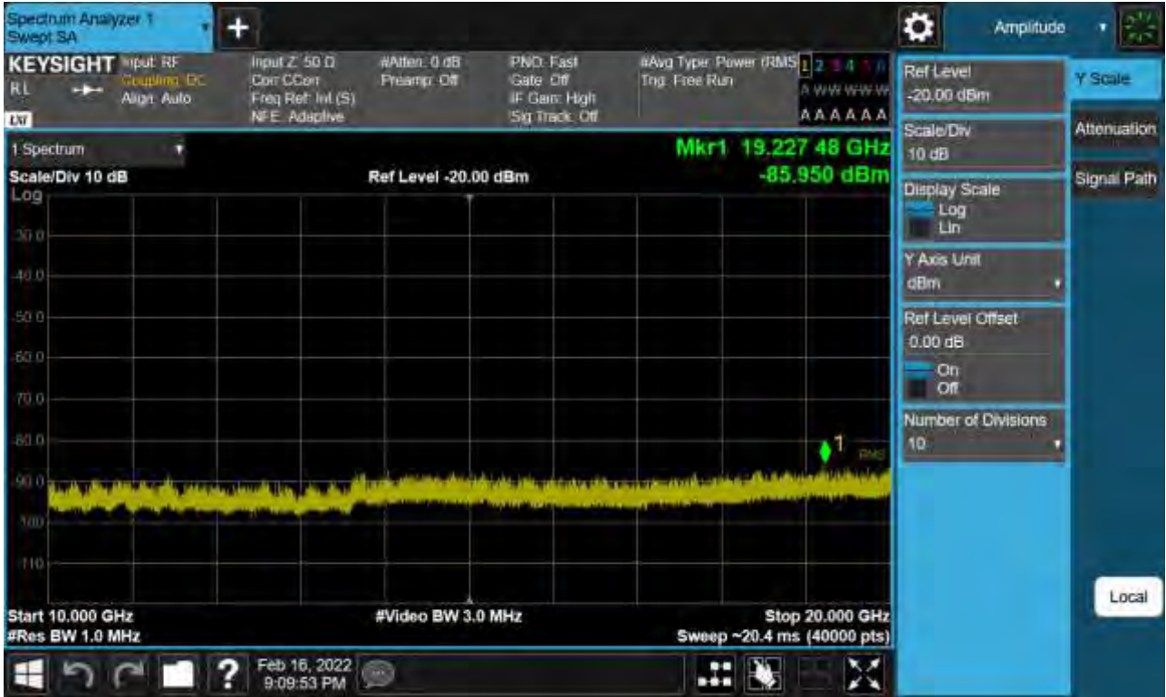
Sub6 n66. Conducted Spurious Plot_2 (349000ch_30 MHz_BPSK_RB 1_1)
