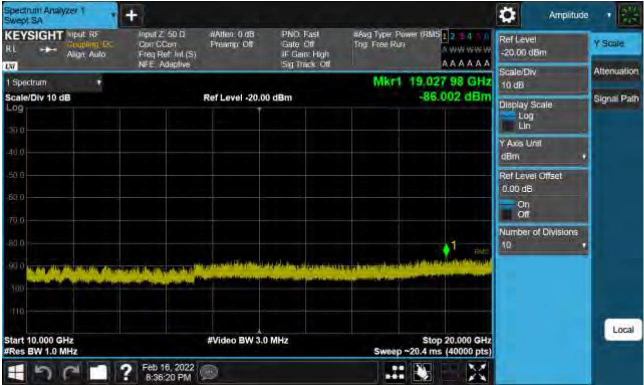
Sub6 n66. Conducted Spurious Plot_2 (343000ch_10 MHz_BPSK_RB 1_1)
