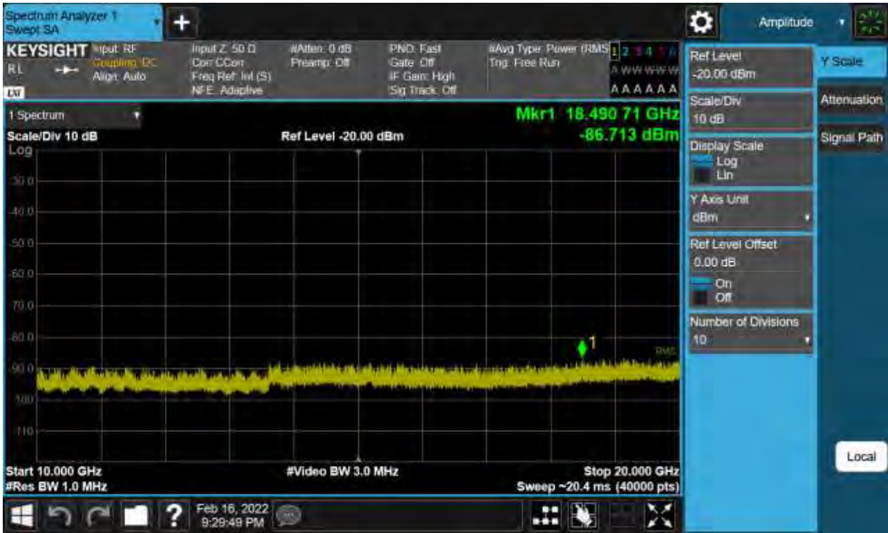
Sub6 n66. Conducted Spurious Plot_2 (352000ch_40 MHz_BPSK_ RB 1_1)
