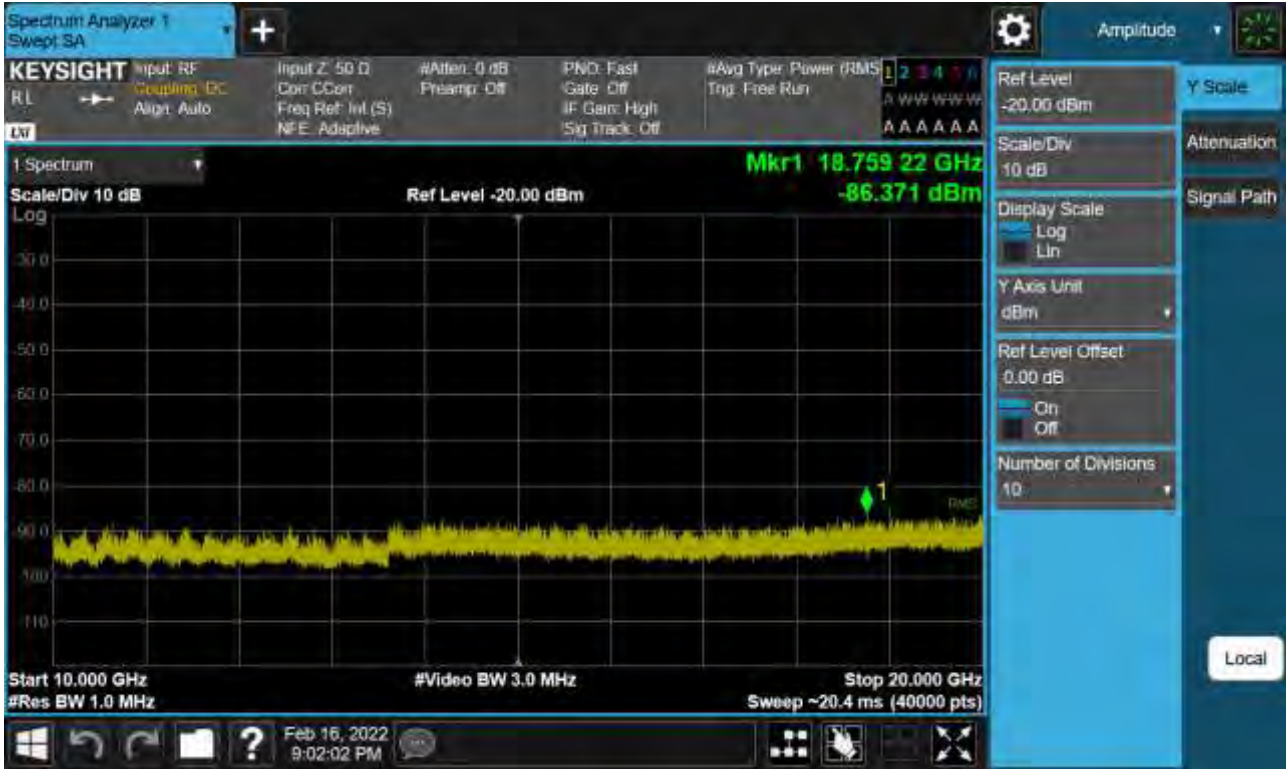
Sub6 n66. Conducted Spurious Plot_2 (349000ch_25 MHz_BPSK_RB 1_1)
