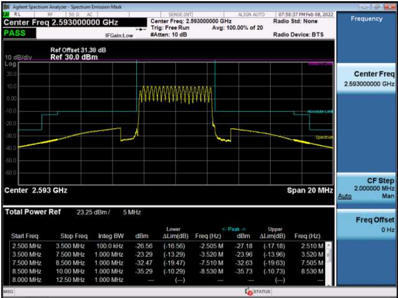
Mid Channel Edge Plot (5 MHz Ch.40620 QPSK RB 25)
