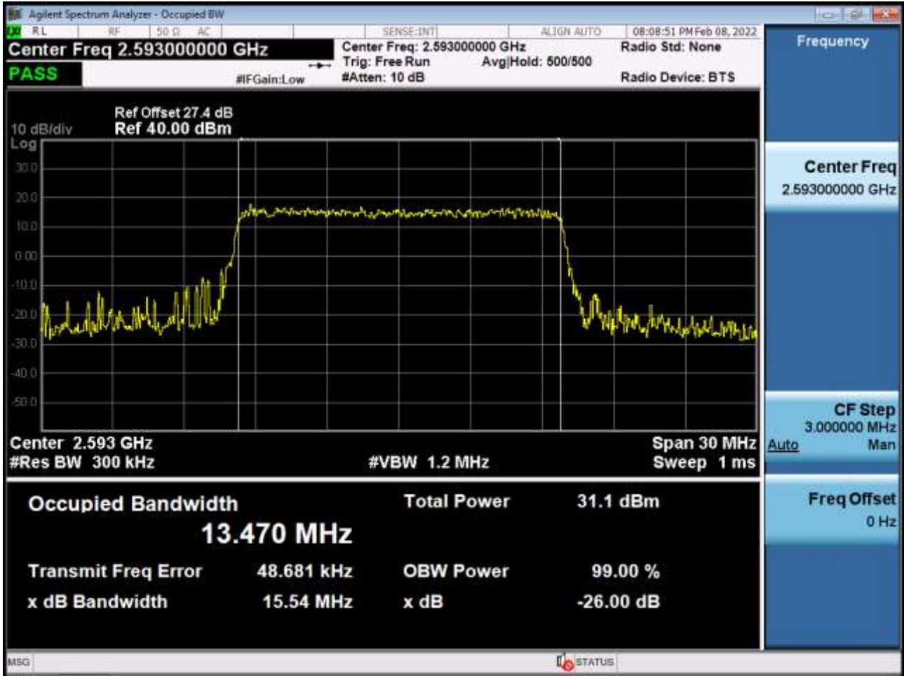
Occupied Bandwidth Plot (15 MHz Ch.40620 QPSK RB 75)
