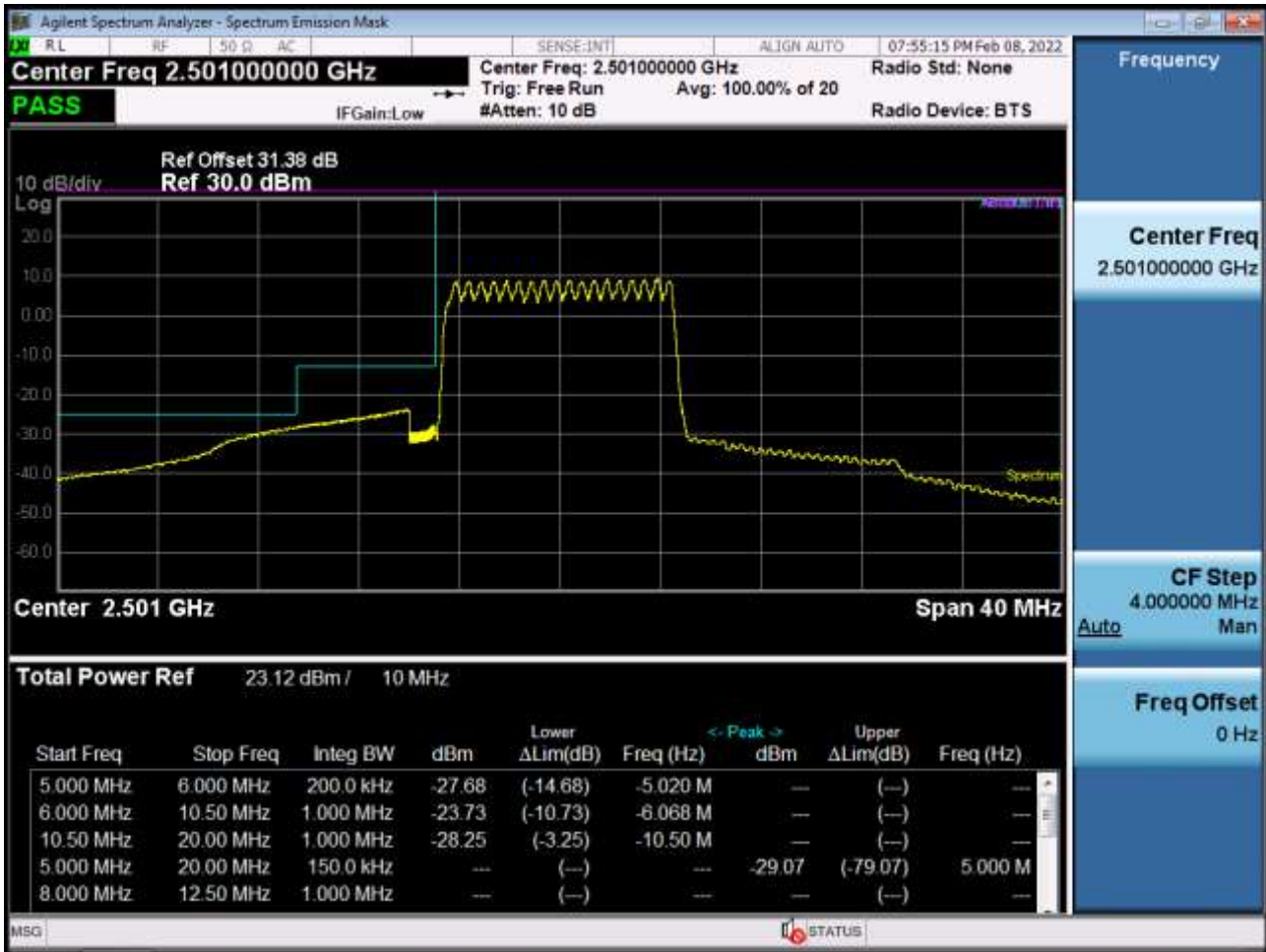
Low Channel Edge Plot (10 MHz Ch.39700 QPSK_RB50_Offset 0)-1
