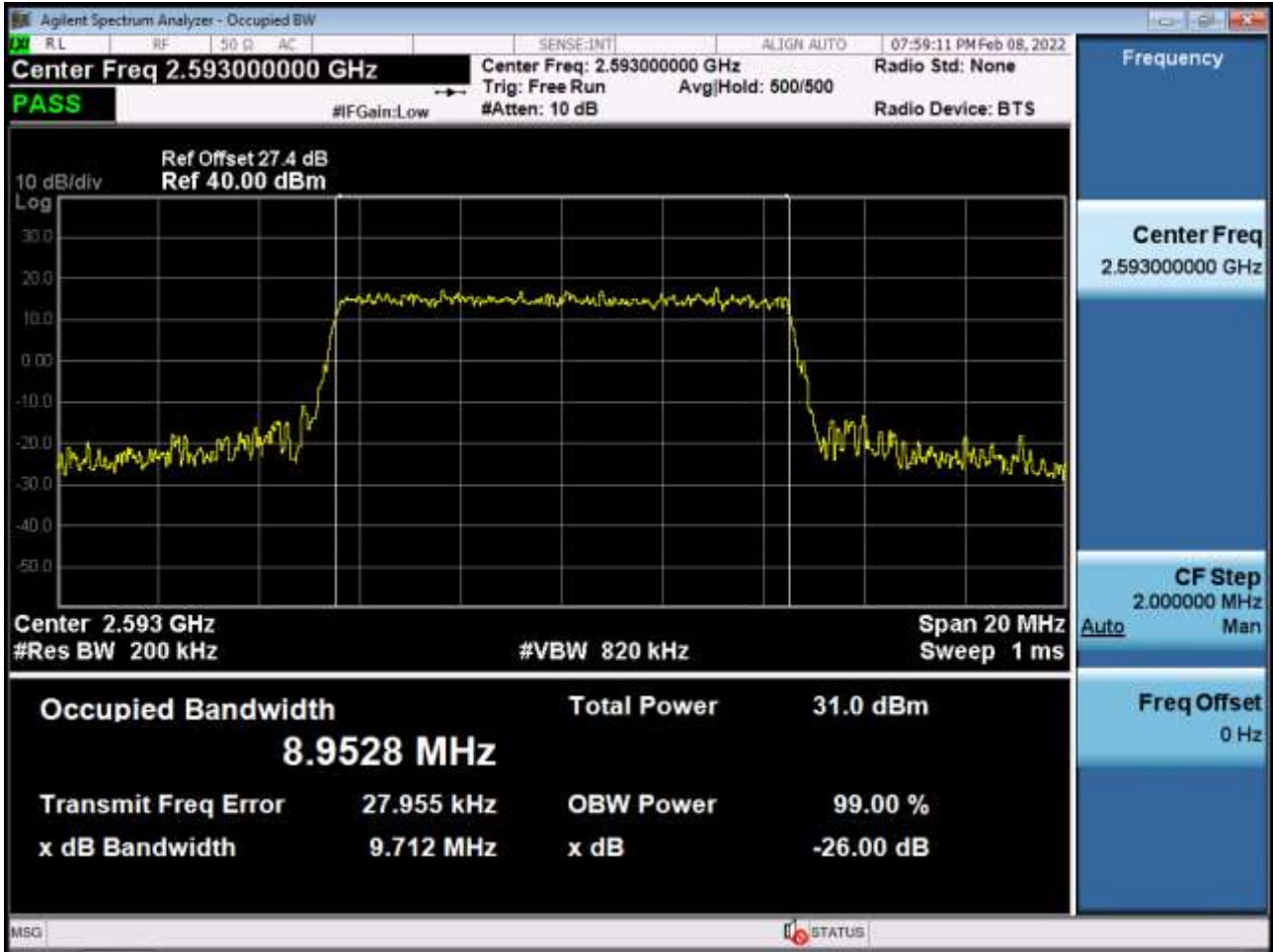
Occupied Bandwidth Plot (10 MHz Ch.40620 QPSK RB 50)
