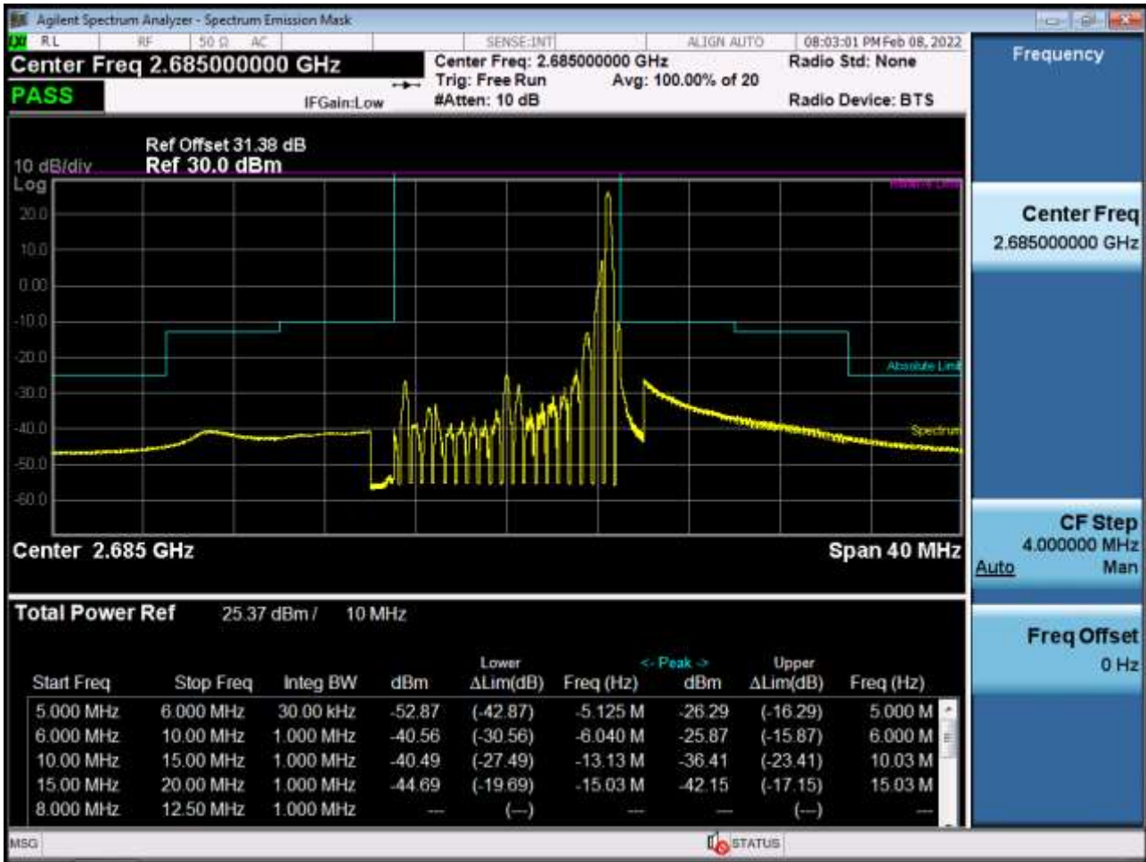
High Channel Edge Plot (10 MHz Ch.41540 QPSK RB 1, Offset 24)
