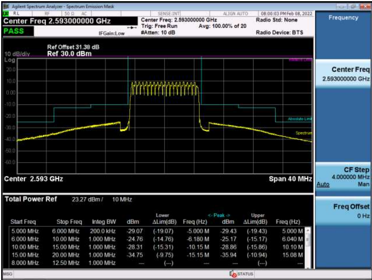
Mid Channel Edge Plot (10 MHz Ch.40620 QPSK RB 50)
