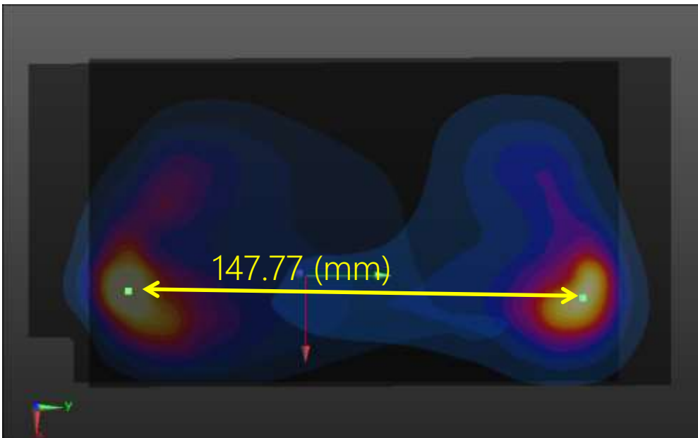
Plot #2 LTE Band 2 + WLAN 2.4 GHz
