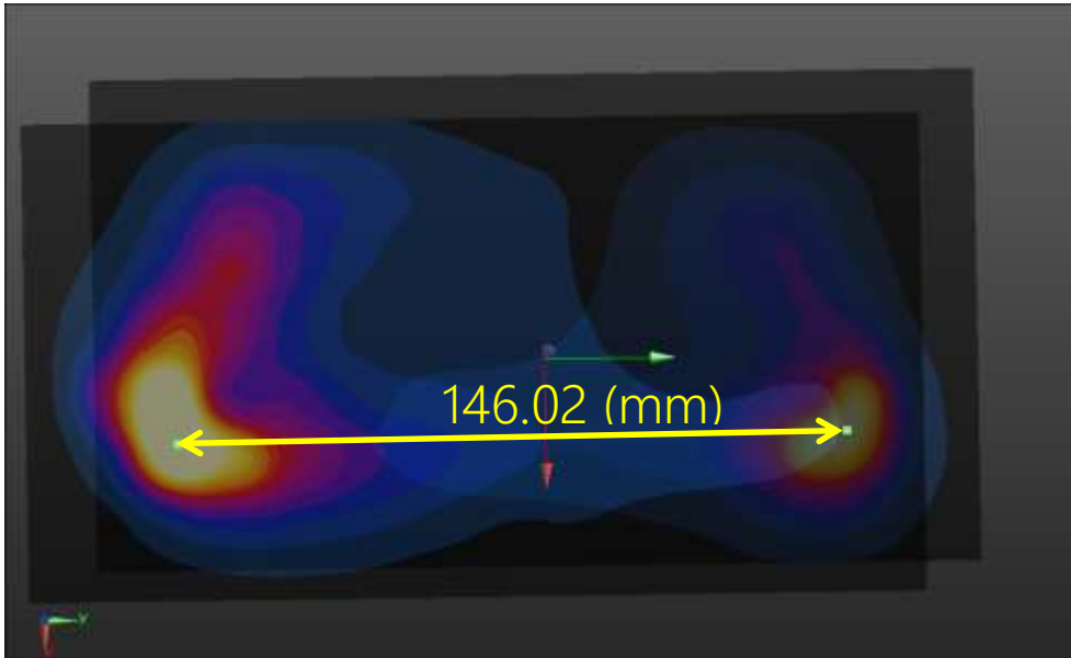
Plot #1 GPRS 1900 + WLAN 2.4 GHz
