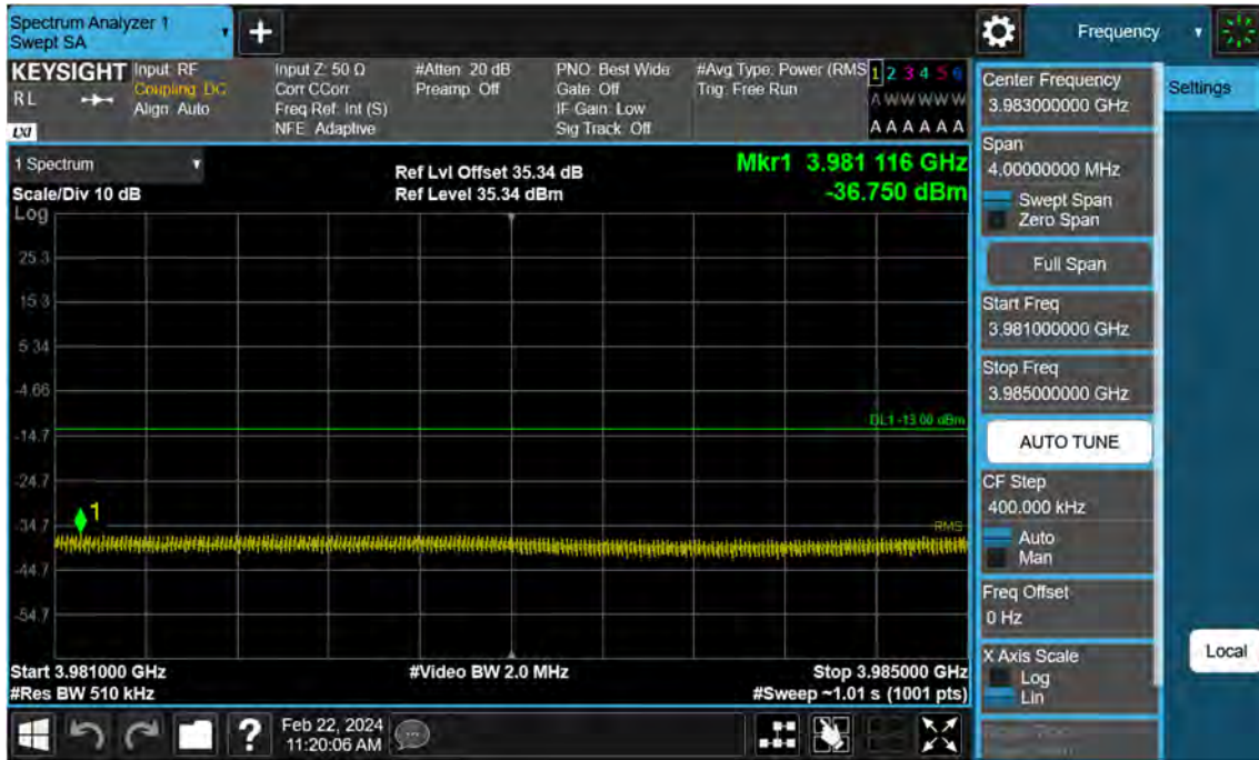
Sub6 n77. High Band Edge Plot (40 M BW Ch.664000 BPSK FullRB)(2)
