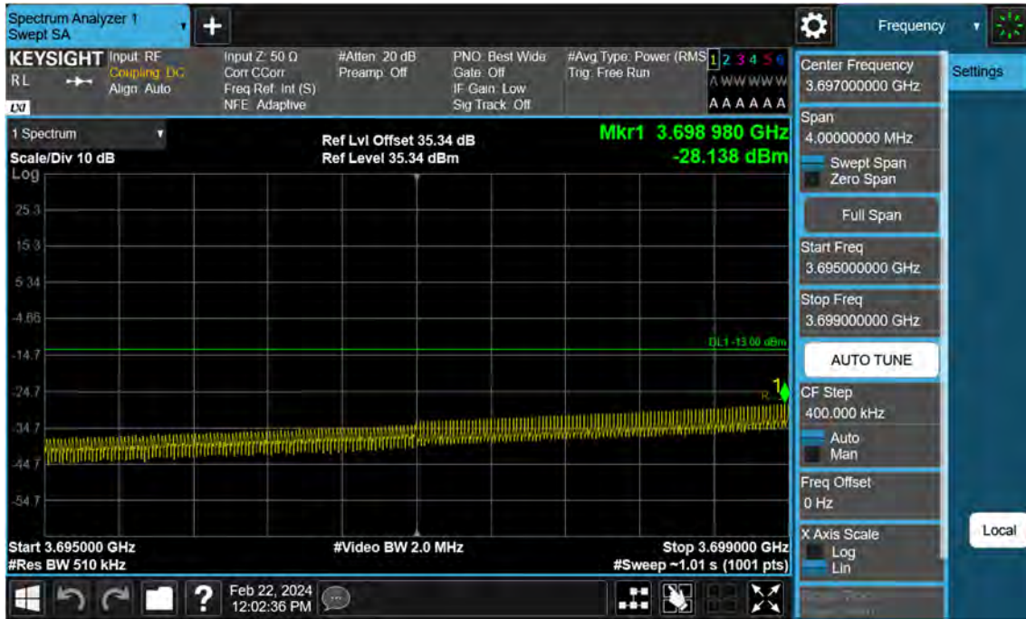
Sub6 n77. Low Band Edge Plot (80 M BW Ch.649334 BPSK FullRB)(2)
