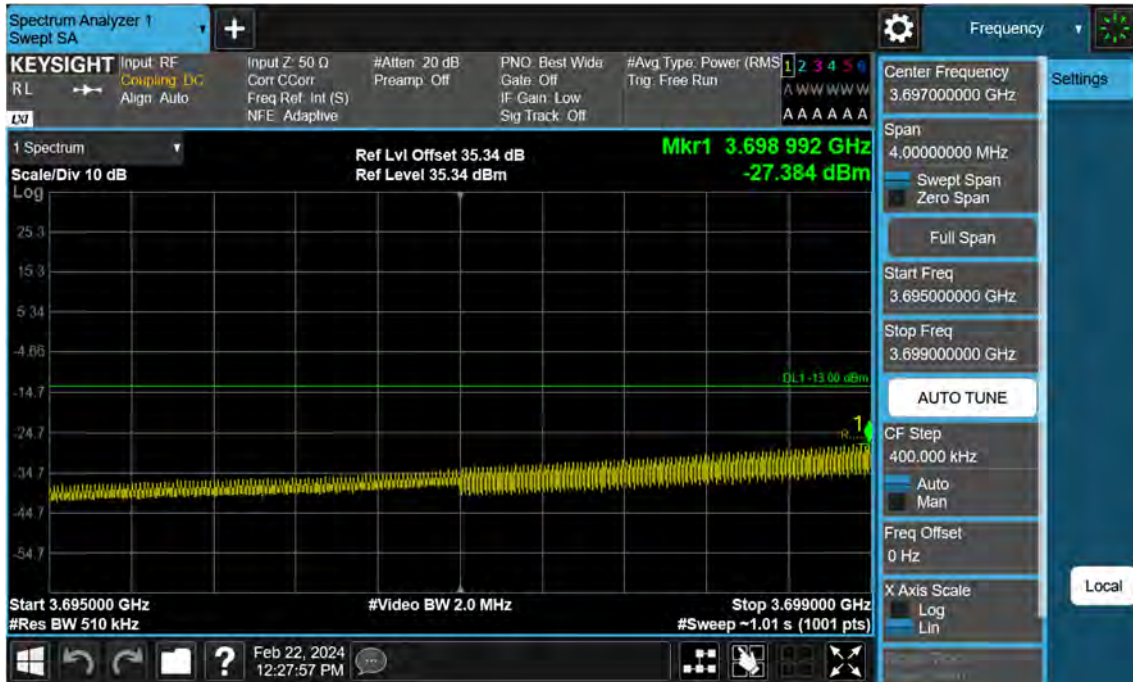
Sub6 n77. Low Band Edge Plot (100 M BW Ch.650000 BPSK FullRB)(2)
