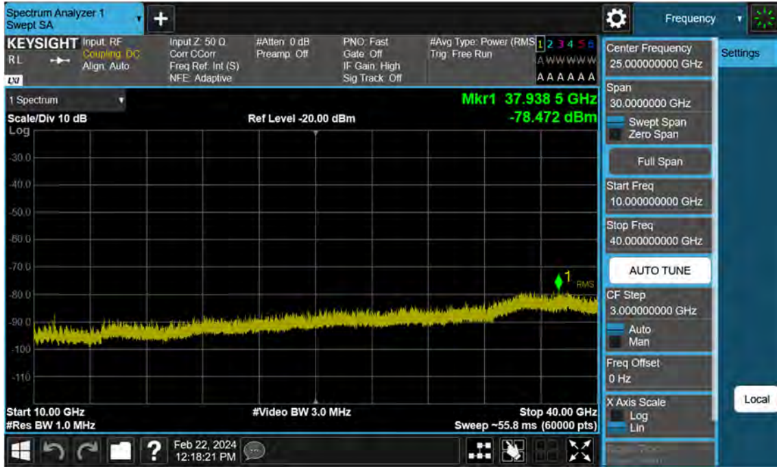
Sub6 n77. Conducted Spurious Plot_2 (649668ch_90 MHz_BPSK)
