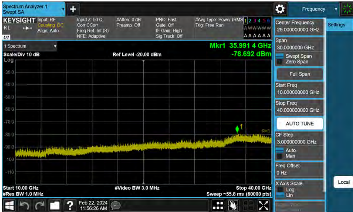
Sub6 n77. Conducted Spurious Plot_2 (656000ch_70 MHz_BPSK)
