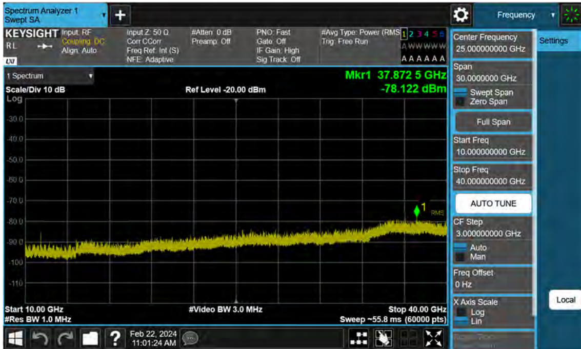
Sub6 n77. Conducted Spurious Plot_2 (647668ch_30 MHz_BPSK)
