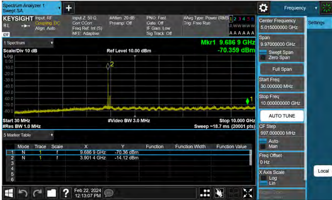
Sub6 n77. Conducted Spurious Plot_1 (662666ch_80 MHz_BPSK)
