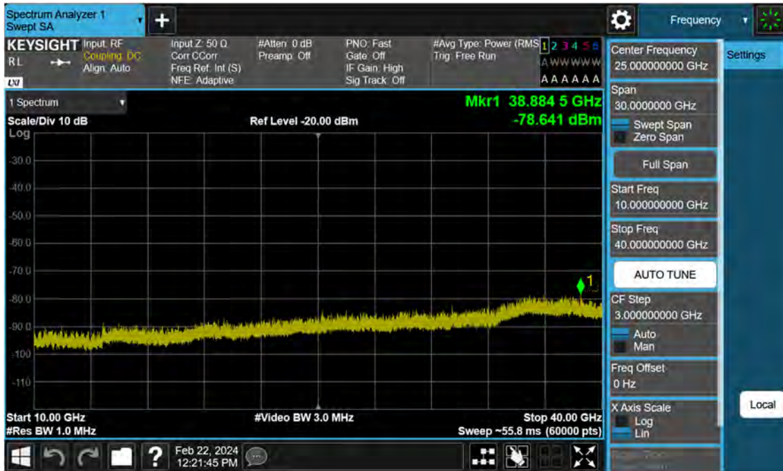
Sub6 n77. Conducted Spurious Plot_2 (656000ch_90 MHz_BPSK)
