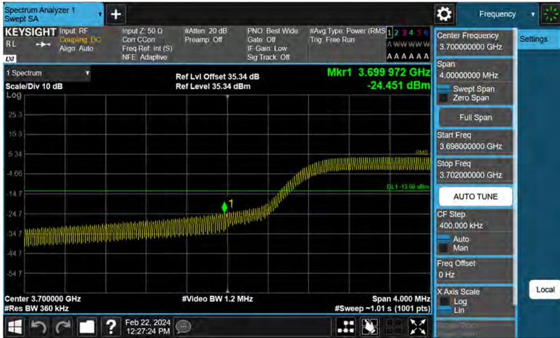
Sub6 n77. Low Band Edge Plot (100 M BW Ch.650000 BPSK FullRB)(1)
