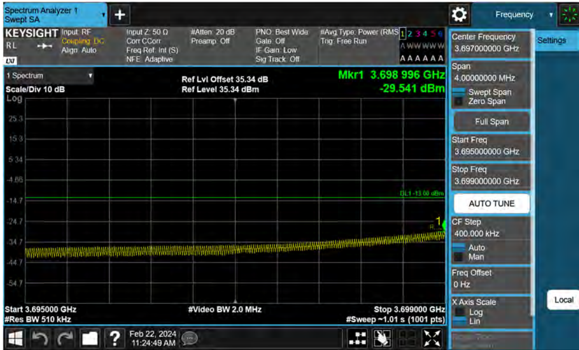
Sub6 n77. Low Band Edge Plot (50 M BW Ch.648334 BPSK FullRB)(2)
