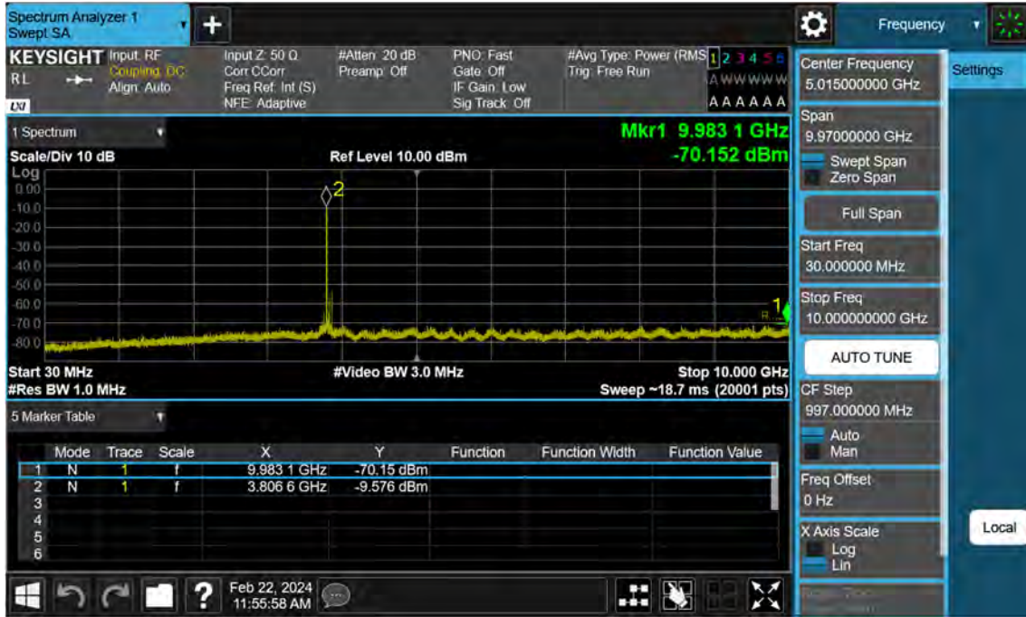
Sub6 n77. Conducted Spurious Plot_1 (656000ch_70 MHz_BPSK)
