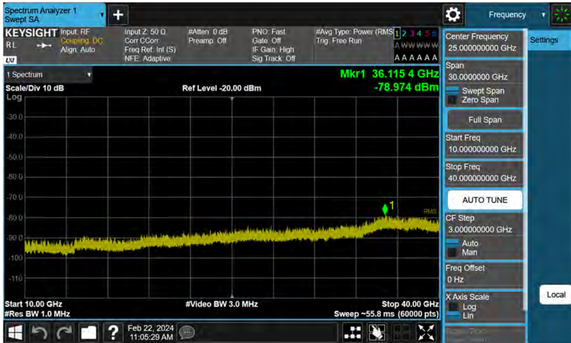
Sub6 n77. Conducted Spurious Plot_2 (656000ch_30 MHz_BPSK)
