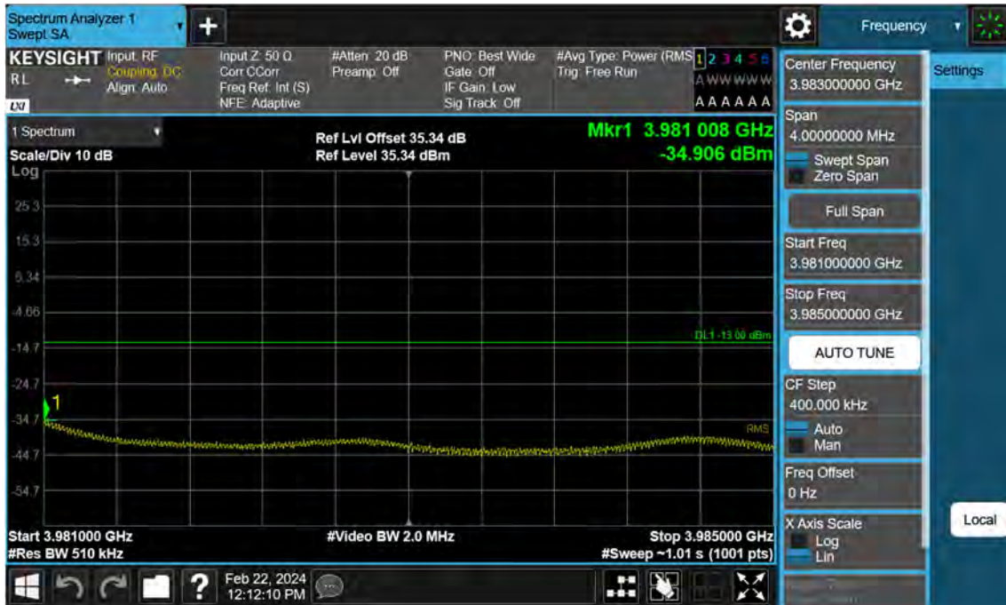
Sub6 n77. High Band Edge Plot (80 M BW Ch.662666 BPSK 1RB)(2)
