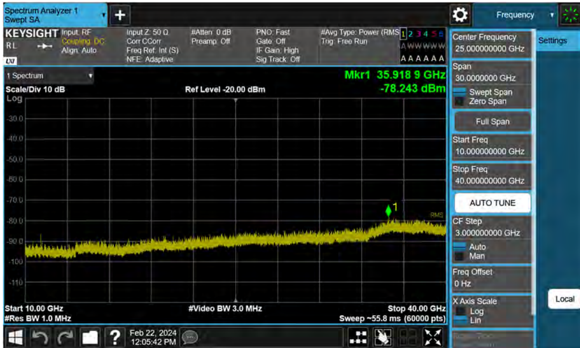
Sub6 n77. Conducted Spurious Plot_2 (649334ch_80 MHz_BPSK)
