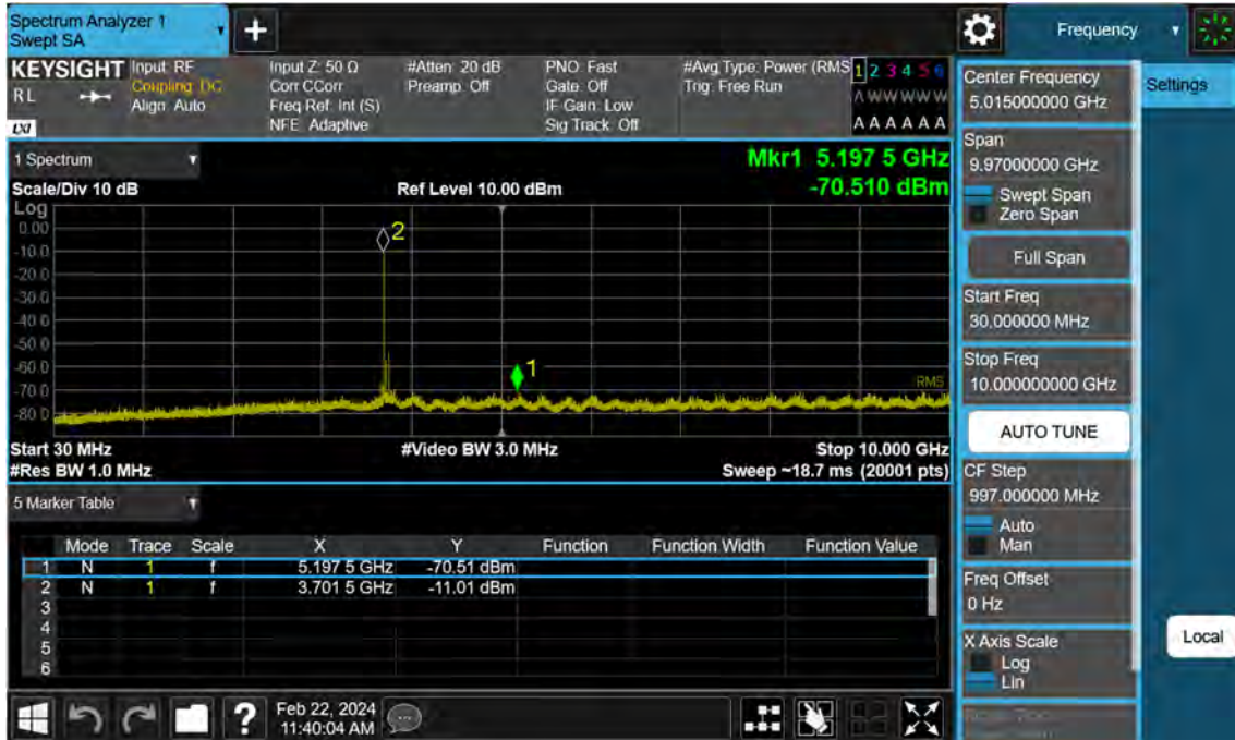
Sub6 n77. Conducted Spurious Plot_1 (648668ch_60 MHz_BPSK)
