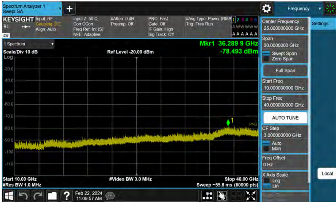
Sub6 n77. Conducted Spurious Plot_2 (664332ch_30 MHz_BPSK)
