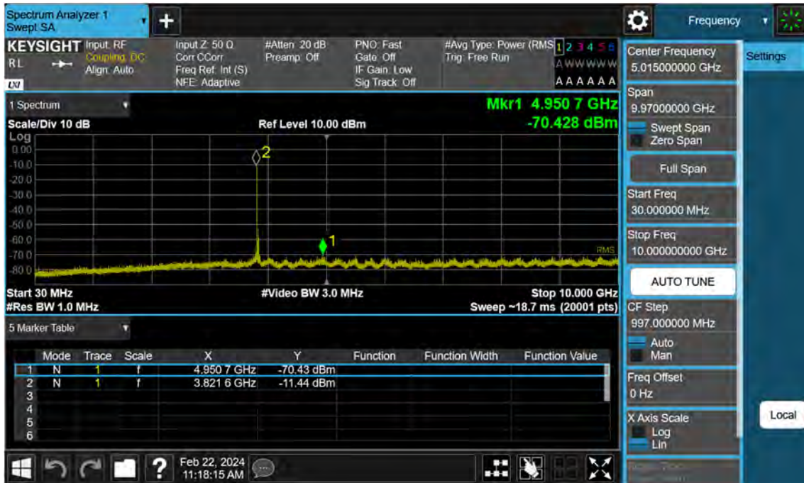
Sub6 n77. Conducted Spurious Plot_1 (656000ch_40 MHz_BPSK)
