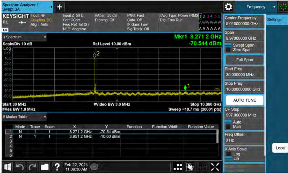
Sub6 n77. Conducted Spurious Plot_1 (664332ch_30 MHz_BPSK)
