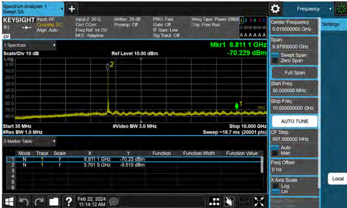
Sub6 n77. Conducted Spurious Plot_1 (648000ch_40 MHz_BPSK)
