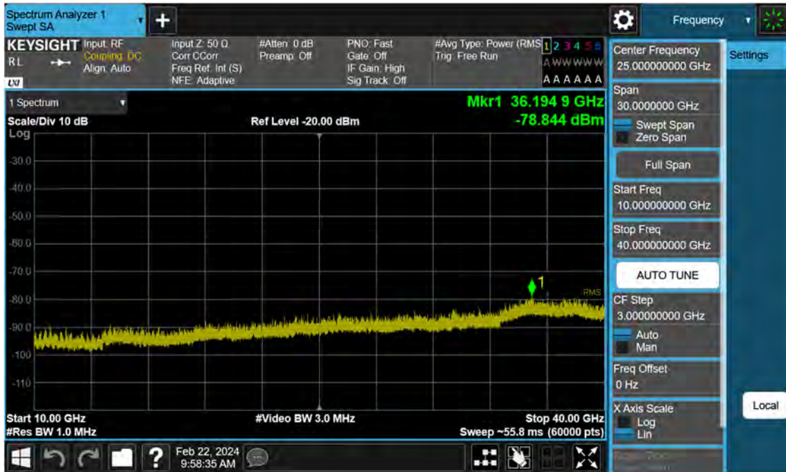
Sub6 n77. Conducted Spurious Plot_2 (656000ch_10 MHz_BPSK)
