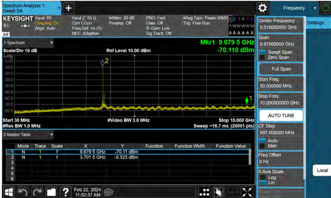
Sub6 n77. Conducted Spurious Plot_1 (649000ch_70 MHz_BPSK)
