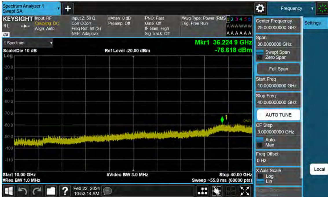
Sub6 n77. Conducted Spurious Plot_2 (656000ch_25 MHz_BPSK)
