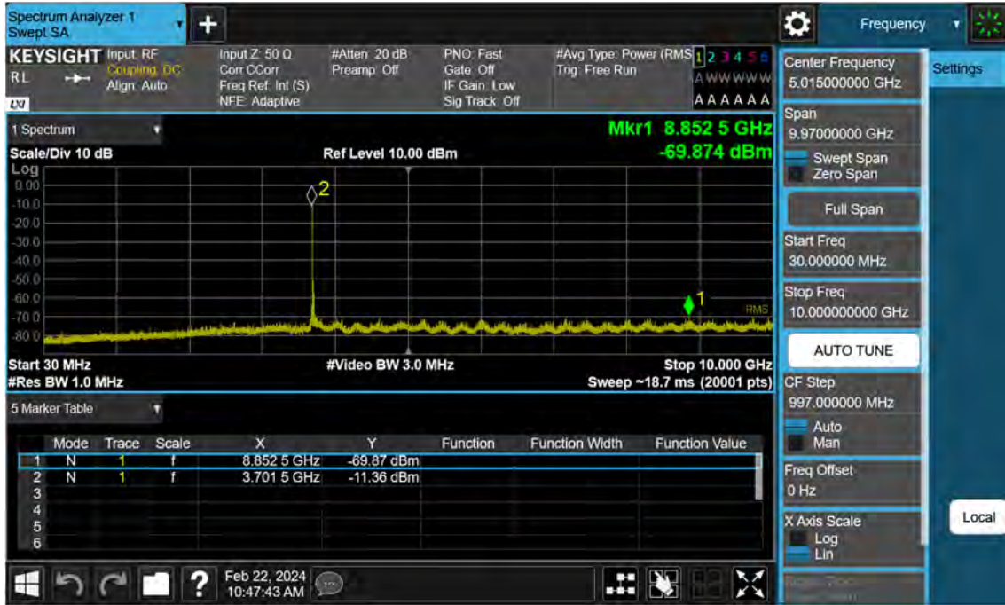
Sub6 n77. Conducted Spurious Plot_1 (647500ch_25 MHz_BPSK)
