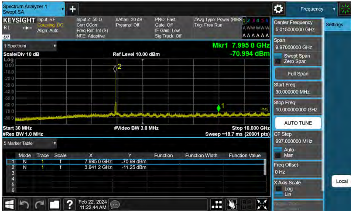
Sub6 n77. Conducted Spurious Plot_1 (664000ch_40 MHz_BPSK)
