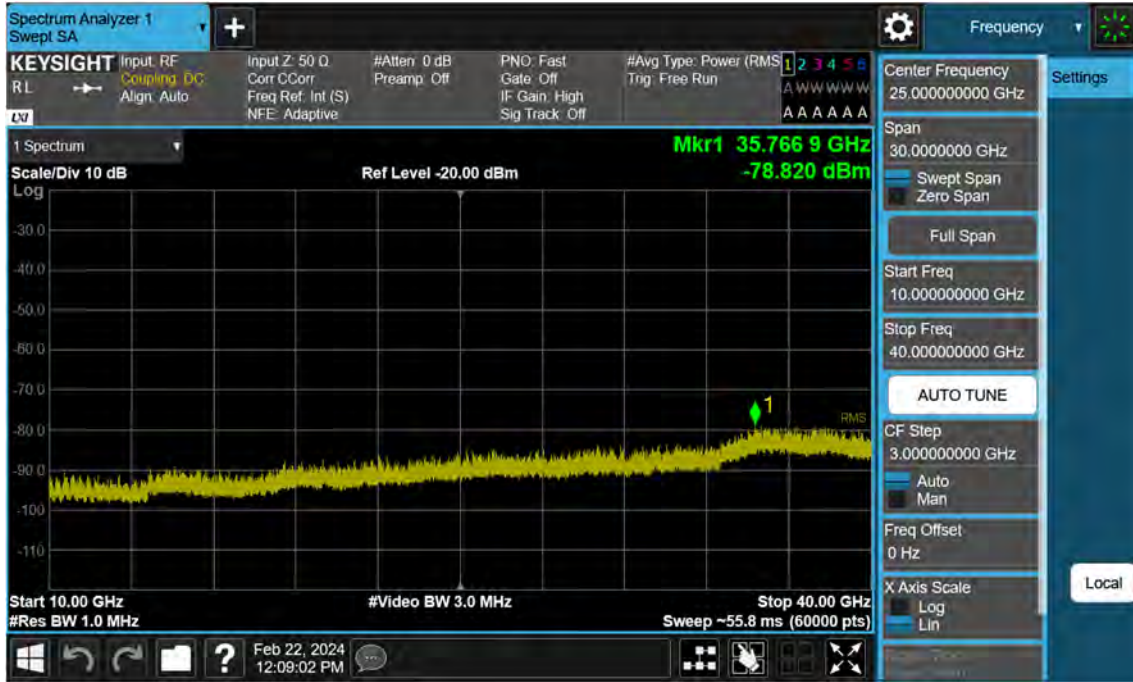
Sub6 n77. Conducted Spurious Plot_2 (656000ch_80 MHz_BPSK)
