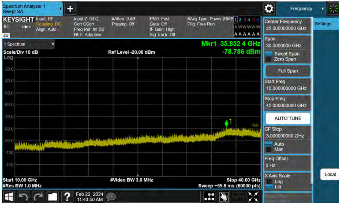
Sub6 n77. Conducted Spurious Plot_2 (656000ch_60 MHz_BPSK)
