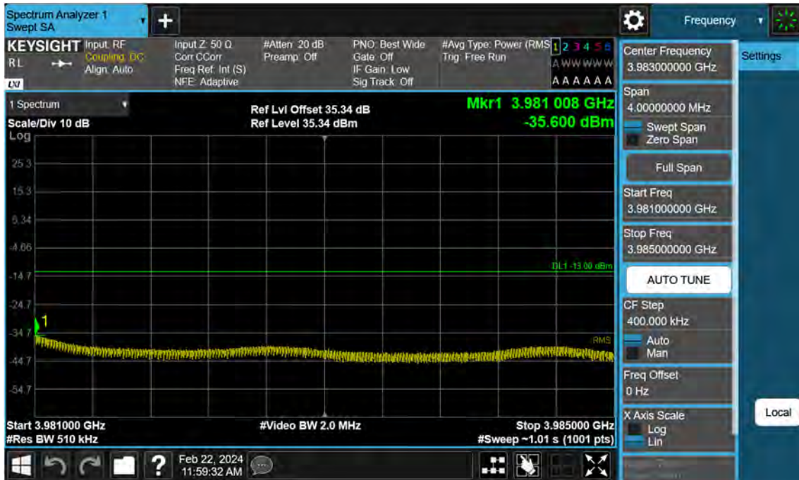
Sub6 n77. High Band Edge Plot (70 M BW Ch.663000 BPSK 1RB)(2)
