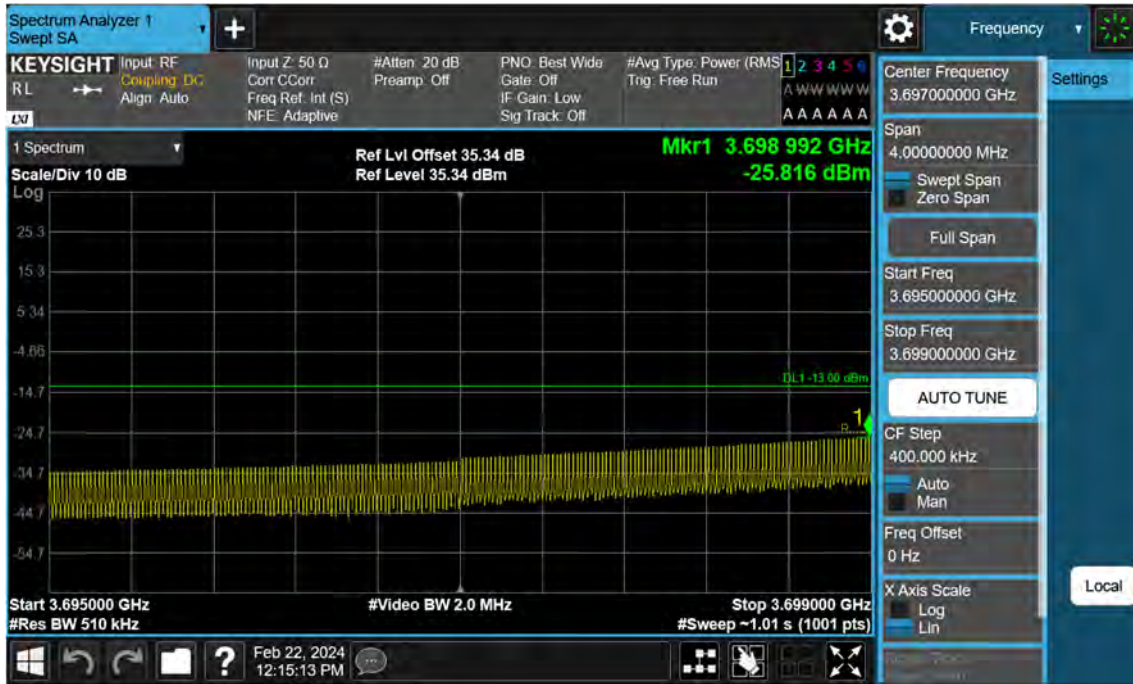
Sub6 n77. Low Band Edge Plot (90 M BW Ch.649668 BPSK FullRB)(2)
