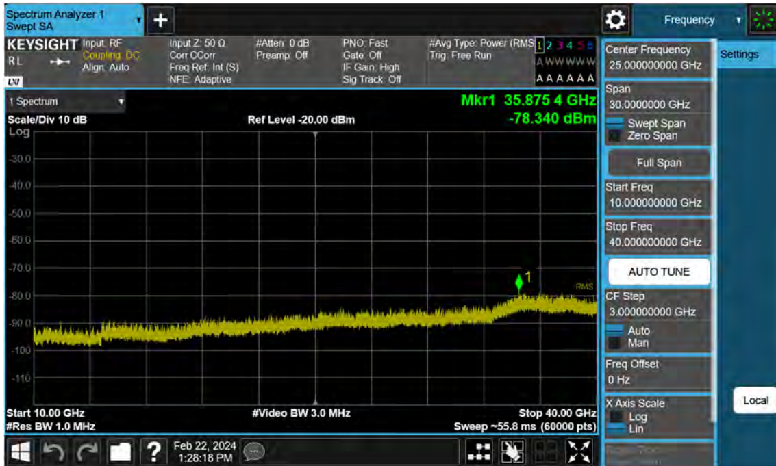
Sub6 n77. Conducted Spurious Plot_2 (656000ch_100 MHz_BPSK)
