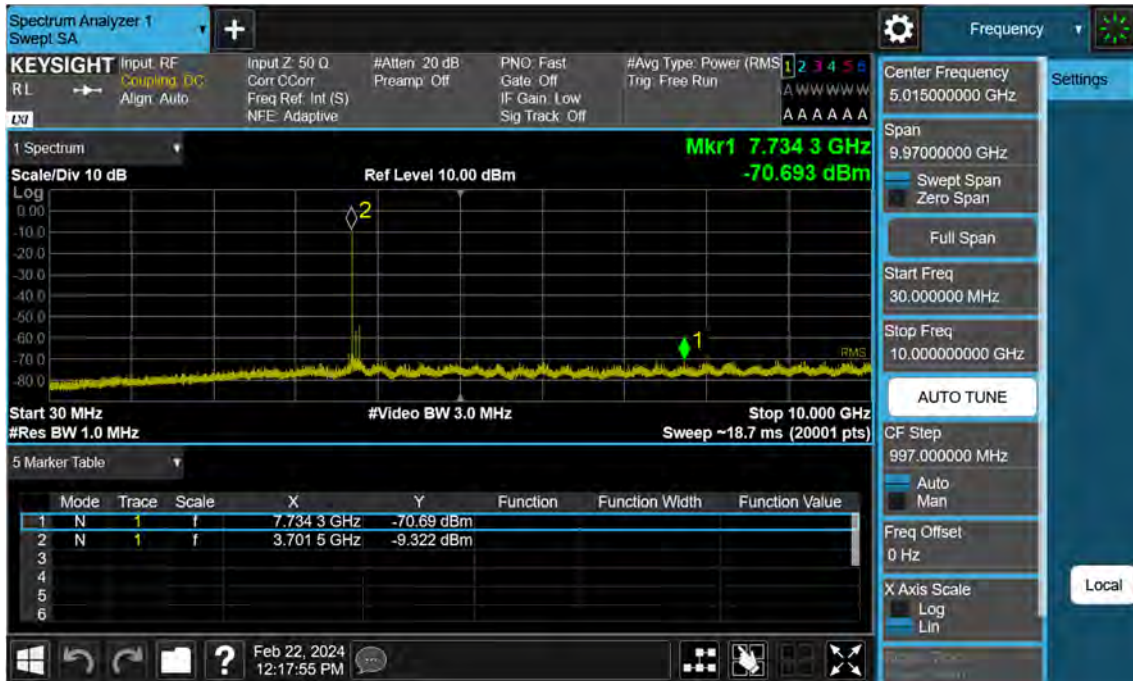
Sub6 n77. Conducted Spurious Plot_1 (649668ch_90 MHz_BPSK)
