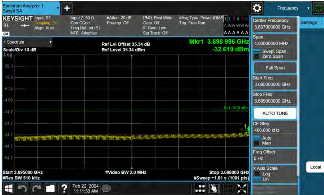
Sub6 n77. Low Band Edge Plot (40 M BW Ch.648000 BPSK FullRB)(2)
