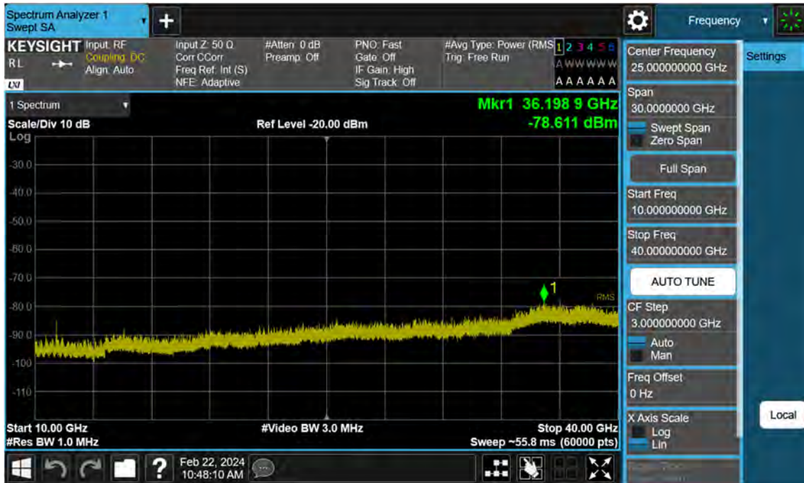
Sub6 n77. Conducted Spurious Plot_2 (647500ch_25 MHz_BPSK)
