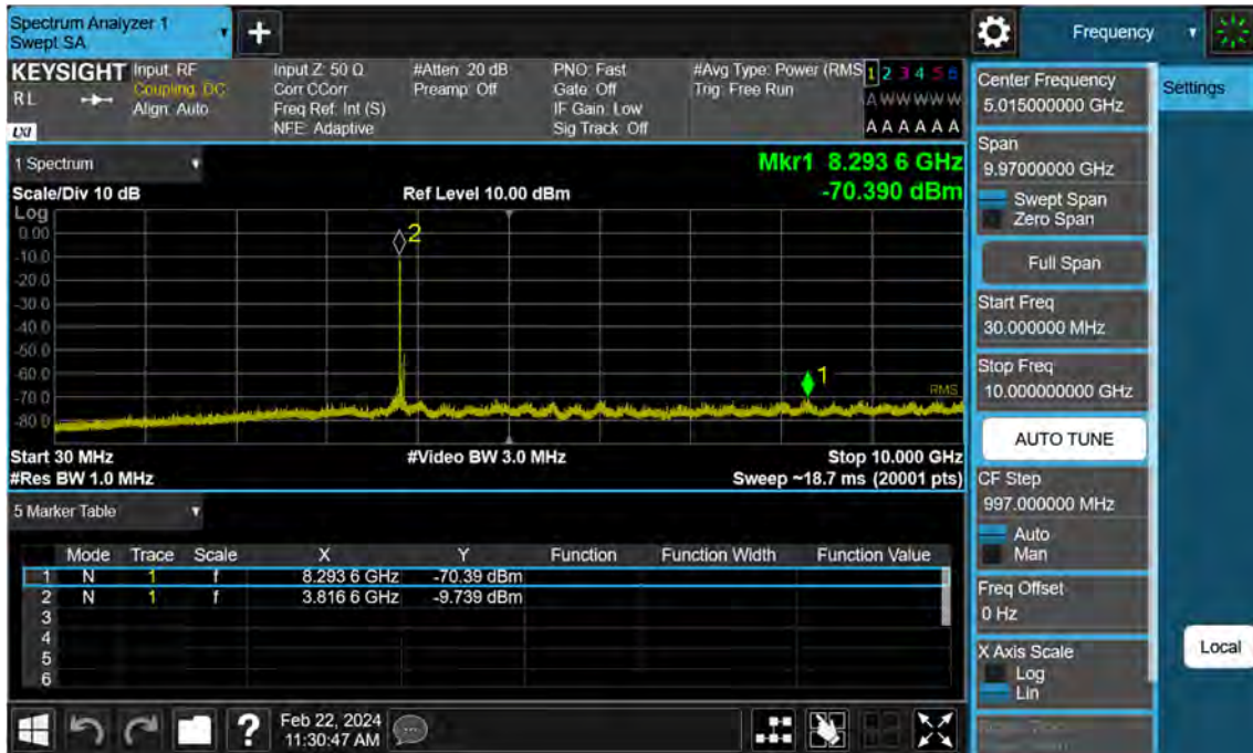
Sub6 n77. Conducted Spurious Plot_1 (656000ch_50 MHz_BPSK)
