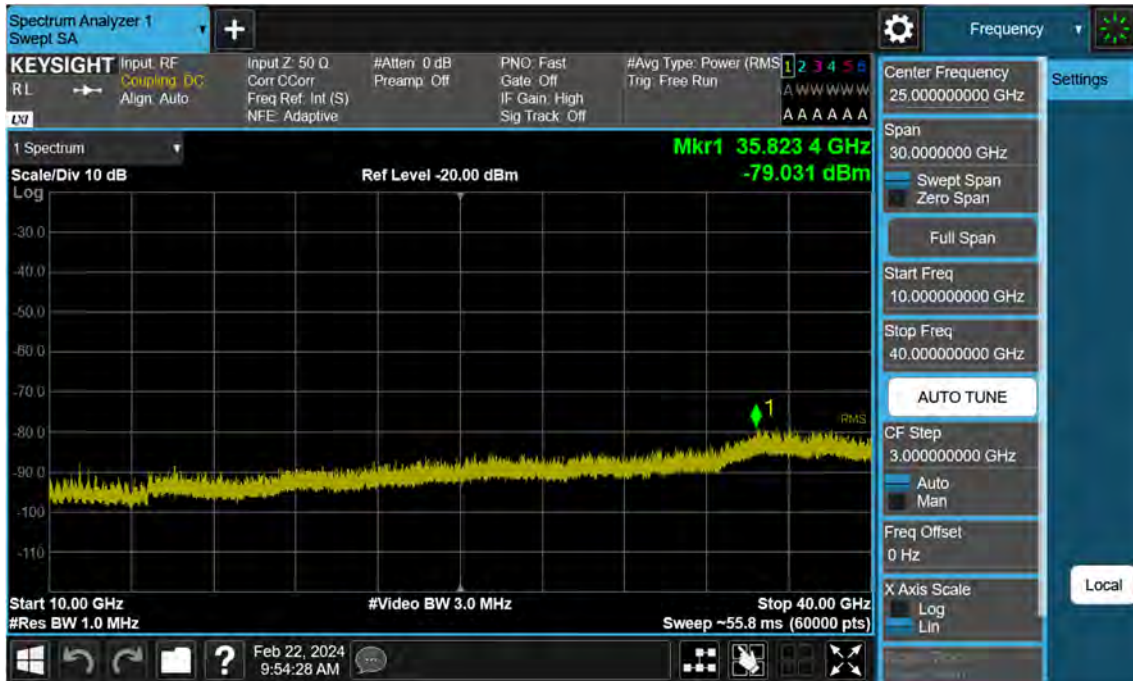
Sub6 n77. Conducted Spurious Plot_2 (647000ch_10 MHz_BPSK)
