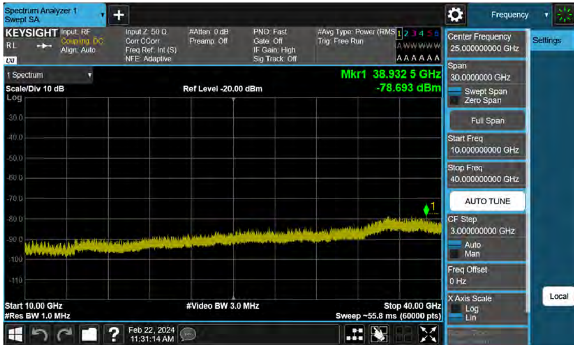
Sub6 n77. Conducted Spurious Plot_2 (656000ch_50 MHz_BPSK)
