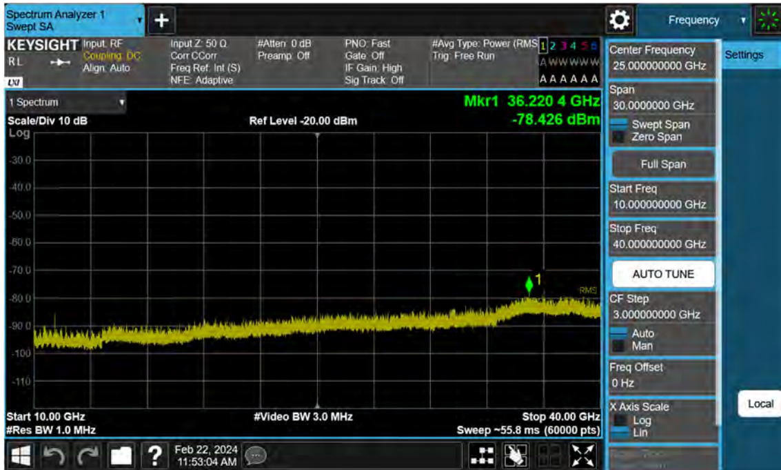
Sub6 n77. Conducted Spurious Plot_2 (649000ch_70 MHz_BPSK)
