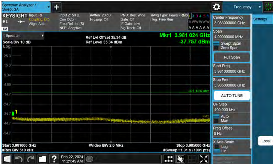
Sub6 n77. High Band Edge Plot (40 M BW Ch.664000 BPSK 1RB)(2)
