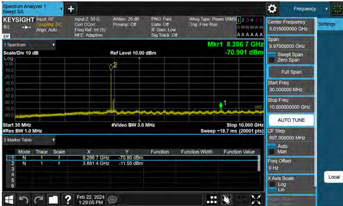
Sub6 n77. Conducted Spurious Plot_1 (662000ch_100 MHz_BPSK)
