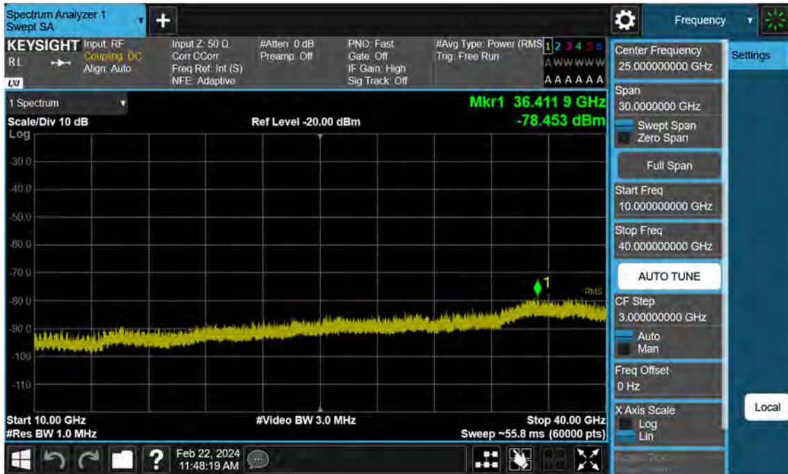
Sub6 n77. Conducted Spurious Plot_2 (663332ch_60 MHz_BPSK)
