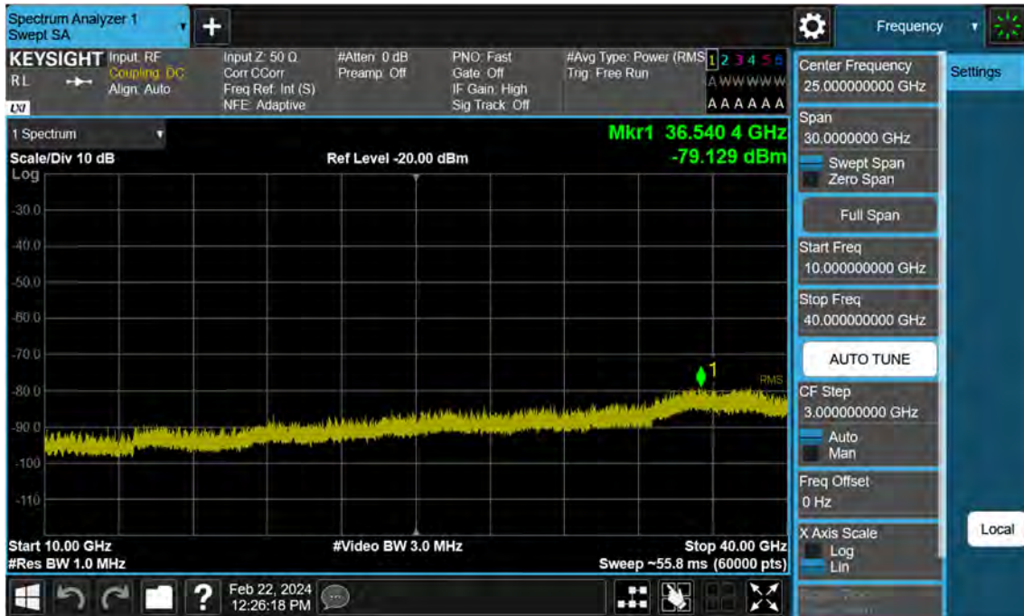
Sub6 n77. Conducted Spurious Plot_2 (662332ch_90 MHz_BPSK)
