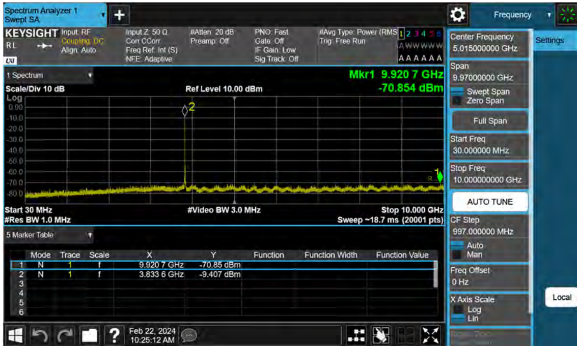
Sub6 n77. Conducted Spurious Plot_1 (656000ch_15 MHz_BPSK)
