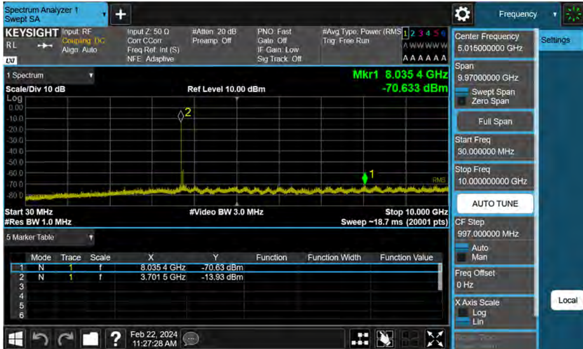
Sub6 n77. Conducted Spurious Plot_1 (648334ch_50 MHz_BPSK)
