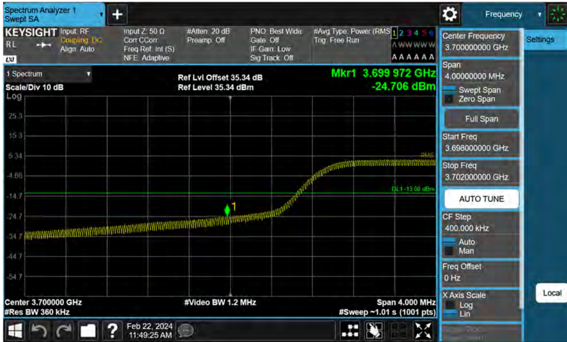
Sub6 n77. Low Band Edge Plot (70 M BW Ch.649000 BPSK FullRB)(1)
