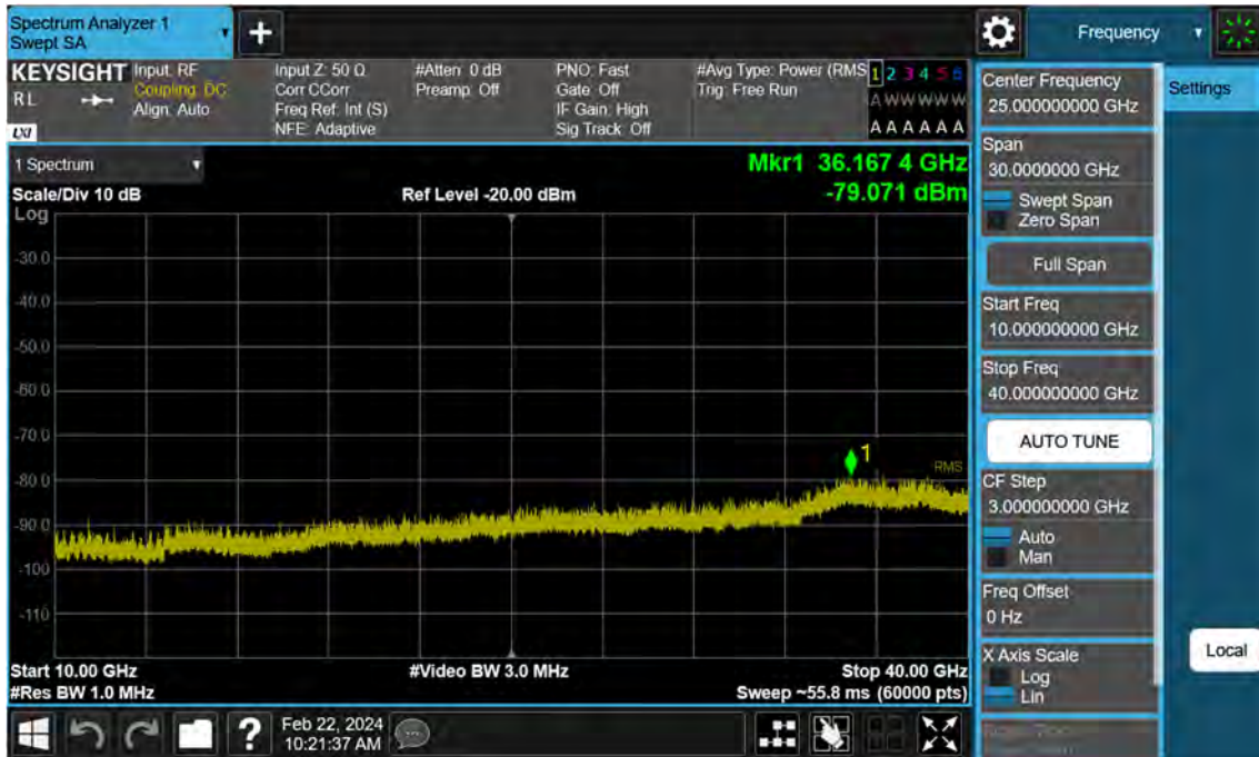
Sub6 n77. Conducted Spurious Plot_2 (647168ch_15 MHz_BPSK)
