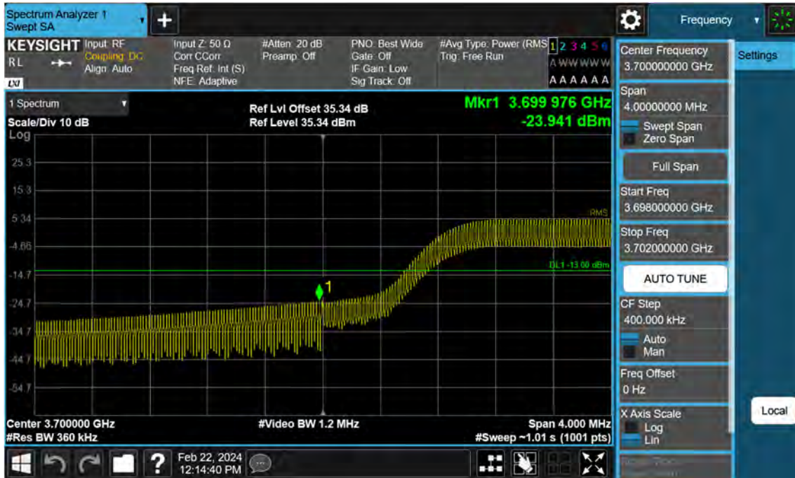
Sub6 n77. Low Band Edge Plot (90 M BW Ch.649668 BPSK FullRB)(1)
