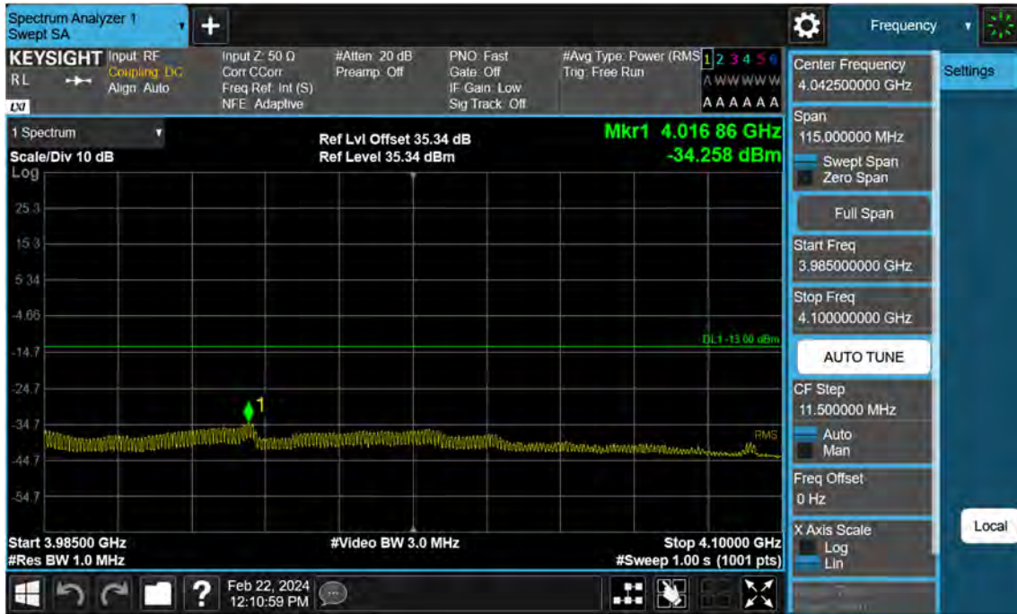
Sub6 n77. High Band Edge Plot (80 M BW Ch.662666 BPSK FullRB)(3)
