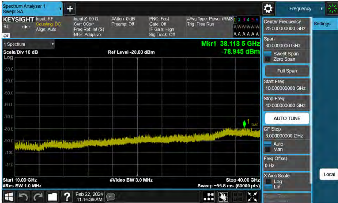
Sub6 n77. Conducted Spurious Plot_2 (648000ch_40 MHz_BPSK)
