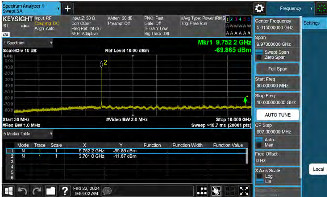
Sub6 n77. Conducted Spurious Plot_1 (647000ch_10 MHz_BPSK)
