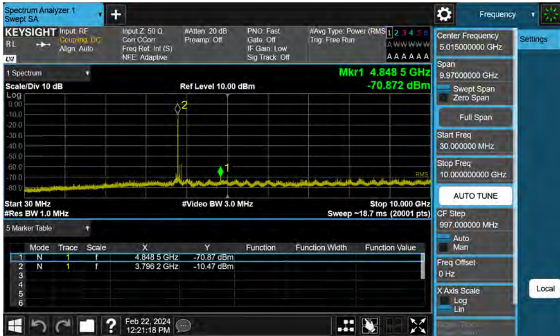
Sub6 n77. Conducted Spurious Plot_1 (656000ch_90 MHz_BPSK)
