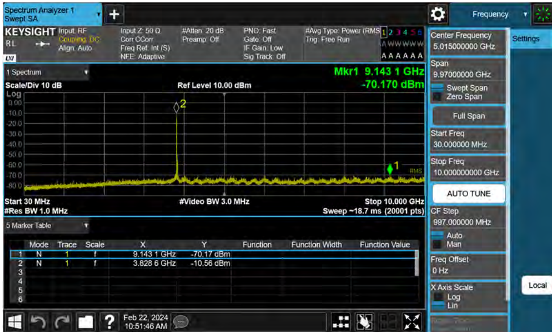
Sub6 n77. Conducted Spurious Plot_1 (656000ch_25 MHz_BPSK)
