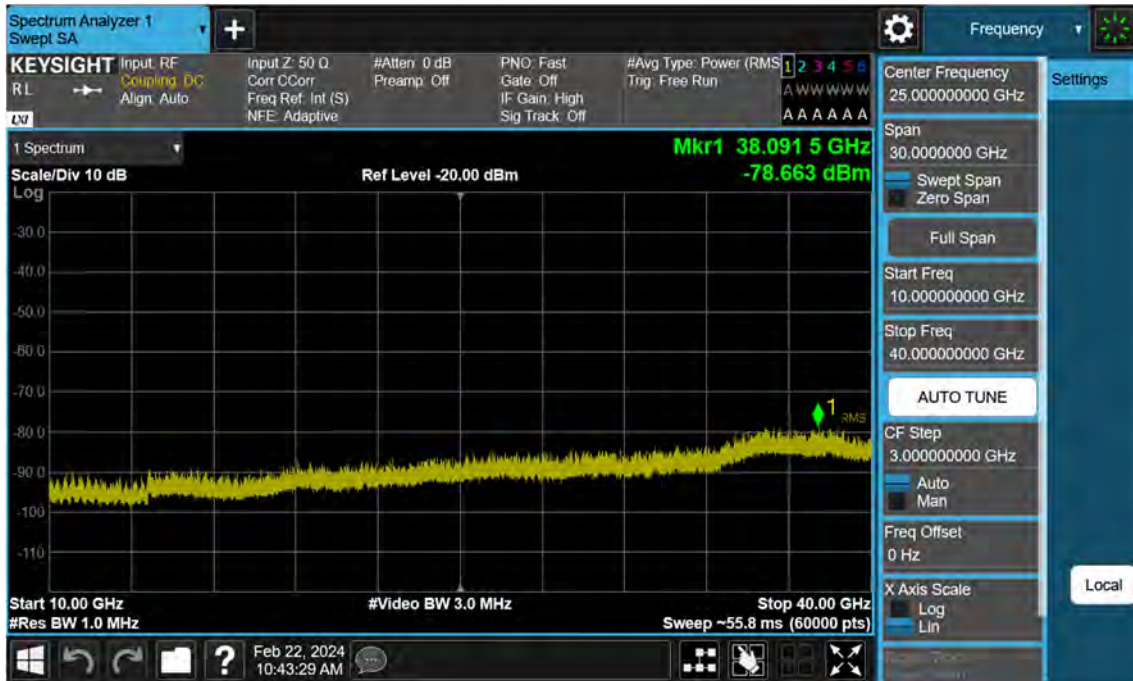
Sub6 n77. Conducted Spurious Plot_2 (664666ch_20 MHz_BPSK)
