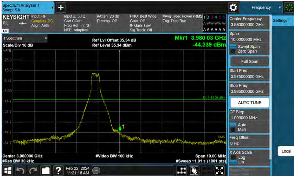
Sub6 n77. High Band Edge Plot (40 M BW Ch.664000 BPSK 1RB)(1)
