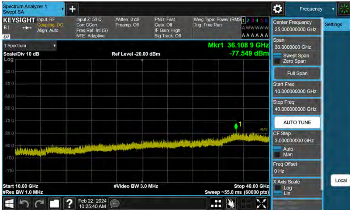
Sub6 n77. Conducted Spurious Plot_2 (656000ch_15 MHz_BPSK)
