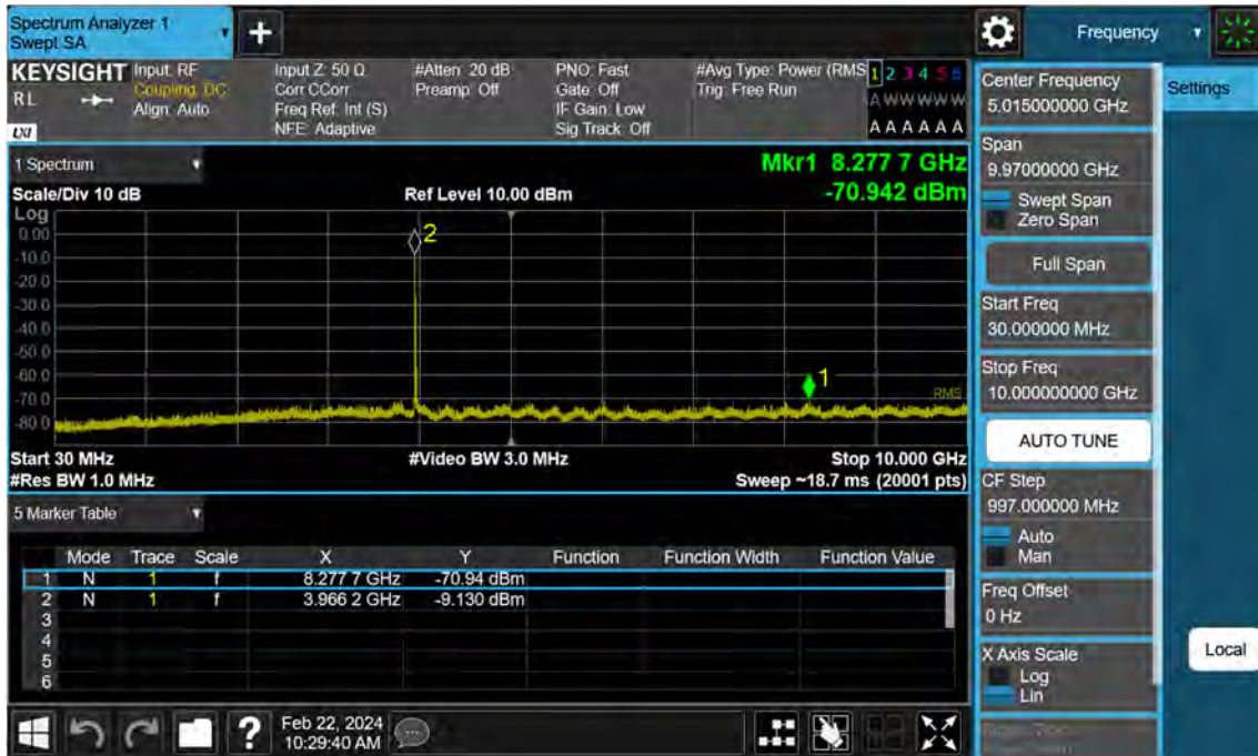
Sub6 n77. Conducted Spurious Plot_1 (664832ch_15 MHz_BPSK)
