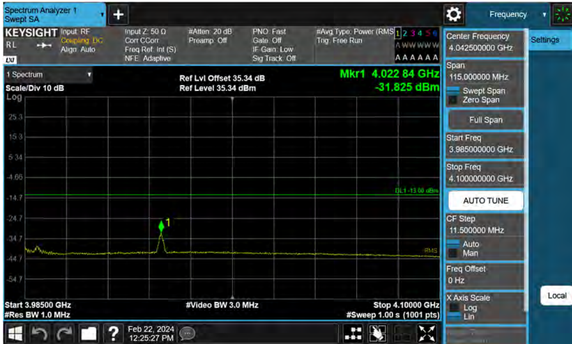
Sub6 n77. High Band Edge Plot (90 M BW Ch.662332 BPSK 1RB)(3)
