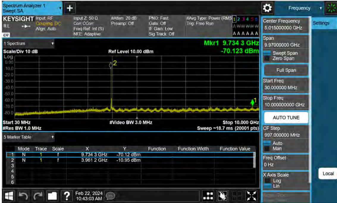
Sub6 n77. Conducted Spurious Plot_1 (664666ch_20 MHz_BPSK)
