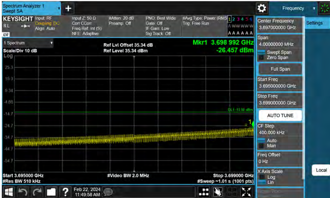
Sub6 n77. Low Band Edge Plot (70 M BW Ch.649000 BPSK FullRB)(2)
