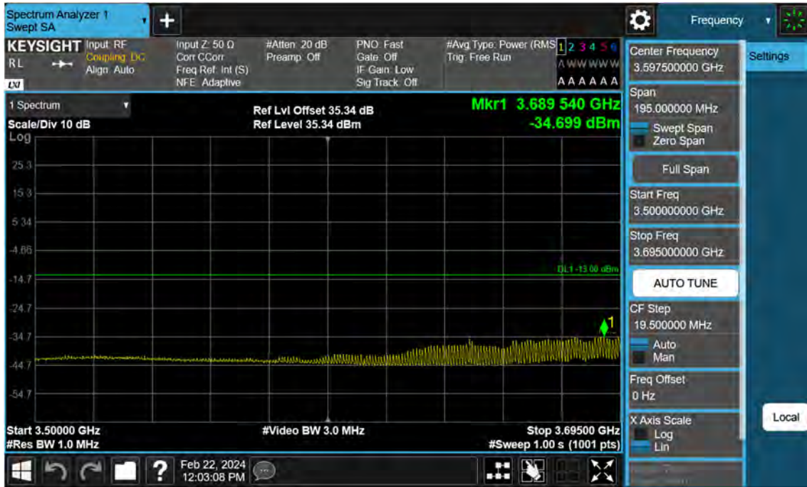
Sub6 n77. Low Band Edge Plot (80 M BW Ch.649334 BPSK FullRB)(3)
