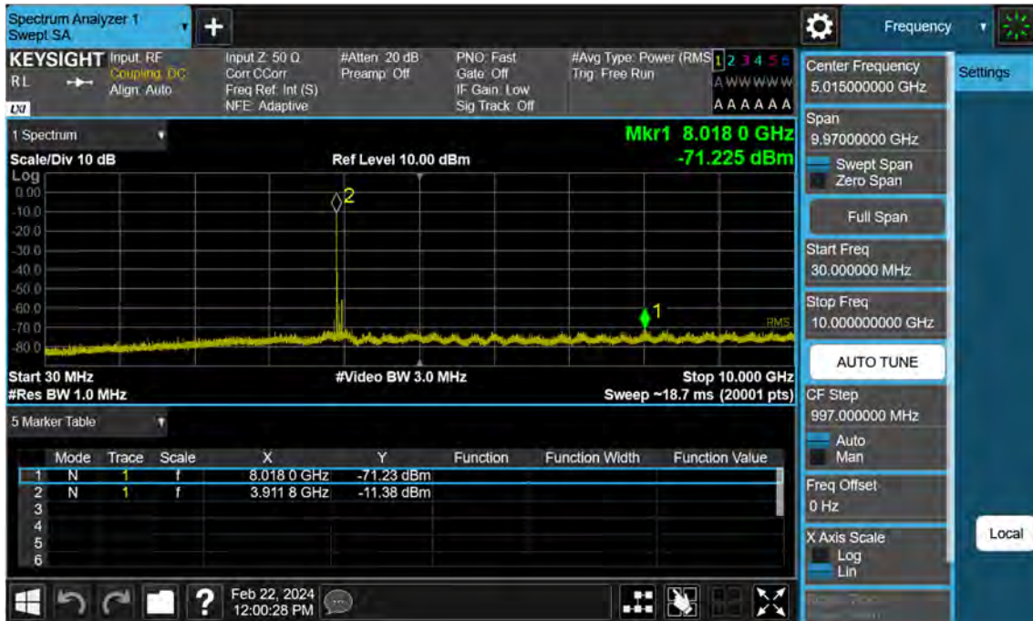
Sub6 n77. Conducted Spurious Plot_1 (663000ch_70 MHz_BPSK)
