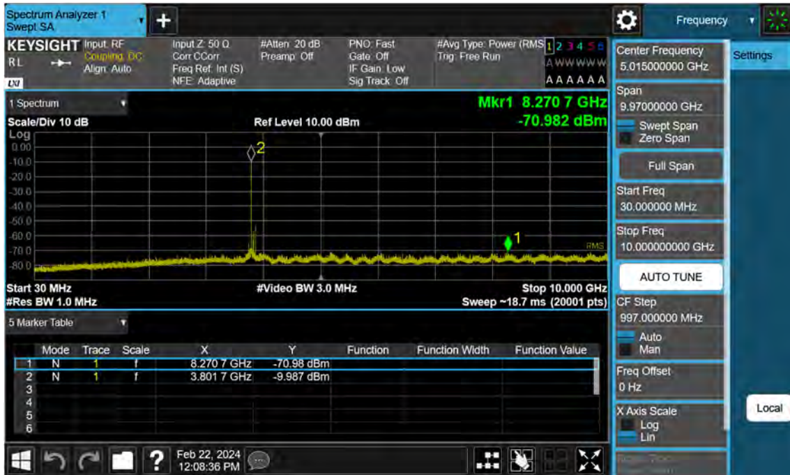
Sub6 n77. Conducted Spurious Plot_1 (656000ch_80 MHz_BPSK)
