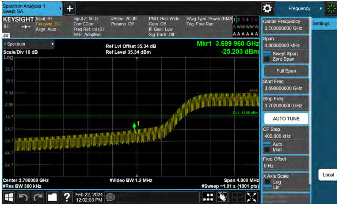
Sub6 n77. Low Band Edge Plot (80 M BW Ch.649334 BPSK FullRB)(1)
