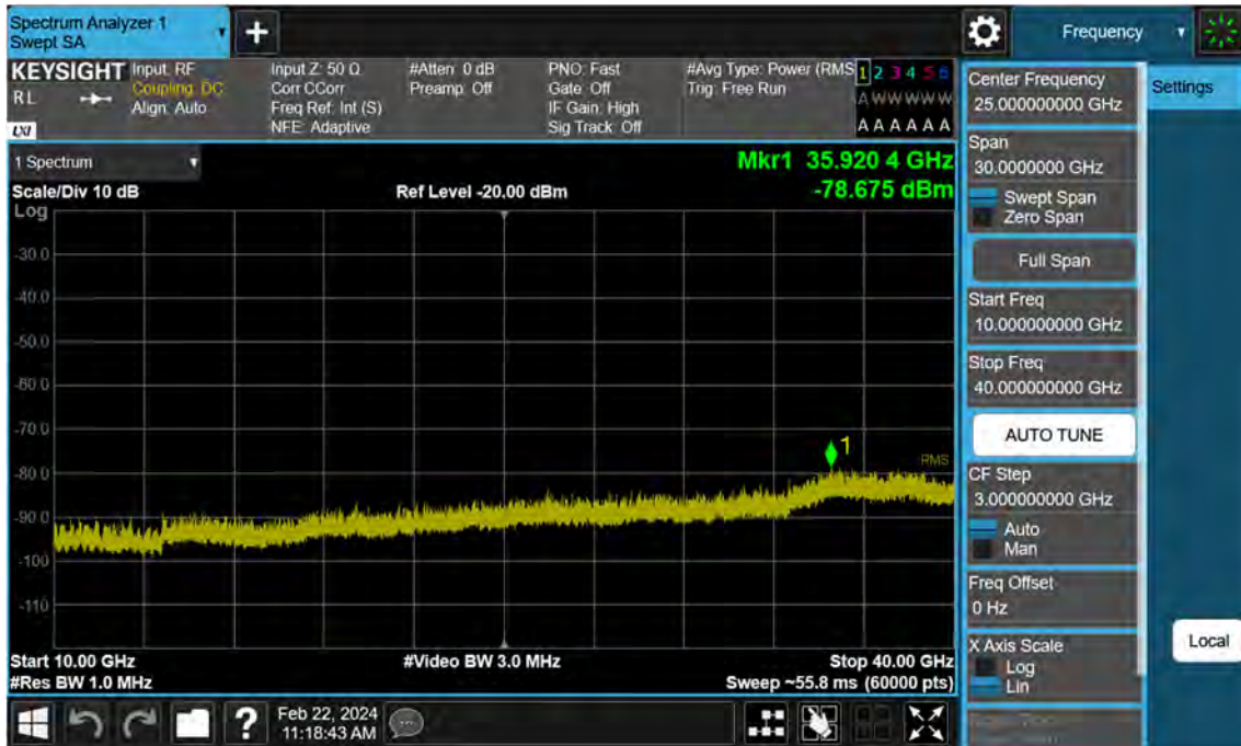
Sub6 n77. Conducted Spurious Plot_2 (656000ch_40 MHz_BPSK)
