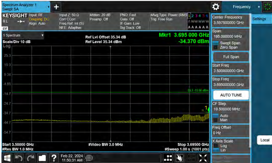
Sub6 n77. Low Band Edge Plot (70 M BW Ch.649000 BPSK FullRB)(3)
