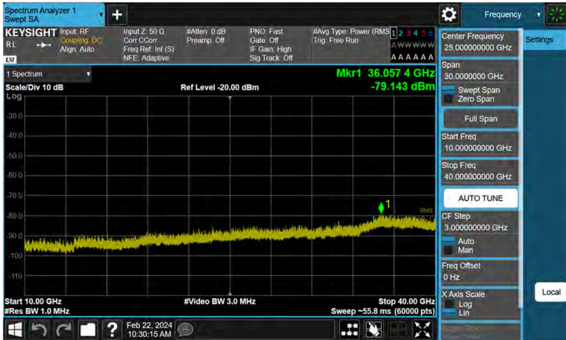
Sub6 n77. Conducted Spurious Plot_2 (664832ch_15 MHz_BPSK)
