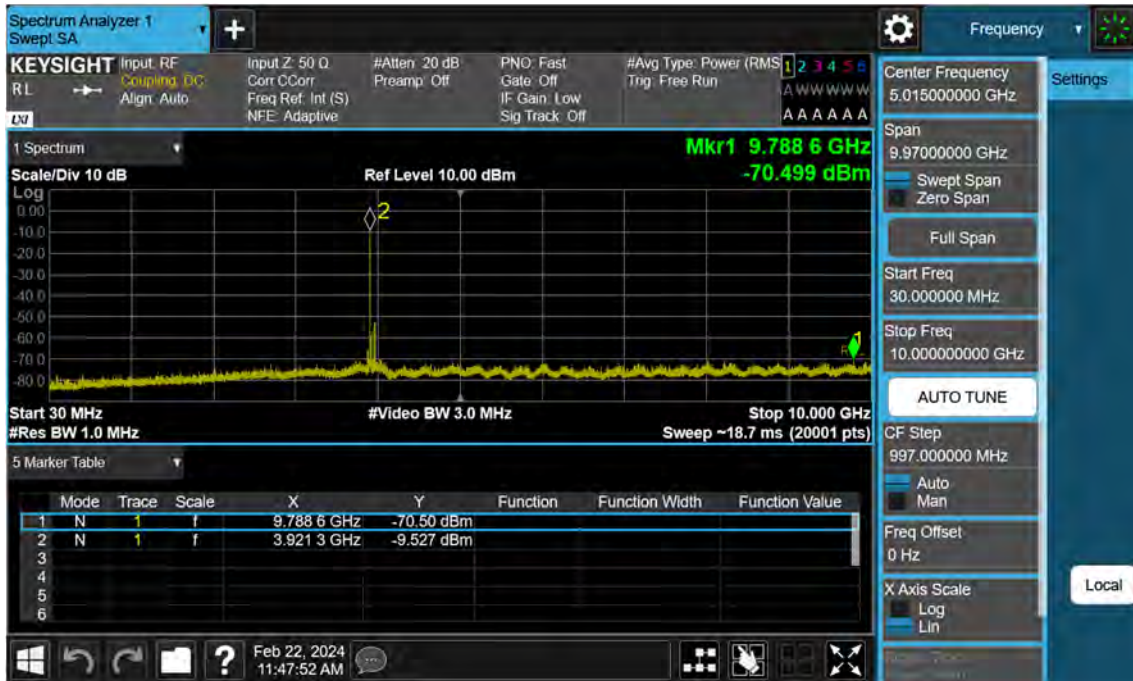
Sub6 n77. Conducted Spurious Plot_1 (663332ch_60 MHz_BPSK)
