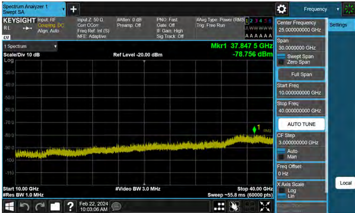
Sub6 n77. Conducted Spurious Plot_2 (665000ch_10 MHz_BPSK)
