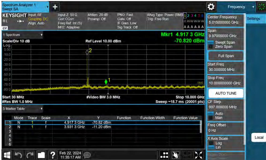
Sub6 n77. Conducted Spurious Plot_1 (663666ch_50 MHz_BPSK)
