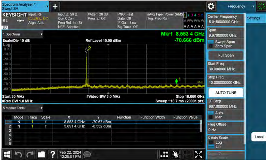
Sub6 n77. Conducted Spurious Plot_1 (662332ch_90 MHz_BPSK)
