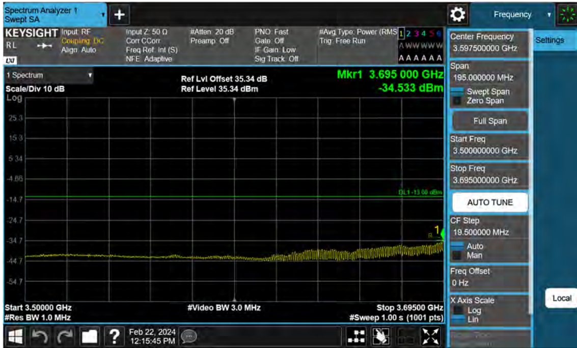
Sub6 n77. Low Band Edge Plot (90 M BW Ch.649668 BPSK FullRB)(3)
