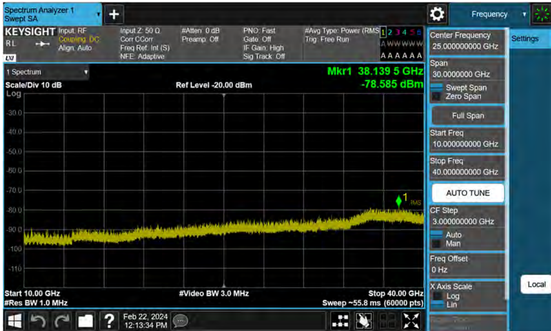
Sub6 n77. Conducted Spurious Plot_2 (662666ch_80 MHz_BPSK)
