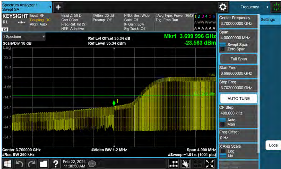
Sub6 n77. Low Band Edge Plot (60 M BW Ch.648668 BPSK FullRB)(1)
