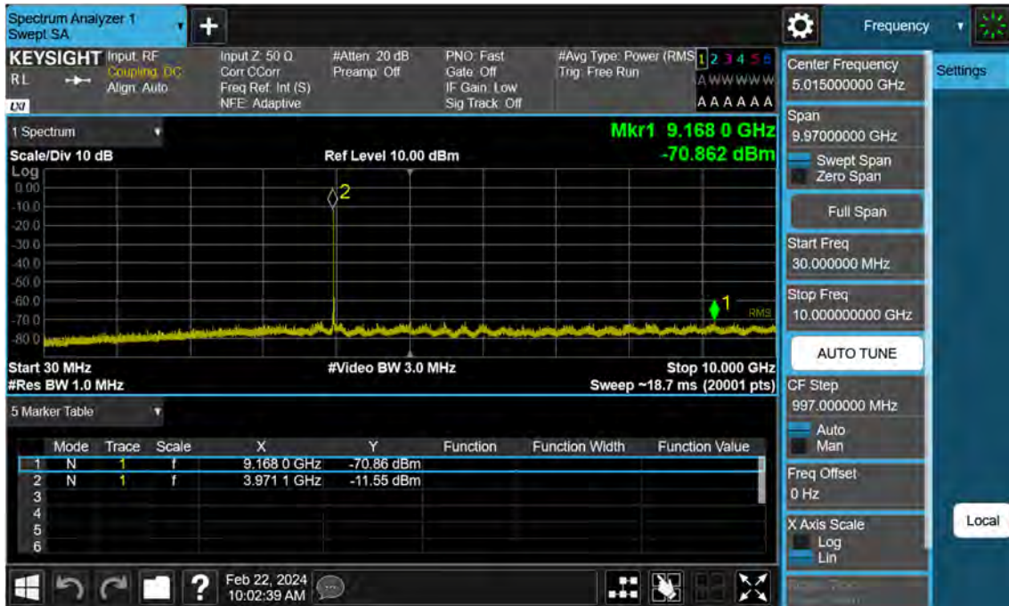
Sub6 n77. Conducted Spurious Plot_1 (665000ch_10 MHz_BPSK)
