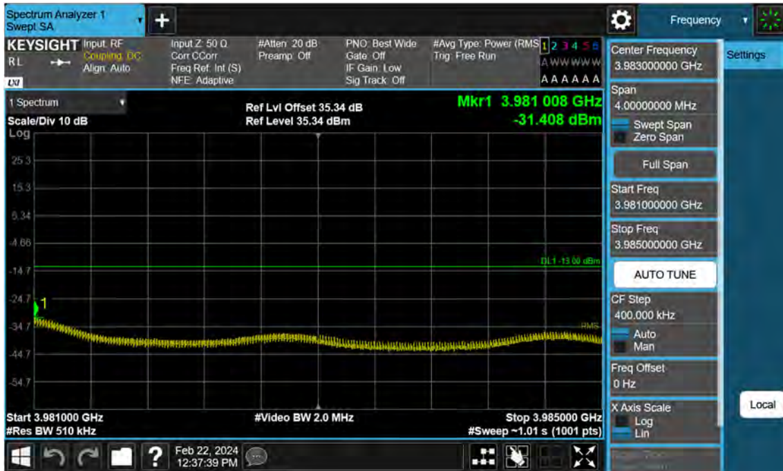
Sub6 n77. High Band Edge Plot (100 M BW Ch.662000 BPSK 1RB)(2)
