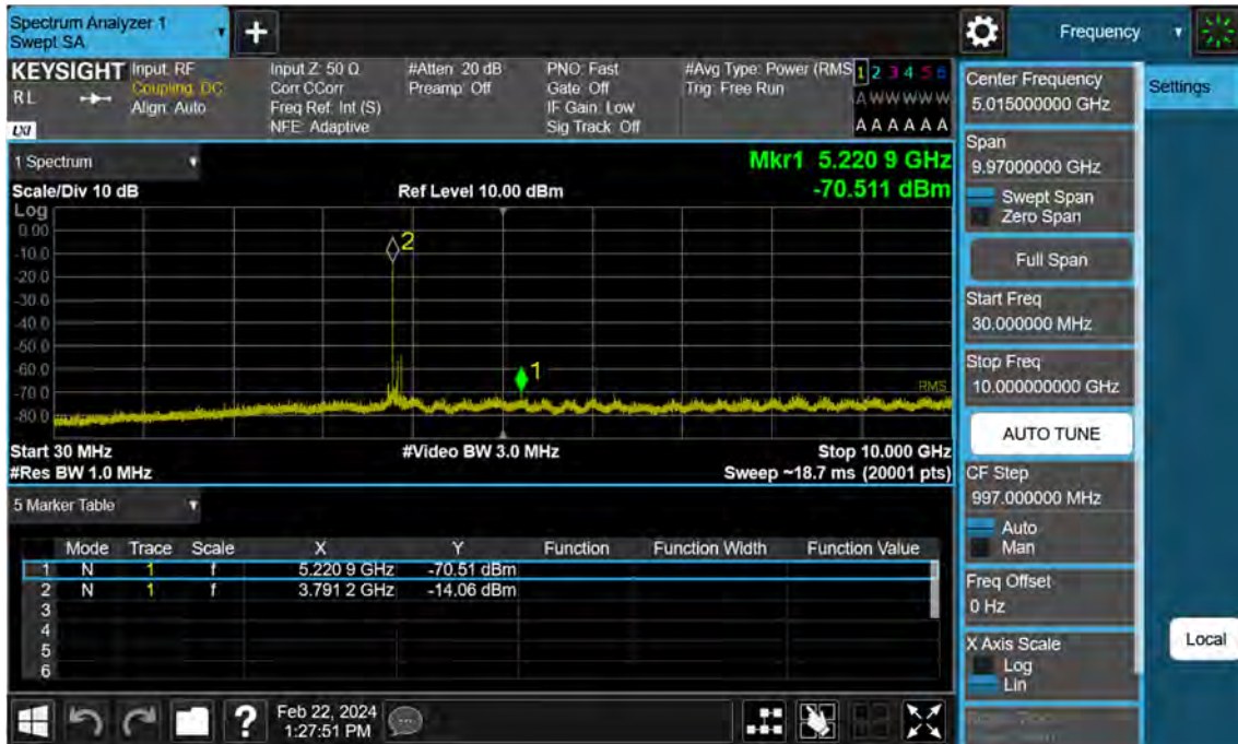
Sub6 n77. Conducted Spurious Plot_1 (656000ch_100 MHz_BPSK)
