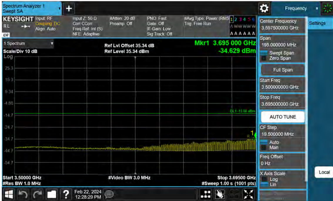
Sub6 n77. Low Band Edge Plot (100 M BW Ch.650000 BPSK FullRB)(3)
