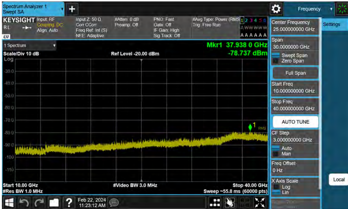
Sub6 n77. Conducted Spurious Plot_2 (664000ch_40 MHz_BPSK)
