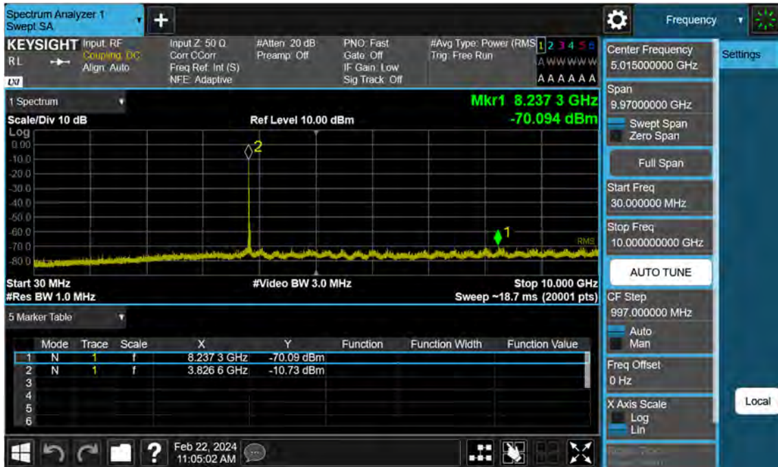
Sub6 n77. Conducted Spurious Plot_1 (656000ch_30 MHz_BPSK)
