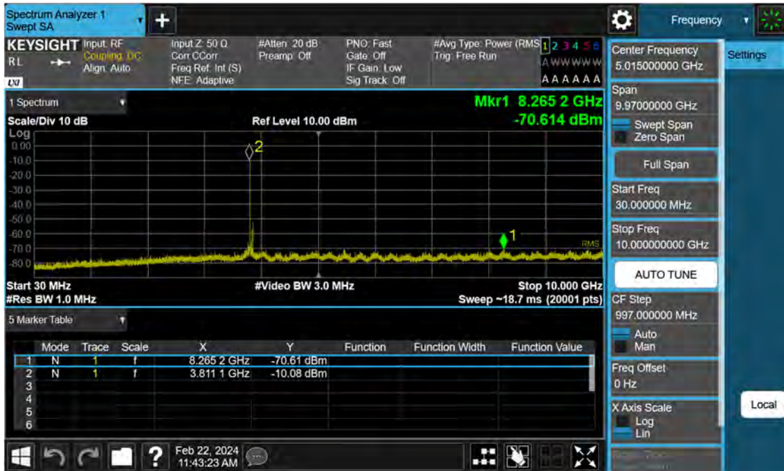
Sub6 n77. Conducted Spurious Plot_1 (656000ch_60 MHz_BPSK)
