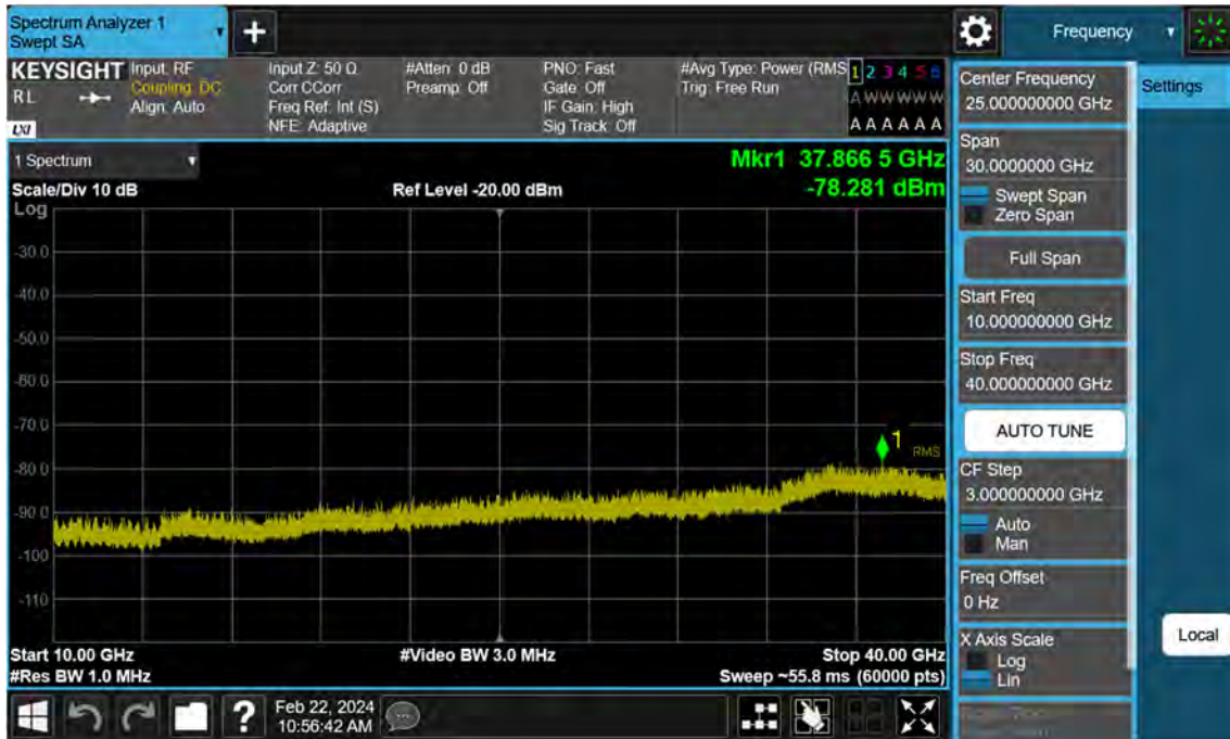
Sub6 n77. Conducted Spurious Plot_2 (664500ch_25 MHz_BPSK)
