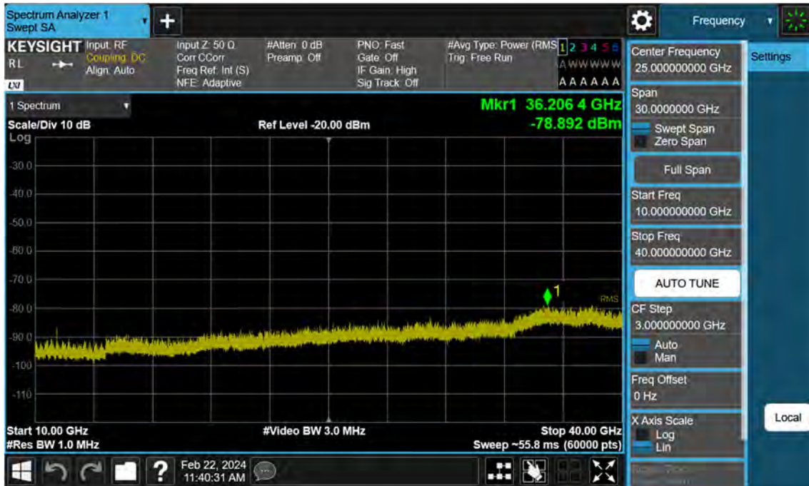
Sub6 n77. Conducted Spurious Plot_2 (648668ch_60 MHz_BPSK)
