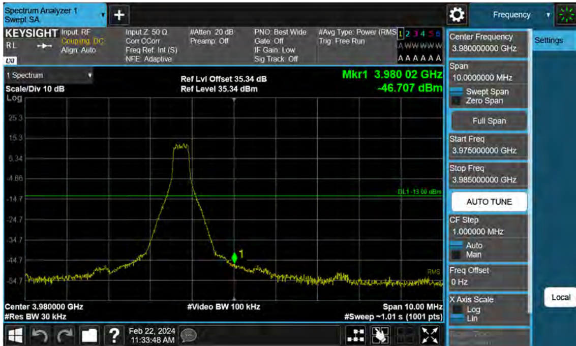
Sub6 n77. High Band Edge Plot (50 M BW Ch.663666 BPSK 1RB)(1)
