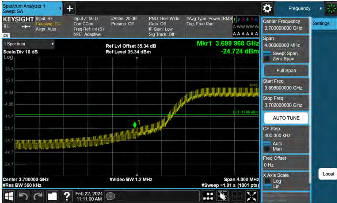
Sub6 n77. Low Band Edge Plot (40 M BW Ch.648000 BPSK FullRB)(1)
