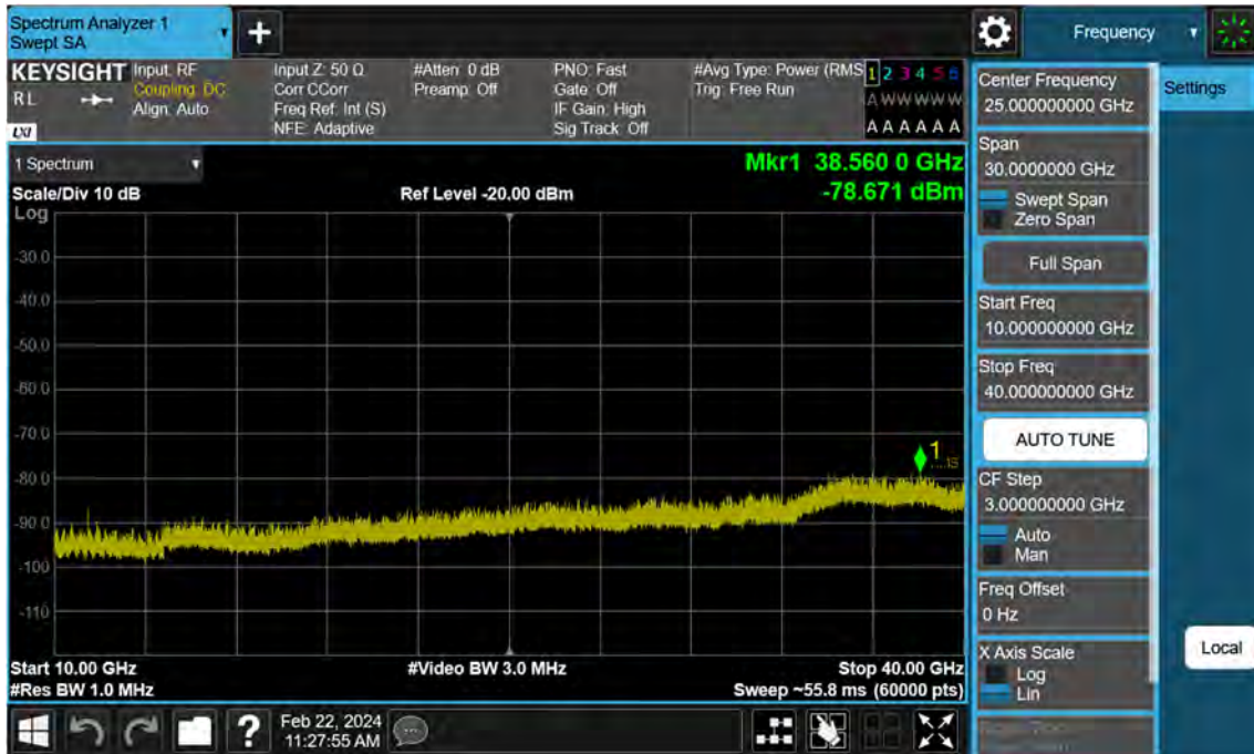
Sub6 n77. Conducted Spurious Plot_2 (648334ch_50 MHz_BPSK)
