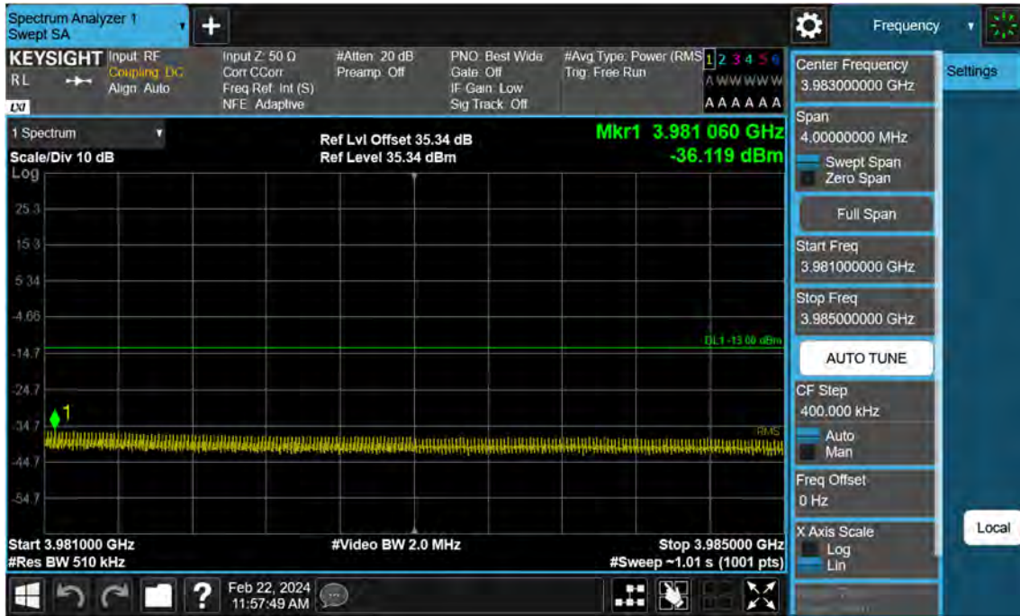
Sub6 n77. High Band Edge Plot (70 M BW Ch.663000 BPSK FullRB)(2)
