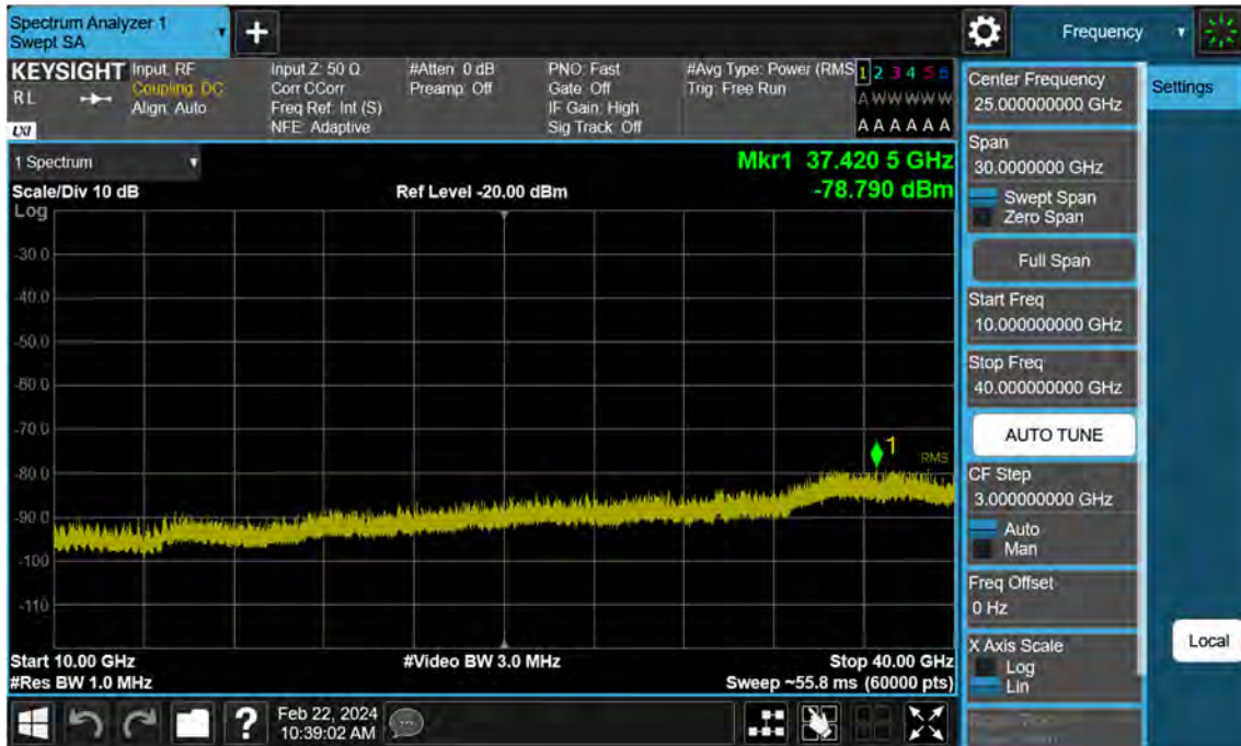
Sub6 n77. Conducted Spurious Plot_2 (656000ch_20 MHz_BPSK)
