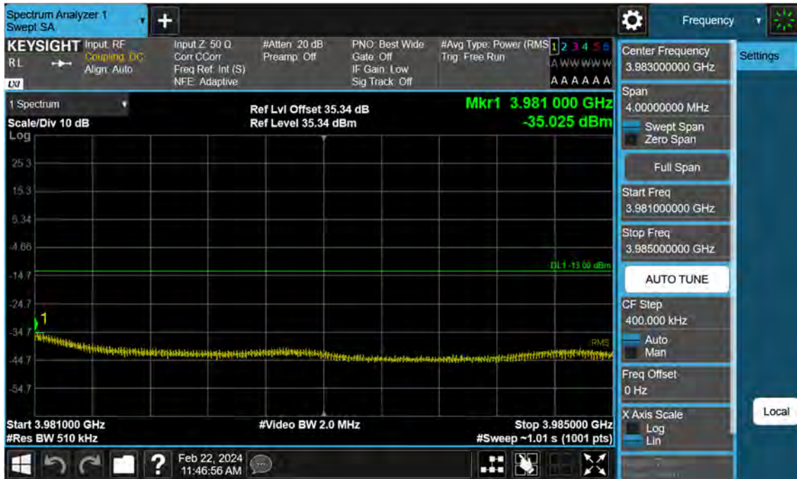
Sub6 n77. High Band Edge Plot (60 M BW Ch.663332 BPSK 1RB)(2)
