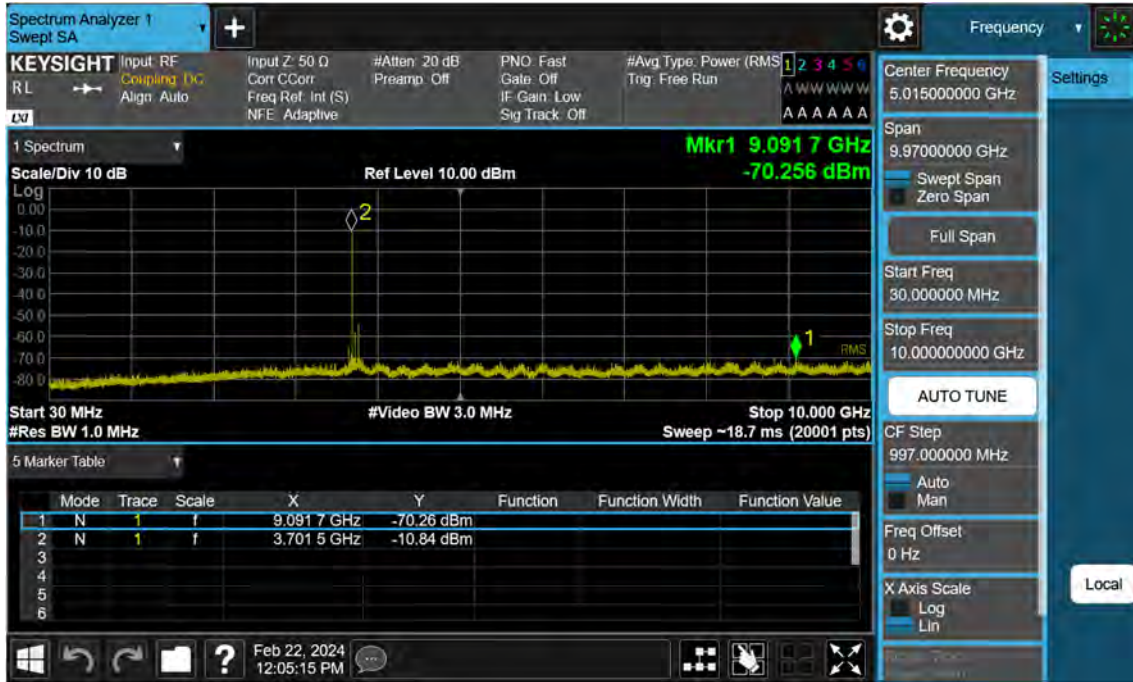
Sub6 n77. Conducted Spurious Plot_1 (649334ch_80 MHz_BPSK)
