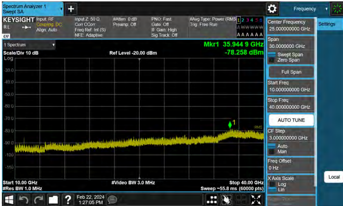
Sub6 n77. Conducted Spurious Plot_2 (650000ch_100 MHz_BPSK)
