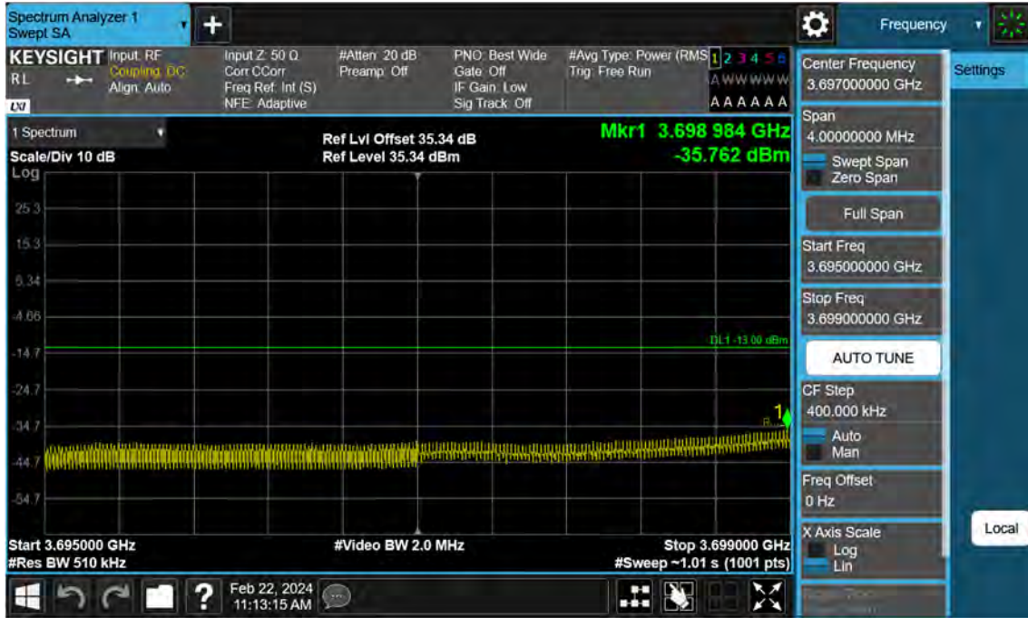
Sub6 n77. Low Band Edge Plot (40 M BW Ch.648000 BPSK 1RB)(2)
