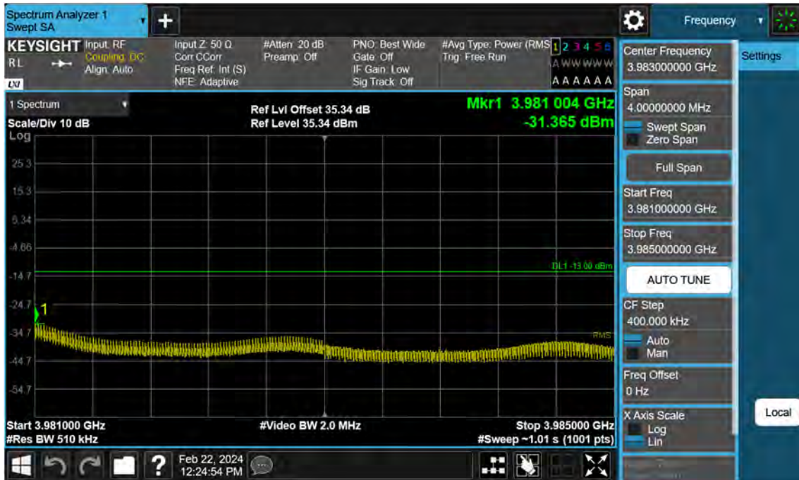
Sub6 n77. High Band Edge Plot (90 M BW Ch.662332 BPSK 1RB)(2)
