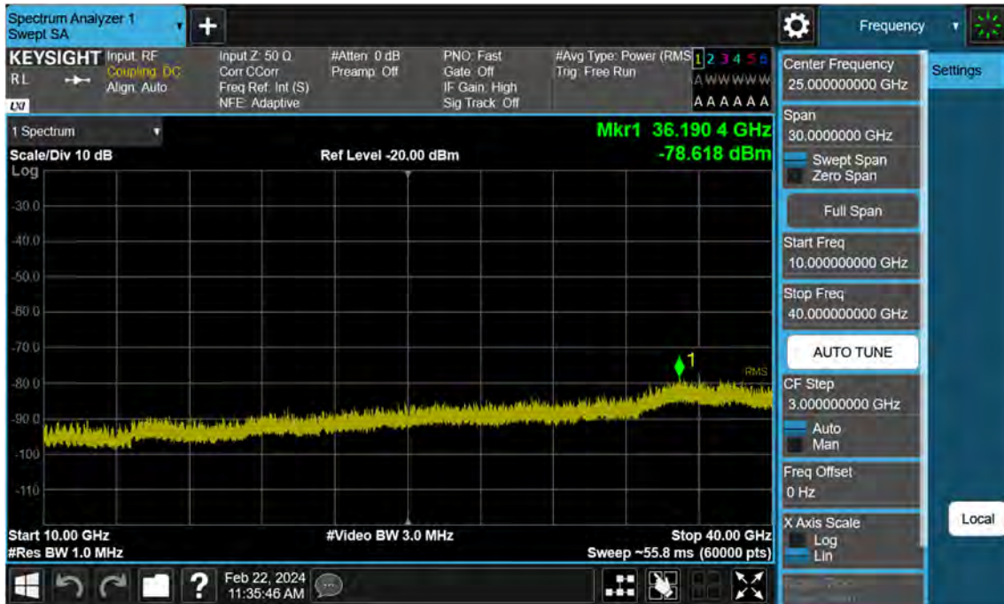
Sub6 n77. Conducted Spurious Plot_2 (663666ch_50 MHz_BPSK)
