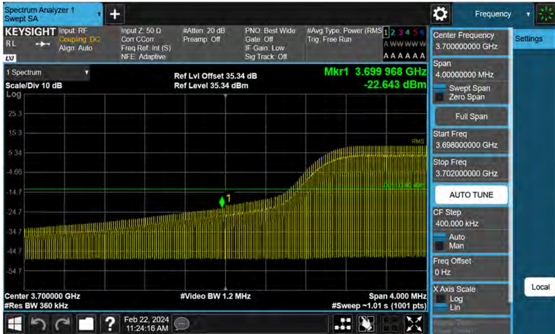
Sub6 n77. Low Band Edge Plot (50 M BW Ch.648334 BPSK FullRB)(1)
