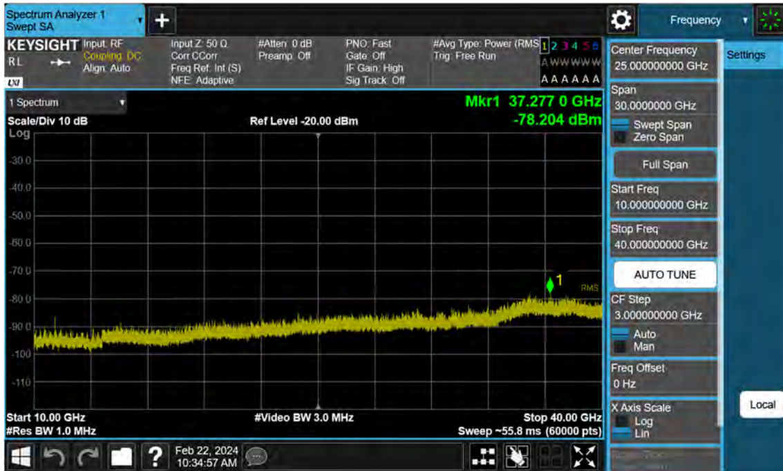
Sub6 n77. Conducted Spurious Plot_2 (647334ch_20 MHz_BPSK)
