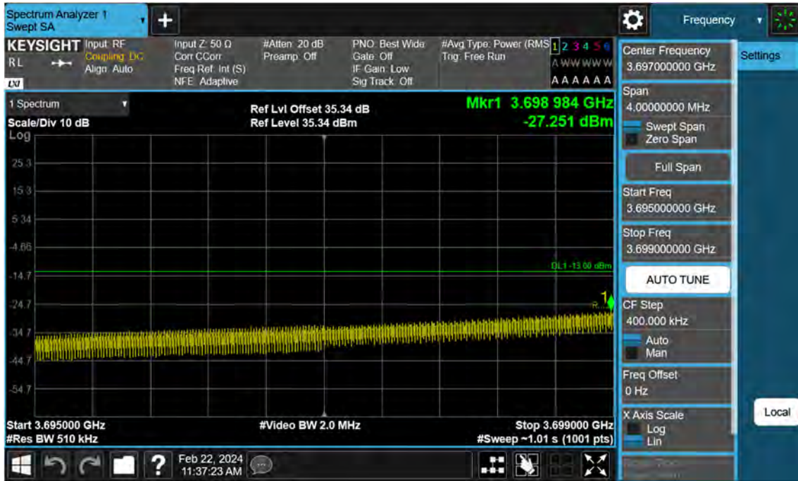
Sub6 n77. Low Band Edge Plot (60 M BW Ch.648668 BPSK FullRB)(2)
