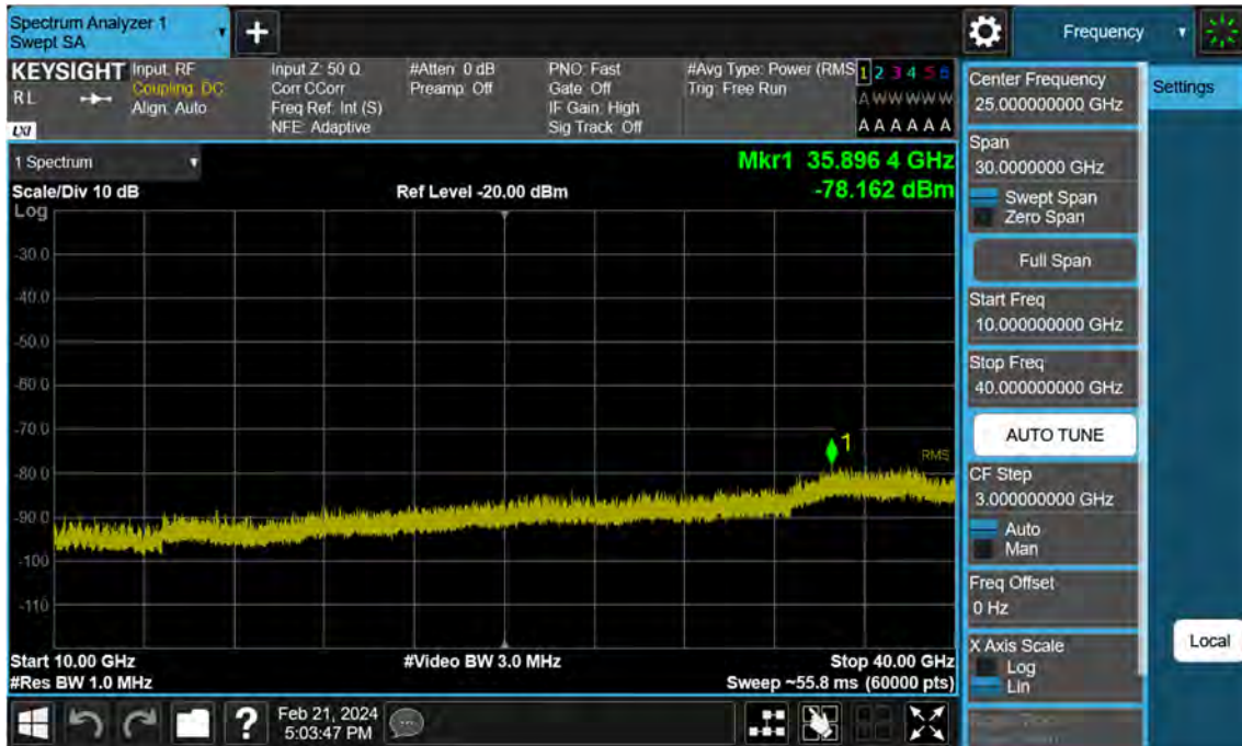
Sub6 n77. Conducted Spurious Plot_2 (631000ch_30 MHz_BPSK)
