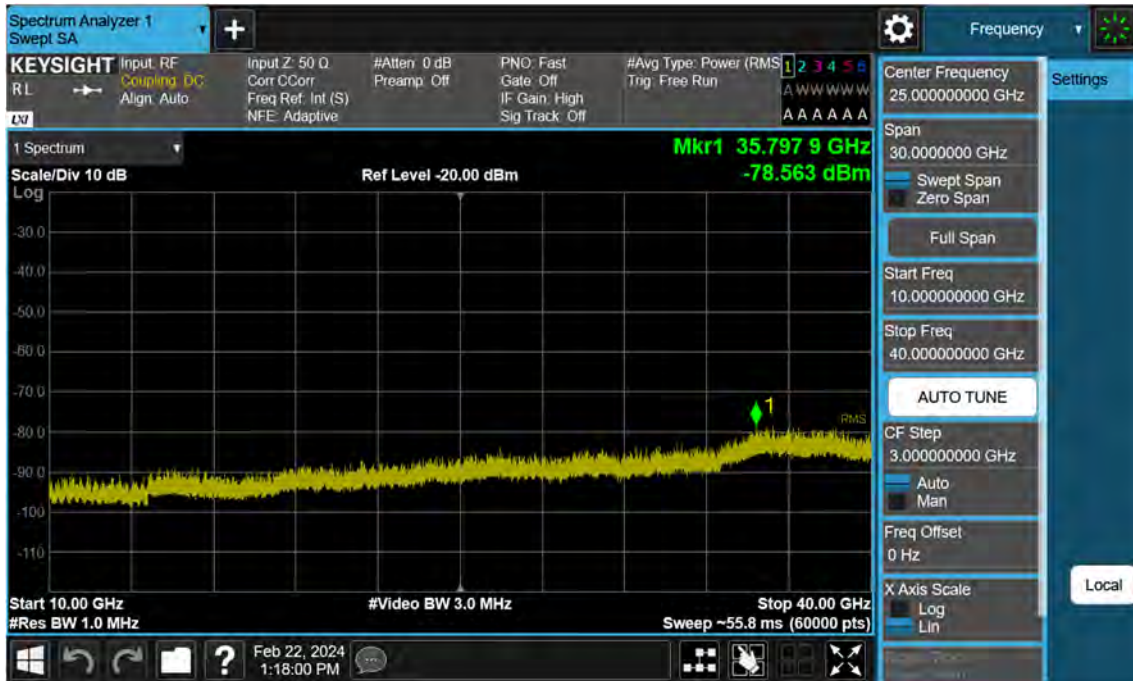
Sub6 n77. Conducted Spurious Plot_2 (633334ch_25 MHz_BPSK)
