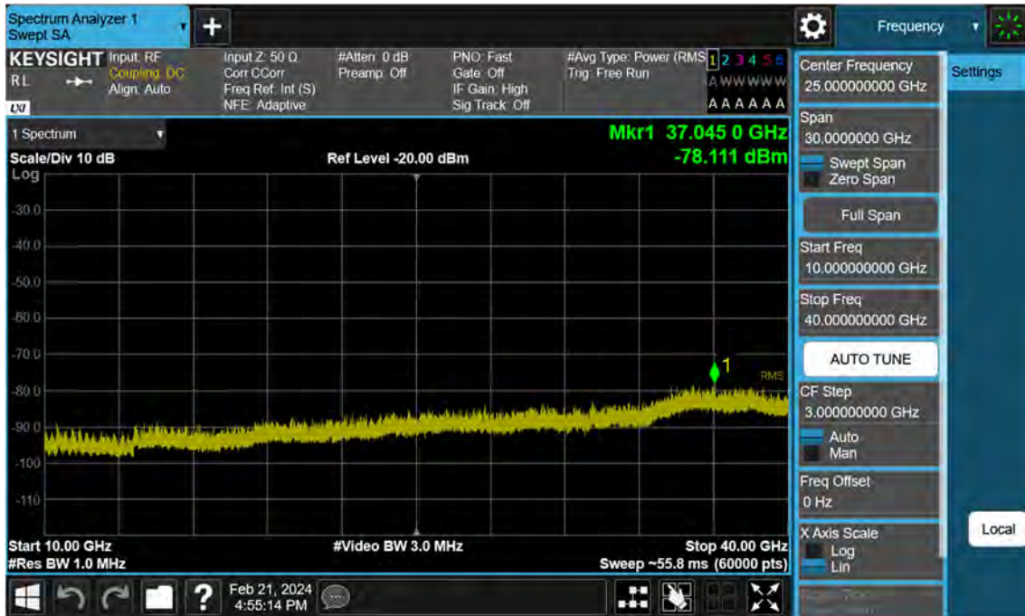
Sub6 n77. Conducted Spurious Plot_2 (633334ch_20 MHz_BPSK)
