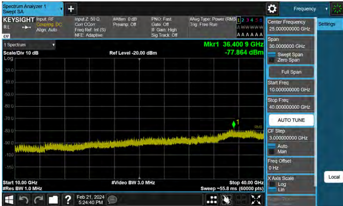
Sub6 n77. Conducted Spurious Plot_2 (635332ch_40 MHz_BPSK)
