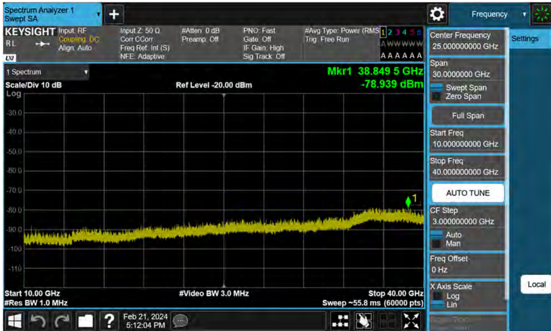
Sub6 n77. Conducted Spurious Plot_2 (635666ch_30 MHz_BPSK)
