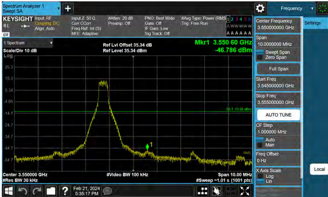
Sub6 n77. High Band Edge Plot (50 M BW Ch.635000 BPSK 1RB)(1)
