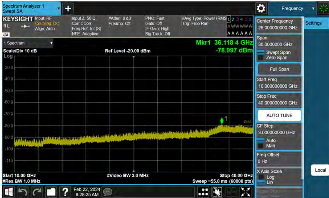
Sub6 n77. Conducted Spurious Plot_2 (632000ch_60 MHz_BPSK)
