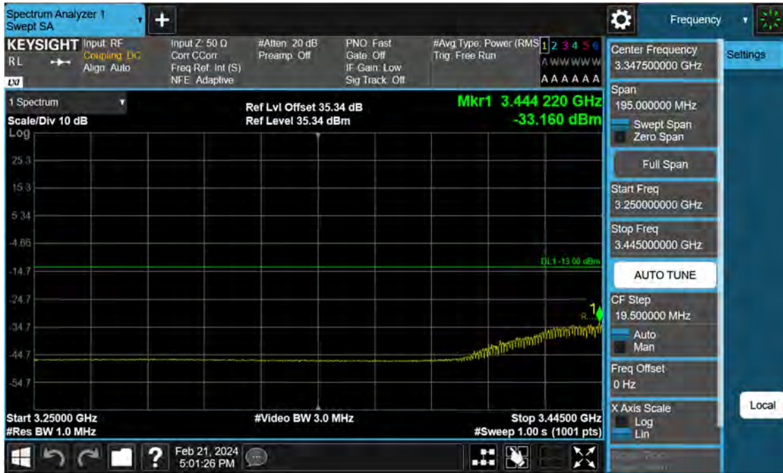
Sub6 n77. Low Band Edge Plot (30 M BW Ch.631000 BPSK FullRB)(3)
