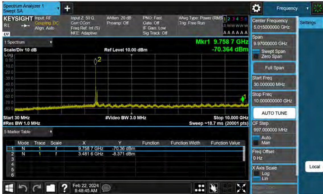
Sub6 n77. Conducted Spurious Plot_1 (634332ch_70 MHz_BPSK)
