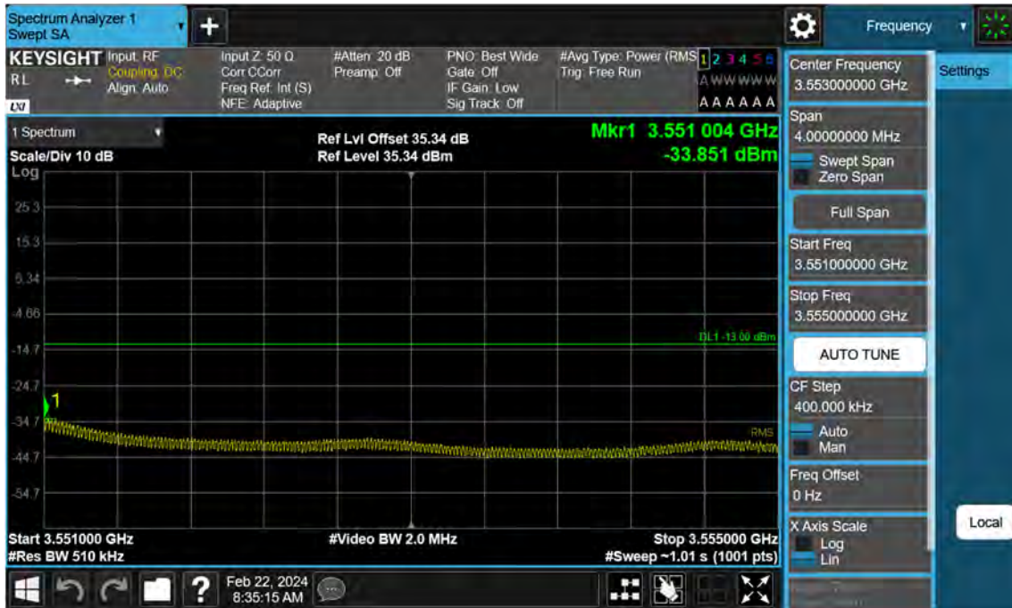
Sub6 n77. High Band Edge Plot (60 M BW Ch.634666 BPSK 1RB)(2)
