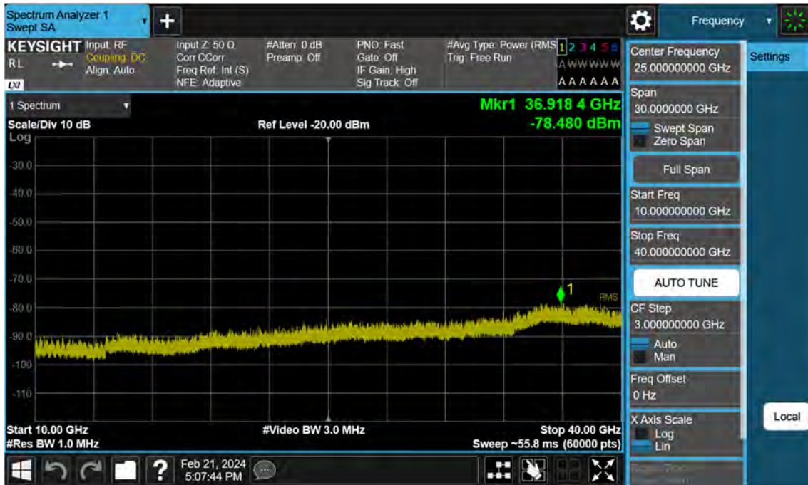
Sub6 n77. Conducted Spurious Plot_2 (633334ch_30 MHz_BPSK)
