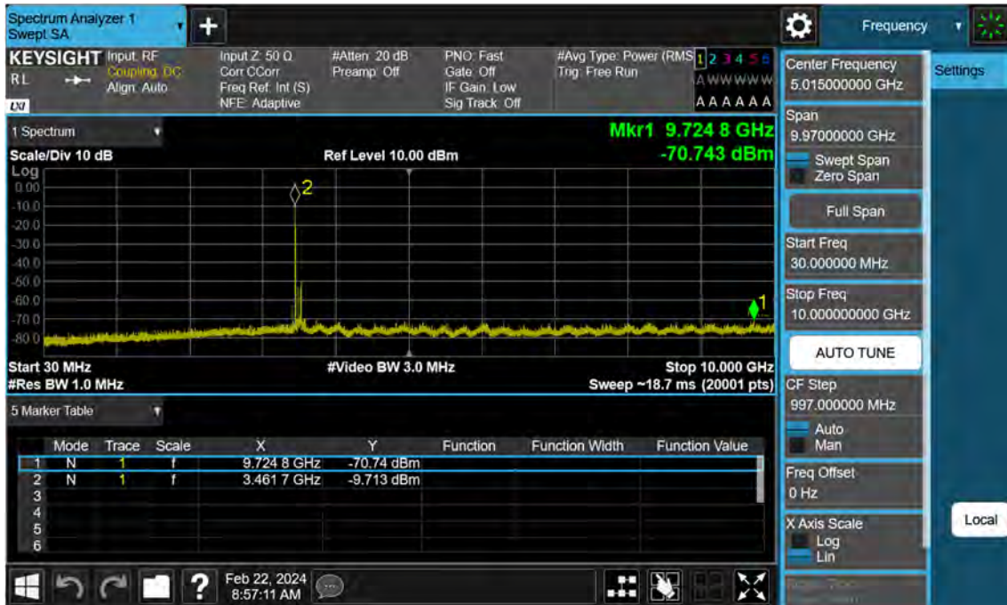
Sub6 n77. Conducted Spurious Plot_1 (633334ch_80 MHz_BPSK)
