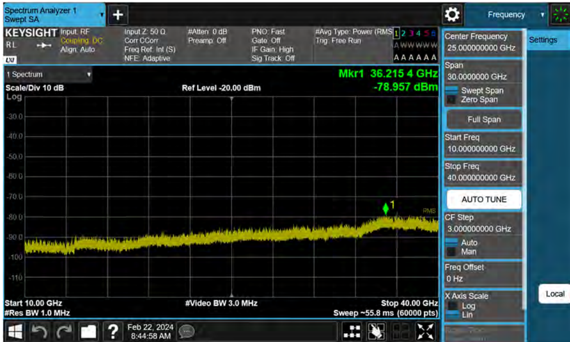
Sub6 n77. Conducted Spurious Plot_2 (633334ch_70 MHz_BPSK)
