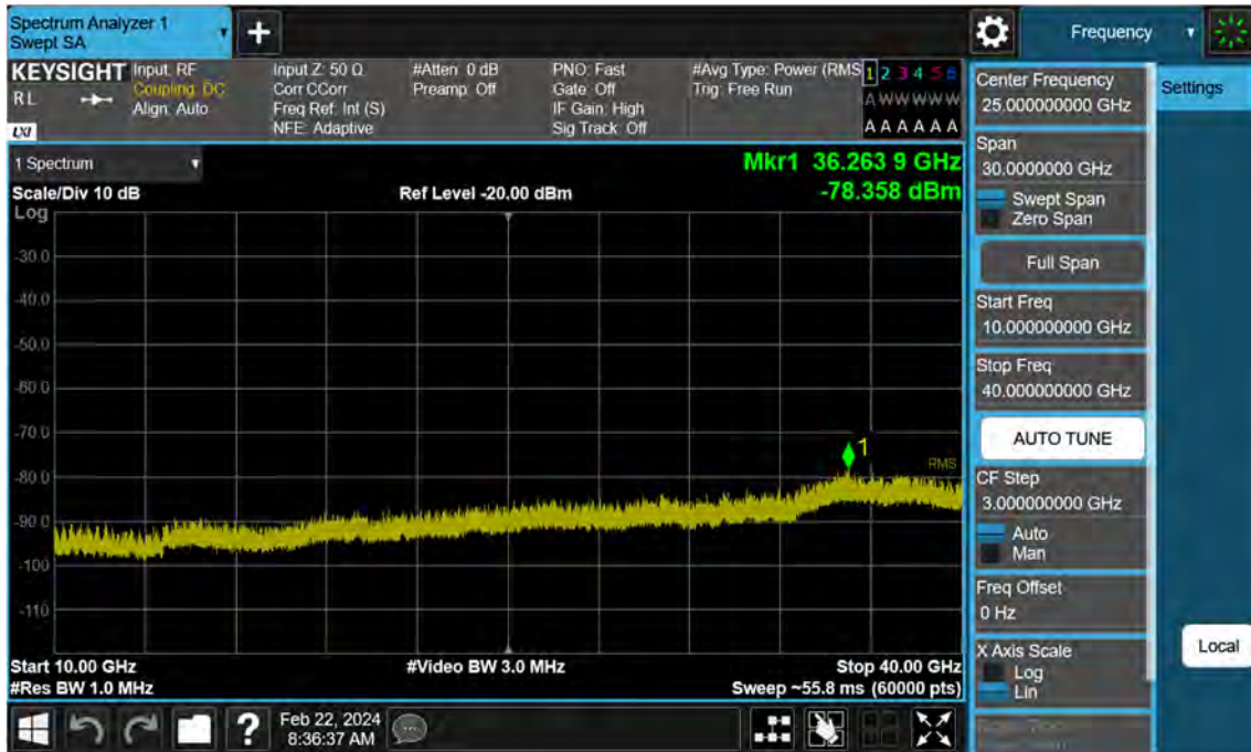
Sub6 n77. Conducted Spurious Plot_2 (634666ch_60 MHz_BPSK)
