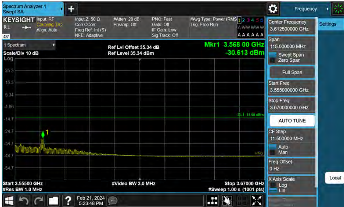
Sub6 n77. High Band Edge Plot (40 M BW Ch.635332 BPSK 1RB)(3)
