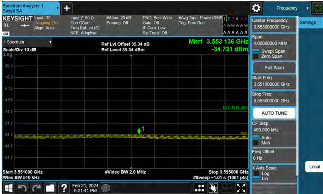
Sub6 n77. High Band Edge Plot (40 M BW Ch.635332 BPSK FullRB)(2)
