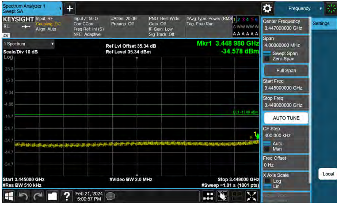
Sub6 n77. Low Band Edge Plot (30 M BW Ch.631000 BPSK FullRB)(2)
