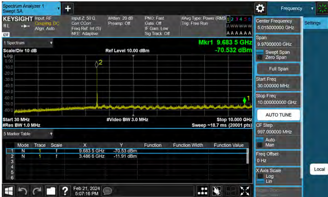
Sub6 n77. Conducted Spurious Plot_1 (633334ch_30 MHz_BPSK)
