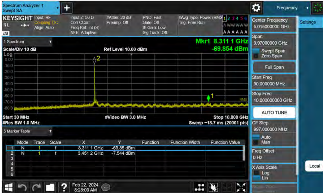
Sub6 n77. Conducted Spurious Plot_1 (632000ch_60 MHz_BPSK)
