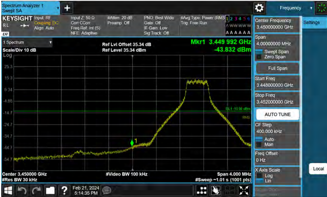
Sub6 n77. Low Band Edge Plot (40 M BW Ch.631334 BPSK 1RB)(1)
