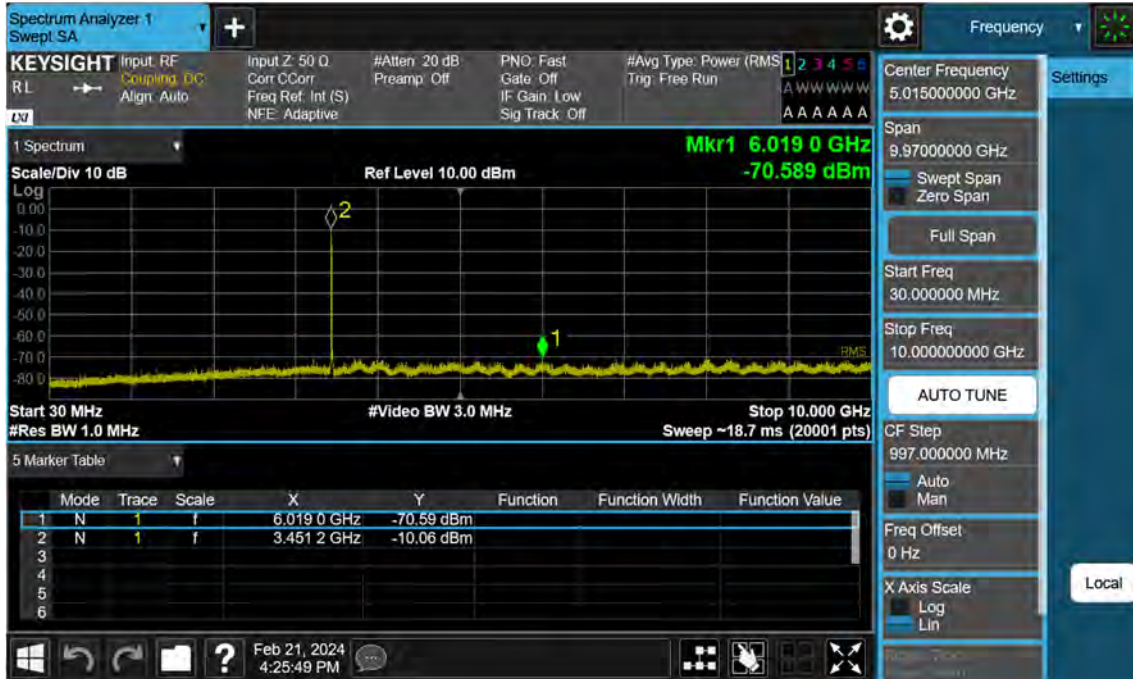
Sub6 n77. Conducted Spurious Plot_1 (630334ch_10 MHz_BPSK)
