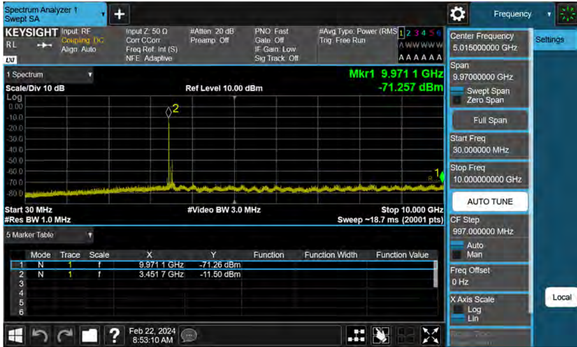
Sub6 n77. Conducted Spurious Plot_1 (632668ch_80 MHz_BPSK)
