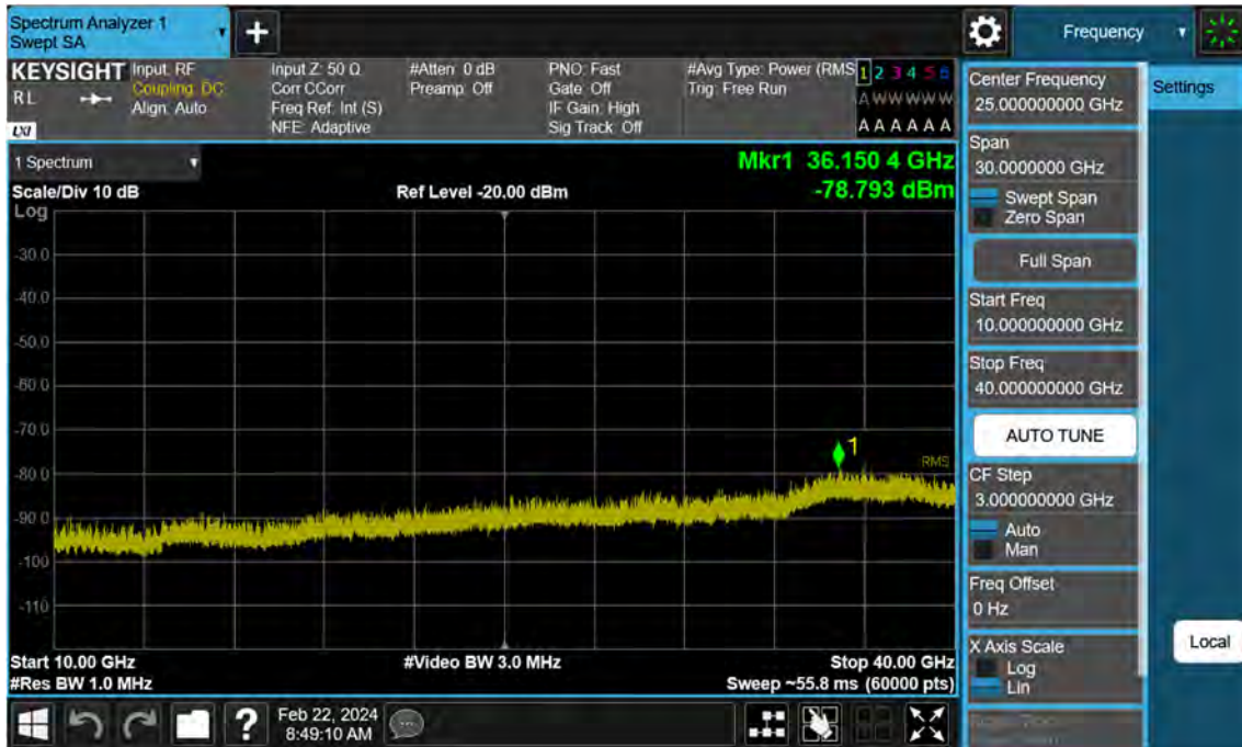
Sub6 n77. Conducted Spurious Plot_2 (634332ch_70 MHz_BPSK)
