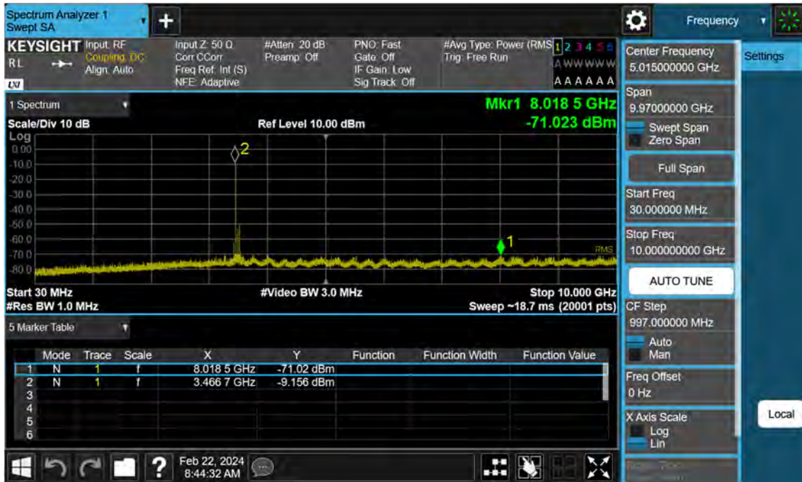
Sub6 n77. Conducted Spurious Plot_1 (633334ch_70 MHz_BPSK)
