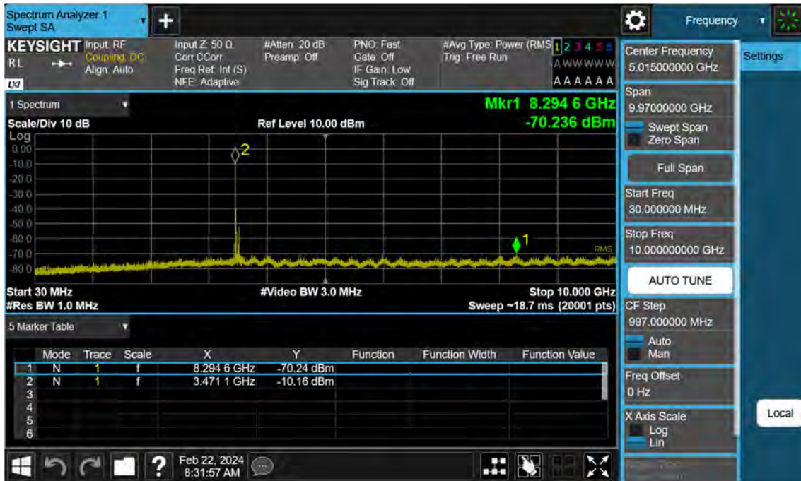
Sub6 n77. Conducted Spurious Plot_1 (633334ch_60 MHz_BPSK)
