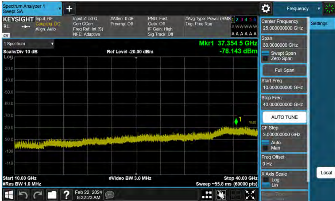
Sub6 n77. Conducted Spurious Plot_2 (633334ch_60 MHz_BPSK)
