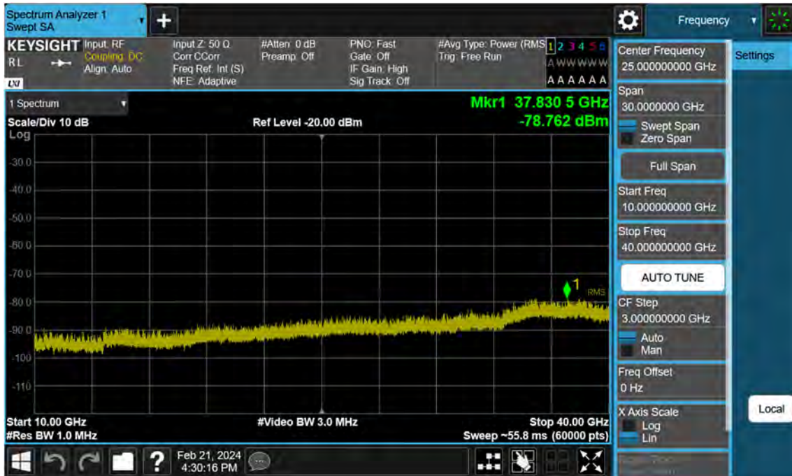
Sub6 n77. Conducted Spurious Plot_2 (633334ch_10 MHz_BPSK)
