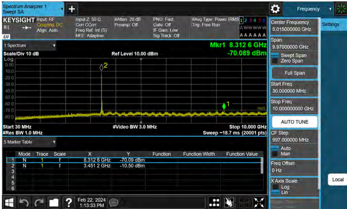
Sub6 n77. Conducted Spurious Plot_1 (630836ch_25 MHz_BPSK)
