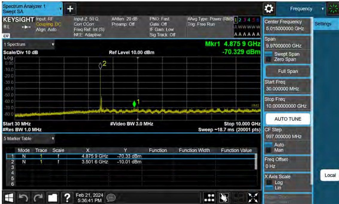
Sub6 n77. Conducted Spurious Plot_1 (635000ch_50 MHz_BPSK)
