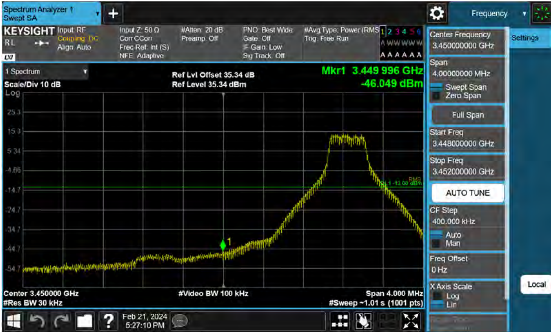
Sub6 n77. Low Band Edge Plot (50 M BW Ch.631668 BPSK 1RB)(1)
