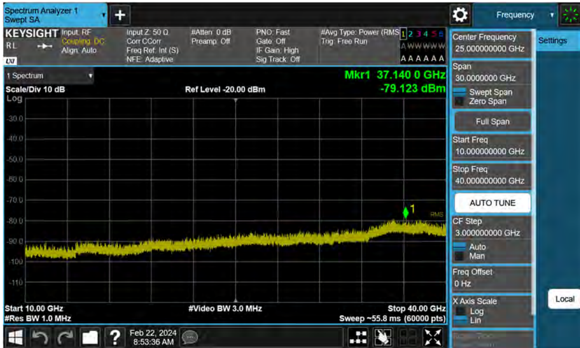
Sub6 n77. Conducted Spurious Plot_2 (632668ch_80 MHz_BPSK)
