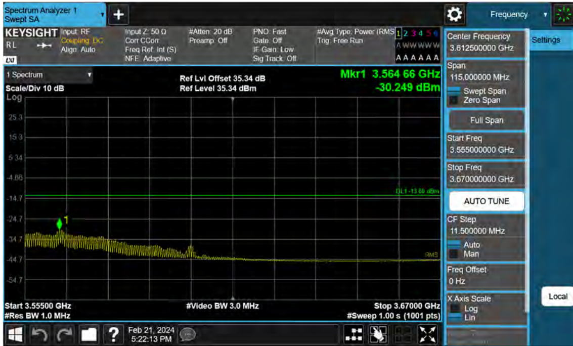
Sub6 n77. High Band Edge Plot (40 M BW Ch.635332 BPSK FullRB)(3)
