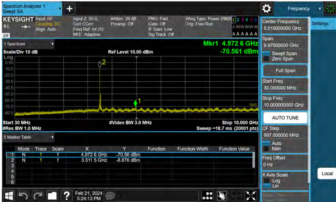
Sub6 n77. Conducted Spurious Plot_1 (635332ch_40 MHz_BPSK)
