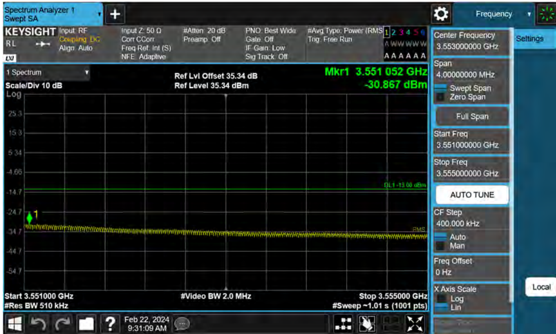
Sub6 n77. High Band Edge Plot (100 M BW Ch.633334 BPSK FullRB)(2)
