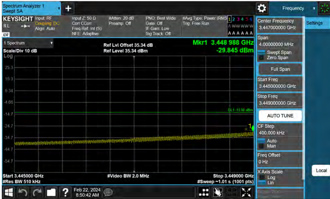
Sub6 n77. Low Band Edge Plot (80 M BW Ch.632668 BPSK FullRB)(2)
