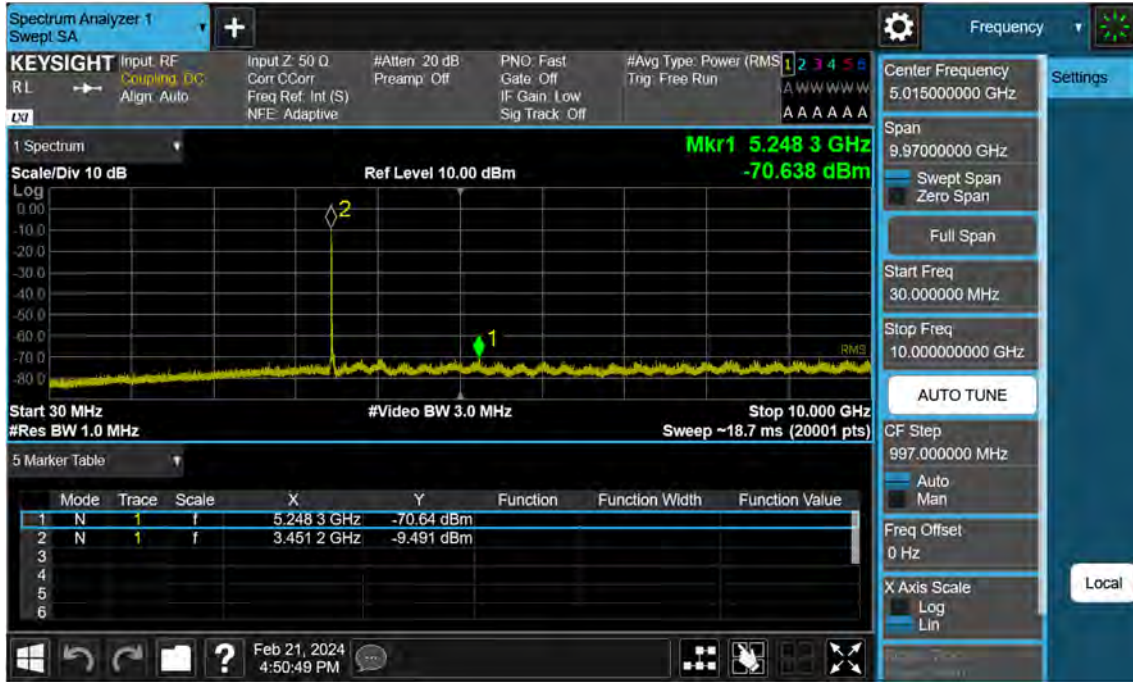
Sub6 n77. Conducted Spurious Plot_1 (630668ch_20 MHz_BPSK)
