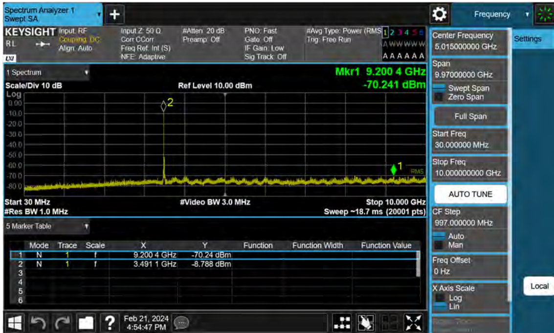
Sub6 n77. Conducted Spurious Plot_1 (633334ch_20 MHz_BPSK)
