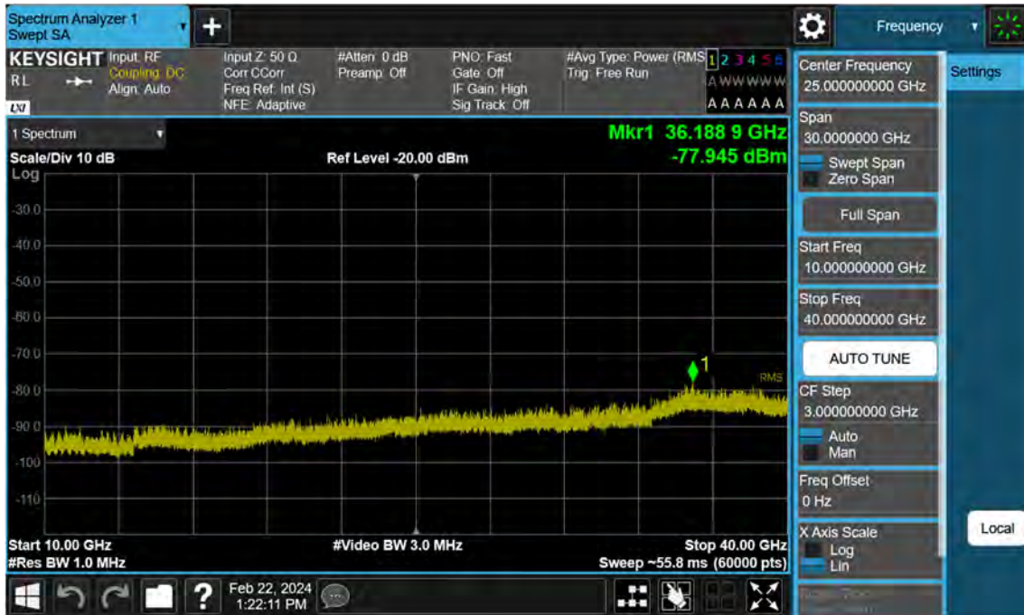
Sub6 n77. Conducted Spurious Plot_2 (635834ch_25 MHz_BPSK)
