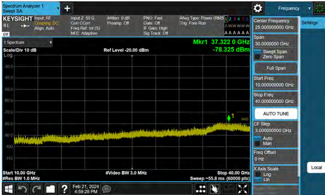
Sub6 n77. Conducted Spurious Plot_2 (636000ch_20 MHz_BPSK)
