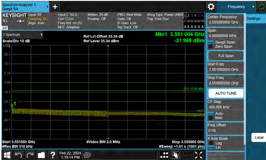
Sub6 n77. High Band Edge Plot (25 M BW Ch.635834 BPSK FullRB)(2)
