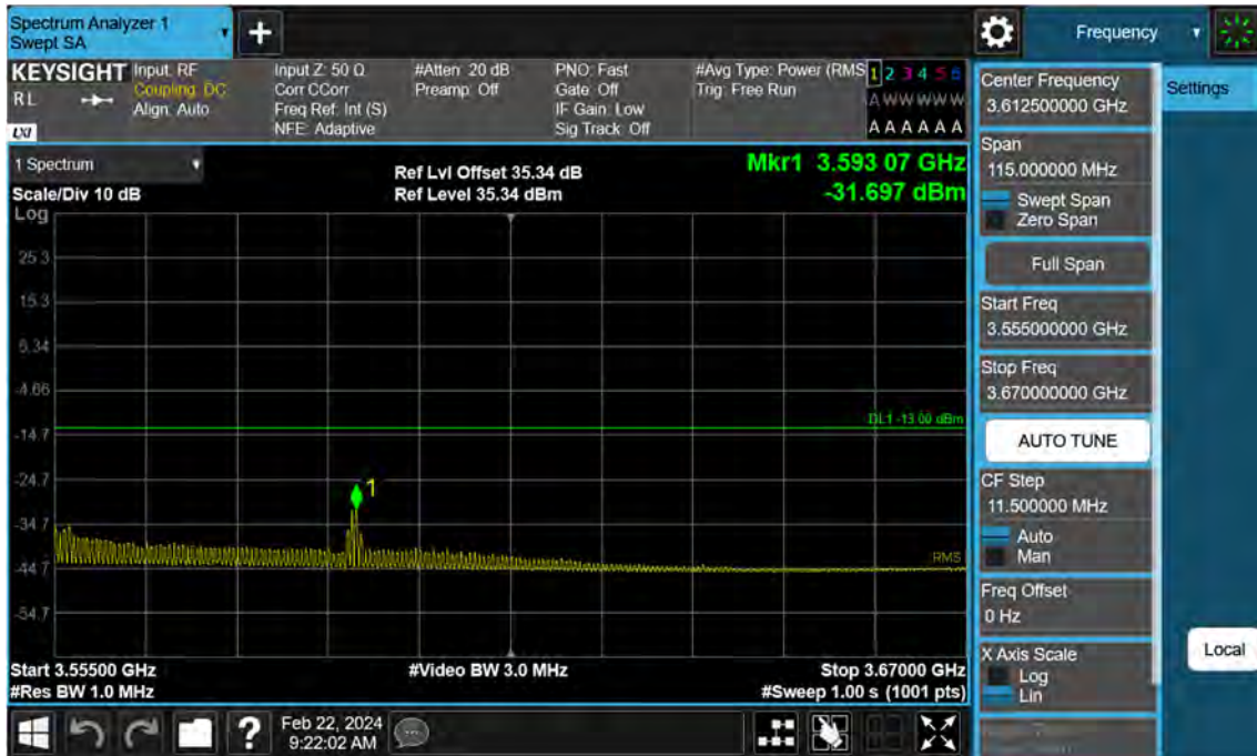
Sub6 n77. High Band Edge Plot (90 M BW Ch.633666 BPSK 1RB)(3)
