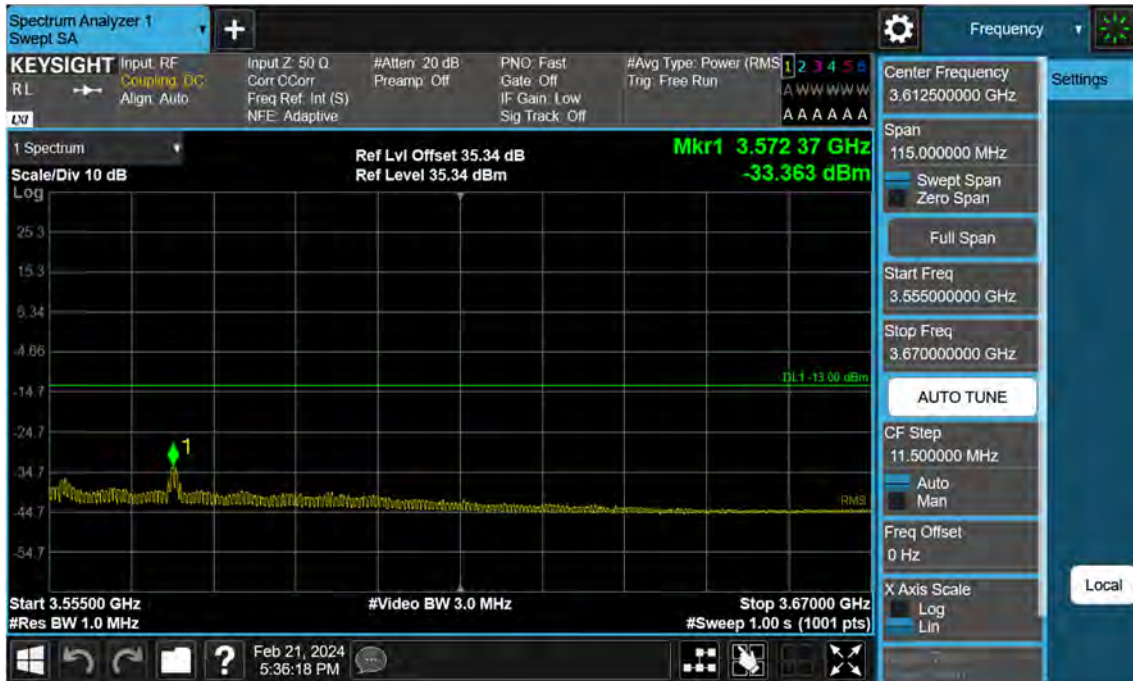
Sub6 n77. High Band Edge Plot (50 M BW Ch.635000 BPSK 1RB)(3)
