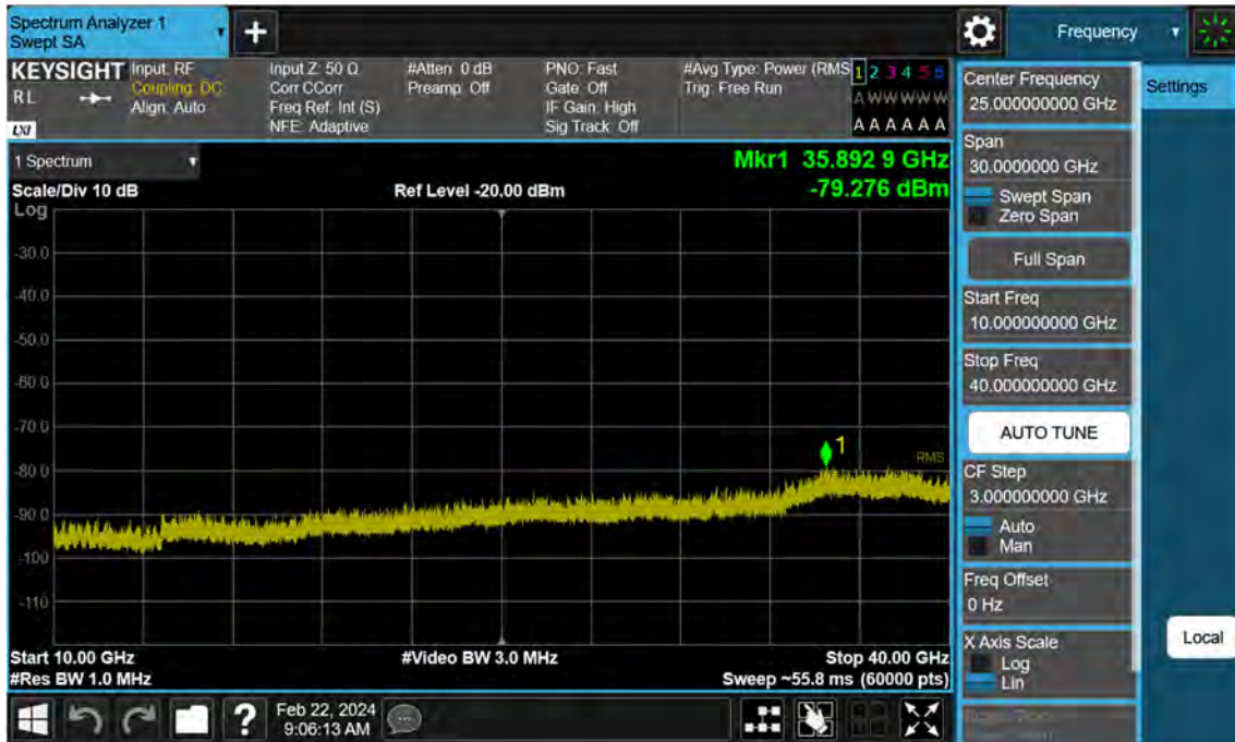
Sub6 n77. Conducted Spurious Plot_2 (633000ch_90 MHz_BPSK)
