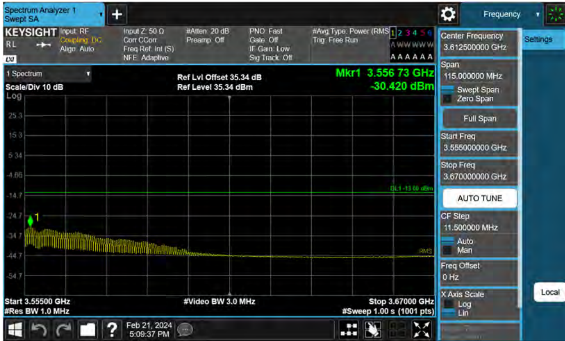
Sub6 n77. High Band Edge Plot (30 M BW Ch.635666 BPSK FullRB)(3)
