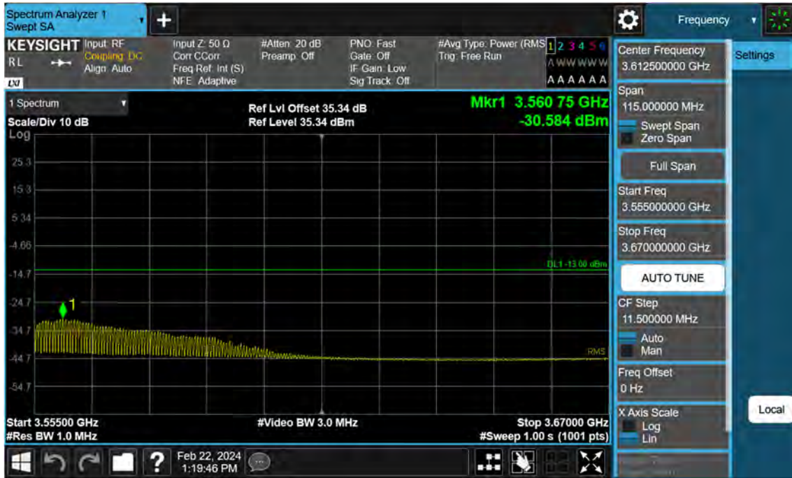
Sub6 n77. High Band Edge Plot (25 M BW Ch.636166 BPSK FullRB)(3)
