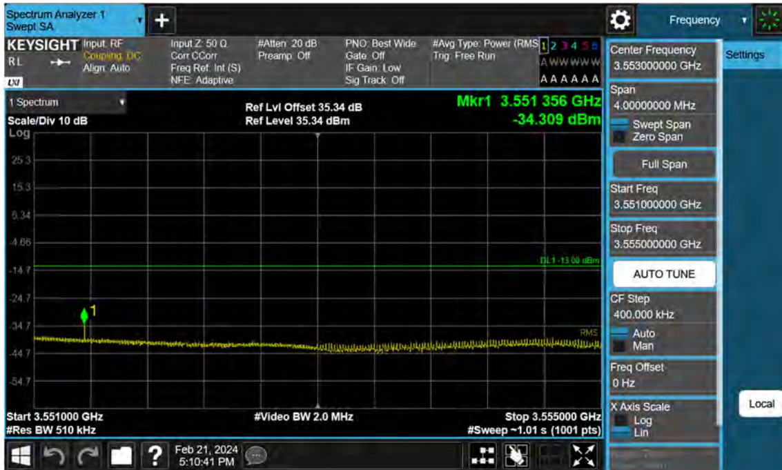
Sub6 n77. High Band Edge Plot (30 M BW Ch.635666 BPSK 1RB)(2)
