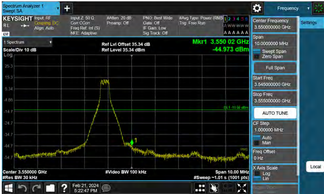
Sub6 n77. High Band Edge Plot (40 M BW Ch.635332 BPSK 1RB)(1)
