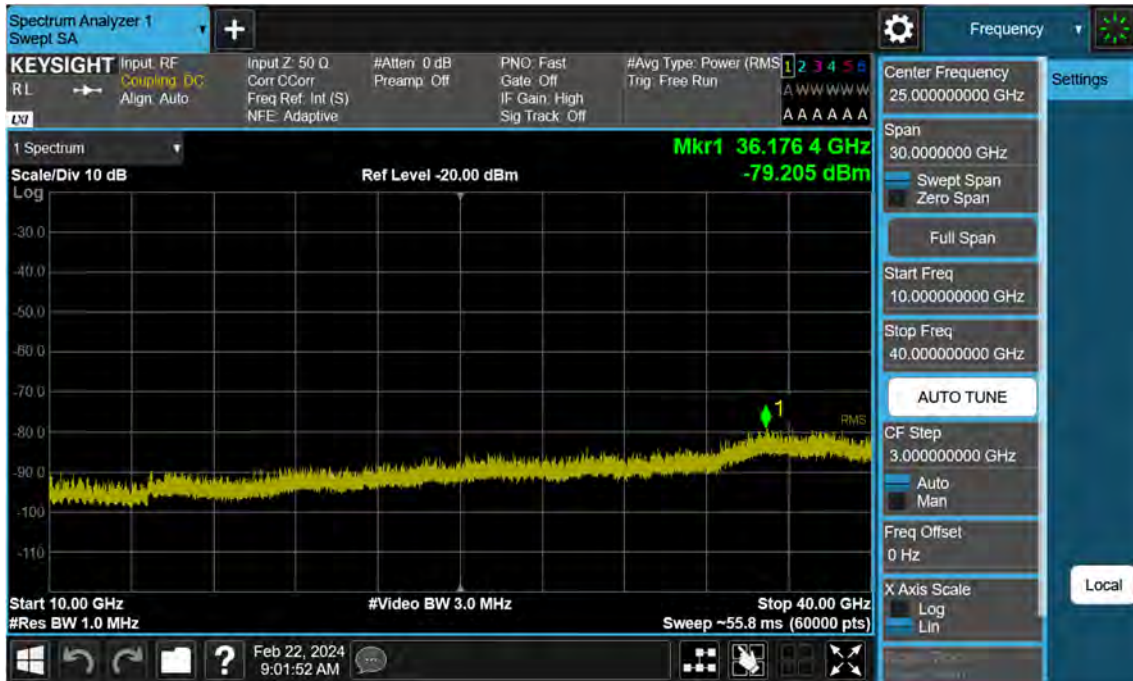
Sub6 n77. Conducted Spurious Plot_2 (634000ch_80 MHz_BPSK)
