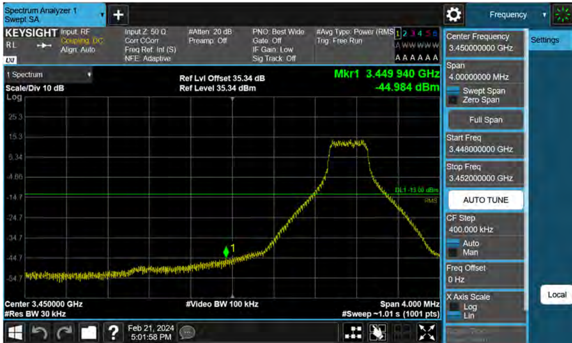
Sub6 n77. Low Band Edge Plot (30 M BW Ch.631000 BPSK 1RB)(1)
