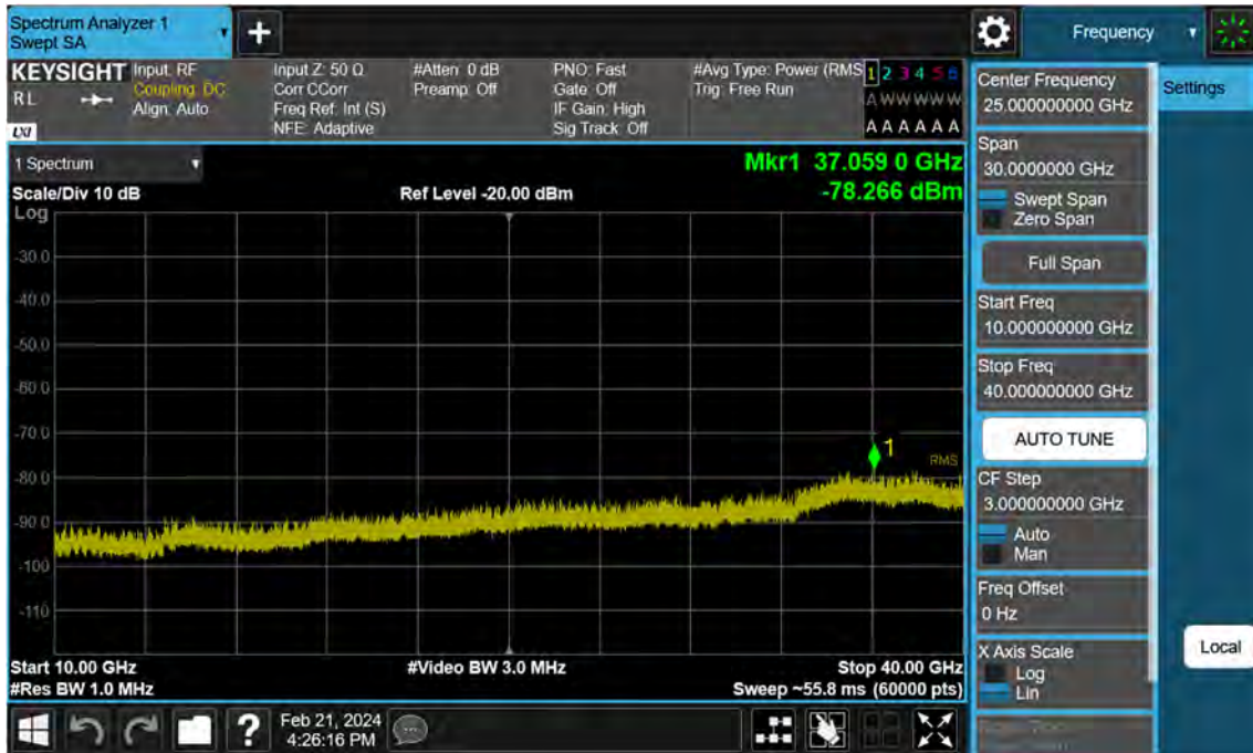
Sub6 n77. Conducted Spurious Plot_2 (630334ch_10 MHz_BPSK)
