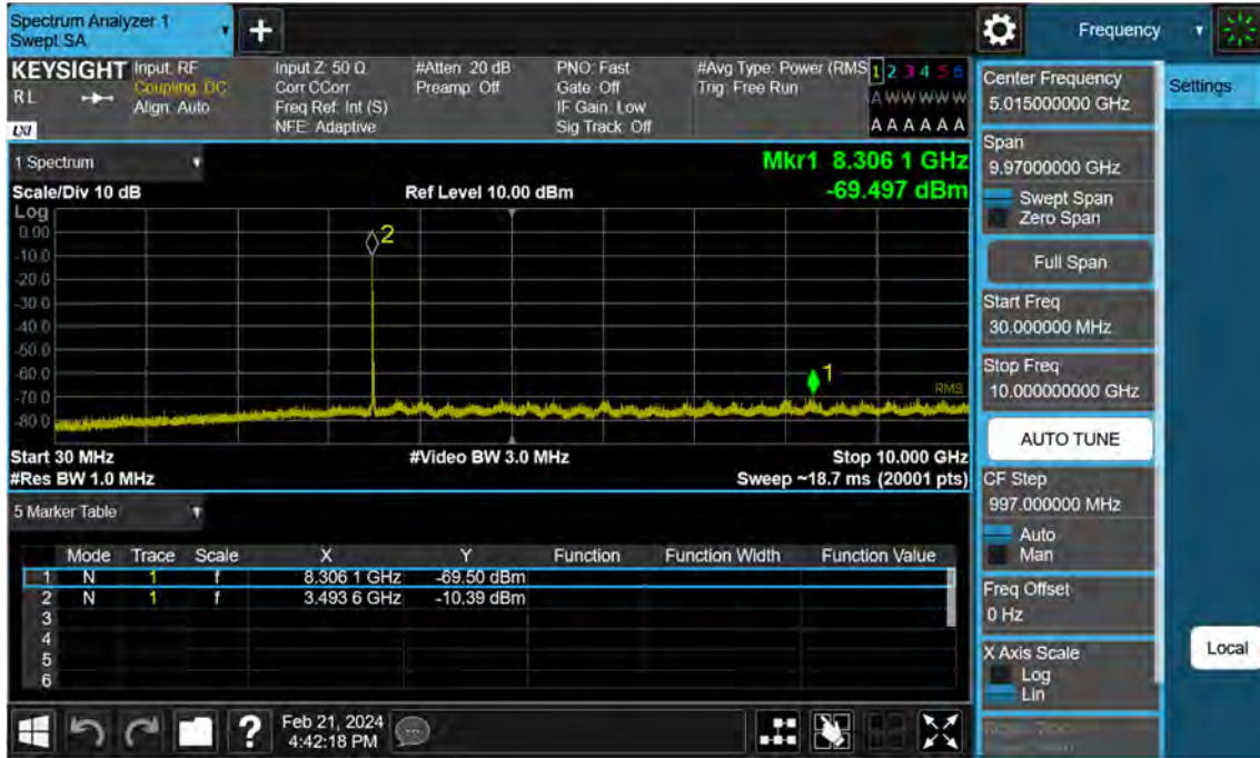
Sub6 n77. Conducted Spurious Plot_1 (633334ch_15 MHz_BPSK)
