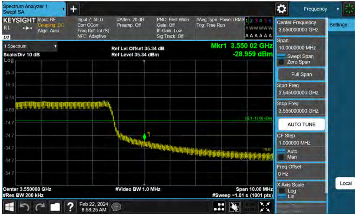
Sub6 n77. High Band Edge Plot (80 M BW Ch.634000 BPSK FullRB)(1)
