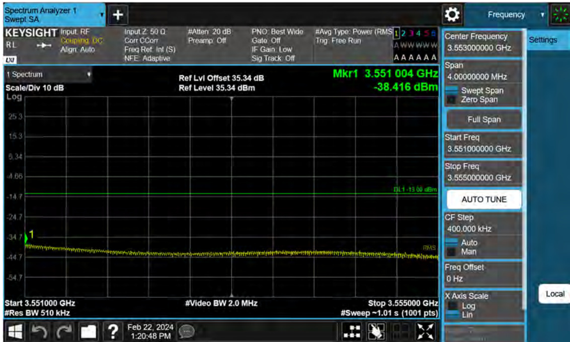
Sub6 n77. High Band Edge Plot (25 M BW Ch.635834 BPSK 1RB)(2)
