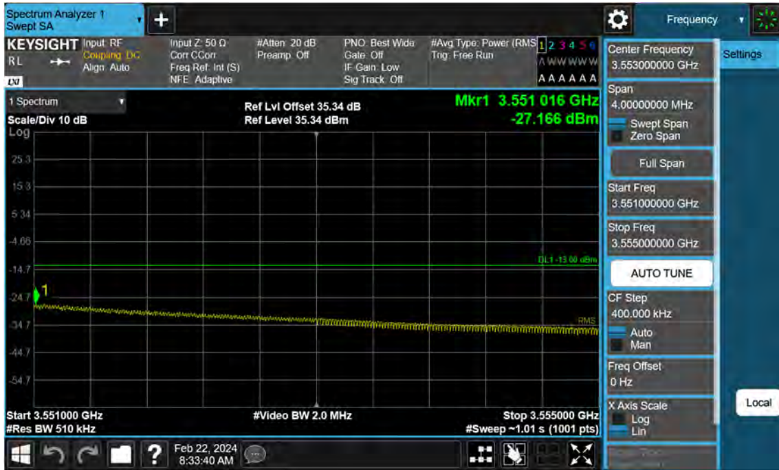
Sub6 n77. High Band Edge Plot (60 M BW Ch.634666 BPSK FullRB)(2)
