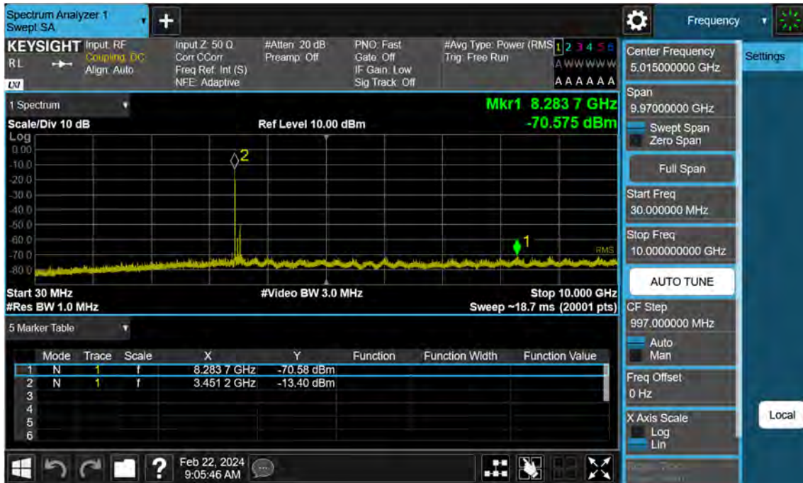
Sub6 n77. Conducted Spurious Plot_1 (633000ch_90 MHz_BPSK)
