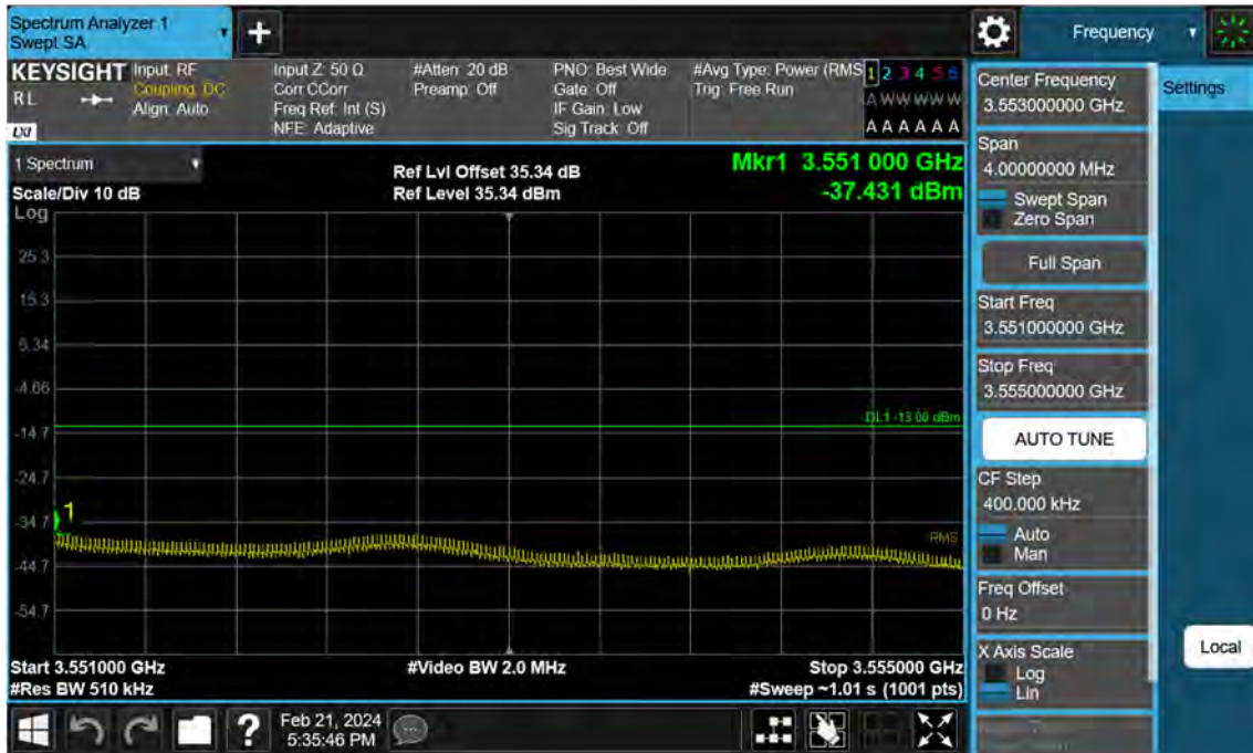
Sub6 n77. High Band Edge Plot (50 M BW Ch.635000 BPSK 1RB)(2)
