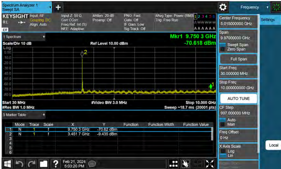
Sub6 n77. Conducted Spurious Plot_1 (631000ch_30 MHz_BPSK)
