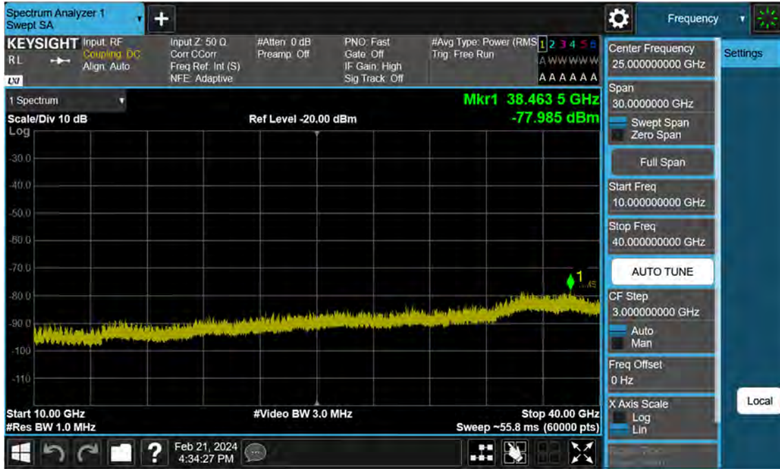
Sub6 n77. Conducted Spurious Plot_2 (636322ch_10 MHz_BPSK)
