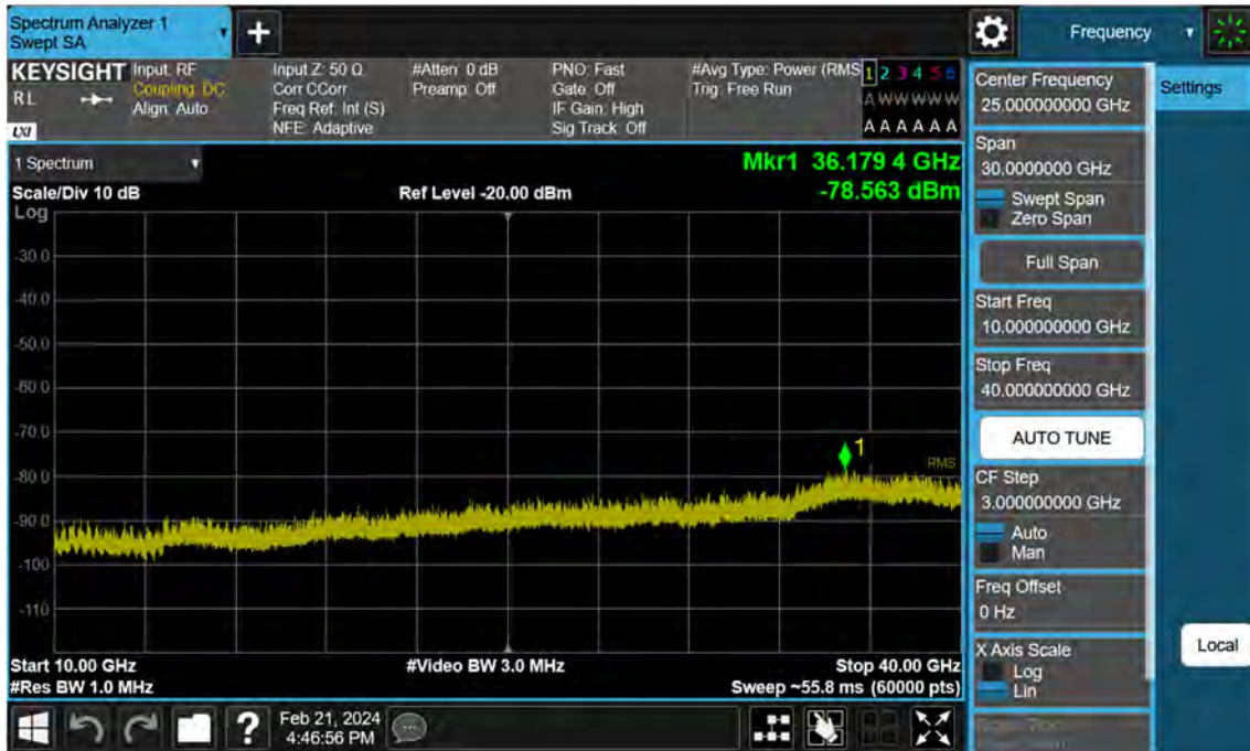
Sub6 n77. Conducted Spurious Plot_2 (636166ch_15 MHz_BPSK)
