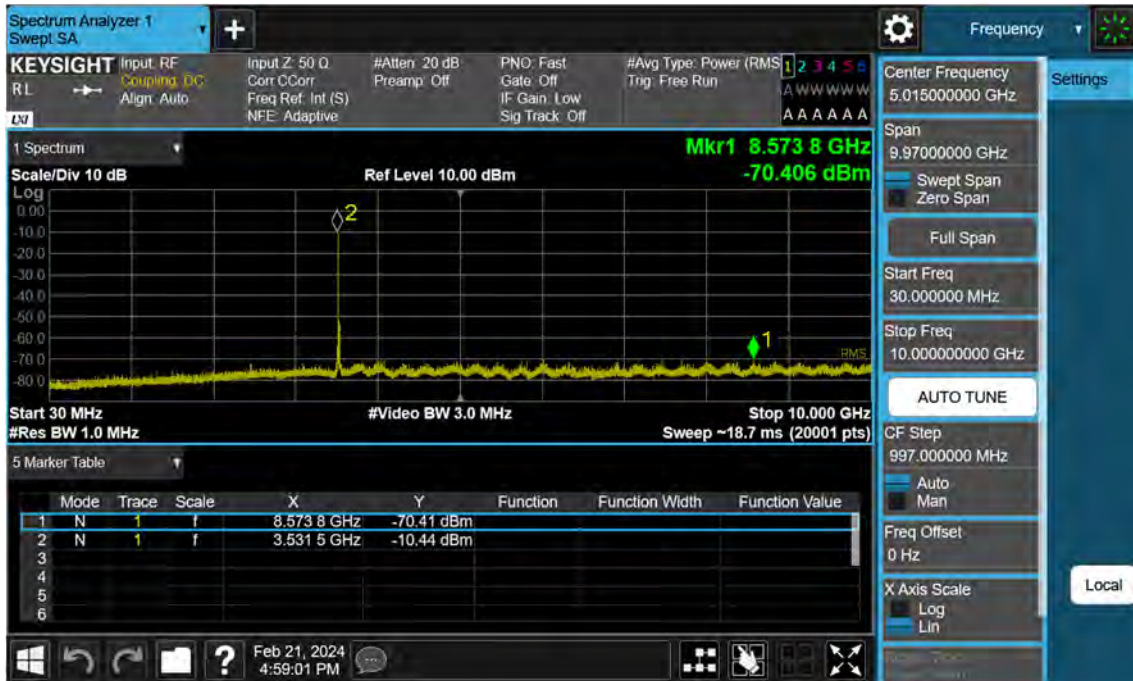
Sub6 n77. Conducted Spurious Plot_1 (636000ch_20 MHz_BPSK)
