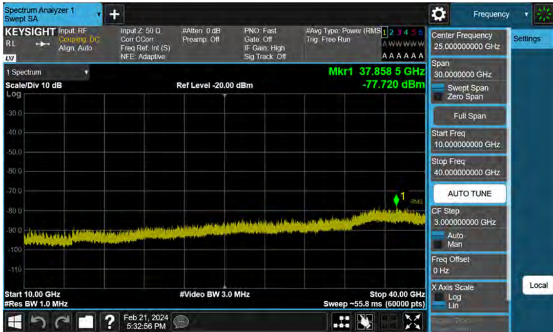
Sub6 n77. Conducted Spurious Plot_2 (633334ch_50 MHz_BPSK)
