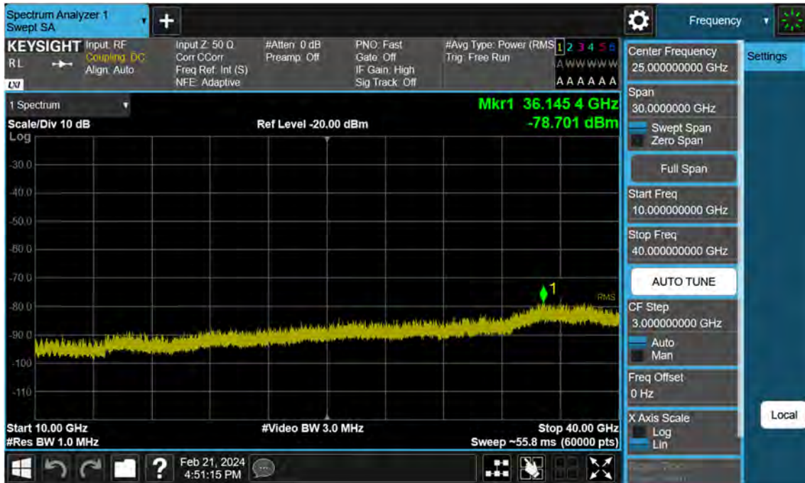
Sub6 n77. Conducted Spurious Plot_2 (630668ch_20 MHz_BPSK)
