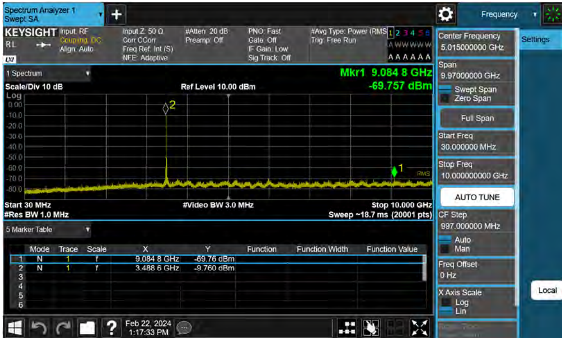
Sub6 n77. Conducted Spurious Plot_1 (633334ch_25 MHz_BPSK)
