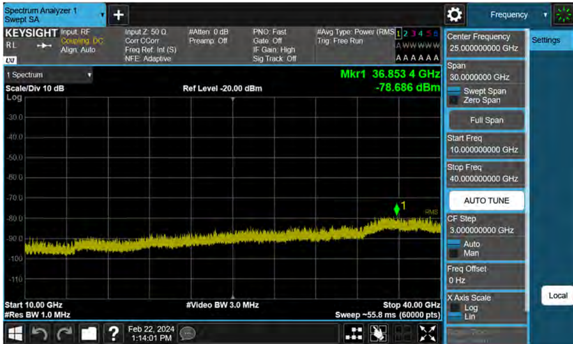
Sub6 n77. Conducted Spurious Plot_2 (630836ch_25 MHz_BPSK)
