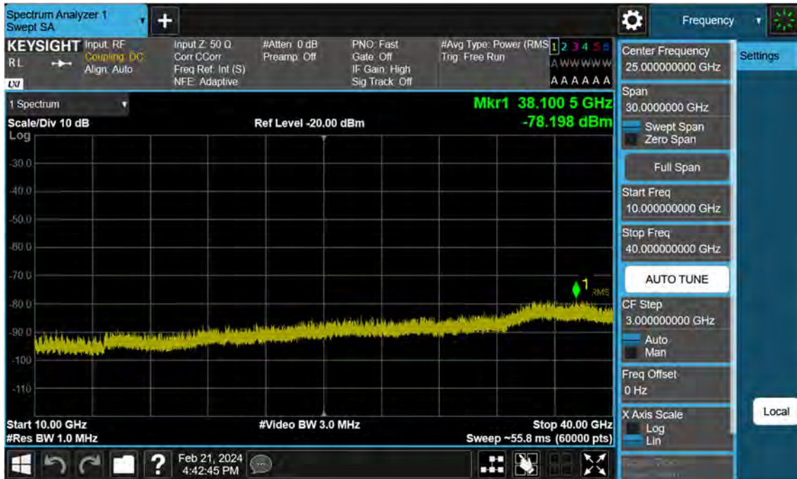
Sub6 n77. Conducted Spurious Plot_2 (633334ch_15 MHz_BPSK)
