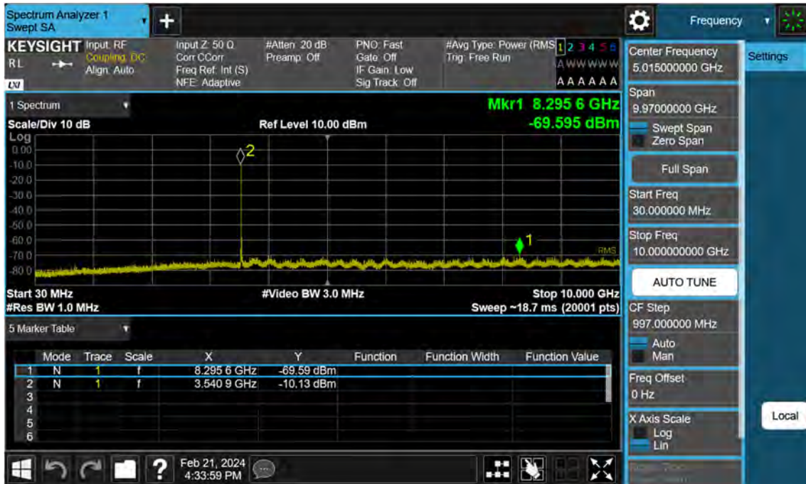
Sub6 n77. Conducted Spurious Plot_1 (636322ch_10 MHz_BPSK)
