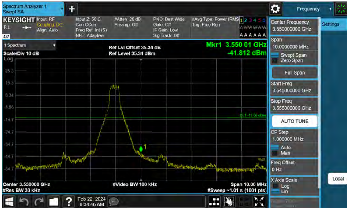
Sub6 n77. High Band Edge Plot (60 M BW Ch.634666 BPSK 1RB)(1)
