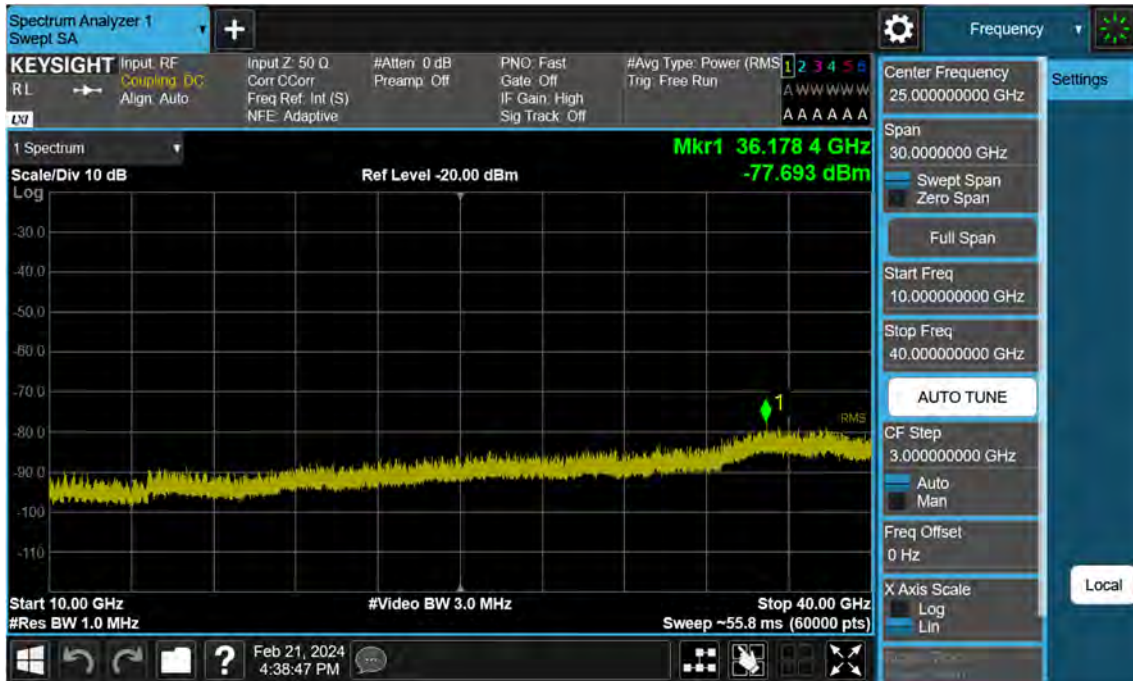
Sub6 n77. Conducted Spurious Plot_2 (630500ch_15 MHz_BPSK)
