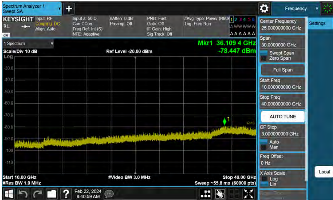
Sub6 n77. Conducted Spurious Plot_2 (632334ch_70 MHz_BPSK)
