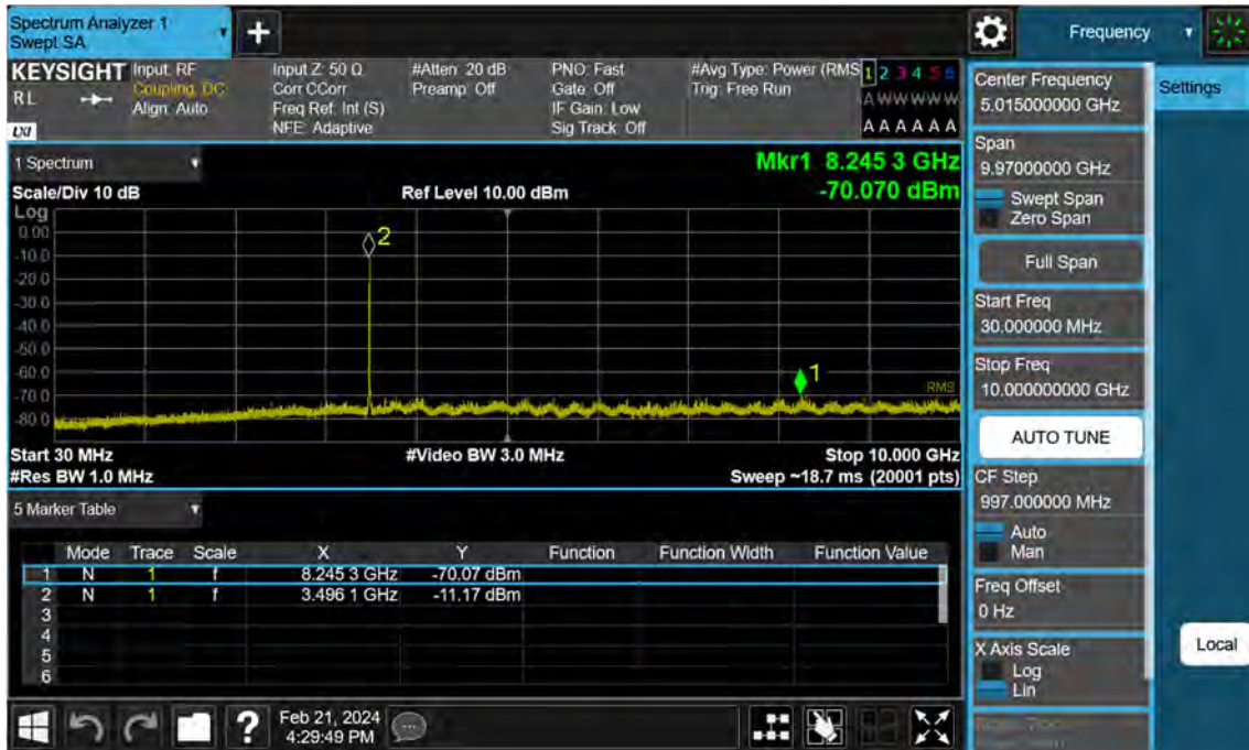
Sub6 n77. Conducted Spurious Plot_1 (633334ch_10 MHz_BPSK)
