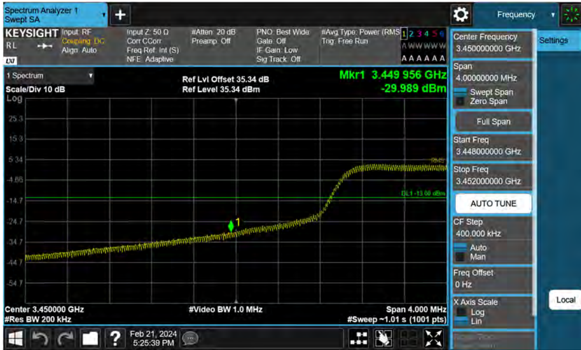
Sub6 n77. Low Band Edge Plot (50 M BW Ch.631668 BPSK FullRB)(1)
