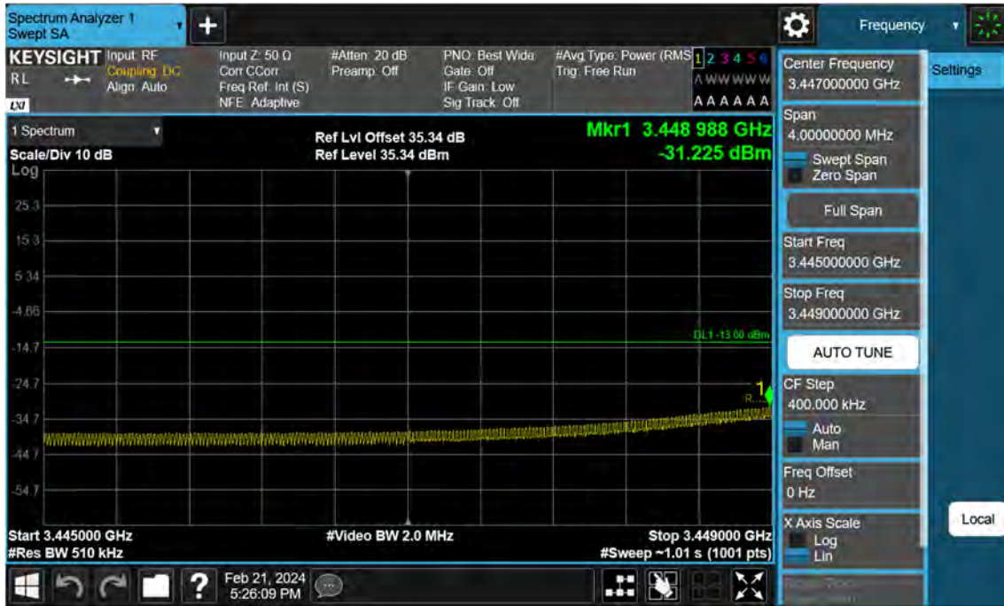
Sub6 n77. Low Band Edge Plot (50 M BW Ch.631668 BPSK FullRB)(2)
