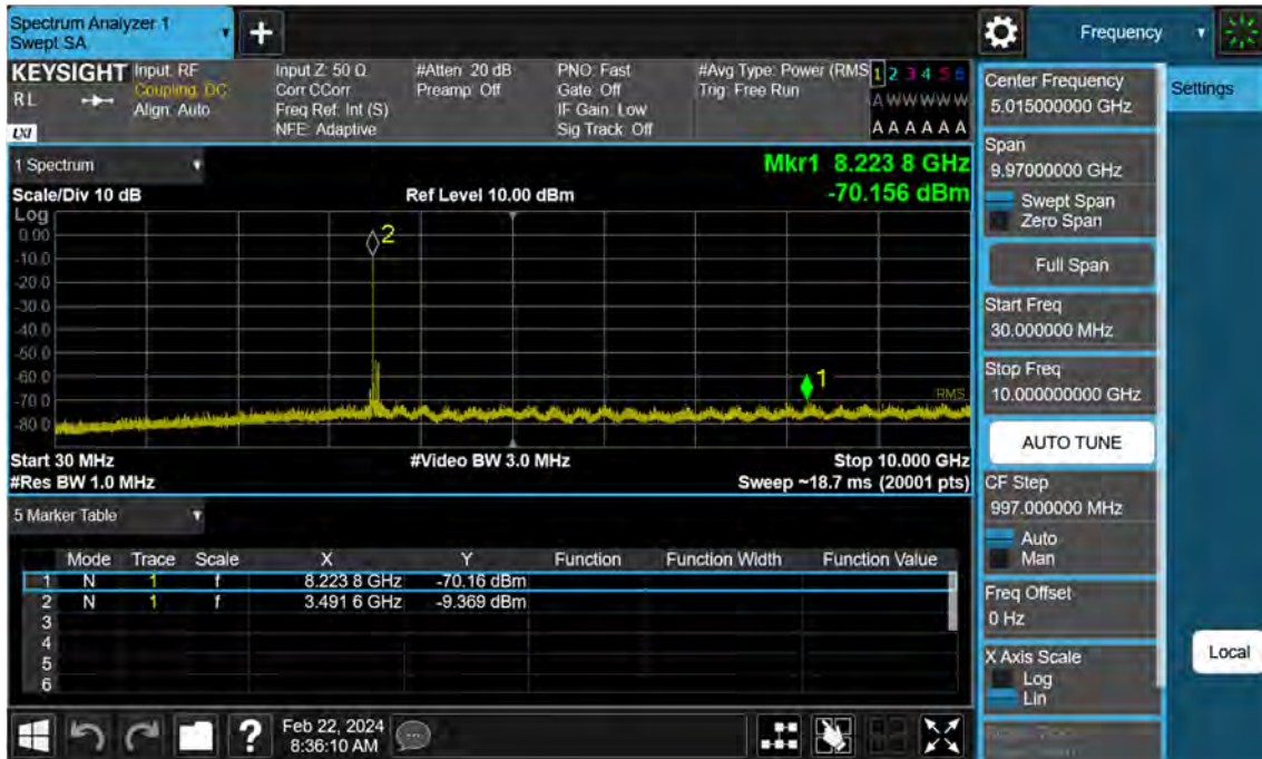
Sub6 n77. Conducted Spurious Plot_1 (634666ch_60 MHz_BPSK)
