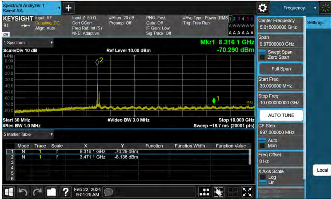
Sub6 n77. Conducted Spurious Plot_1 (634000ch_80 MHz_BPSK)
