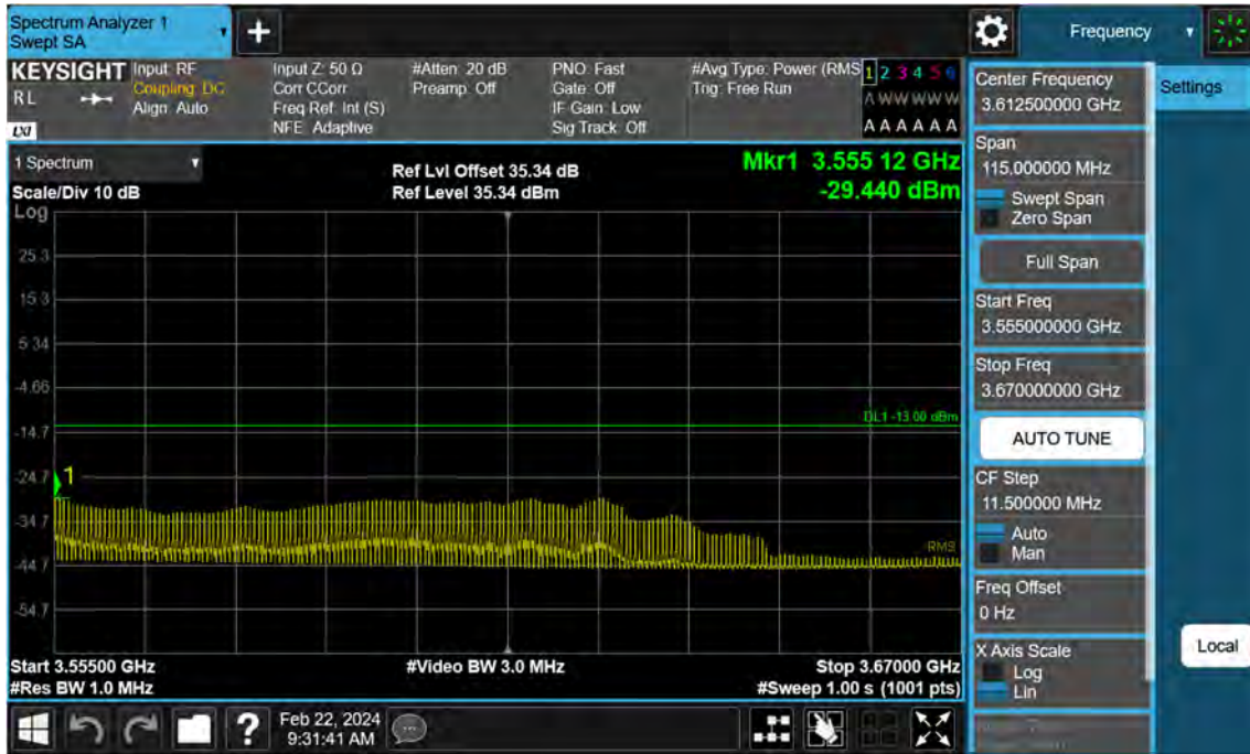
Sub6 n77. High Band Edge Plot (100 M BW Ch.633334 BPSK FullRB)(3)
