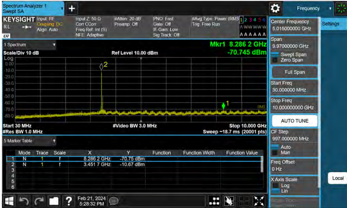
Sub6 n77. Conducted Spurious Plot_1 (631668ch_50 MHz_BPSK)
