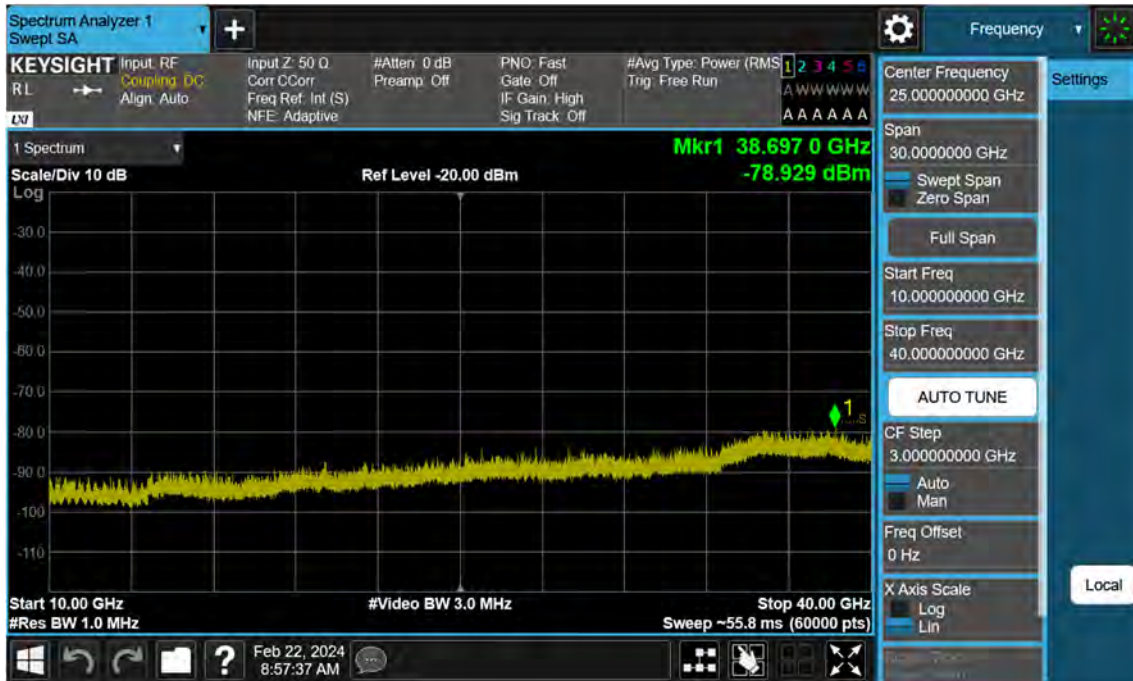
Sub6 n77. Conducted Spurious Plot_2 (633334ch_80 MHz_BPSK)
