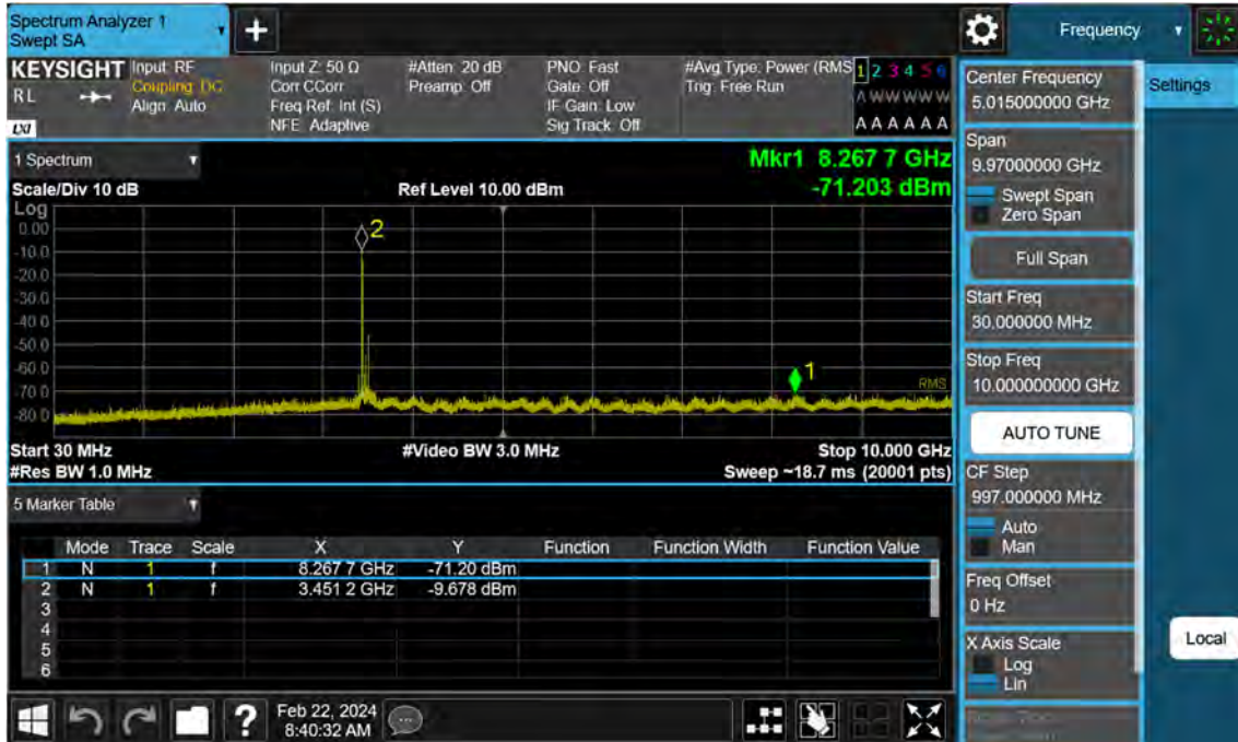
Sub6 n77. Conducted Spurious Plot_1 (632334ch_70 MHz_BPSK)
