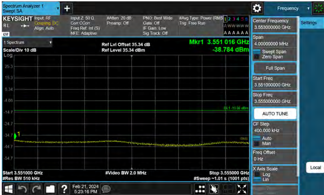
Sub6 n77. High Band Edge Plot (40 M BW Ch.635332 BPSK 1RB)(2)
