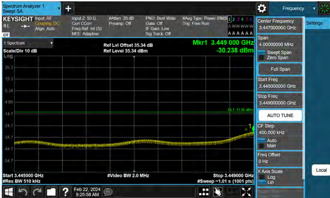
Sub6 n77. Low Band Edge Plot (100 M BW Ch.633334 BPSK 1RB)(2)
