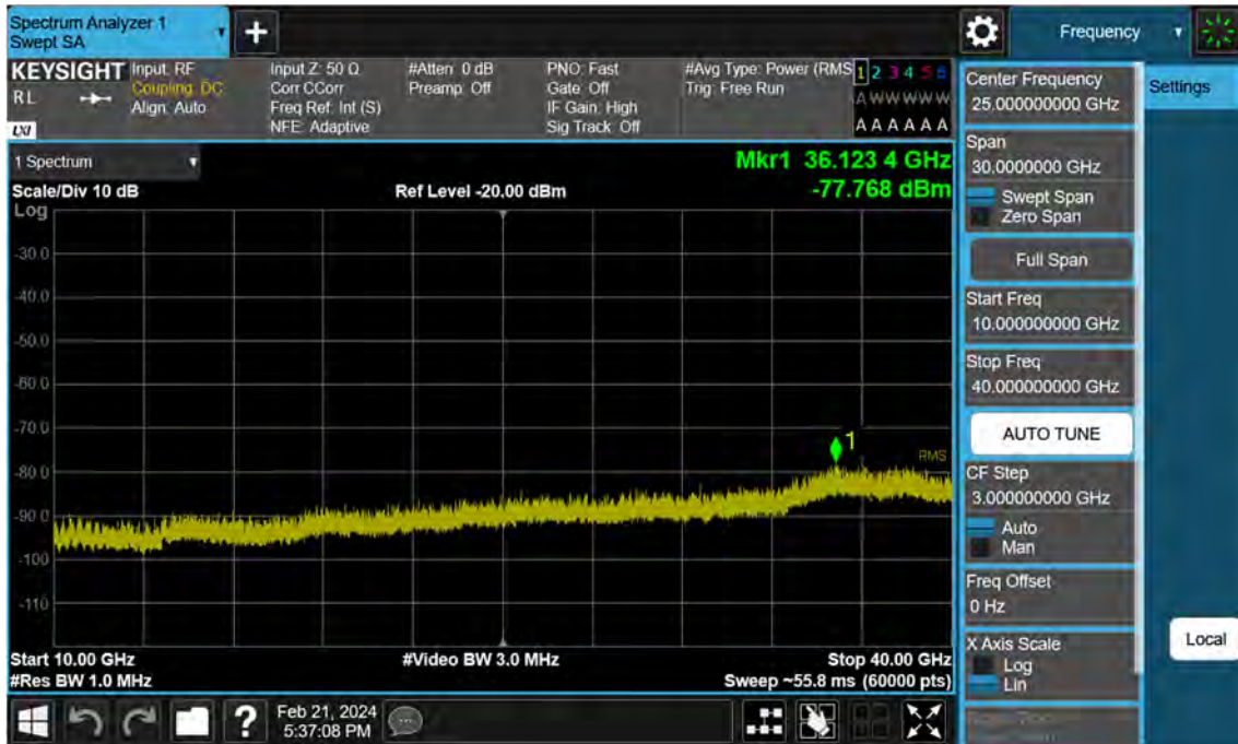
Sub6 n77. Conducted Spurious Plot_2 (635000ch_50 MHz_BPSK)
