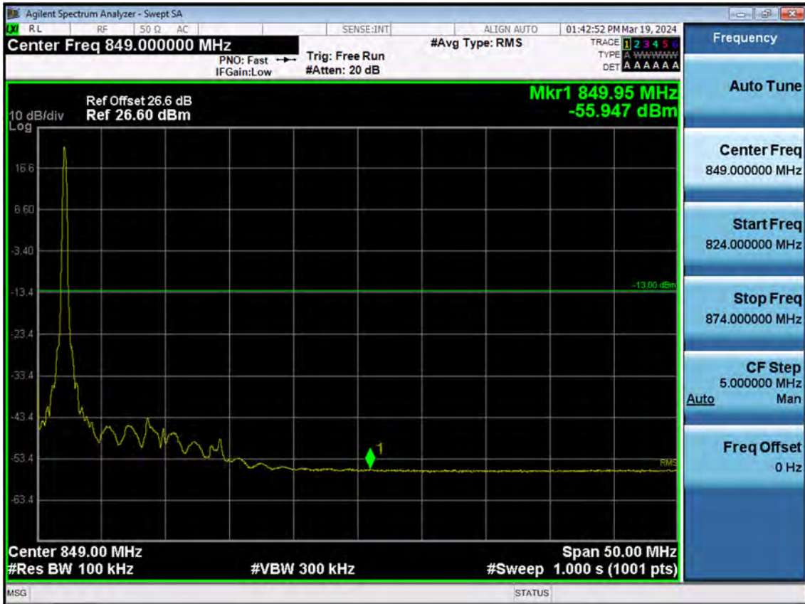
BAND 26. Band Edge (5 MHz_QPSK_RB 1_24)
