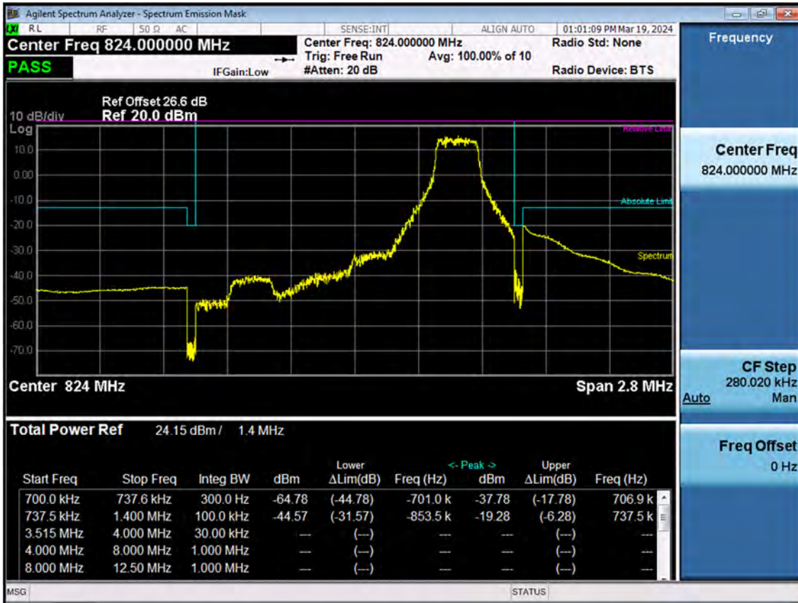
BAND 26. Channel Edge (1.4 MHz_QPSK_RB 1_5)
