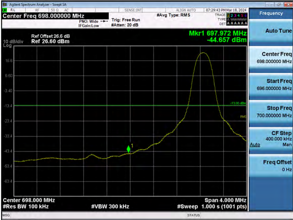
BAND 12. Lower Band Edge Plot (1.4 M BW Ch.23017 QPSK_RB1_Offset 0)
