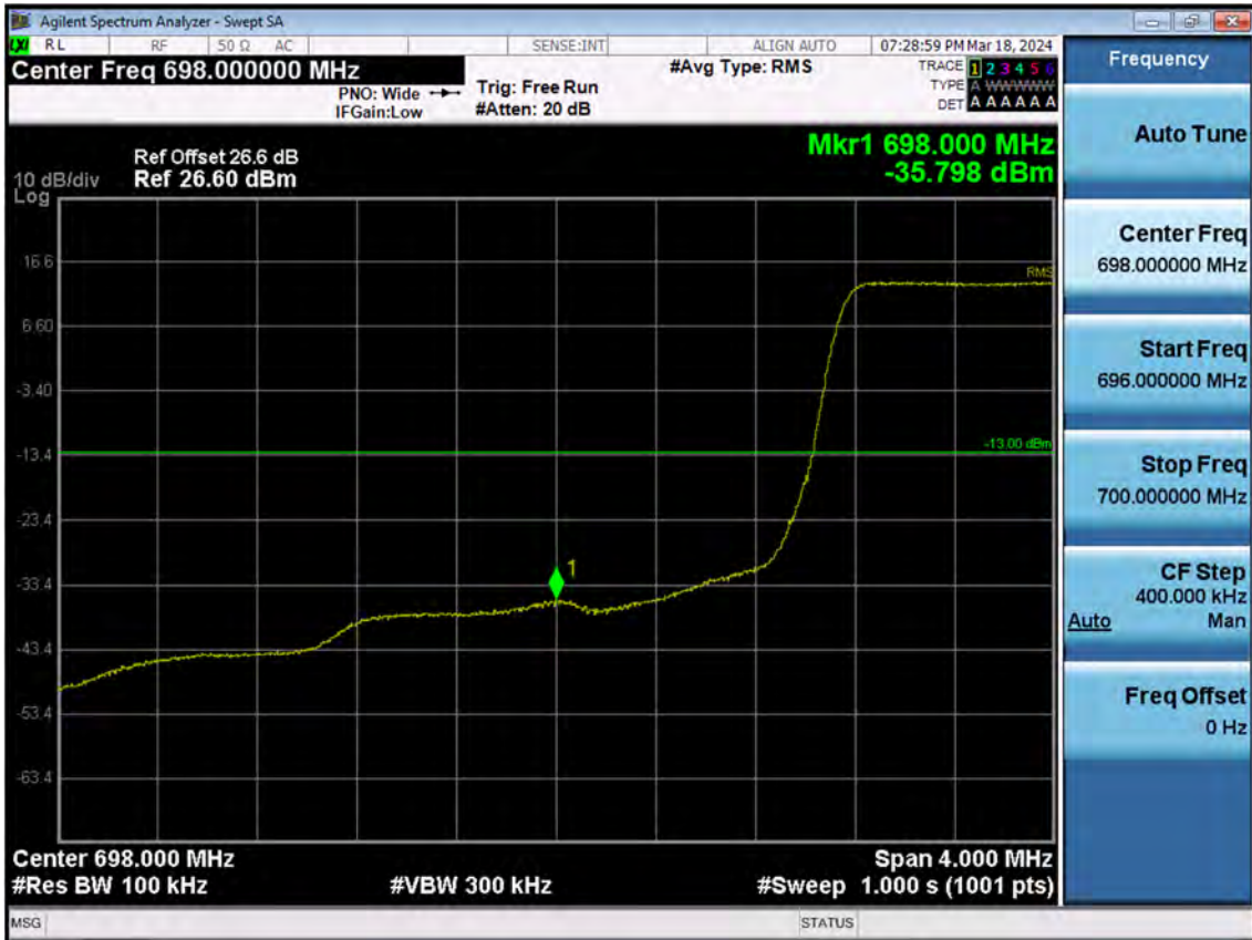
BAND 12. Lower Band Edge Plot (1.4 M BW Ch.23017 QPSK_RB6_Offset 0)
