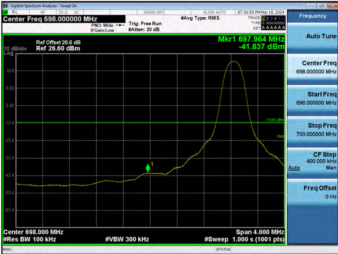
BAND 12. Lower Band Edge Plot (3 M BW Ch.23025 QPSK_RB1_Offset 0)
