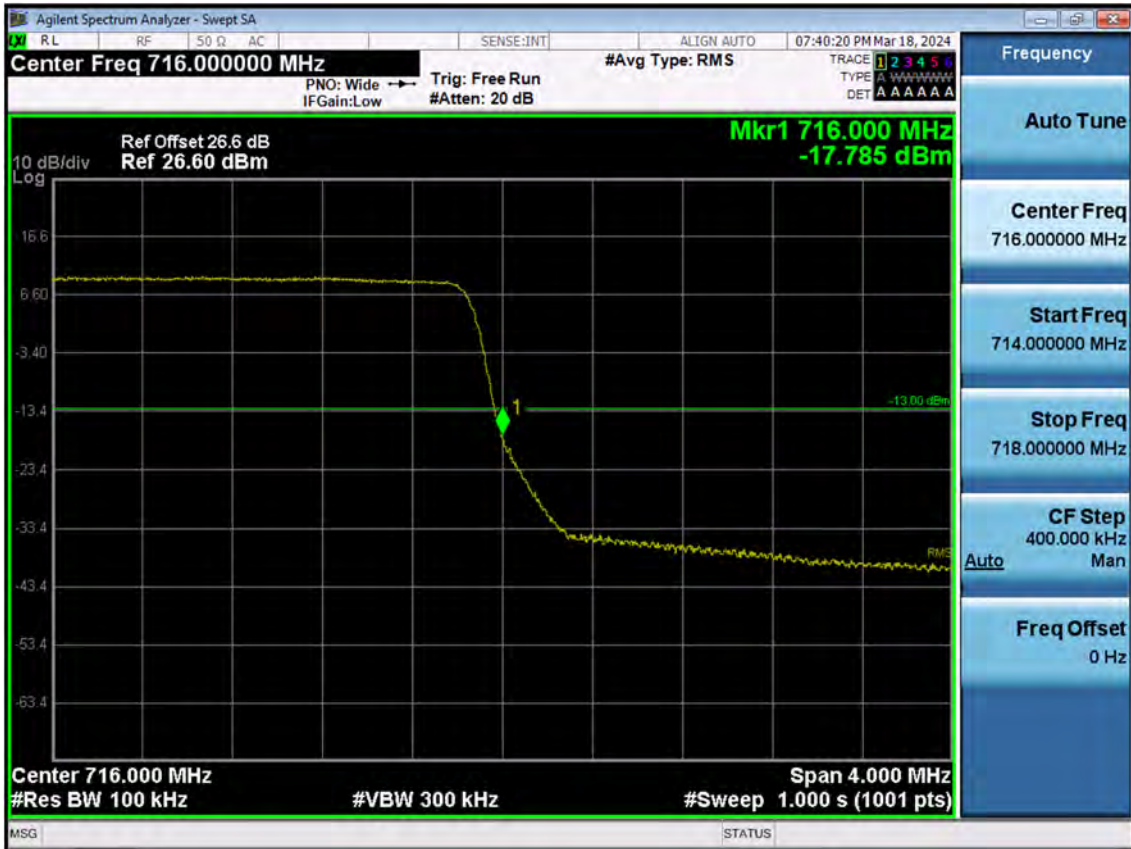
BAND 12. Upper Band Edge Plot (3 M BW Ch.23165 QPSK_RB15_Offset 0)
