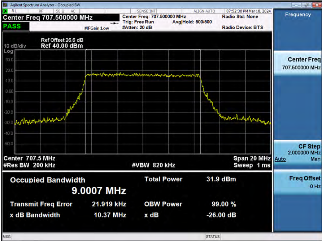
BAND 12/17. Occupied Bandwidth Plot (10 M BW Ch.23095 QPSK_RB50_0)
