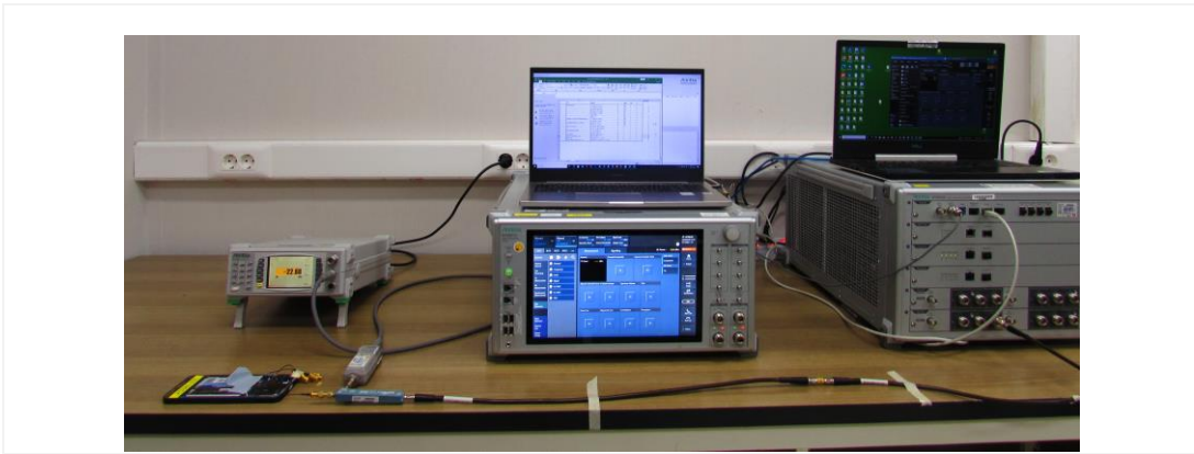
Test setup photo-2(TC 3-1, 3-2, 4-1, 4-2, 9)
