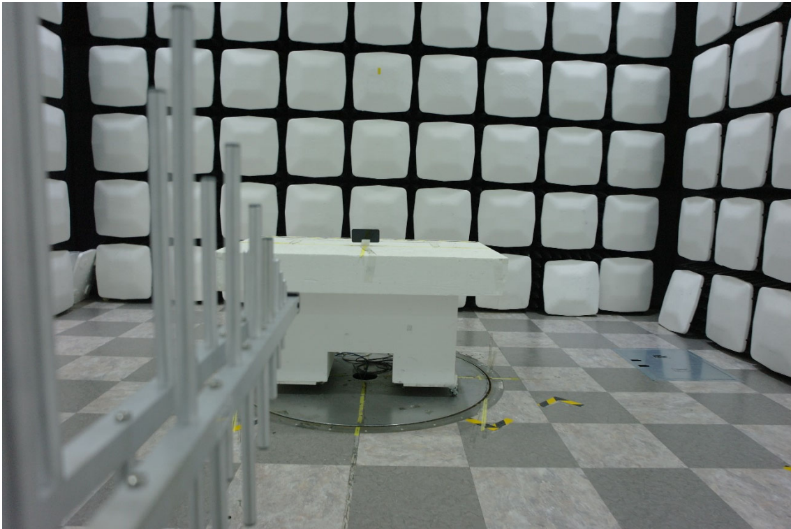
NFC Radiated Test Setup Photo for 30 MHz ~ 1 GHz :
