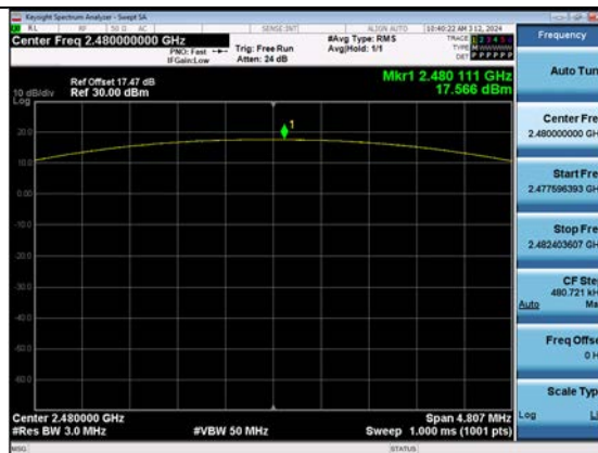
GFSK : Peak Power (Ch. 78)
