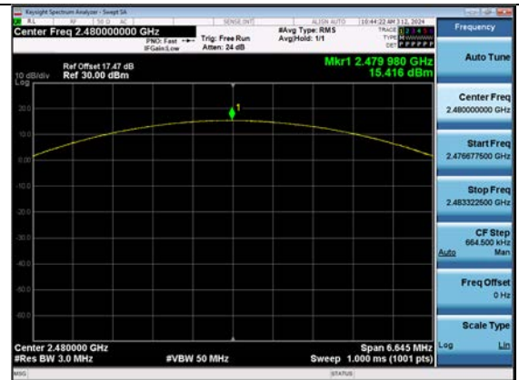
8DPSK : Peak Power (Ch. 78)
