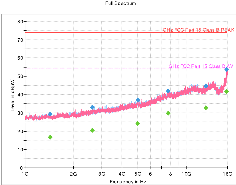
Figure 4: LTE B26 High ch Idle
