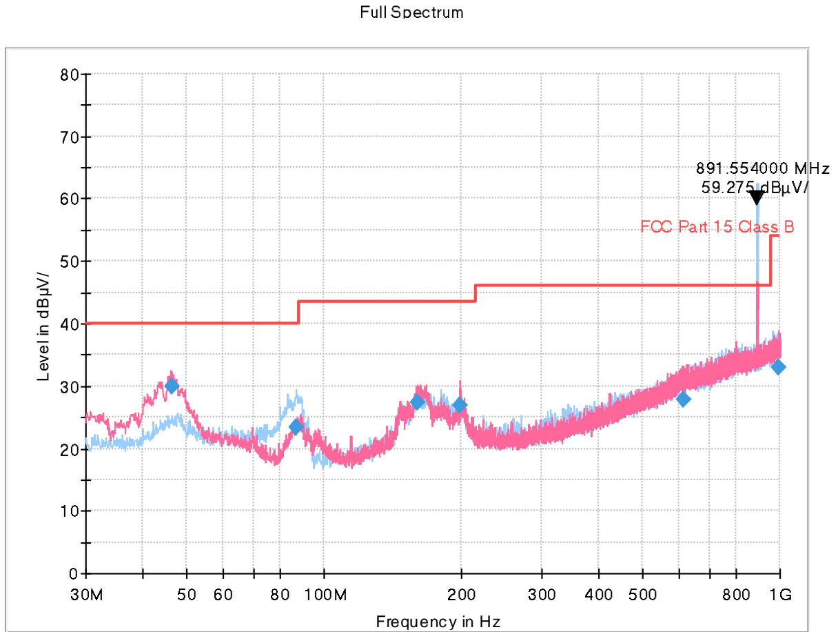
Figure 3: LTE B26 High ch Idle
