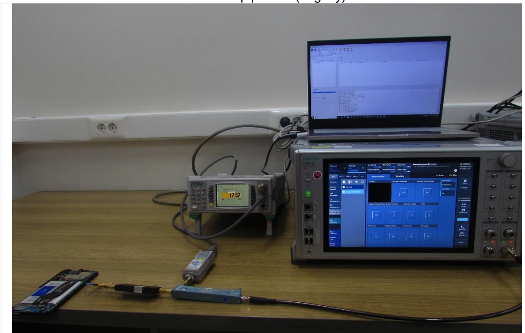
Test setup photo-2(Legacy)
