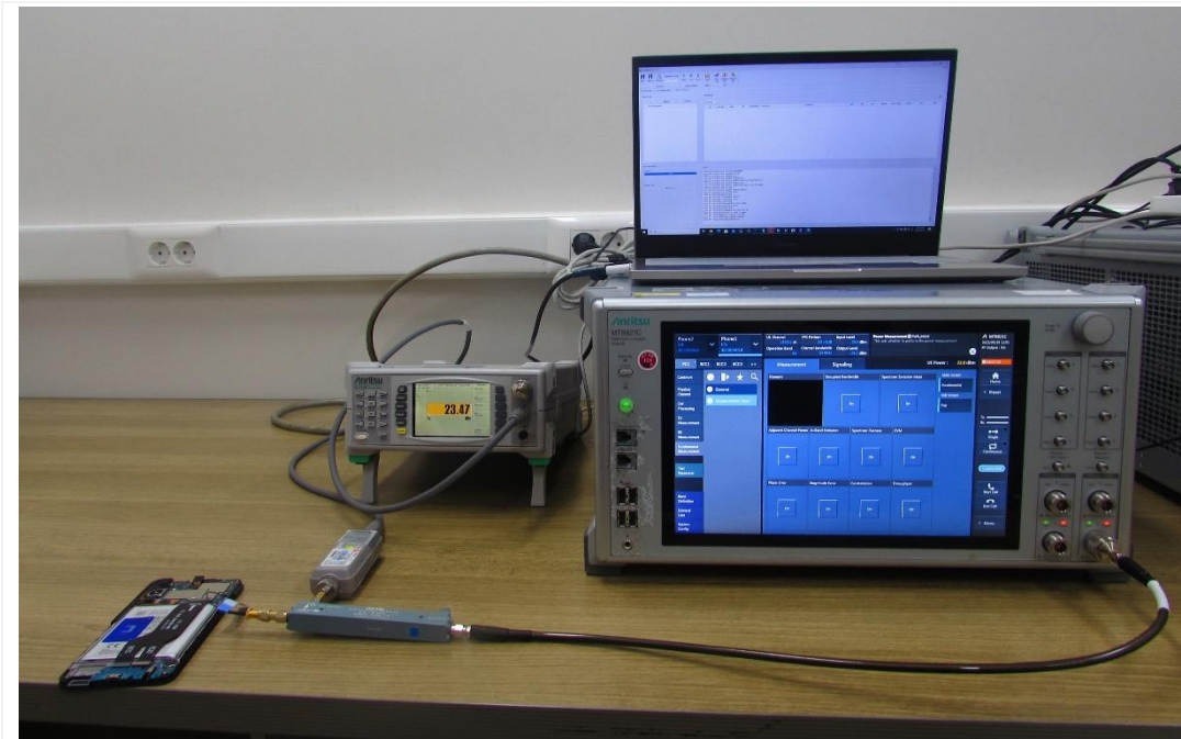
Test setup photo-1(Legacy)
