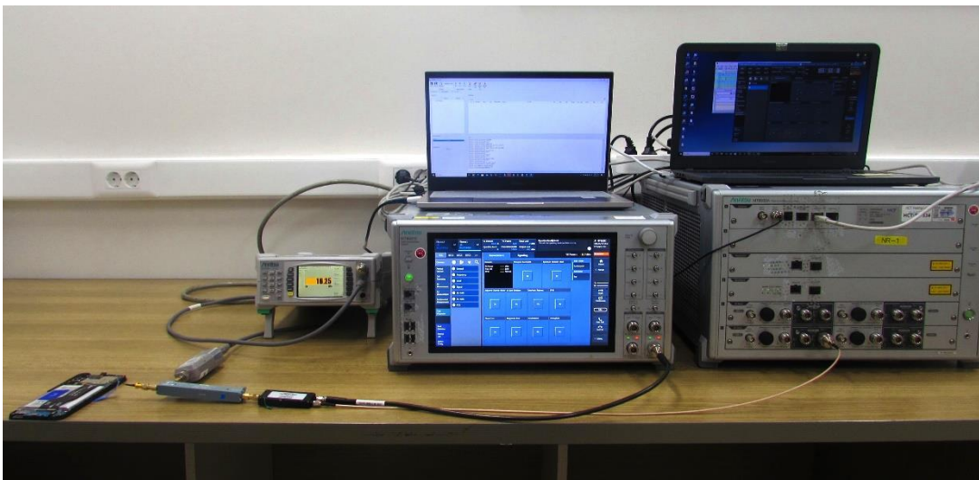
Test setup photo-4(NR SA)
