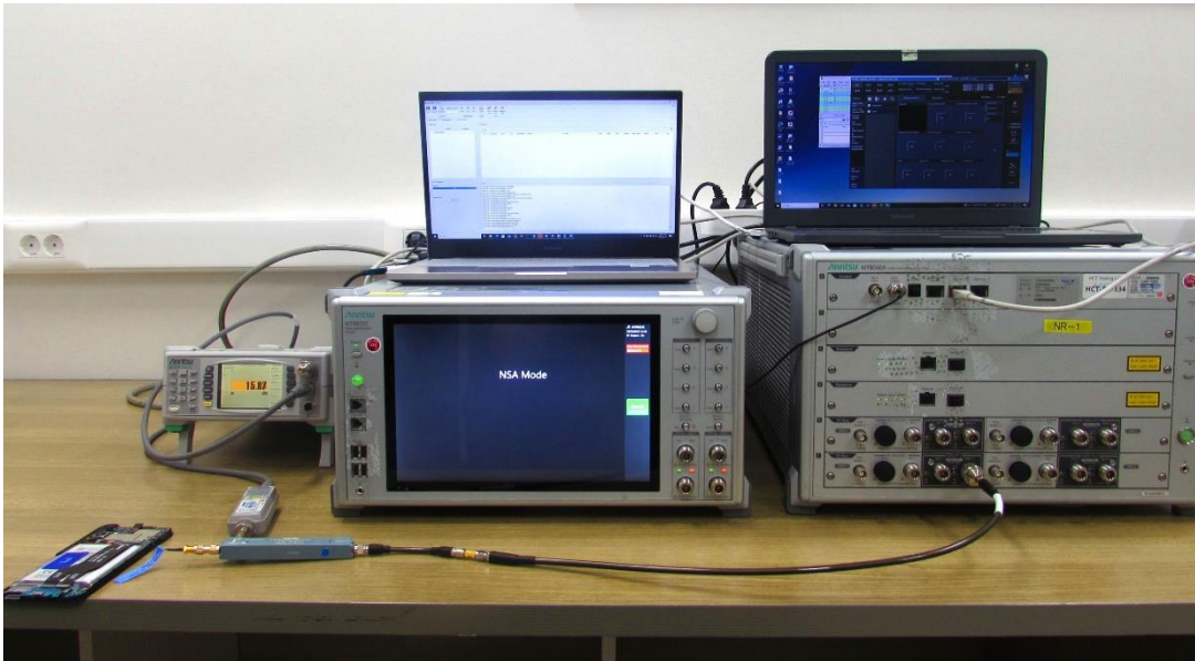
Test setup photo-3(NR SA)
