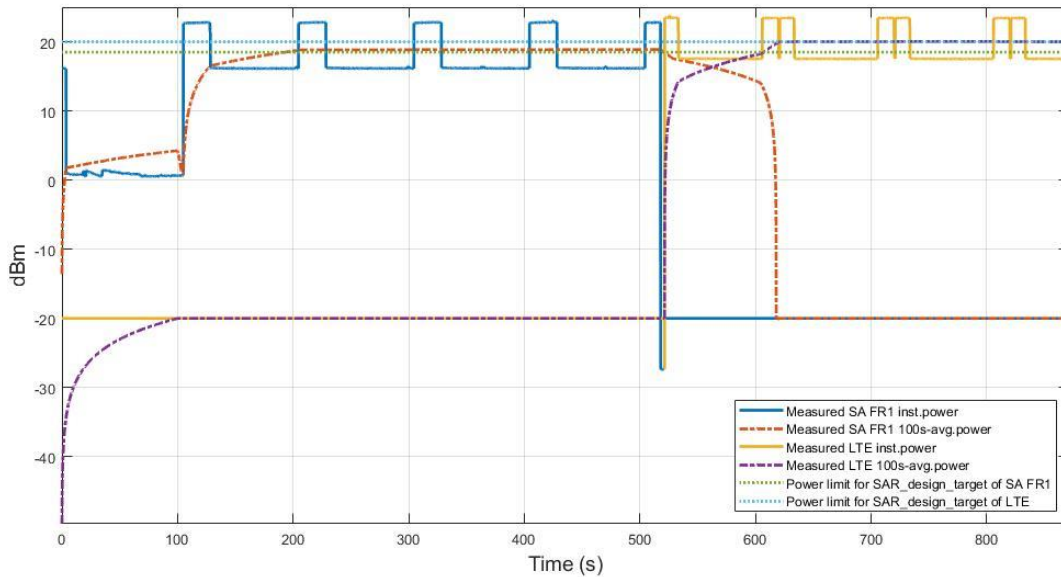
Figure 5.5-3 Conducted Tx power for SAR IRAT re-selection in test TC06 [n41 to LTE Band 66]
