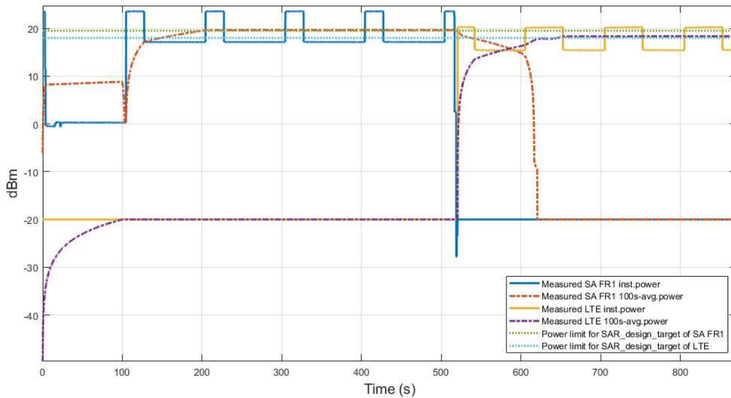
Figure 5.5-1 Conducted Tx power for SAR IRAT re-selection in test TC06 [n66 to LTE Band 41]
