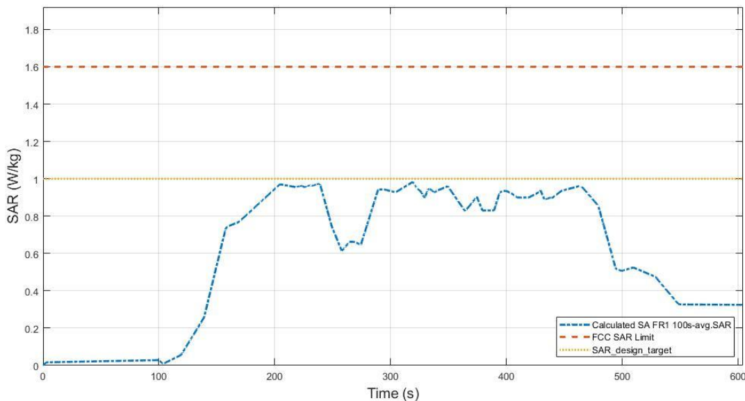
Figure 5.3-16 Total time-averaged SAR in TC04
