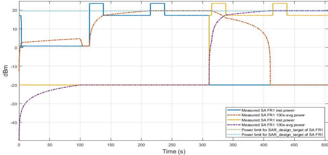
Figure 5.7-1 Conducted Tx power for SAR RSI change FR1 n66 in test TC8
