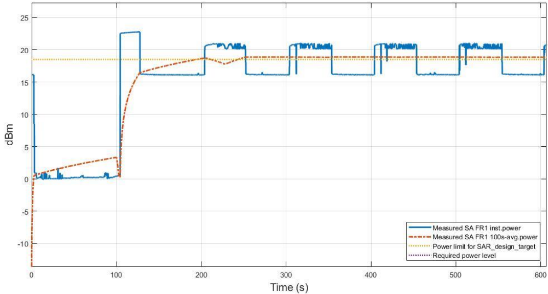
Figure 5.3-5 Time-average conducted power of SA FR1 n41 in TC02
