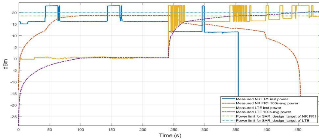
Figure 5.6-1 Time average SAR of LTE Band 66 and FR1 n41 EN-DC case
