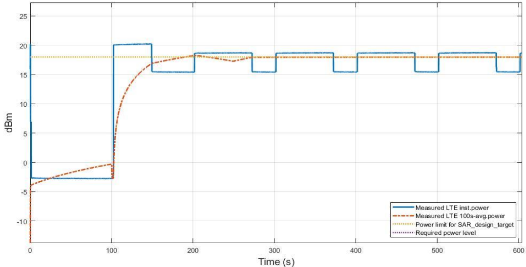
Figure 5.3-1 Time average conducted power of LTE B41 in TC01
