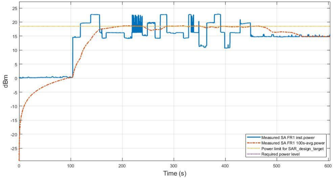
Figure 5.3-13 Conducted Tx power for SA FR1 n41 in TC04
