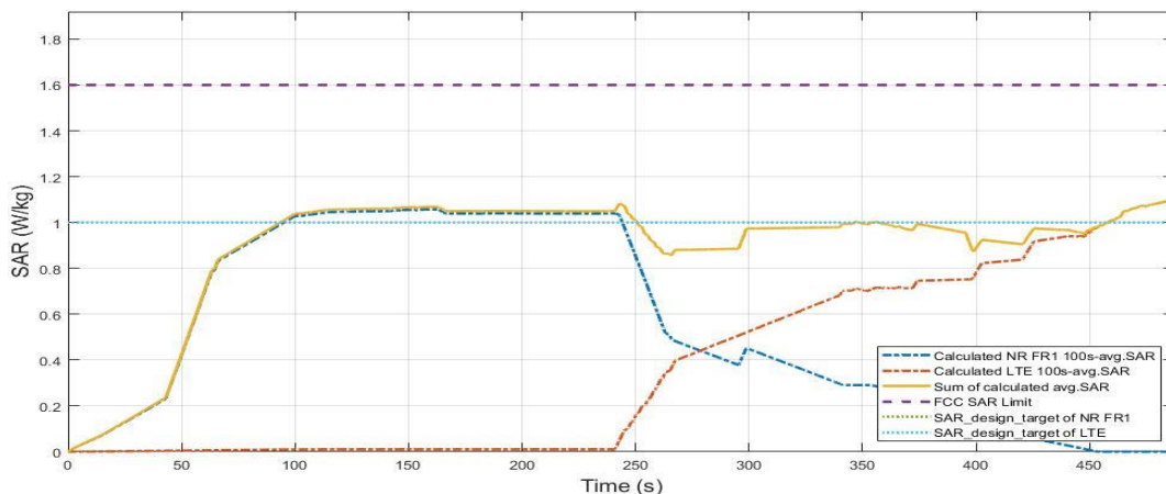
Figure 5.6-2 Total time-averaged SAR in TC07
