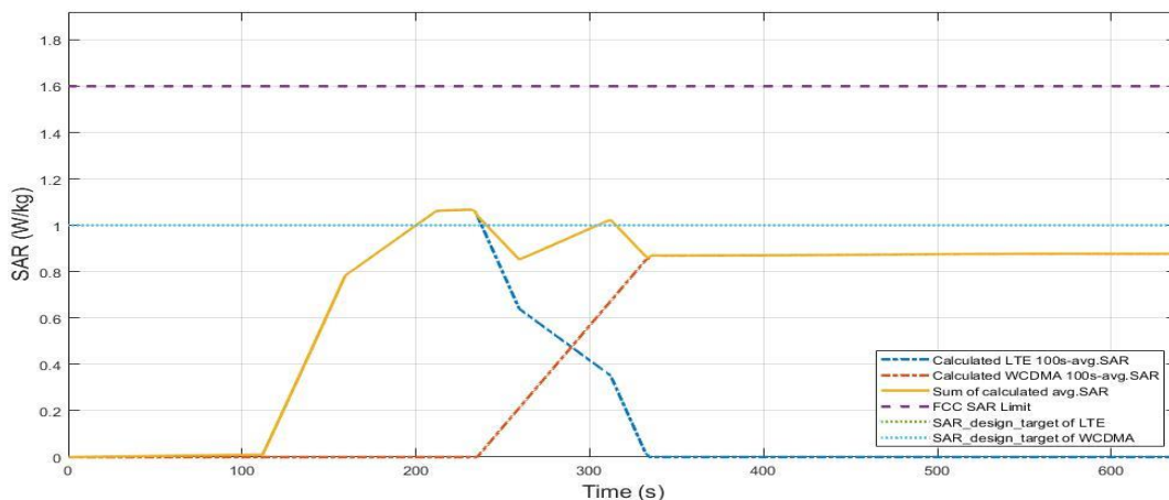
Figure 5.8-2 Total time-averaged SAR in TC14
