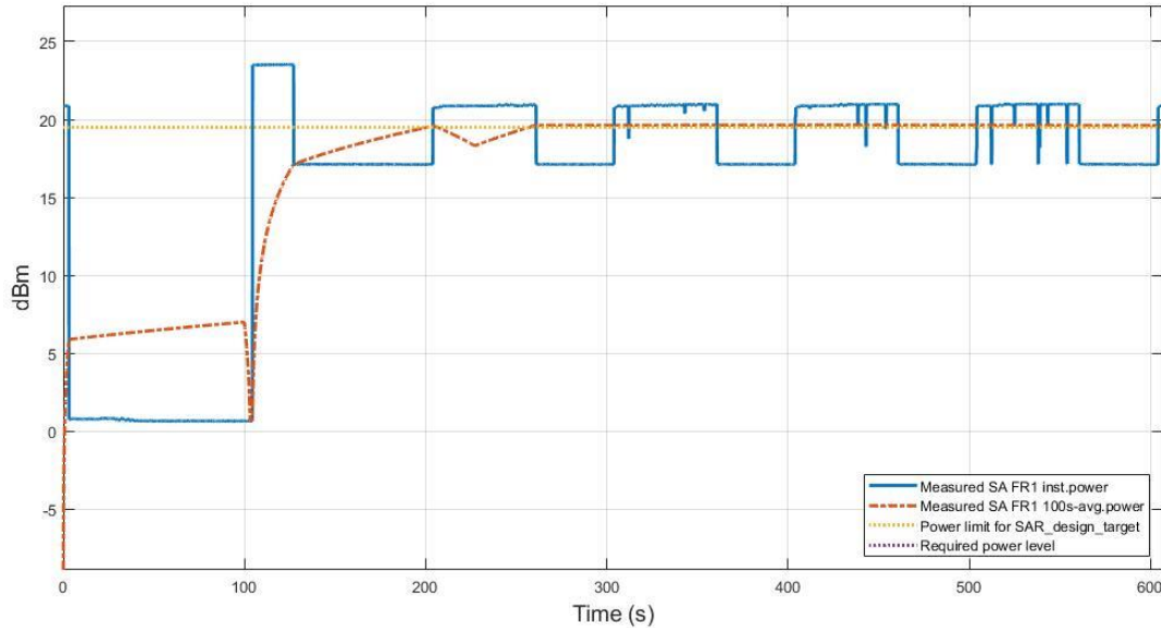
Figure 5.3-7 Time-average conducted power of SA FR1 n66 in TC02
