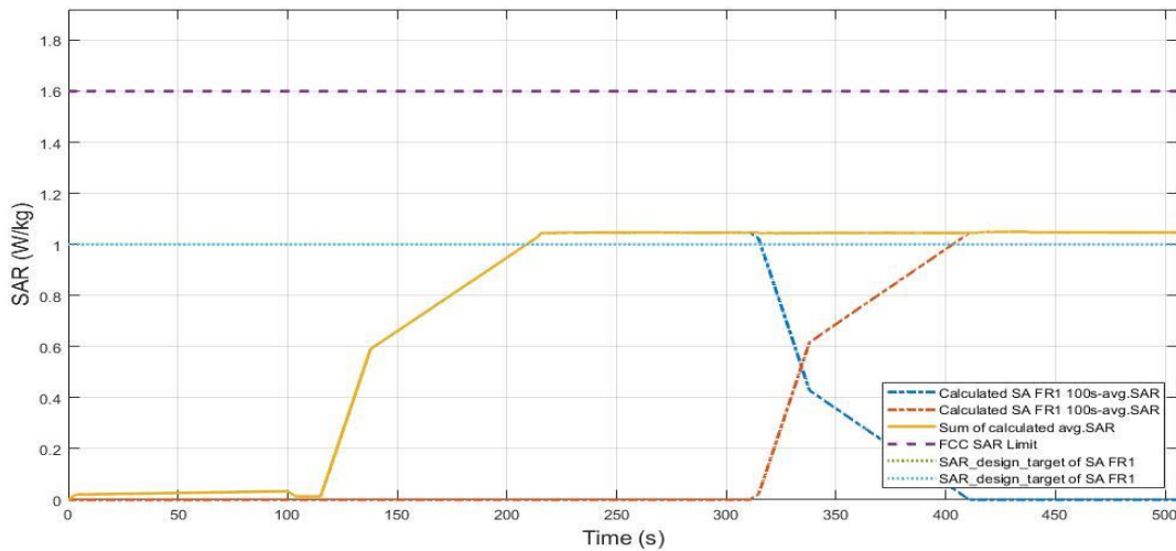
Figure 5.7-2 Total time-averaged SAR FR1 n66 in TC13
