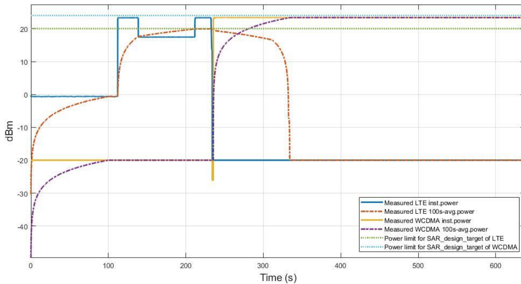
Figure 5.8-3 Conducted Tx power for SAR TAS to non TAS H.O. in test TC9
