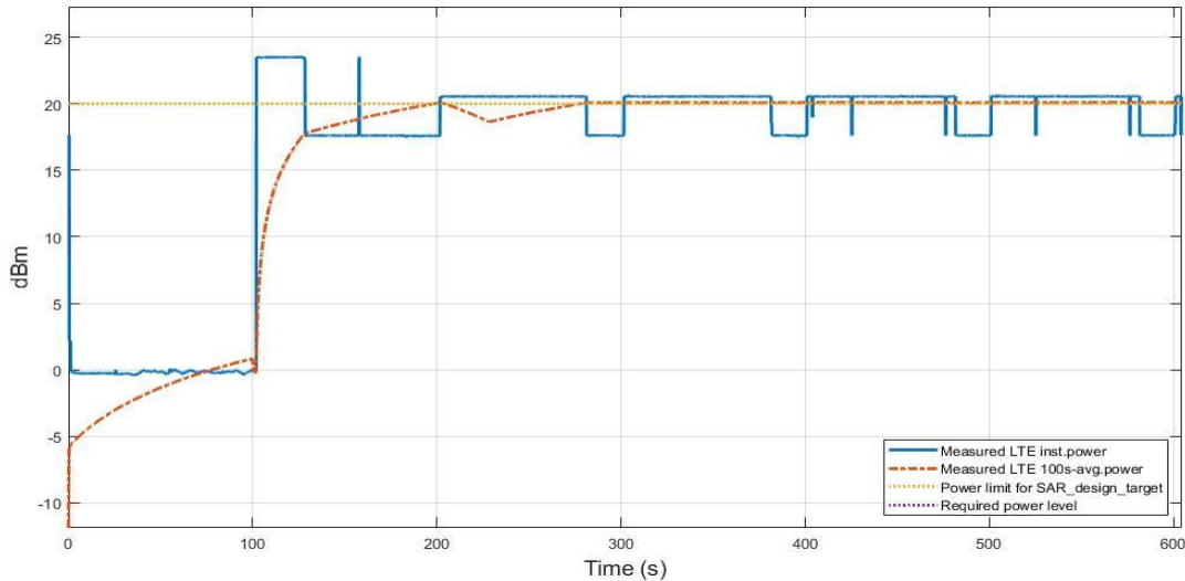
Figure 5.3-3 Time average conducted power of LTE B66 in TC01
