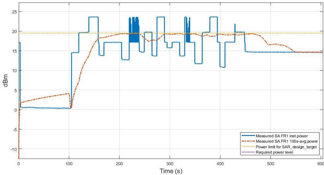
Figure 5.3-15 Conducted Tx power for SA FR1 n66 in TC04
