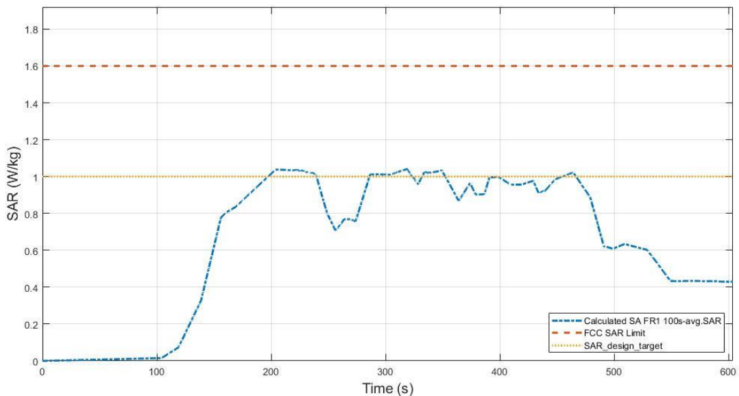
Figure 5.3-14 Total time-averaged SAR in TC04
