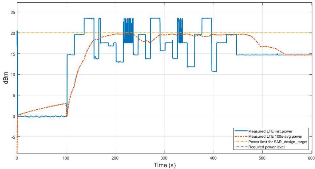
Figure 5.3-11 Conducted Tx power of LTE B66 in TC03
