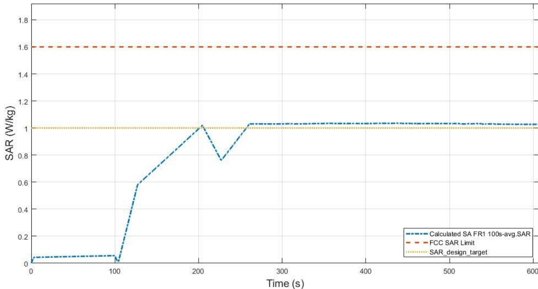
Figure 5.3-8 Total time-averaged SAR in TC02
