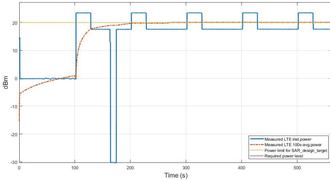
Figure 5.4-3 Conducted Tx power in Call_Disconnect_Re-establishment LTE Band 66 case TC05
