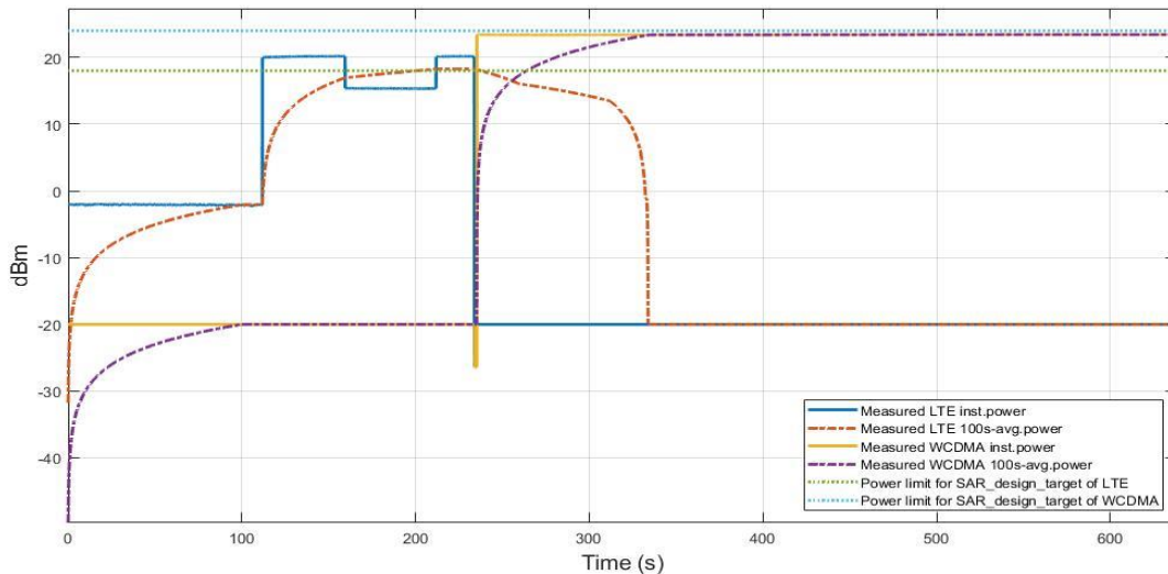
Figure 5.8-1 Conducted Tx power for SAR TAS to nonTAS H.O. in test TC9
