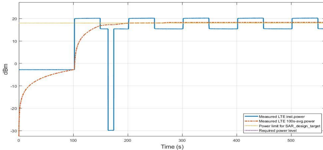
Figure 5.4-1 Conducted Tx power in Call_Disconnect_Reestablishment LTE Band 41 case TC05
