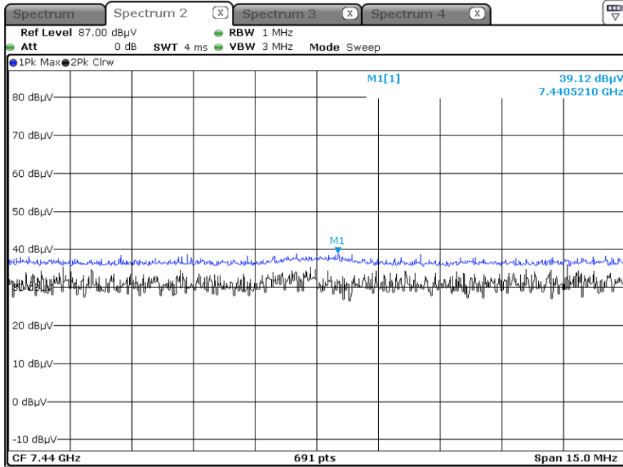
Radiated Spurious Emissions plot – Average & Peak Result ( \pi /4DQPSK, Ch.78 3rd Harmonic, Y-H)
