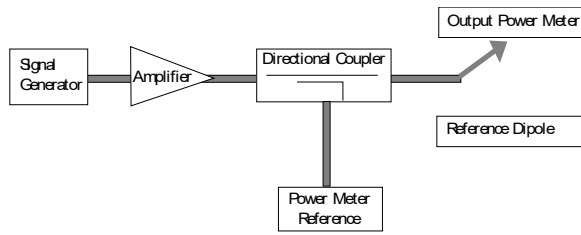
Figure 6-2 Setup for Desired Output Power to Dipole
