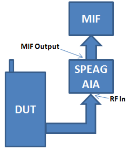
Figure 7-2 MIF Measurement Setup for unlicensed modes
