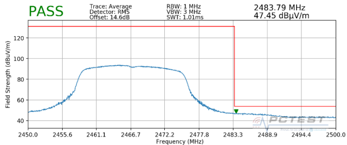
Plot 7-47. Radiated Restricted Band Edge Measurement (Average)
