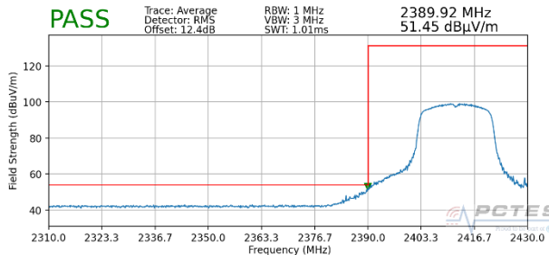
Plot 7-41. Radiated Restricted Lower Band Edge Measurement (Average)
