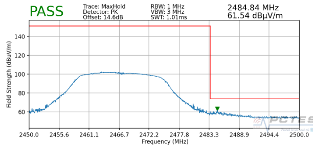
Plot 7-48. Radiated Restricted Band Edge Measurement (Peak)
