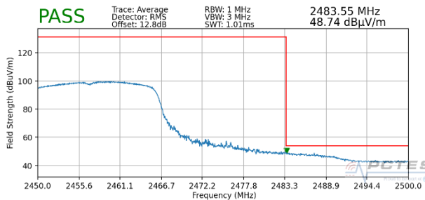
Plot 7-43. Radiated Restricted Upper Band Edge Measurement (Average)
