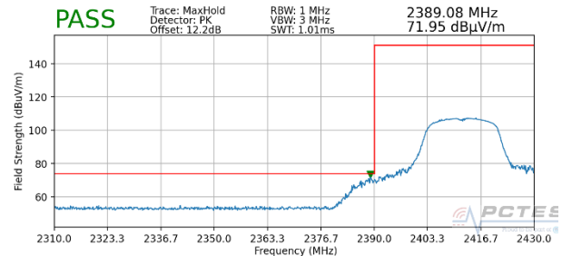
Plot 7-42. Radiated Restricted Lower Band Edge Measurement (Peak)
