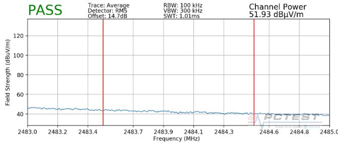
Plot 7-49. Radiated Restricted Band Edge Measurement (Average)
