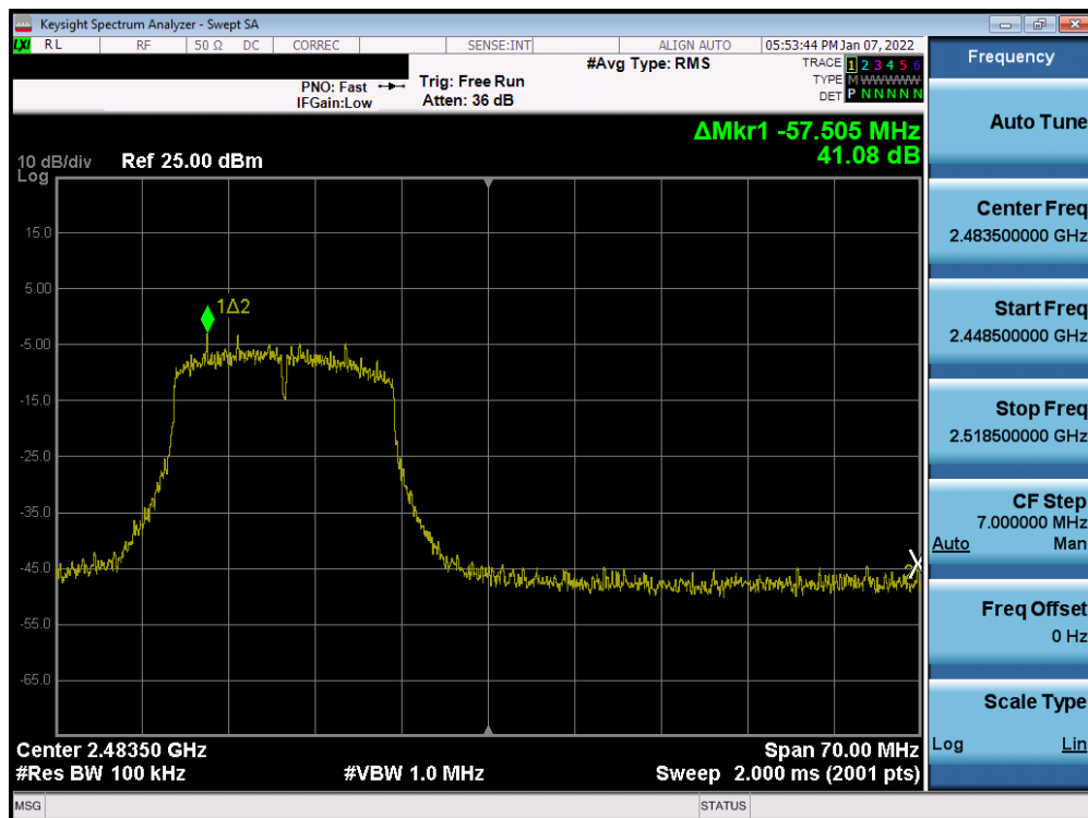
Plot 7-30. Band Edge Plot (802.11n (2.4GHz) – Ch. 12)
