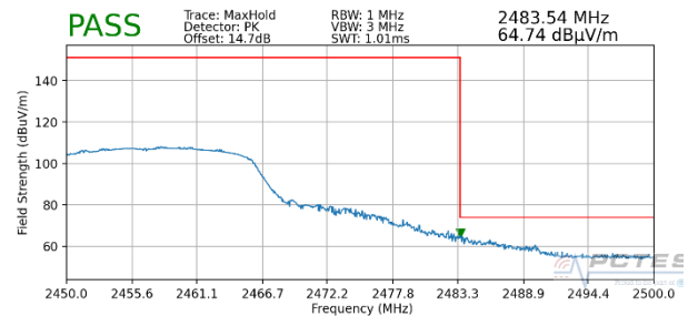
Plot 7-44. Radiated Restricted Upper Band Edge Measurement (Peak)
