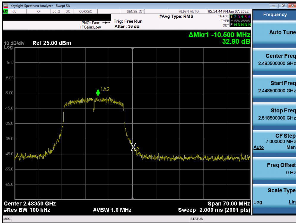
Plot 7-31. Band Edge Plot (802.11n (2.4GHz) – Ch. 13)
