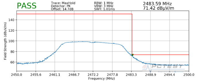
Plot 7-50. Radiated Restricted Band Edge Measurement (Peak)
