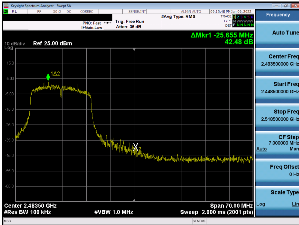
Plot 7-29. Band Edge Plot (802.11n (2.4GHz) – Ch. 11)
