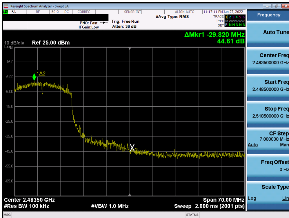
Plot 7-28. Band Edge Plot (802.11n (2.4GHz) – Ch. 10)
