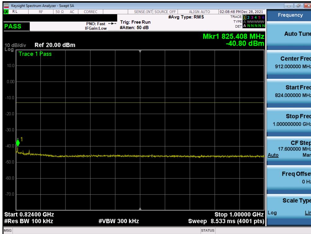
Plot 7-12. Conducted Spurious Plot (LTE Band 26 - 15MHz QPSK - RB Size 1, RB Offset 0 – Ant1)
