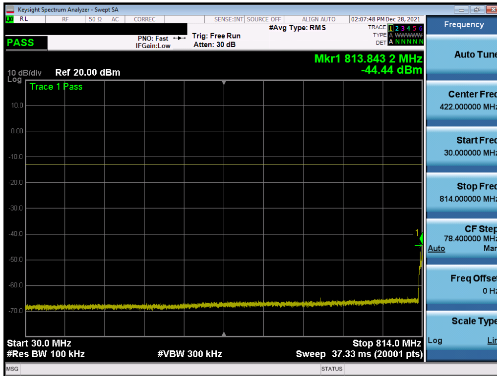
Plot 7-11. Conducted Spurious Plot (LTE Band 26 - 15MHz QPSK - RB Size 1, RB Offset 0 – Ant1)
