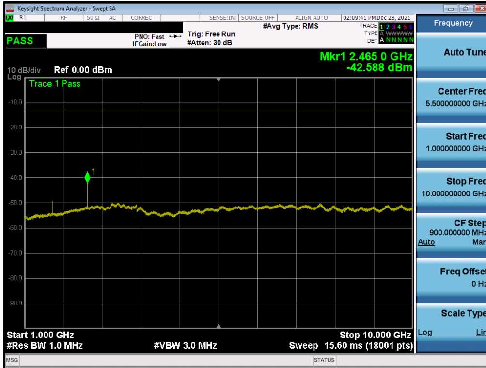
Plot 7-13. Conducted Spurious Plot (LTE Band 26 - 15MHz QPSK - RB Size 1, RB Offset 0 – Ant1)
