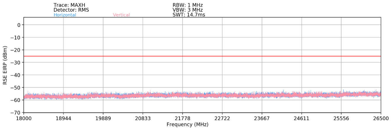
Plot 7-27. Radiated Spurious Plot – 18-26.5 GHz (LTE Band 41(PC3))
