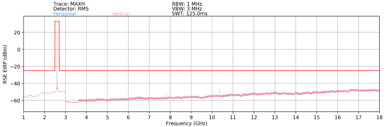
Plot 7-26. Radiated Spurious Plot – 1-18 GHz (LTE Band 41(PC3))
