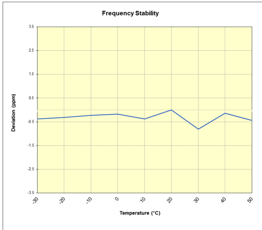
Plot 7-28. LTE Band 41(PC3) Frequency Stability Chart
