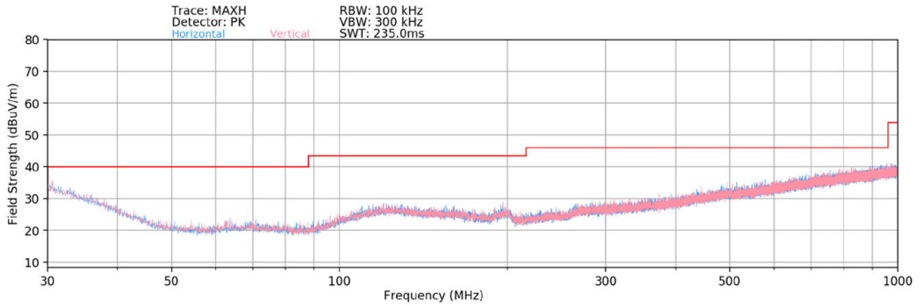
Plot 7-47. Radiated Spurious Plot below 1GHz
