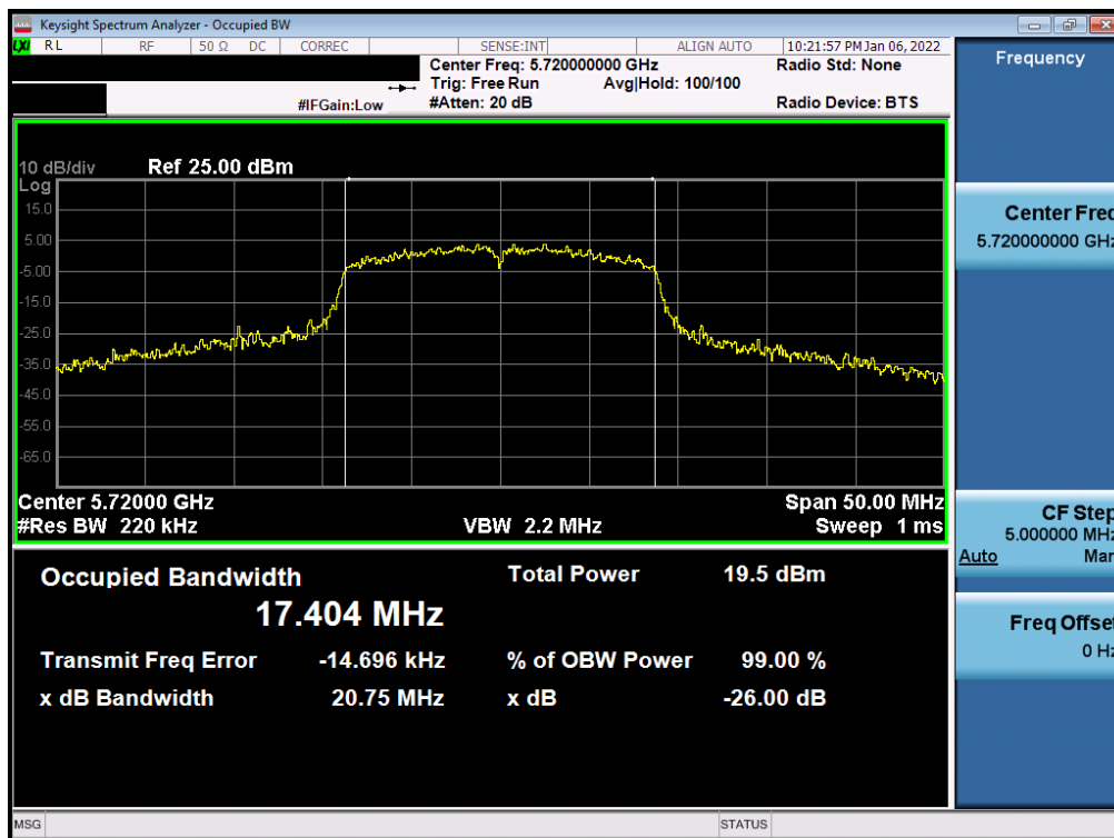
Plot 7-24. 26dB Bandwidth Plot (20MHz BW 802.11n (UNII Band 2C) – Ch. 140144)
