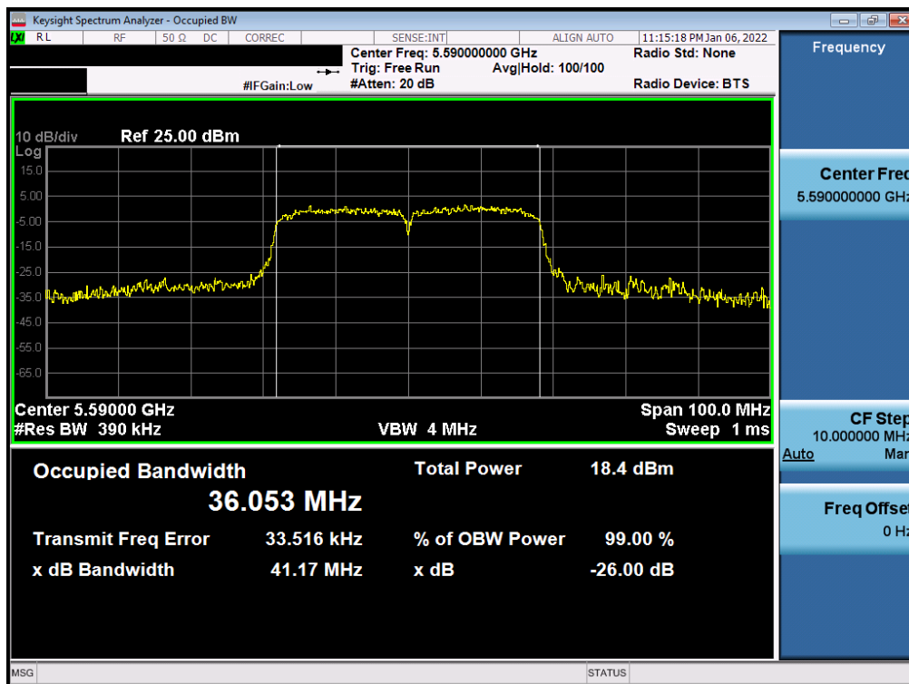
Plot 7-26. 26dB Bandwidth Plot (40MHz BW 802.11n (UNII Band 2C) – Ch. 110118)
