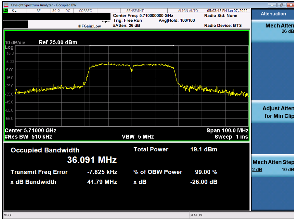
Plot 7-27. 26dB Bandwidth Plot (40MHz BW 802.11n (UNII Band 2C) – Ch. 134142)
