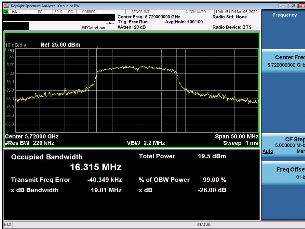
Plot 7-21. 26dB Bandwidth Plot (802.11a (UNII Band 2C) – Ch. 140144)
