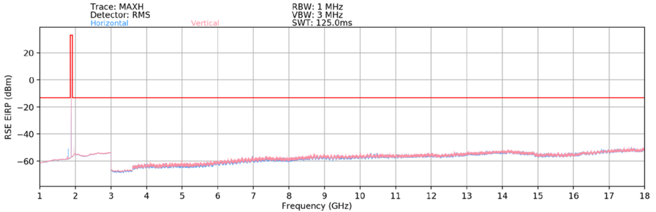
Plot 7-89. Radiated Spurious Plot (GPRS PCS)
