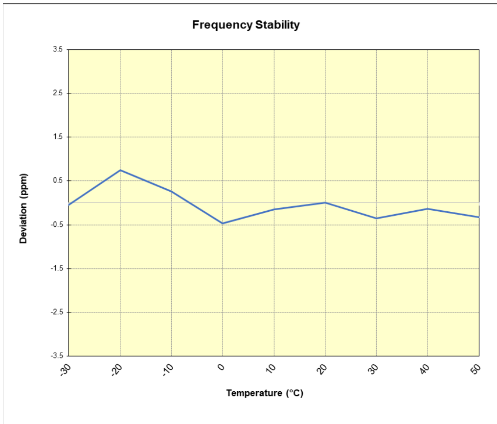
Plot 7-91. LTE Band 2 Frequency Stability Chart
