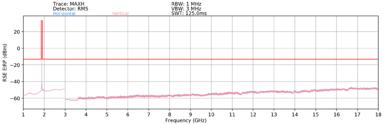
Plot 7-88. Radiated Spurious Plot (LTE Band 2)
