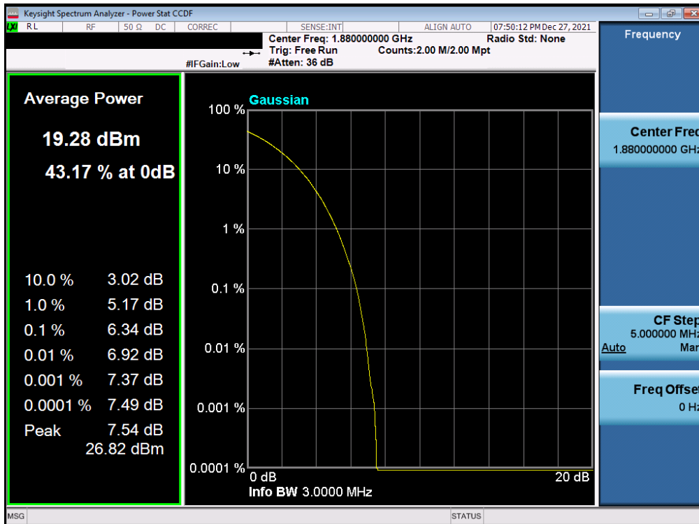
Plot 7-82. PAR Plot (LTE Band 2 - 3MHz 256-QAM - Full RB)
