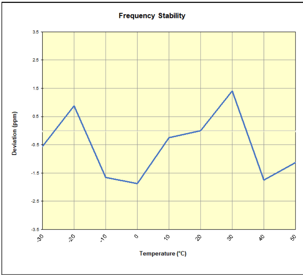
Plot 7-93. WCDMA PCS Frequency Stability Chart
