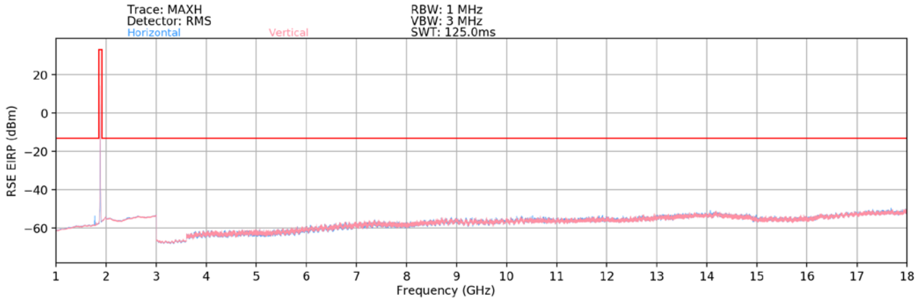
Plot 7-90. Radiated Spurious Plot (WCDMA PCS)
