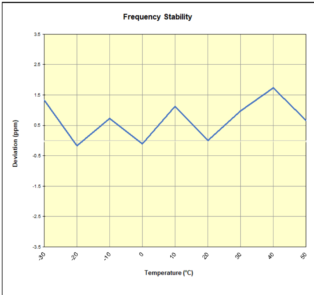
Plot 7-92. GSM/GPRS PCS Frequency Stability Chart
