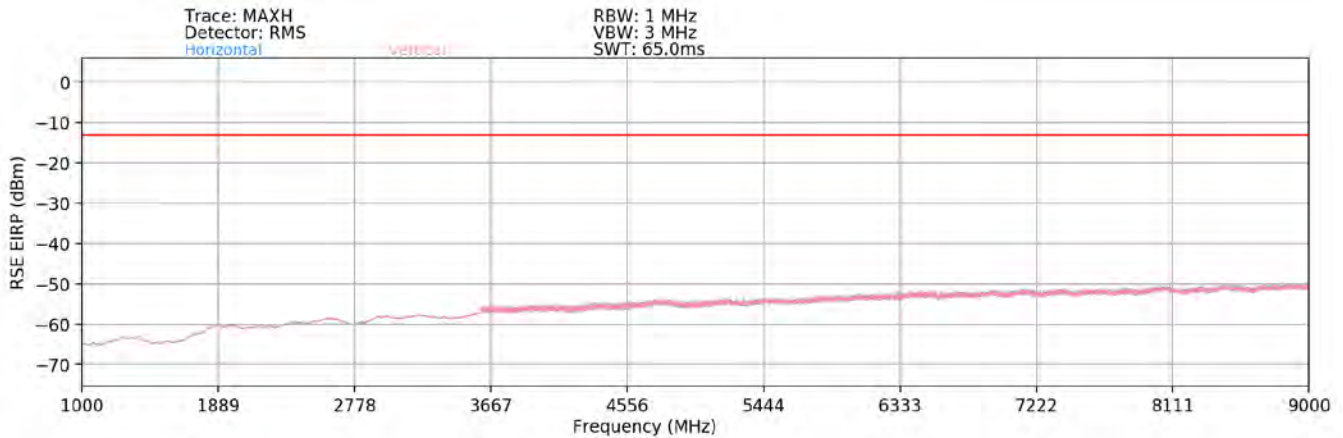
Plot 7-86. Radiated Spurious Plot (LTE Band 26/5)
