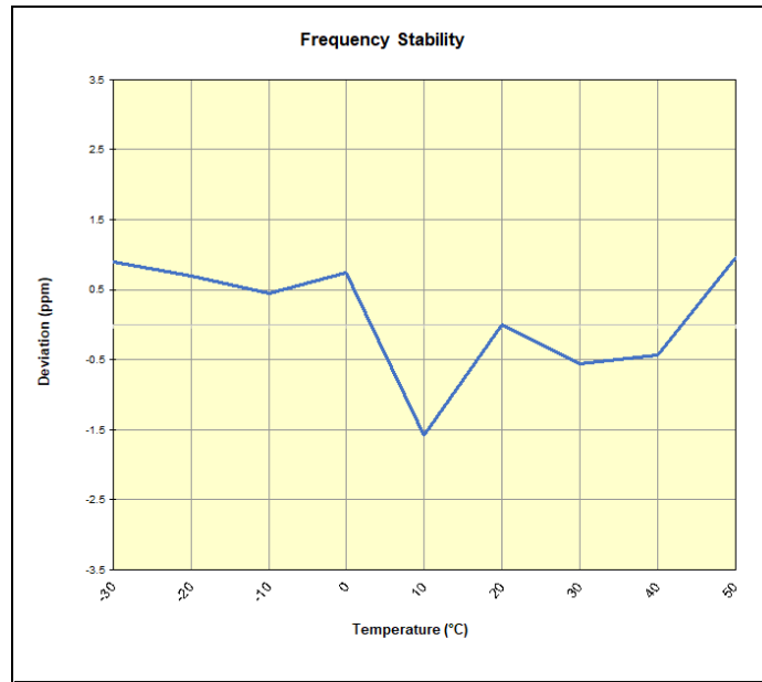
Plot 7-88. GSM/GPRS Cell Frequency Stability Chart
