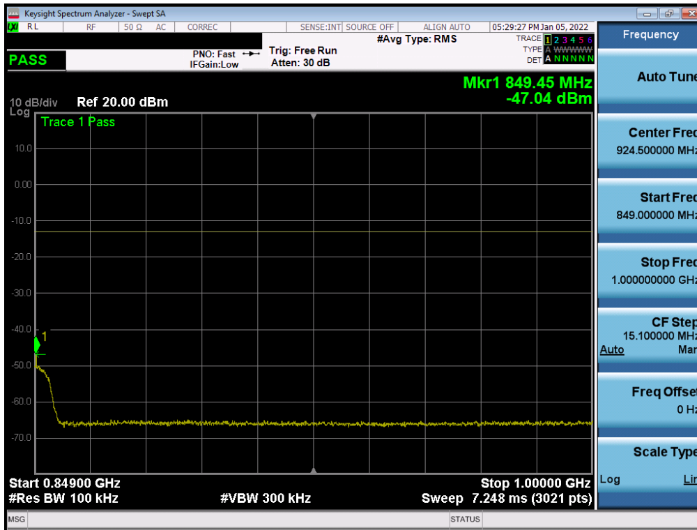
Plot 7-54. Conducted Spurious Plot (NR Band n5 - 20.0MHz - 1 RB - Low Channel)
