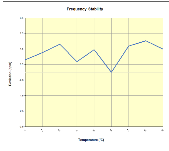
Plot 7-90. LTE Band 26/5 Frequency Stability Chart
