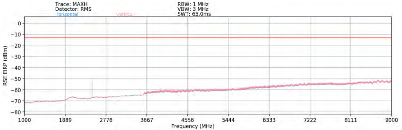
Plot 7-84. Radiated Spurious Plot (GPRS Cell)
