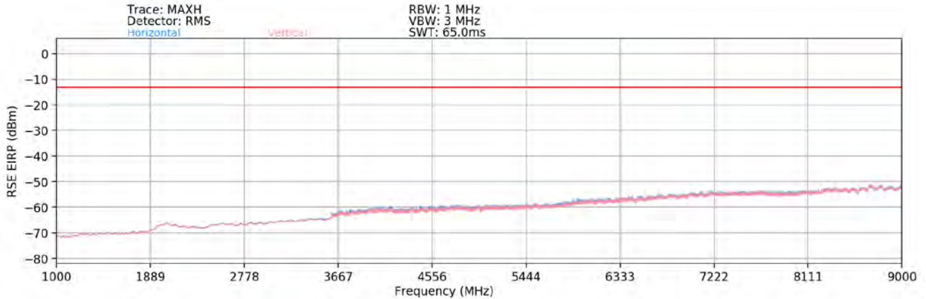
Plot 7-85. Radiated Spurious Plot (WCDMA Cell)
