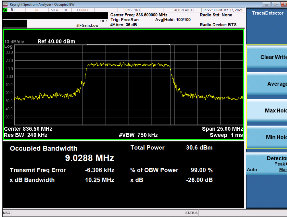
Plot 7-6. Occupied Bandwidth Plot (LTE Band 26/5 - 10MHz QPSK - Full RB)
