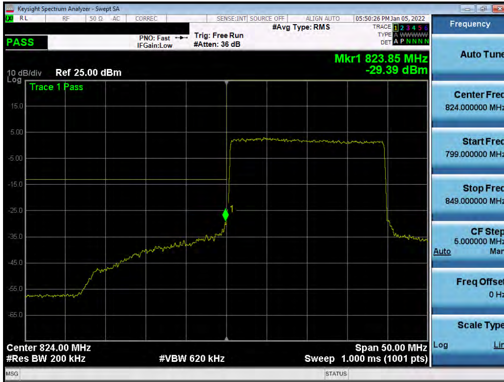
Plot 7-76. Lower Band Edge Plot (NR Band n5 – 20.0MHz - Full RB)
