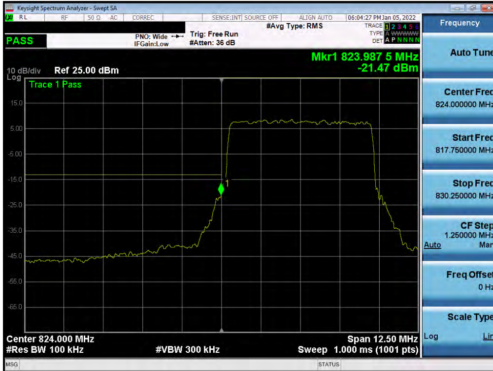
Plot 7-82. Lower Band Edge Plot (NR Band n5 – 5.0MHz - Full RB)
