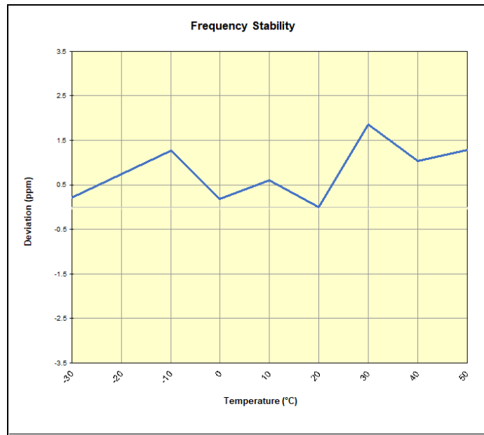
Plot 7-91. NR Band n5 Frequency Stability Chart
