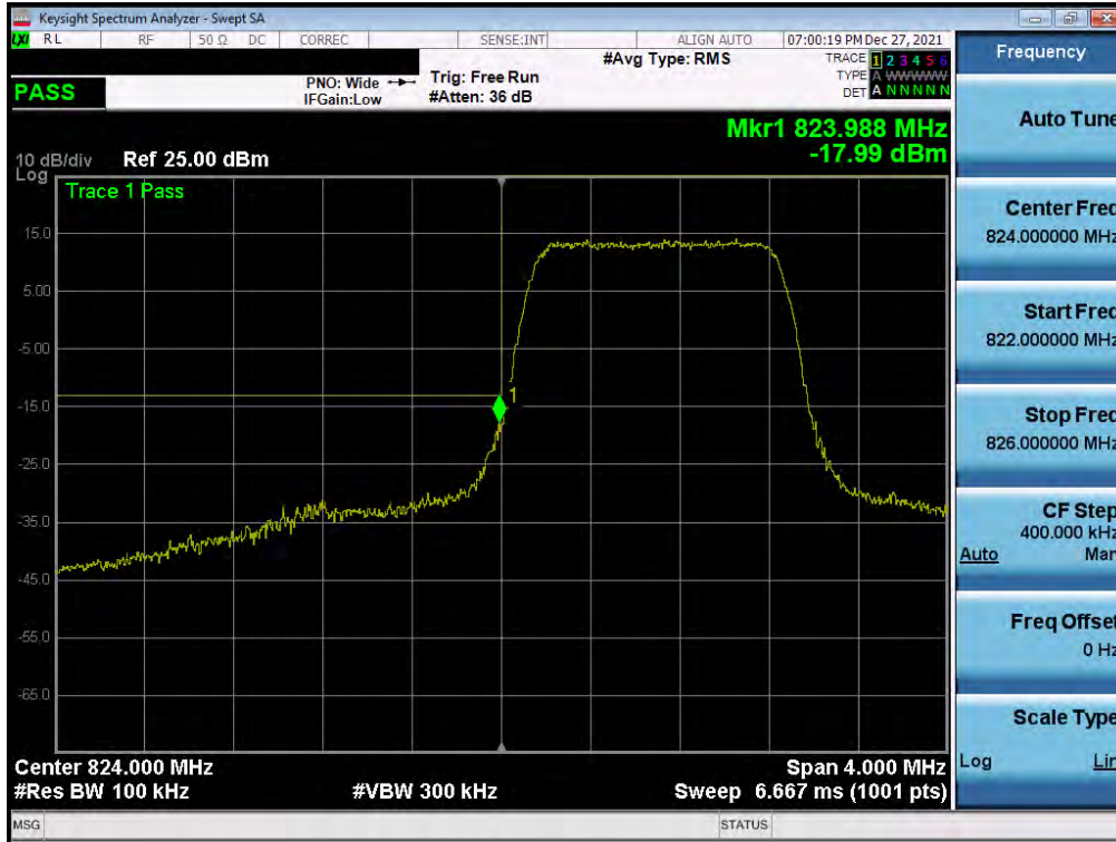
Plot 7-74. Lower Band Edge Plot (LTE Band 26/5 – 1.4MHz QPSK – Full RB)
