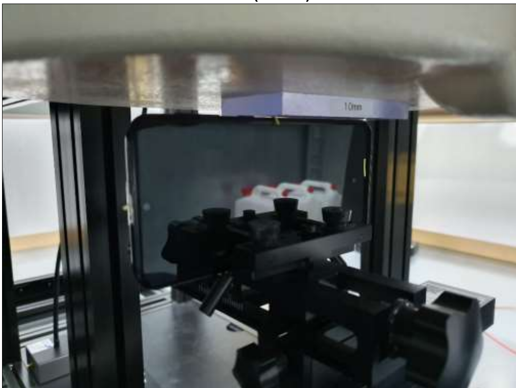
Rear (10mm)
