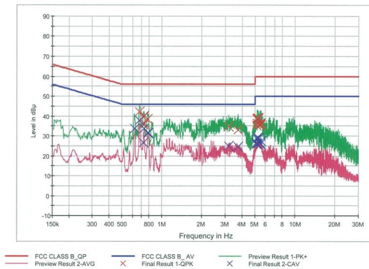
FCC CLASS B_Exten Cable
