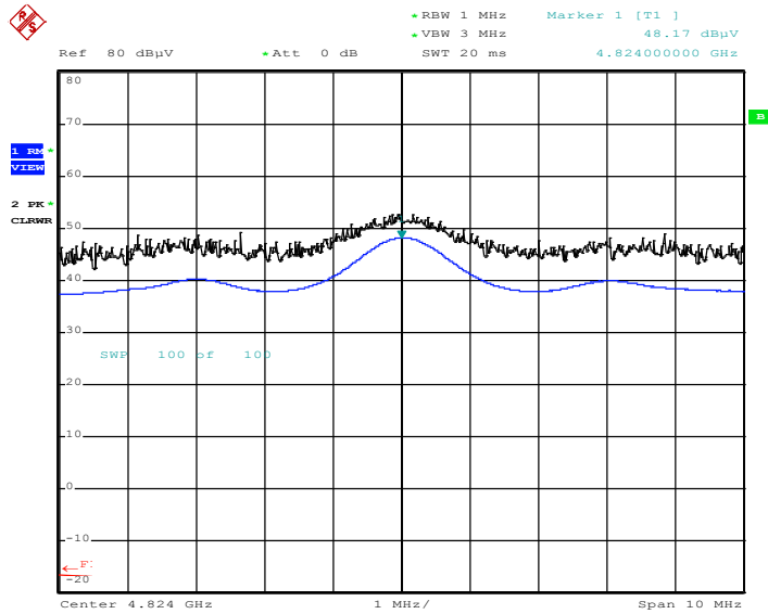
Radiated Spurious Emissions plot – Average Reading (802.11b, Ch.1 2nd Harmonic, X-H)
