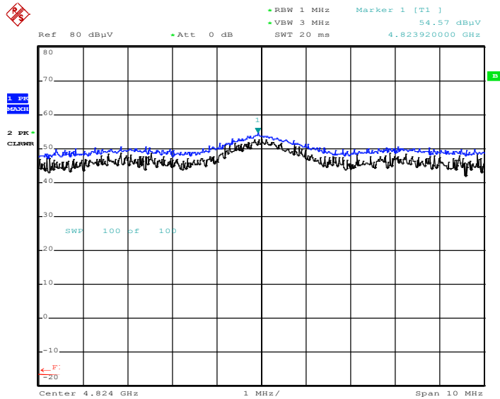
Radiated Spurious Emissions plot – Peak Reading (802.11b, Ch.1 2nd Harmonic, X-H)
