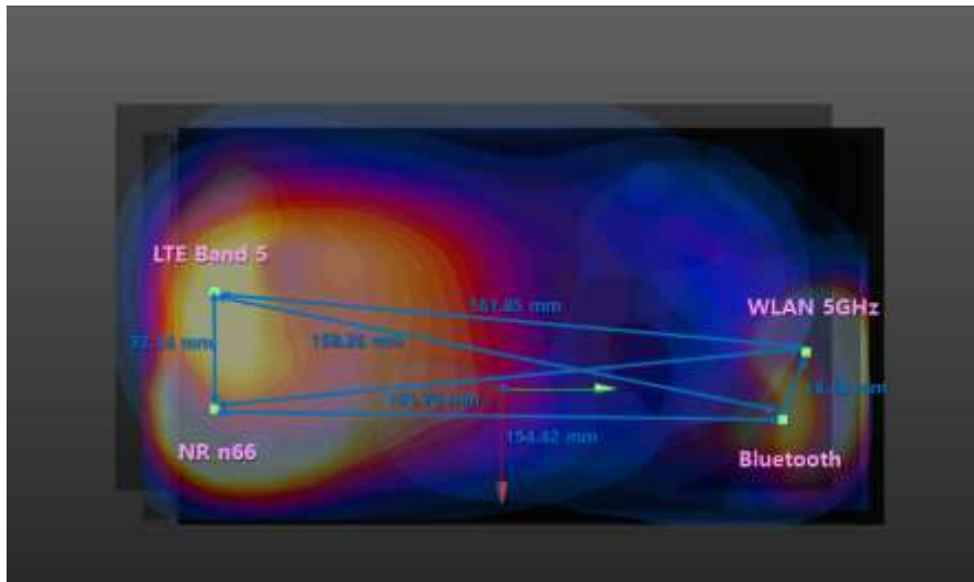
Plot #1 NR n66 + LTE Band 5 + WLAN 5GHz + Bluetooth
