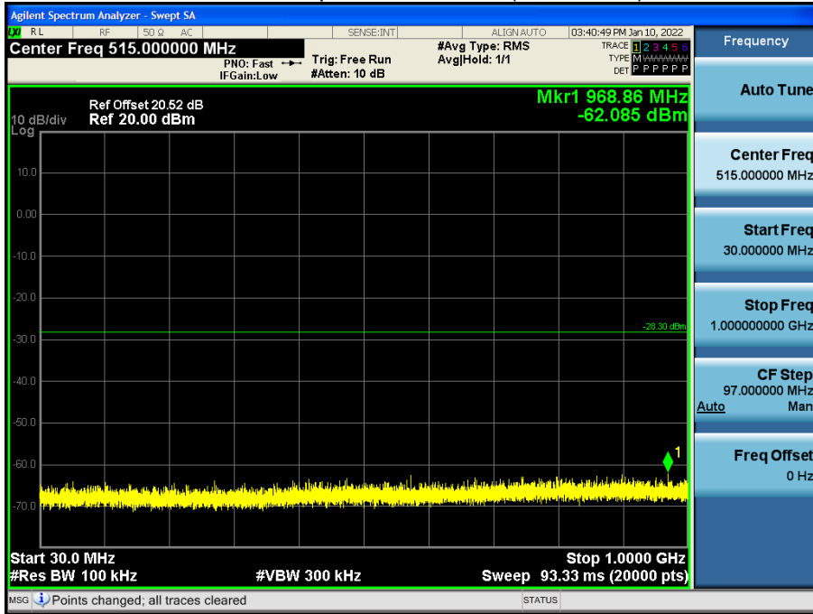
Conducted Spurious Emission (Low-CH 78)
